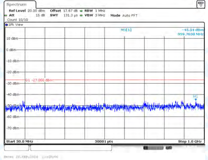
11AX40-CDD-Ant2-5550-30~1000-PASS
