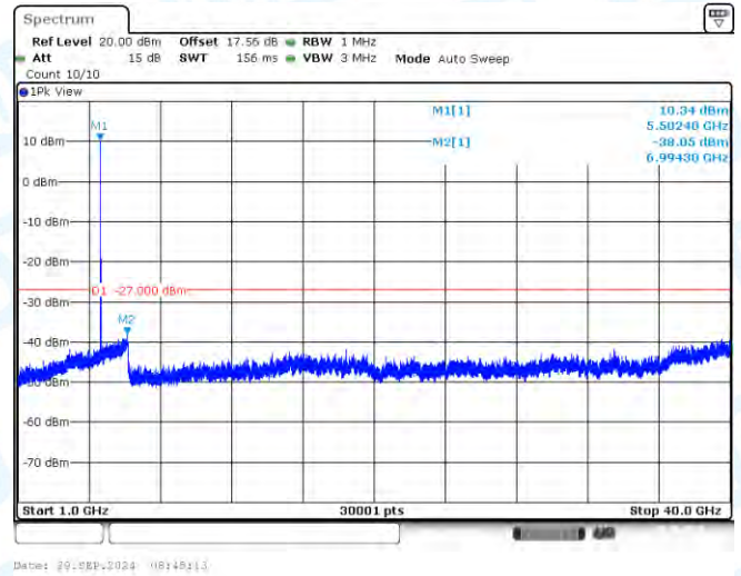
11AX20-CDD-Ant1-5500-1000~40000-PASS
