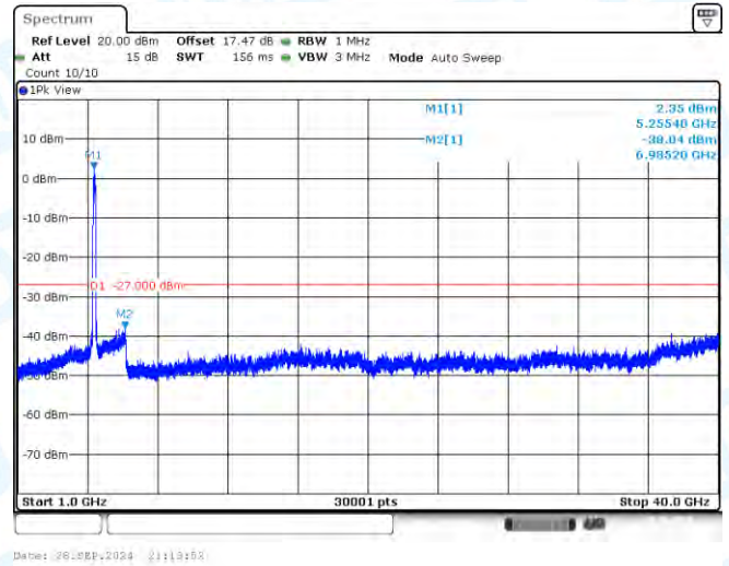
11AC160-CDD-Ant1-5250-1000~40000-PASS
