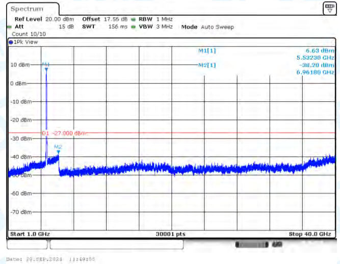
11AX80-CDD-Ant1-5530-1000~40000-PASS
