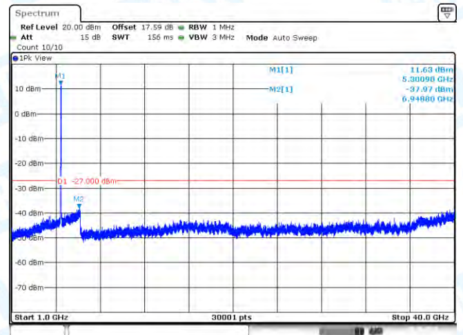
11AX40-CDD-Ant1-5310-1000~40000-PASS
