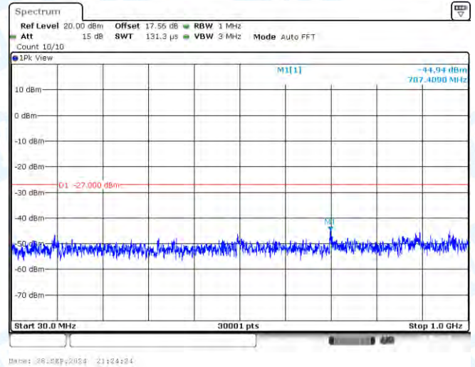
11AX160-CDD-Ant2-5250-30~1000-PASS
