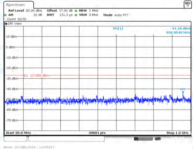
11AC80-CDD-Ant2-5690-30~1000-PASS
