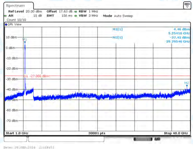
11AX160-CDD-Ant3-5250-1000~40000-PASS
