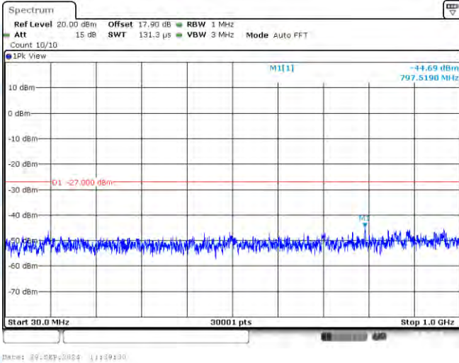
11AX40-CDD-Ant1-5710-30~1000-PASS
