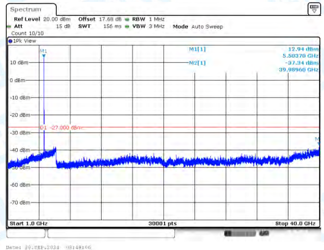
11AX20-CDD-Ant3-5500-1000~40000-PASS
