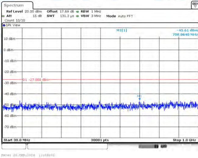
11AX80-CDD-Ant3-5530-30~1000-PASS
