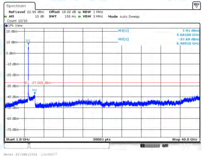
11AC80-CDD-Ant3-5690-1000~40000-PASS
