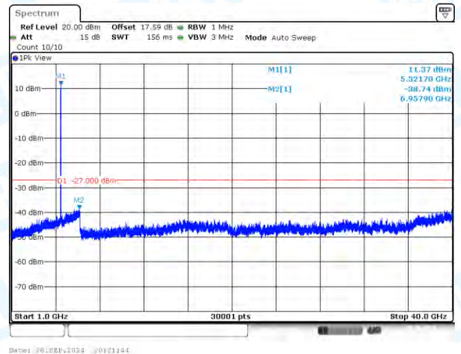
11AX20-CDD-Ant3-5320-1000~40000-PASS
