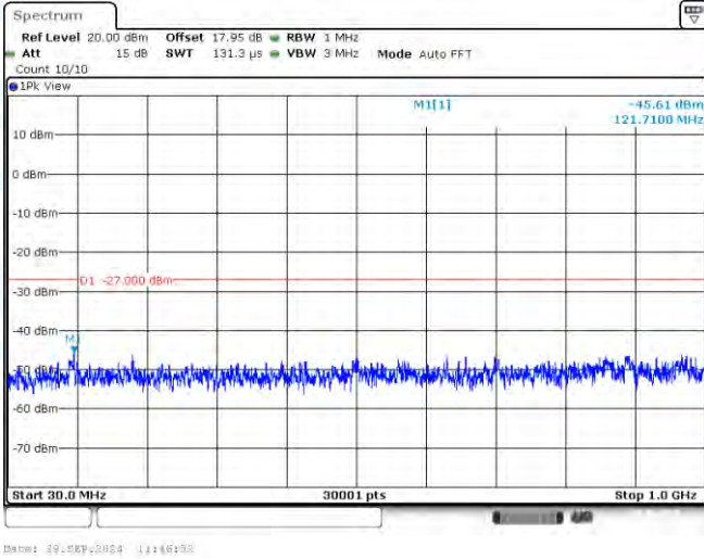
11AX40-CDD-Ant3-5710-30~1000-PASS
