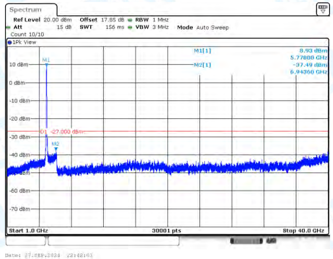
11AC80-CDD-Ant3-5775-1000~40000-PASS
