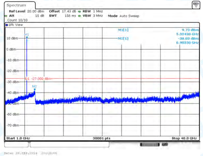
11AX20-CDD-Ant1-5320-1000~40000-PASS
