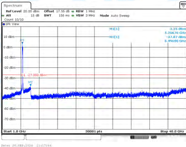
11AC160-CDD-Ant2-5250-1000~40000-PASS
