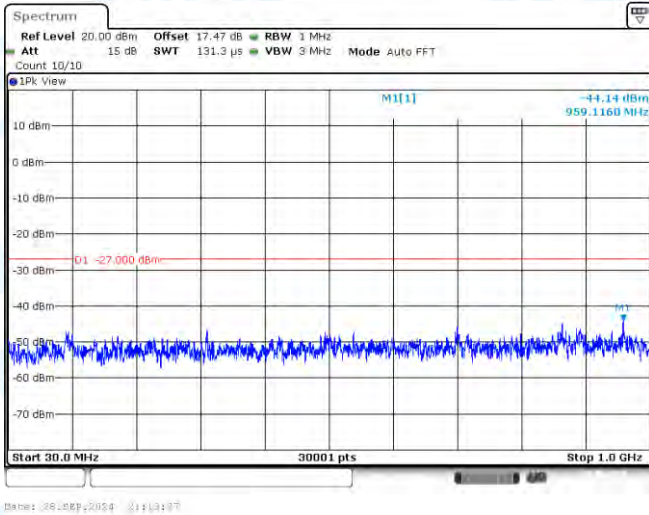
11AC160-CDD-Ant1-5250-30~1000-PASS
