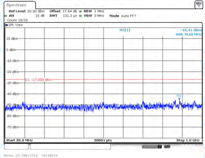
11AX20-CDD-Ant2-5500-30~1000-PASS
