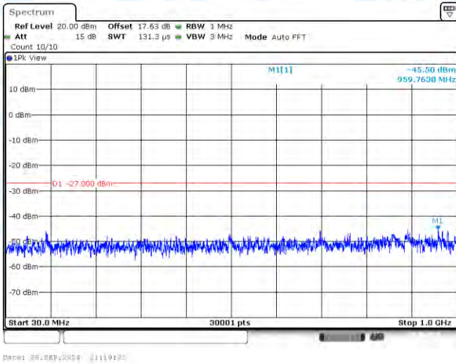
11AC160-CDD-Ant3-5250-30~1000-PASS
