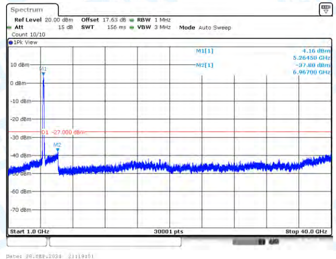
11AC160-CDD-Ant3-5250-1000~40000-PASS
