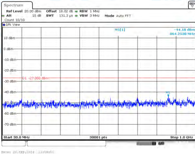
11AC80-CDD-Ant3-5690-30~1000-PASS
