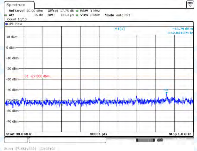
11AX20-CDD-Ant2-5745-30~1000-PASS
