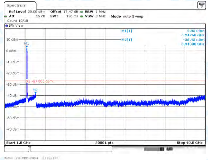
11AX160-CDD-Ant1-5250-1000~40000-PASS
