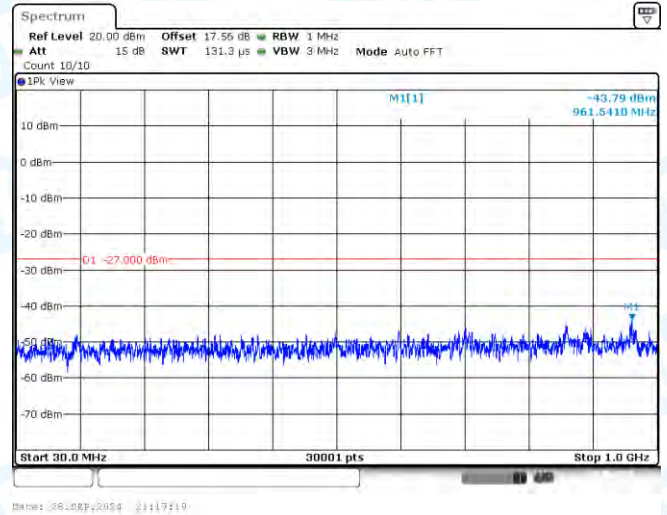
11AC160-CDD-Ant2-5250-30~1000-PASS
