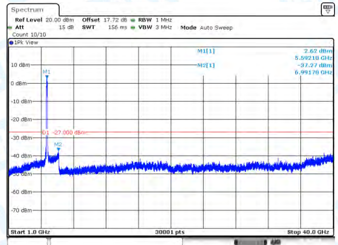
11AC160-CDD-Ant1-5570-1000~40000-PASS
