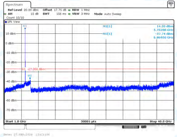
11AX20-CDD-Ant1-5745-1000~40000-PASS
