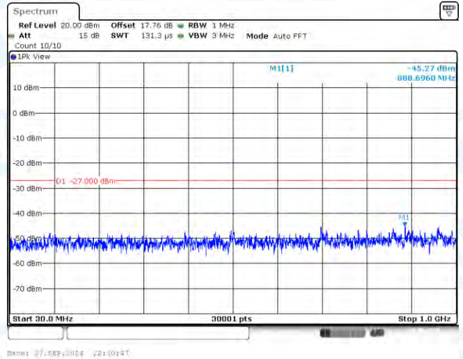
11AC80-CDD-Ant2-5775-30~1000-PASS
