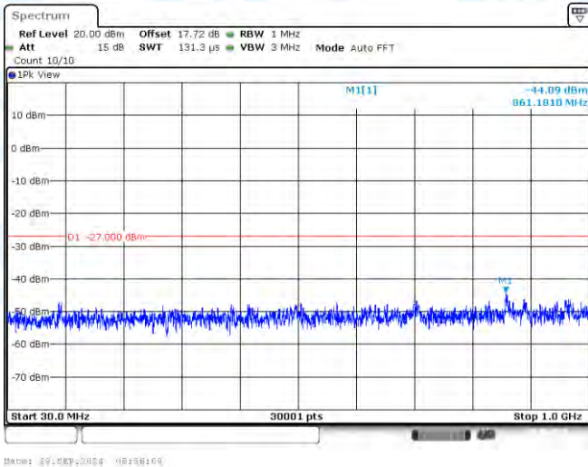
11AX20-CDD-Ant3-5580-30~1000-PASS
