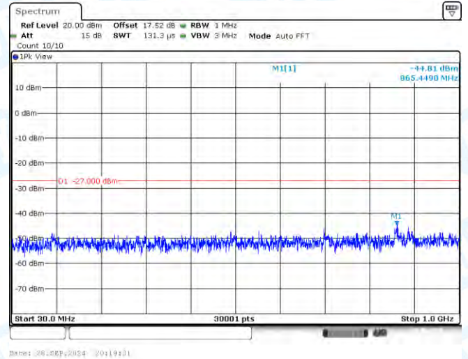
11AX20-CDD-Ant2-5320-30~1000-PASS
