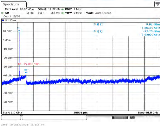
11AX40-CDD-Ant2-5270-1000~40000-PASS
