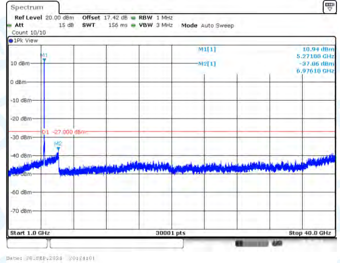
11AX40-CDD-Ant1-5270-1000~40000-PASS
