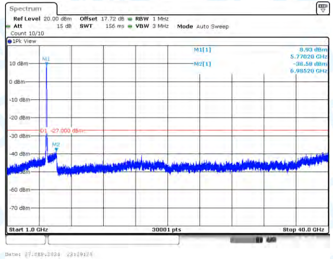
11AC80-CDD-Ant1-5775-1000~40000-PASS
