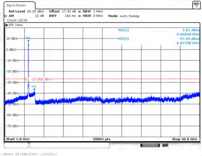
11AC80-CDD-Ant1-5690-1000~40000-PASS
