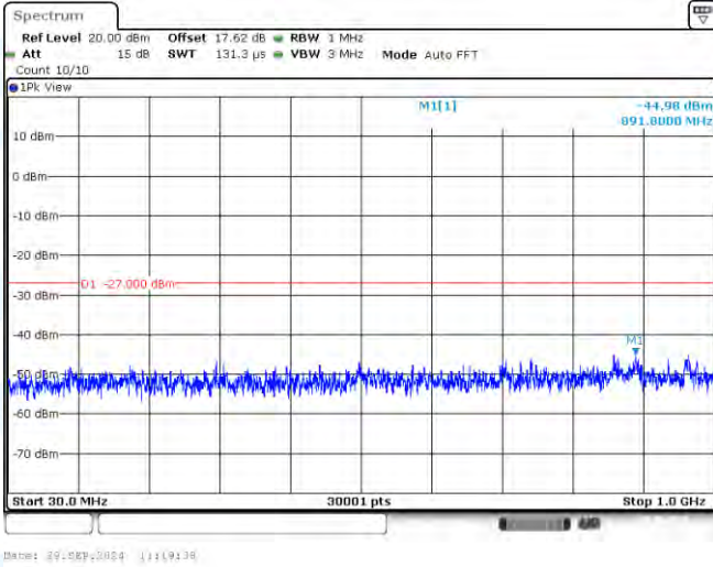
11AX40-CDD-Ant1-5550-30~1000-PASS
