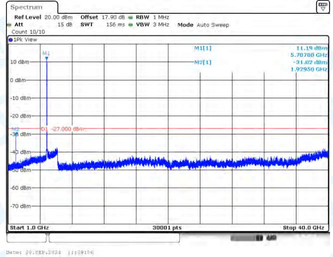
11AX40-CDD-Ant1-5710-1000~40000-PASS
