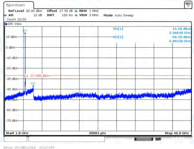
11AX40-CDD-Ant3-5270-1000~40000-PASS
