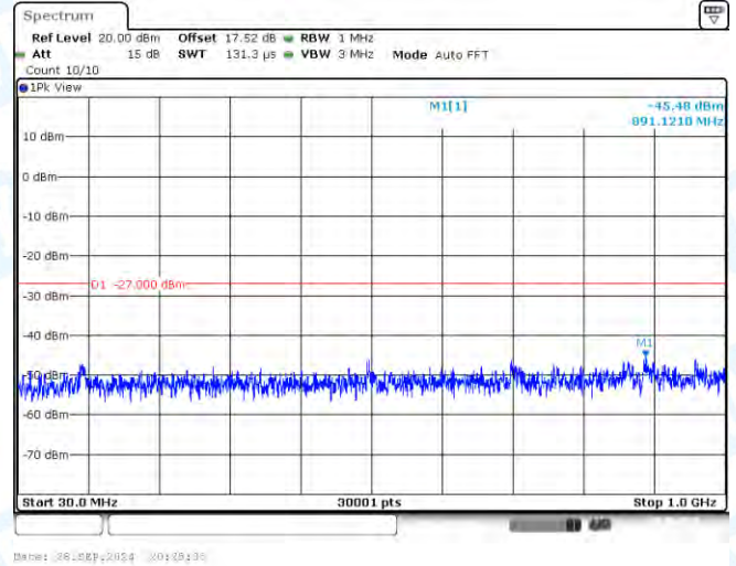
11AX40-CDD-Ant2-5270-30~1000-PASS
