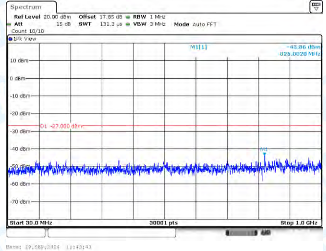
11AX40-CDD-Ant2-5710-30~1000-PASS
