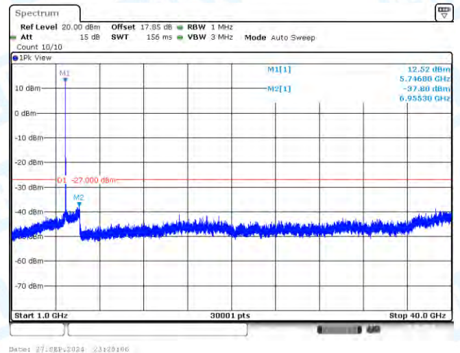
11AX20-CDD-Ant3-5745-1000~40000-PASS
