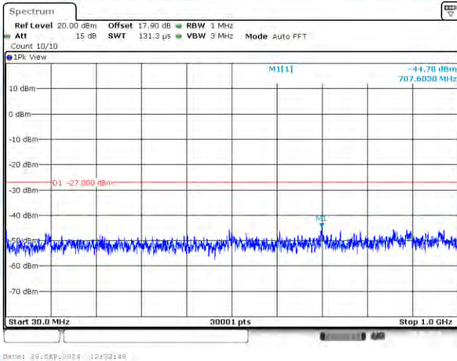
11AC80-CDD-Ant1-5690-30~1000-PASS
