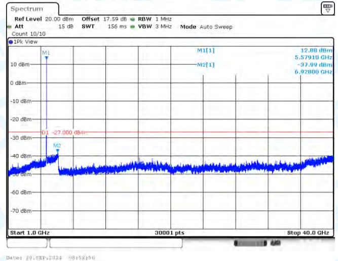
11AX20-CDD-Ant1-5580-1000~40000-PASS
