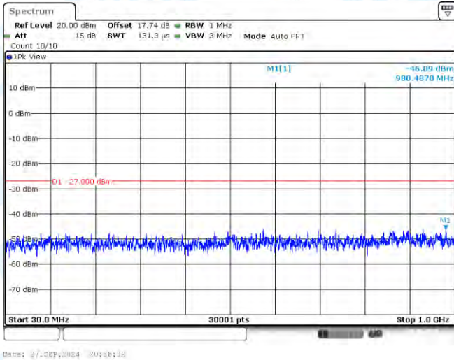
11A-CDD-Ant1-5825-30~1000-PASS
