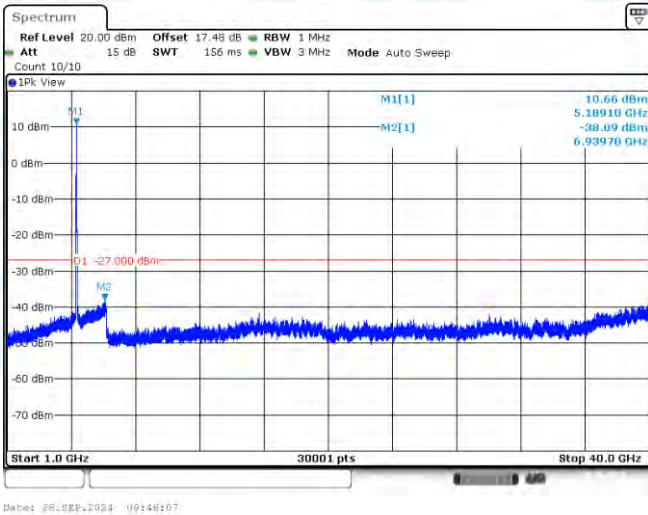
11N40-CDD-Ant2-5190-1000~40000-PASS
