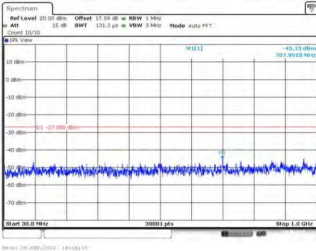
11A-CDD-Ant3-5320-30~1000-PASS
