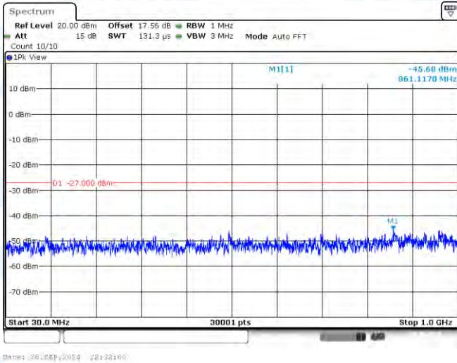
11A-CDD-Ant1-5500-30~1000-PASS
