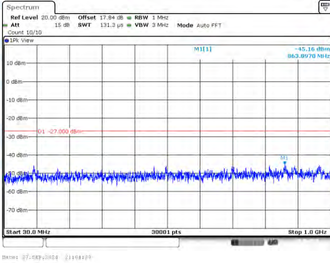
11N20-CDD-Ant3-5785-30~1000-PASS
