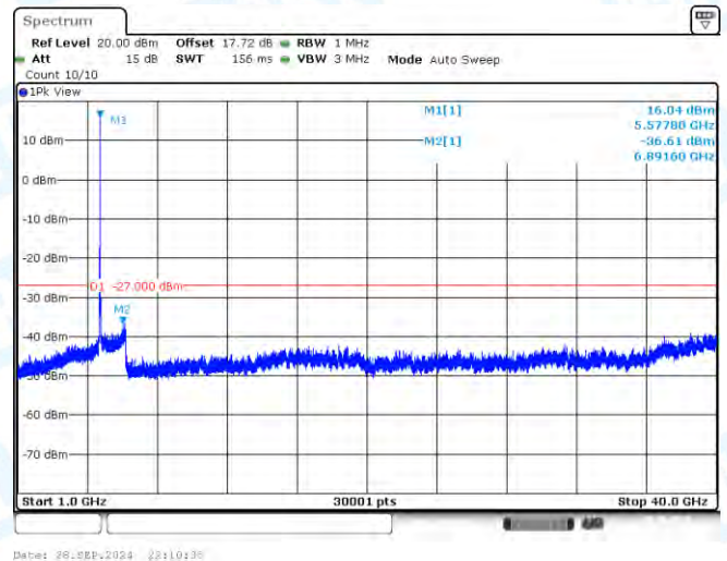
11A-Ant3-5580-1000~40000-PASS
