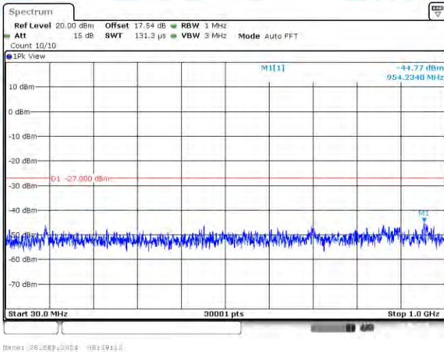
11A-CDD-Ant3-5180-30~1000-PASS
