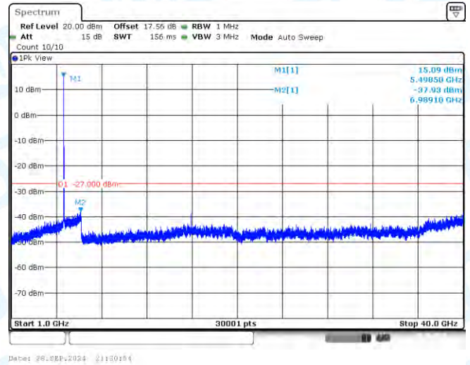
11A-Ant1-5500-1000~40000-PASS
