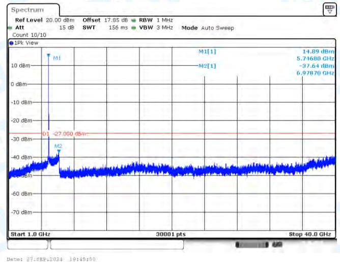
11A-Ant3-5745-1000~40000-PASS
