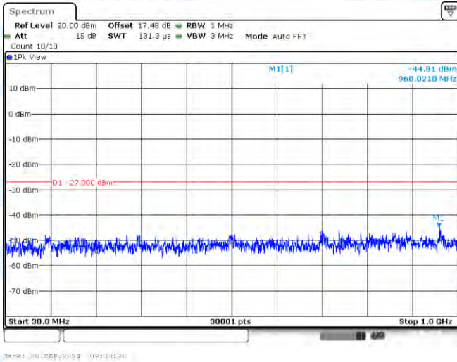
11N20-CDD-Ant1-5240-30~1000-PASS
