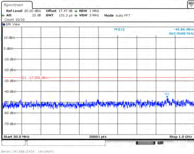
11N20-CDD-Ant1-5260-30~1000-PASS
