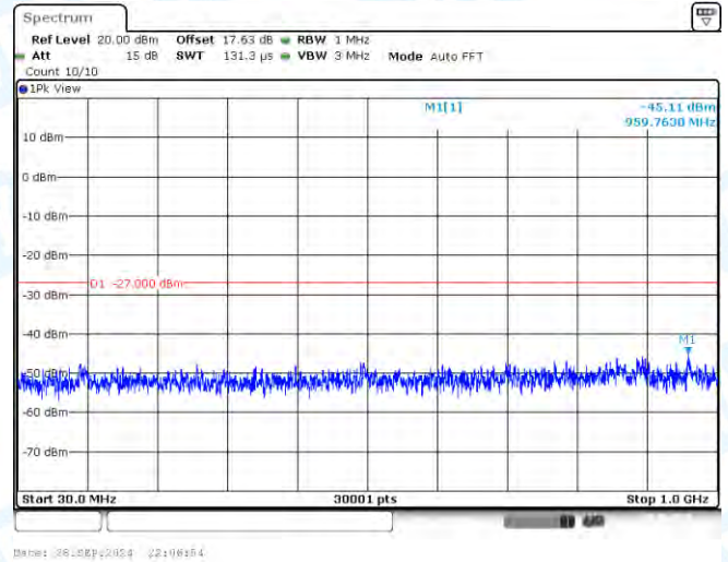
11A-Ant2-5580-30~1000-PASS
