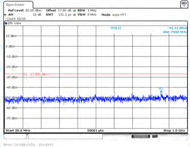
11A-Ant2-5720-30~1000-PASS
