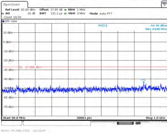
11A-Ant3-5720-30~1000-PASS
