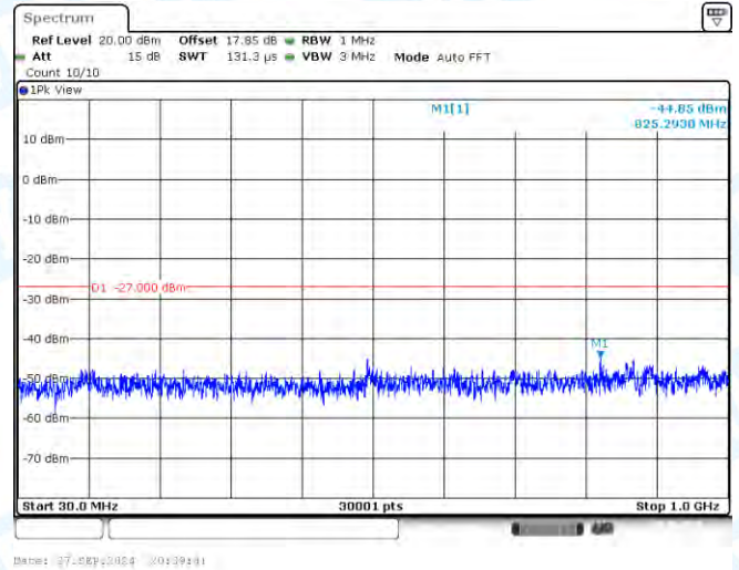
11A-CDD-Ant2-5825-30~1000-PASS
