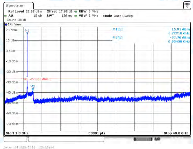
11A-Ant3-5720-1000~40000-PASS
