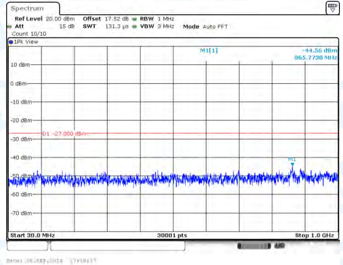
11N20-CDD-Ant2-5320-30~1000-PASS
