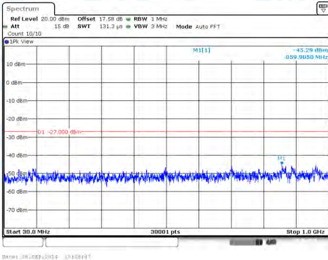
11A-Ant3-5280-30~1000-PASS
