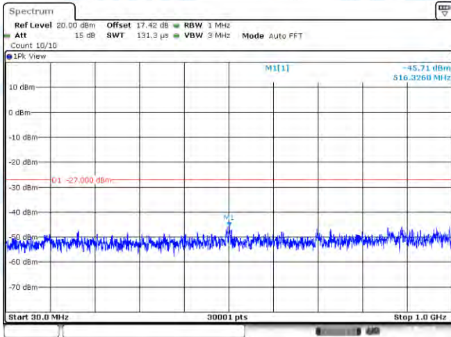
11A-CDD-Ant1-5280-30~1000-PASS
