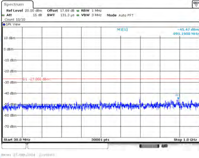
11N20-CDD-Ant1-5785-30~1000-PASS
