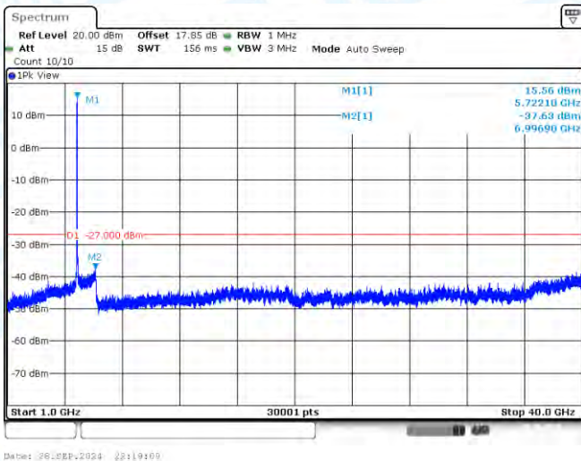
11A-Ant2-5720-1000~40000-PASS
