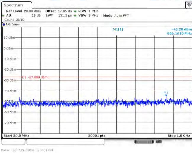
11A-CDD-Ant3-5745-30~1000-PASS
