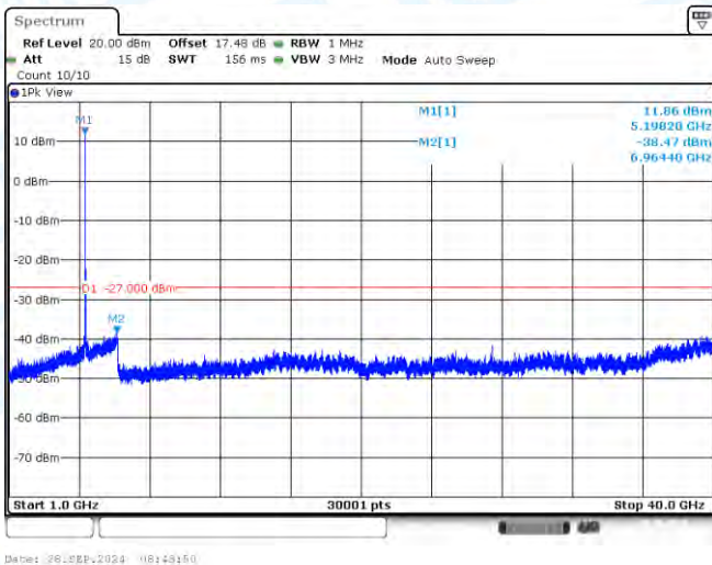
11A-CDD-Ant2-5200-1000~40000-PASS
