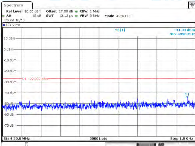
11N20-CDD-Ant1-5280-30~1000-PASS
