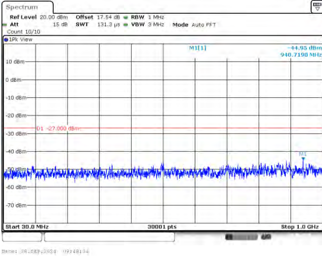
11N40-CDD-Ant3-5190-30~1000-PASS
