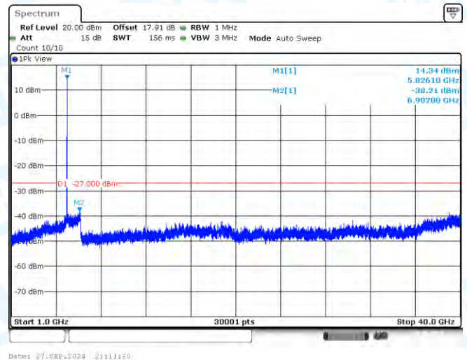
11N20-CDD-Ant3-5825-1000~40000-PASS
