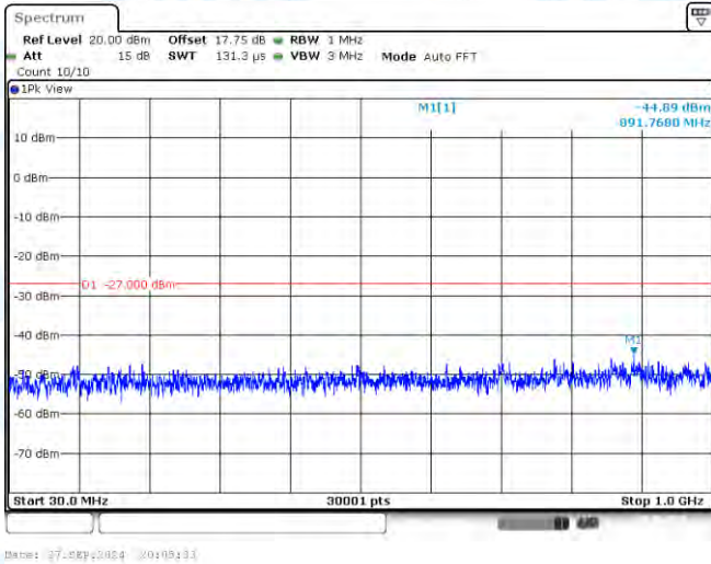
11A-CDD-Ant1-5745-30~1000-PASS
