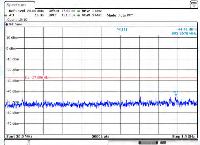
11A-CDD-Ant2-5580-30~1000-PASS
