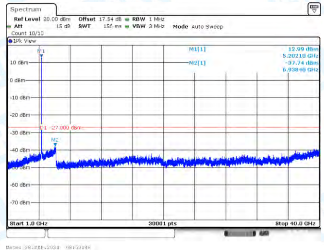
11A-CDD-Ant3-5200-1000~40000-PASS
