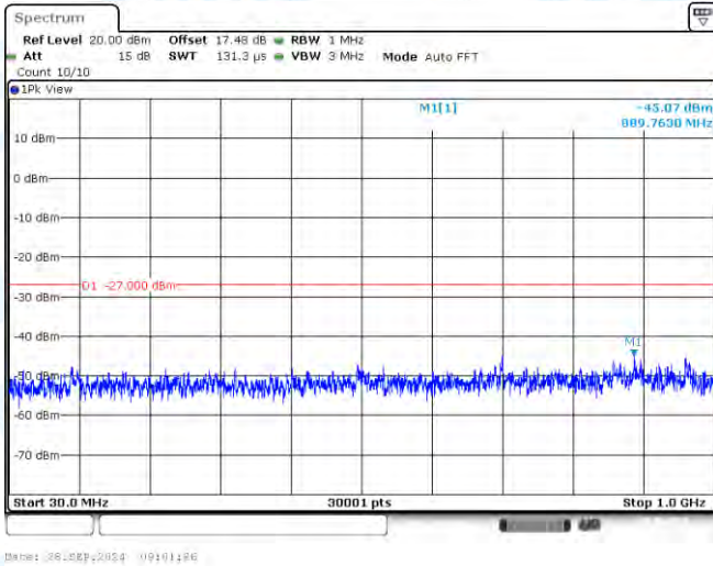
11A-CDD-Ant1-5240-30~1000-PASS
