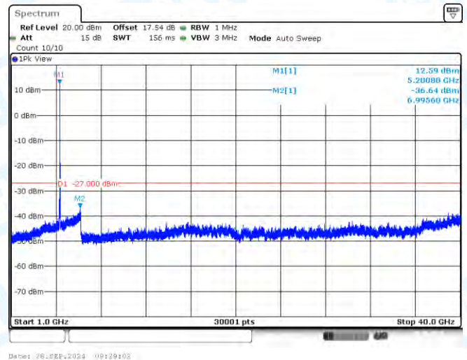
11N20-CDD-Ant3-5200-1000~40000-PASS
