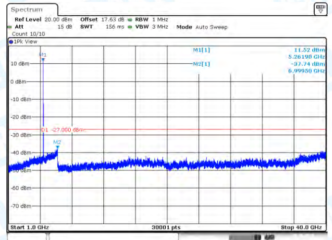
11A-CDD-Ant1-5260-1000~40000-PASS
