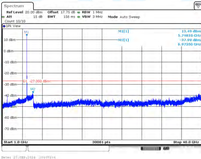
11A-CDD-Ant2-5745-1000~40000-PASS
