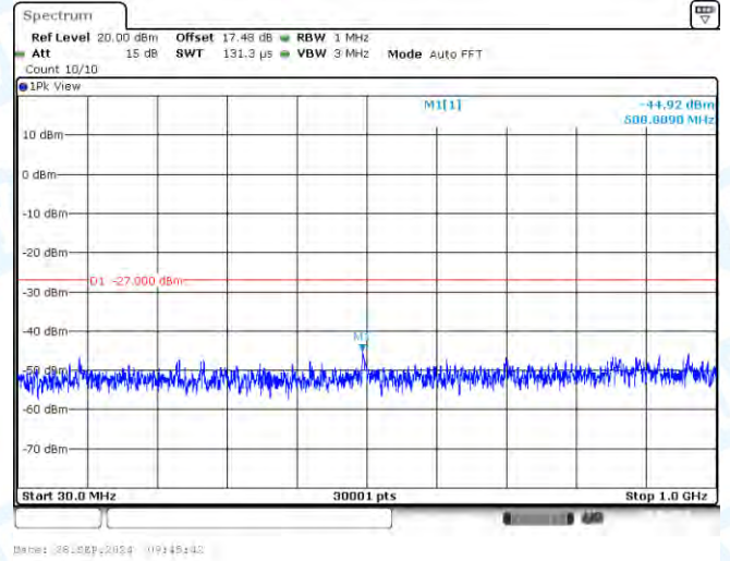
11N40-CDD-Ant2-5190-30~1000-PASS
