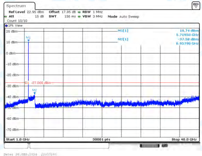
11A-CDD-Ant3-5720-1000~40000-PASS
