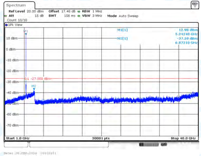
11N20-CDD-Ant1-5240-1000~40000-PASS
