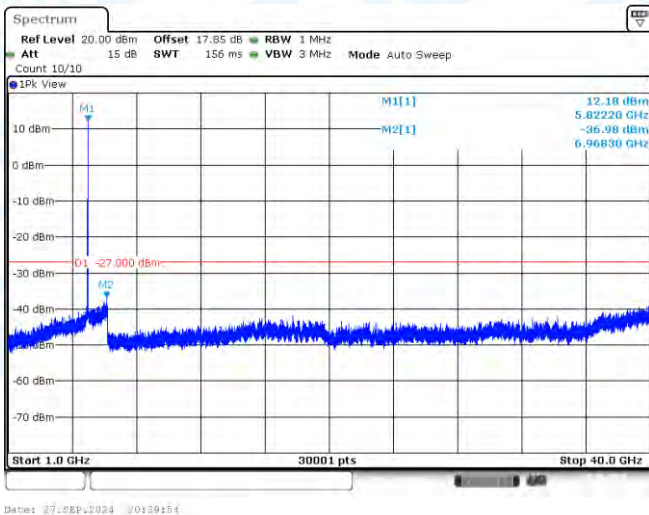
11A-CDD-Ant2-5825-1000~40000-PASS
