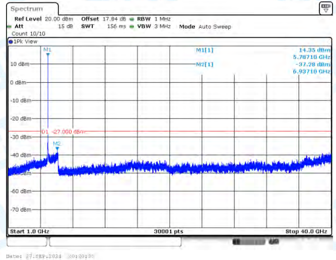
11A-CDD-Ant3-5785-1000~40000-PASS
