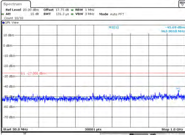
11N20-CDD-Ant1-5745-30~1000-PASS
