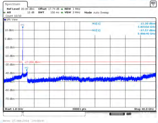
11A-CDD-Ant1-5825-1000~40000-PASS
