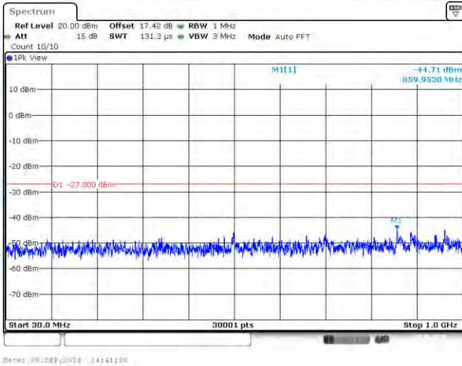
11A-Ant1-5280-30~1000-PASS
