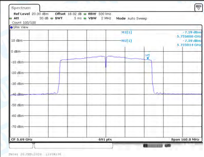
11AC80-CDD-Ant3-5690_UNII-3-PASS
