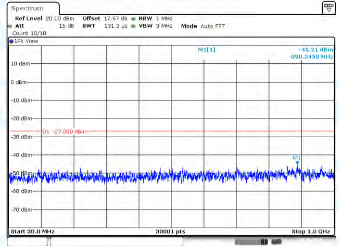
11A-Ant2-5240-30~1000-PASS
