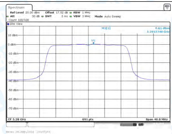
11AX20-CDD-Ant2-5280-PASS
