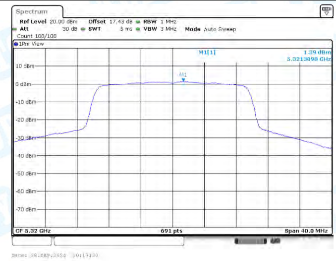
11AX20-CDD-Ant1-5320-PASS
