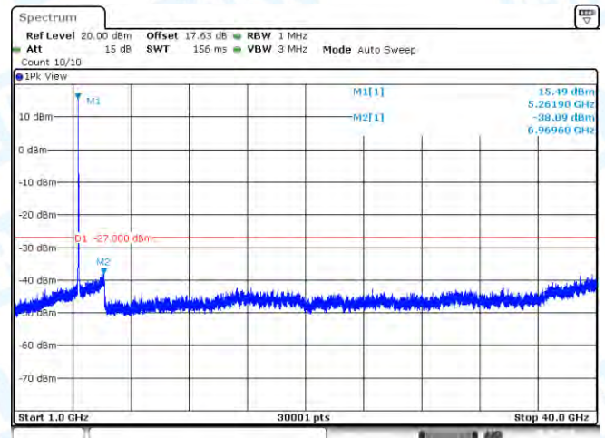
11A-Ant1-5260-1000~40000-PASS
