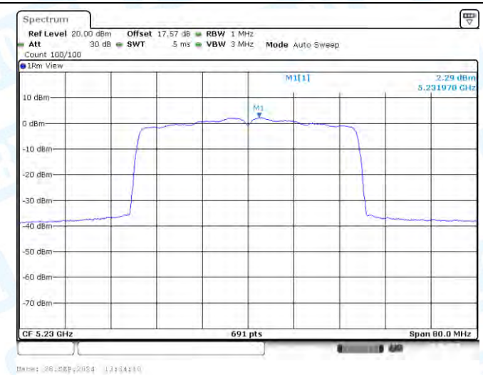
11AX40-CDD-Ant2-5230-PASS
