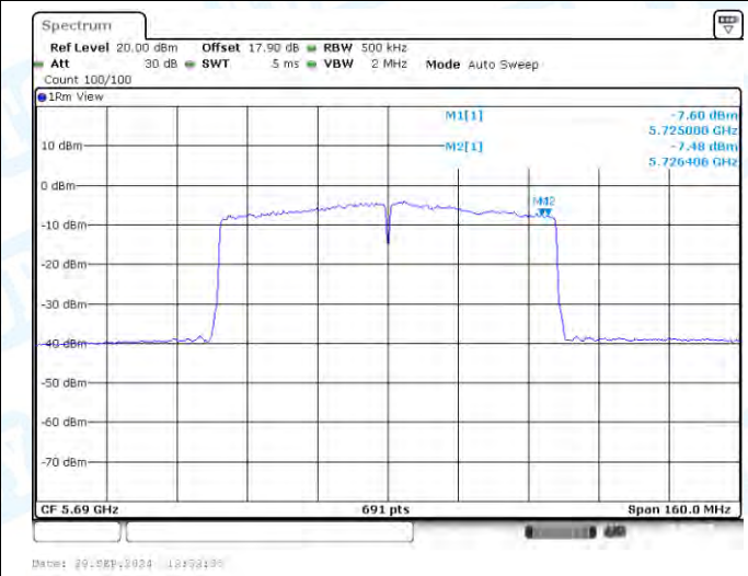
11AC80-CDD-Ant1-5690_UNII-3-PASS
