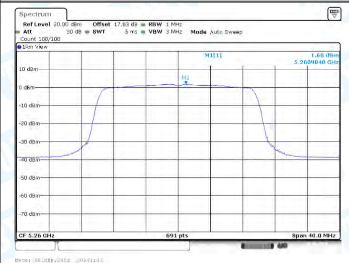
11AX20-CDD-Ant3-5260-PASS
