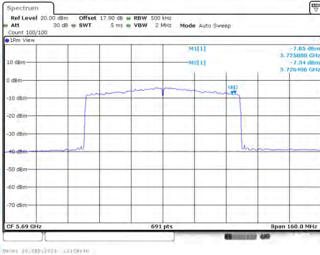
11AX80-CDD-Ant1-5690_UNII-3-PASS
