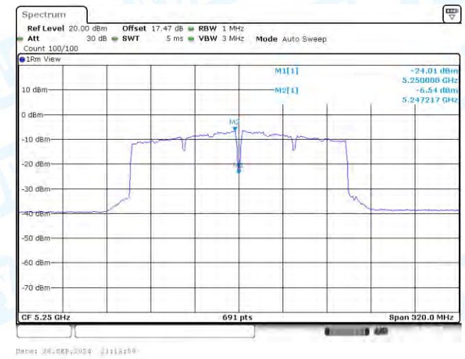
11AC160-CDD-Ant1-5250_UNII-1-PASS
