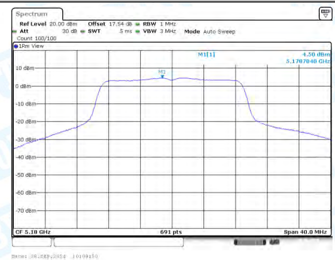
11AC20-CDD-Ant3-5180-PASS
