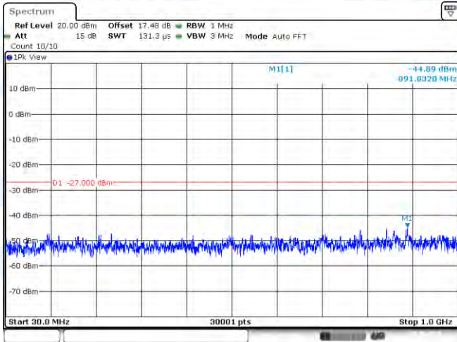
11A-Ant1-5240-30~1000-PASS
