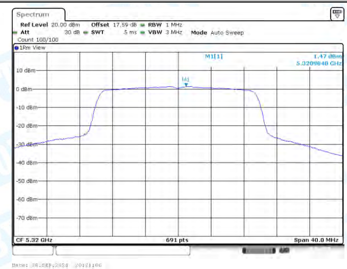
11AX20-CDD-Ant3-5320-PASS
