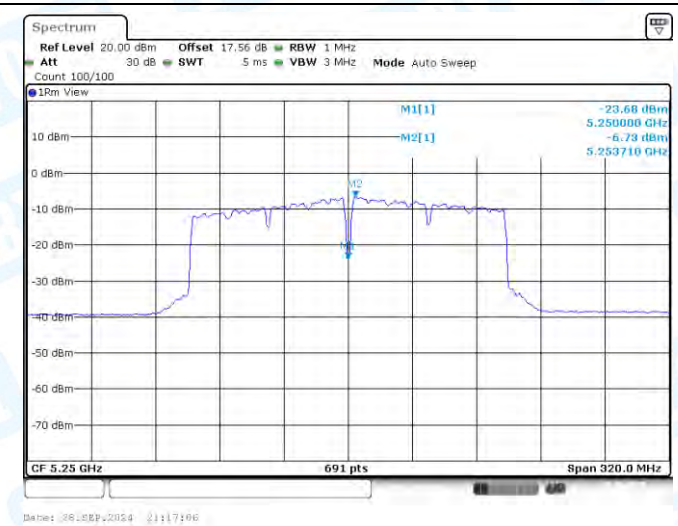
11AC160-CDD-Ant2-5250_UNII-2A-PASS
