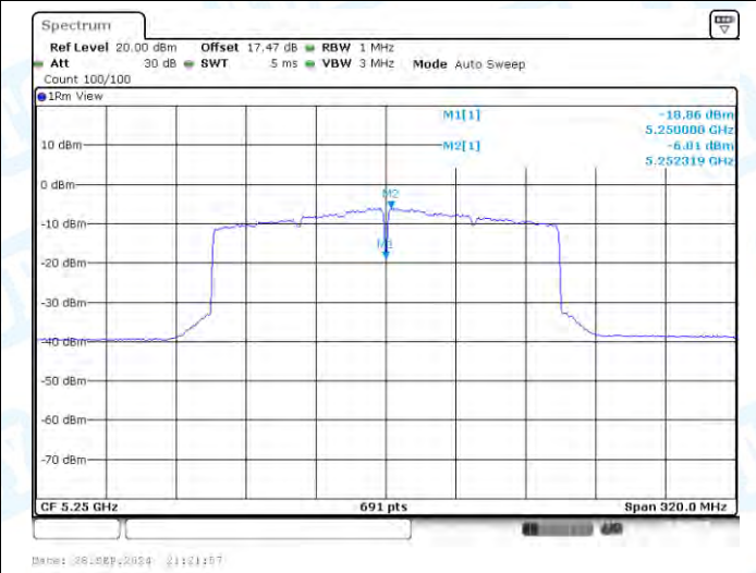
11AX160-CDD-Ant1-5250_UNII-2A-PASS
