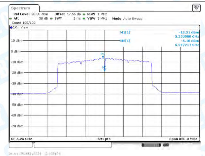
11AX160-CDD-Ant2-5250_UNII-1-PASS
