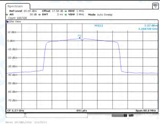
11AX40-CDD-Ant3-5270-PASS
