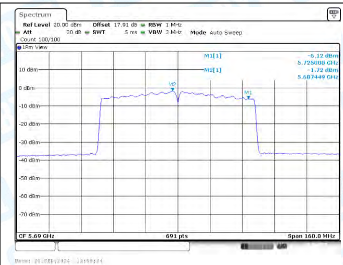
11AC80-CDD-Ant2-5690_UNII-2C-PASS
