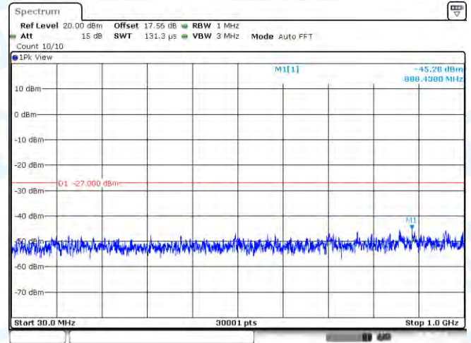
11A-Ant2-5260-30~1000-PASS
