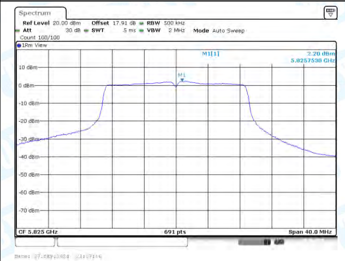
11AC20-CDD-Ant3-5825-PASS
