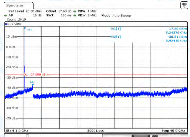
11A-Ant1-5240-1000~40000-PASS
