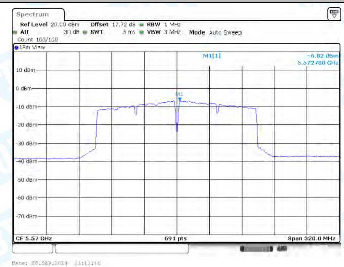
11AC160-CDD-Ant3-5570-PASS
