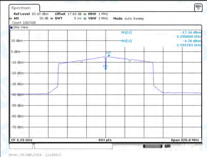
11AX160-CDD-Ant3-5250_UNII-2A-PASS
