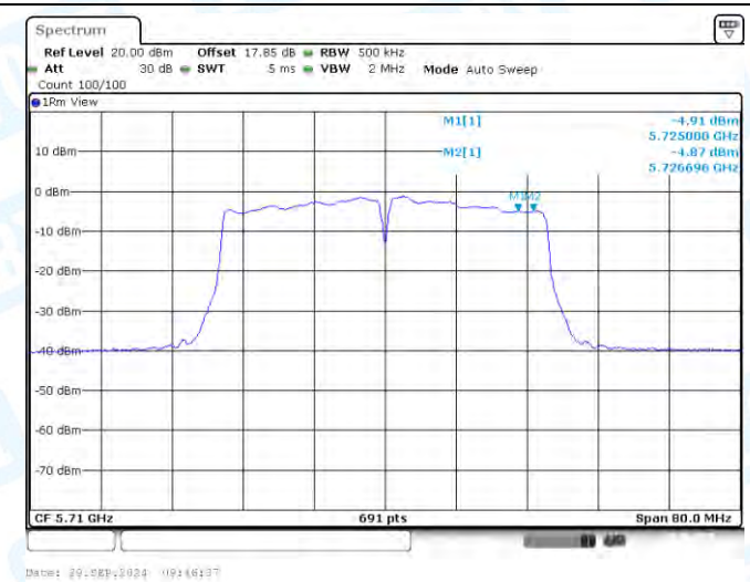
11N40-CDD-Ant2-5710_UNII-3-PASS
