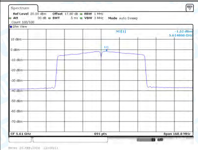
11AC80-CDD-Ant3-5610-PASS
