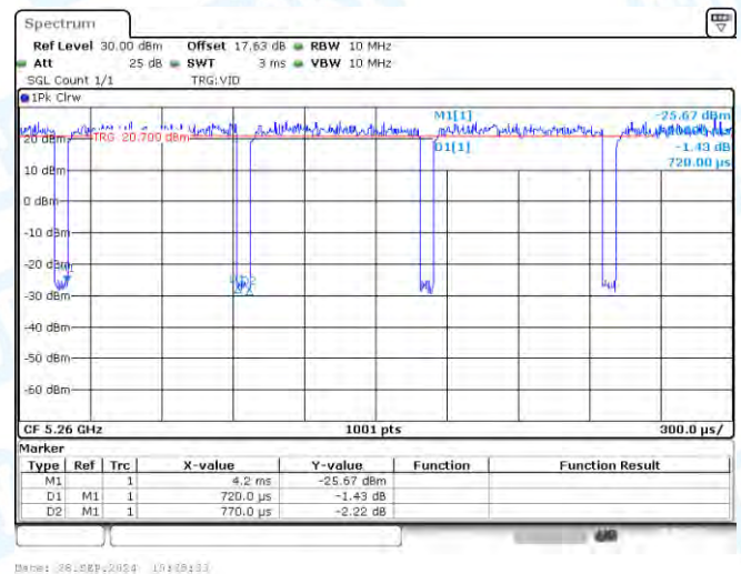
NTVN-11A-Ant3-5260
