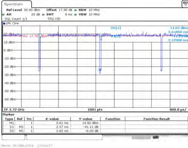
NTNV-11N20-CDD-Ant1-5720
