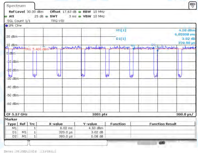
NTNV-11AC160-CDD-Ant2-5570
