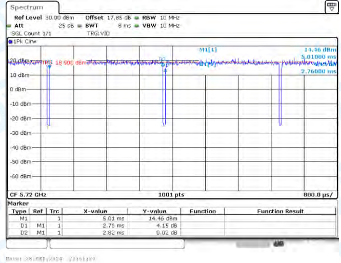
NTNV-11A-CDD-Ant2-5720
