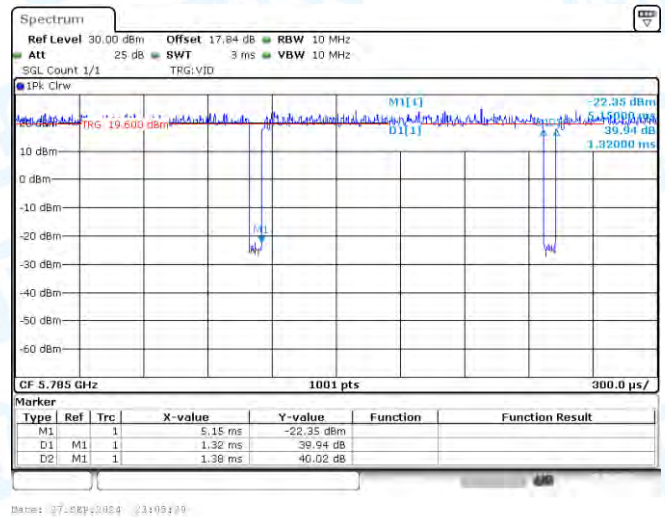
NTNV-11AC20-CDD-Ant3-5785
