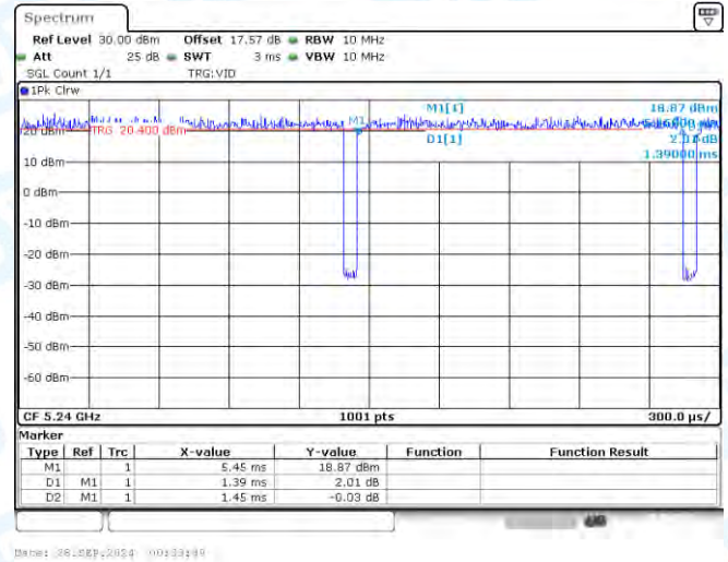
NTVN-11A-Ant2-5240
