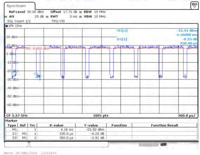
NTNV-11AC160-CDD-Ant3-5570
