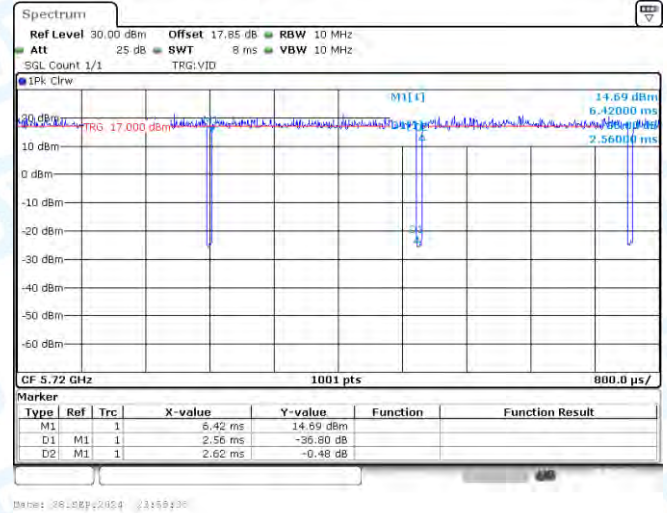
NTNV-11N20-CDD-Ant2-5720
