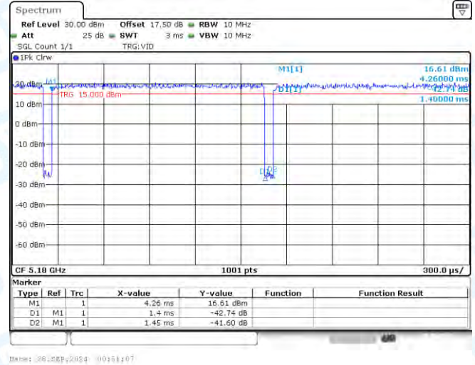
NTNV-11A-CDD-Ant2-5180
