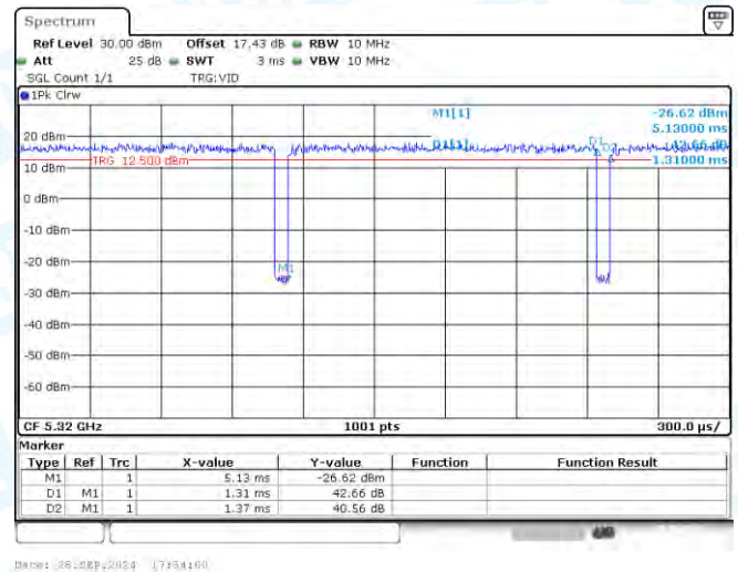
NTNV-11N20-CDD-Ant1-5320
