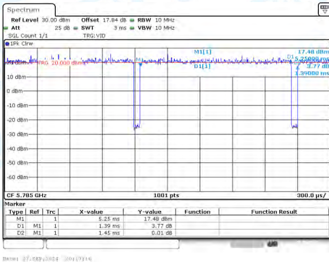
NTNV-11A-CDD-Ant3-5785
