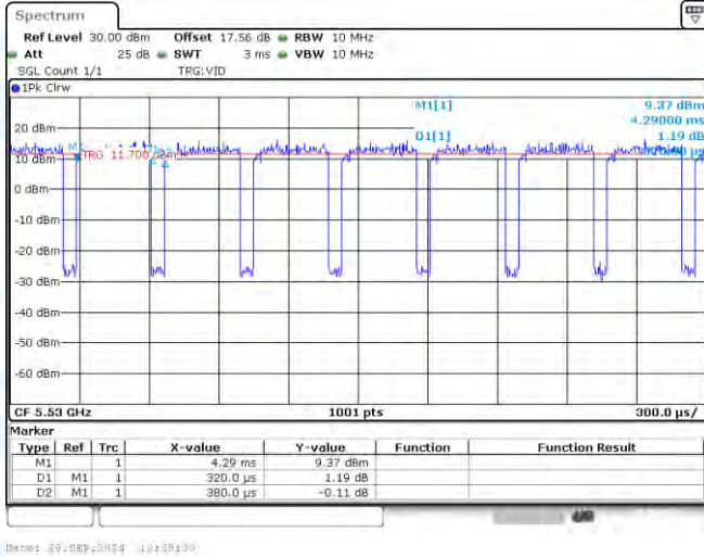
NTNV-11AC80-CDD-Ant1-5530
