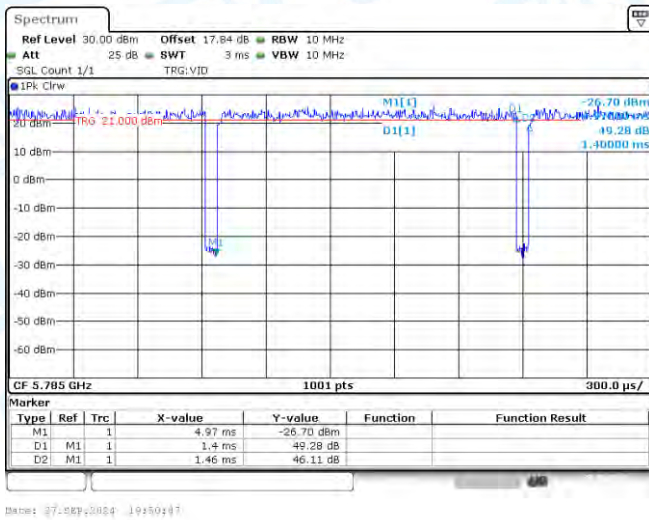
NTNV-11A-Ant3-5785
