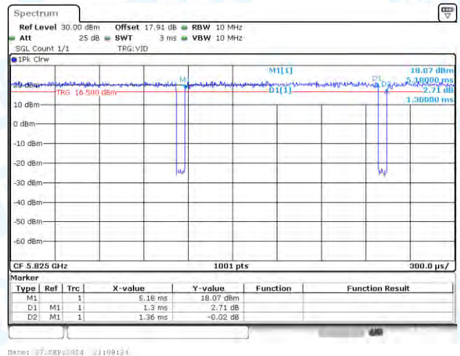
NTNV-11N20-CDD-Ant3-5825
