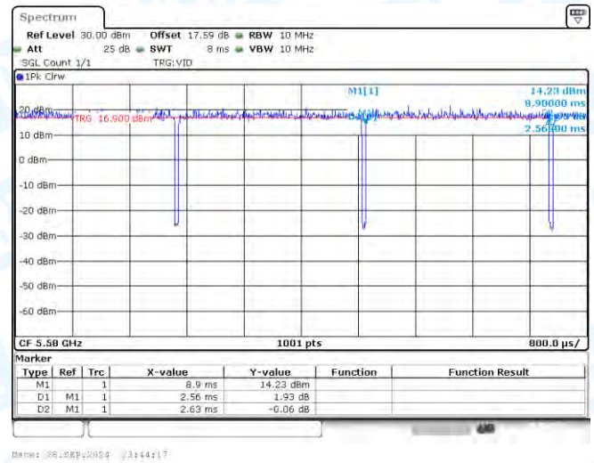
NTNV-11N20-CDD-Ant1-5580
