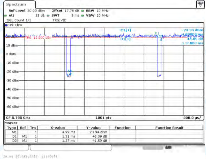
NTNV-11N20-CDD-Ant2-5785
