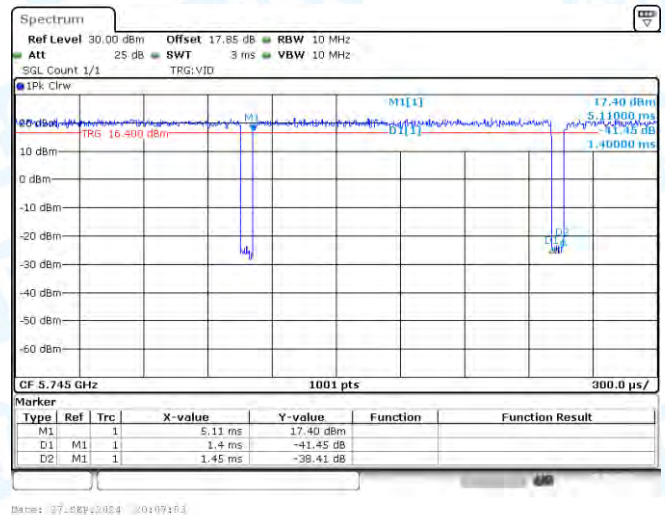
NTNV-11A-CDD-Ant3-5745
