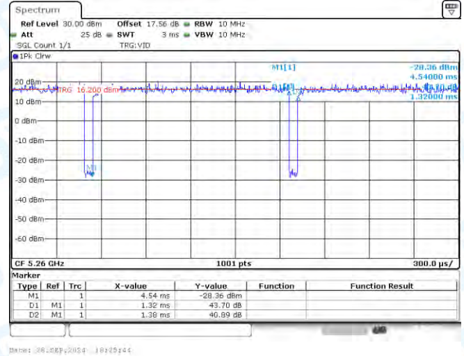
NTNV-11AC20-CDD-Ant2-5260
