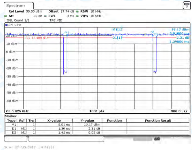
NTNV-11A-Ant1-5825
