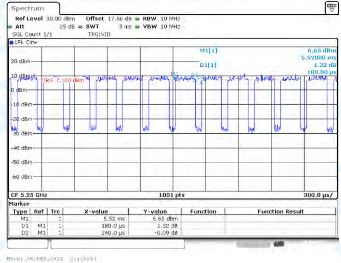
NTNV-11AC160-CDD-Ant2-5250
