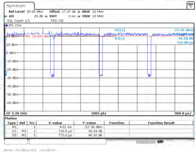
NTVN-11A-Ant1-5260
