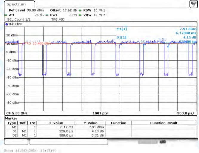
NTNV-11AC80-CDD-Ant2-5530
