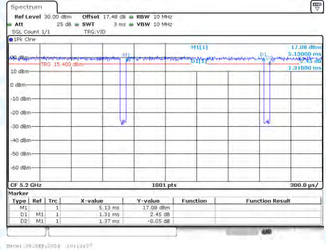
NTNV-11AC20-CDD-Ant2-5200
