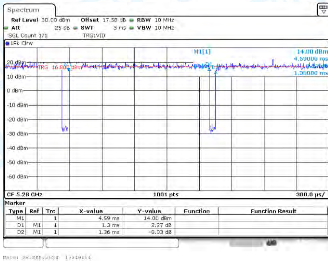
NTNV-11N20-CDD-Ant3-5280
