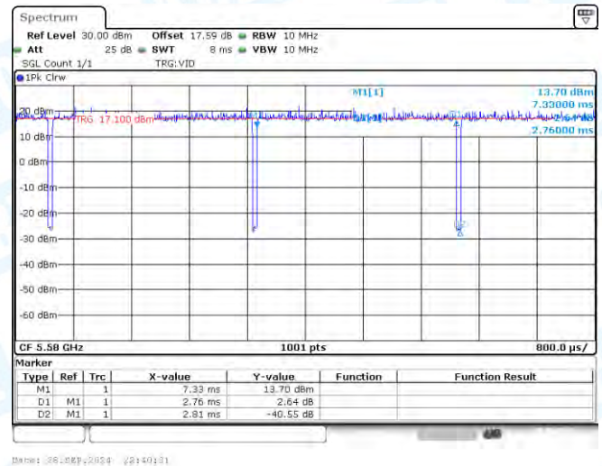
NTNV-11A-CDD-Ant1-5580
