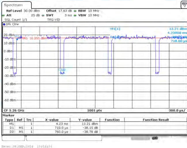
NTNV-11A-CDD-Ant3-5260
