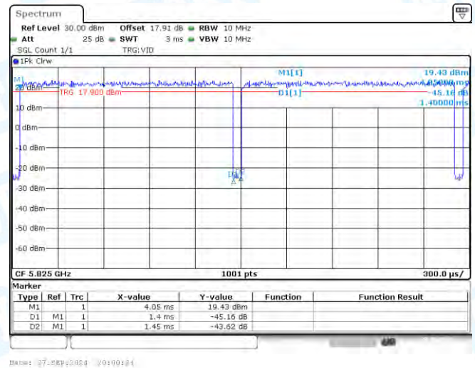
NTNV-11A-Ant3-5825
