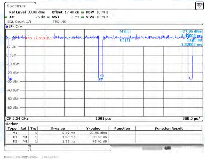
NTNV-11AC20-CDD-Ant1-5240
