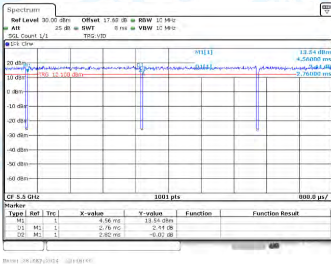
NTNV-11A-CDD-Ant3-5500
