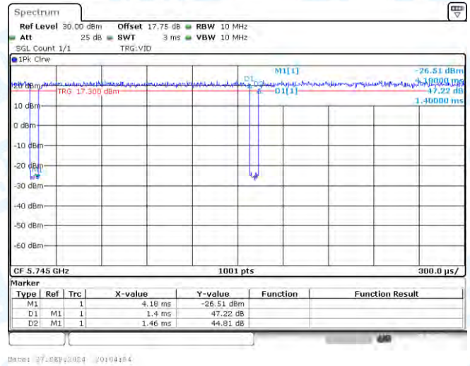
NTNV-11A-CDD-Ant1-5745
