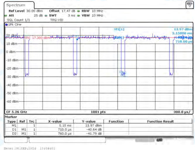
NTNV-11A-CDD-Ant1-5260
