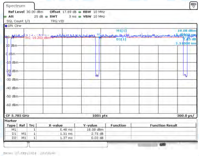
NTNV-11AC20-CDD-Ant1-5785
