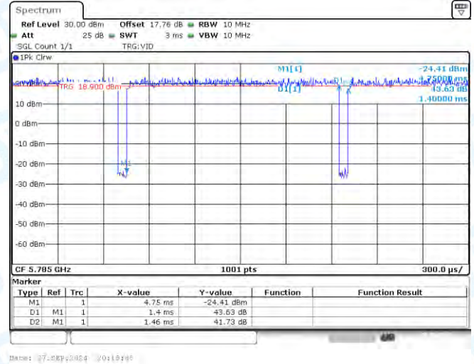
NTNV-11A-CDD-Ant2-5785
