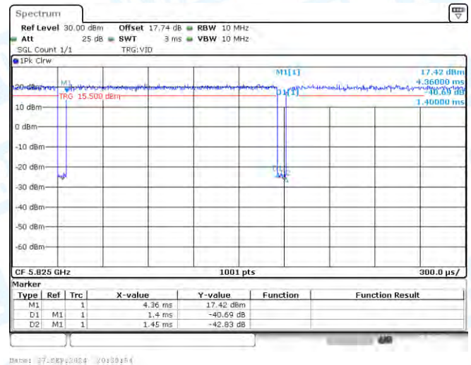
NTNV-11A-CDD-Ant1-5825
