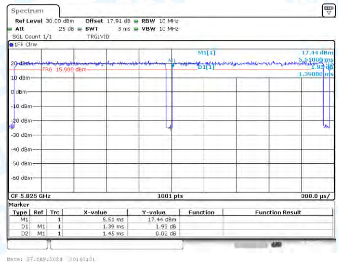
NTNV-11A-CDD-Ant3-5825
