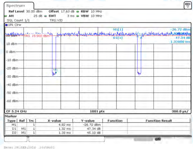
NTNV-11AC20-CDD-Ant3-5240
