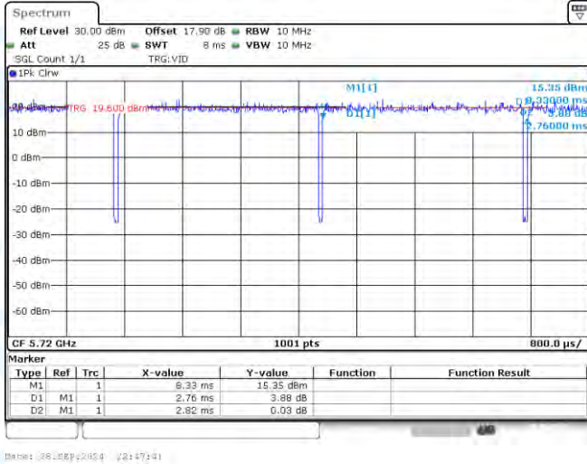
NTNV-11A-CDD-Ant1-5720
