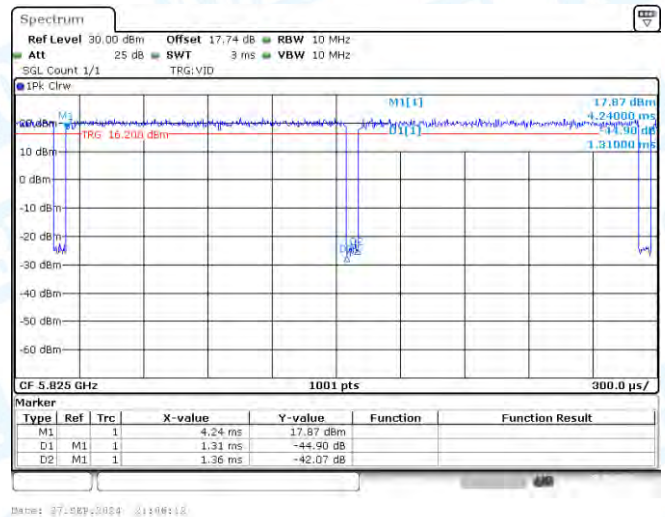
NTNV-11N20-CDD-Ant1-5825
