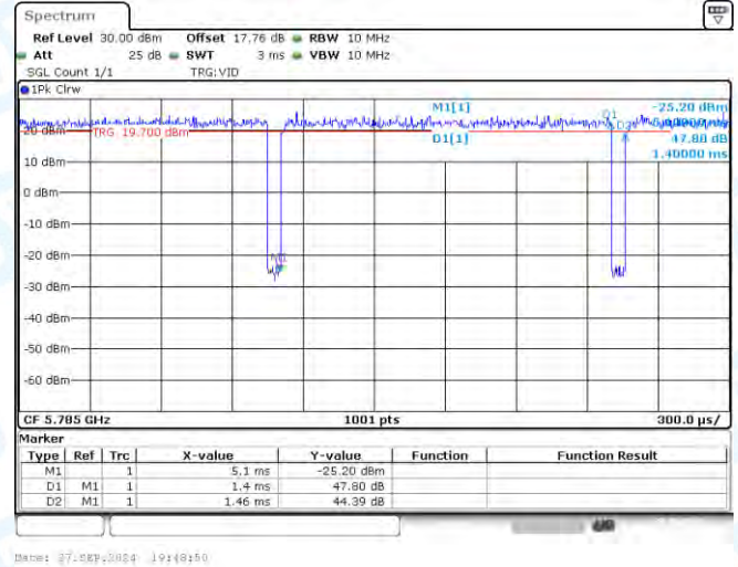
NTNV-11A-Ant2-5785
