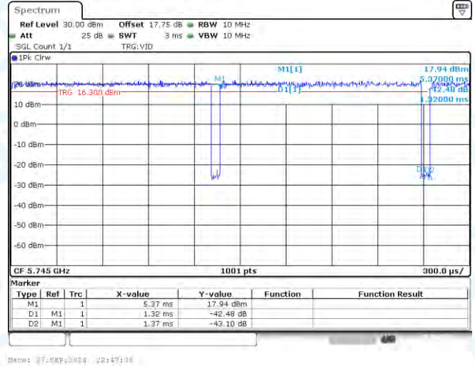
NTNV-11AC20-CDD-Ant2-5745
