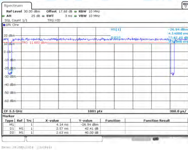
NTNV-11N20-CDD-Ant3-5500
