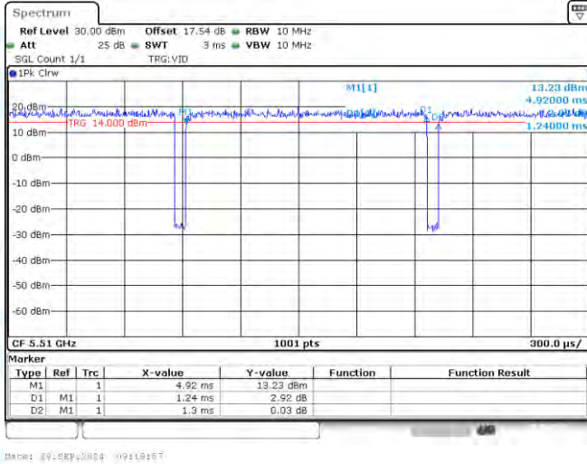
NTNV-11N40-CDD-Ant1-5510
