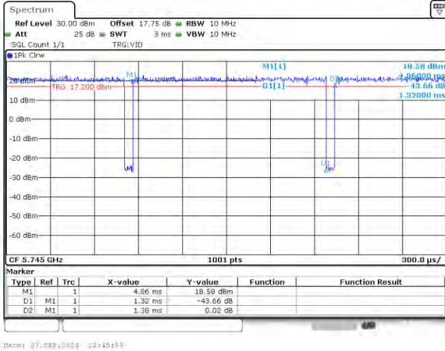
NTNV-11AC20-CDD-Ant1-5745
