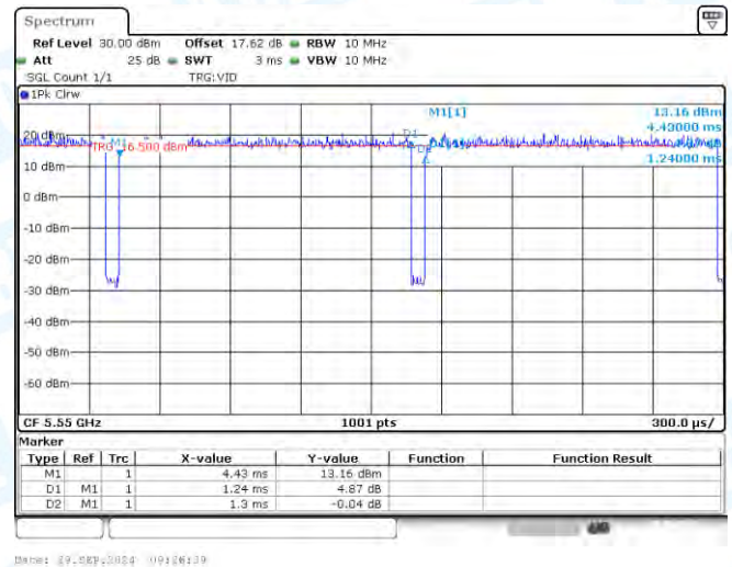
NTNV-11N40-CDD-Ant1-5550
