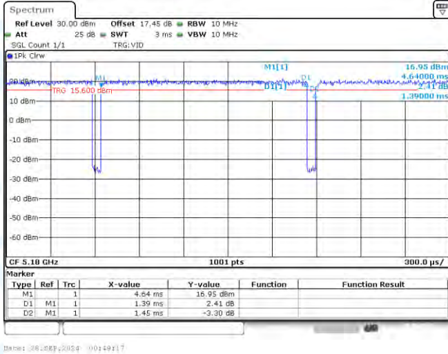
NTNV-11A-CDD-Ant1-5180
