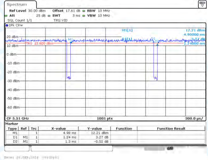
NTNV-11N40-CDD-Ant2-5510
