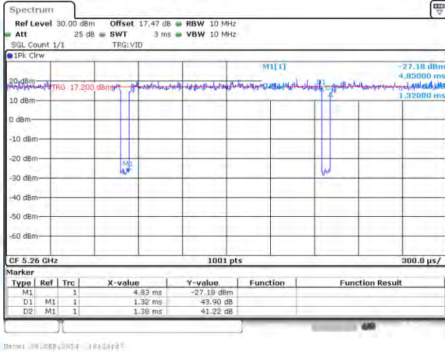
NTNV-11AC20-CDD-Ant1-5260
