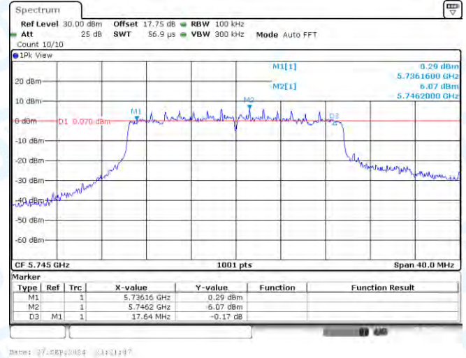
11AX20-CDD-Ant2-5745-PASS
