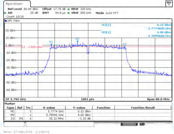
11N40-CDD-Ant2-5795-PASS
