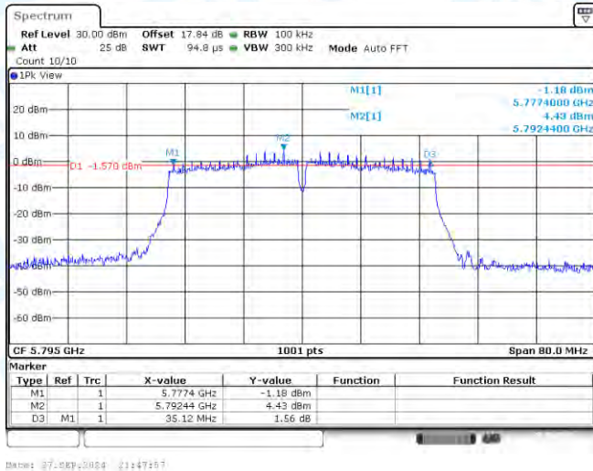
11N40-CDD-Ant3-5795-PASS
