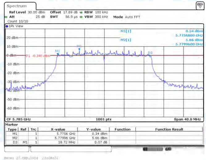
11AX20-CDD-Ant1-5785-PASS
