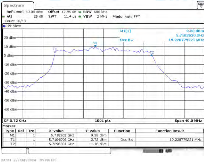
11AX20-CDD-Ant3-5720
