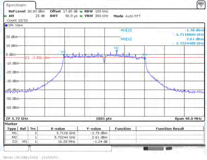
11A-CDD-Ant2-5720
