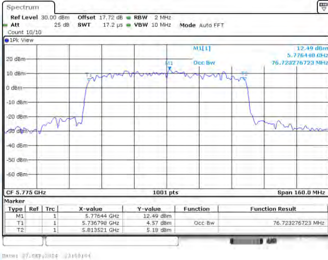
11AX80-CDD-Ant1-5775
