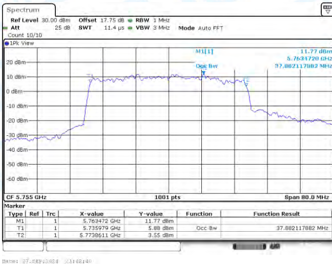
11AX40-CDD-Ant2-5755
