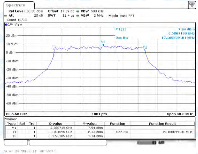
11AX20-CDD-Ant1-5580
