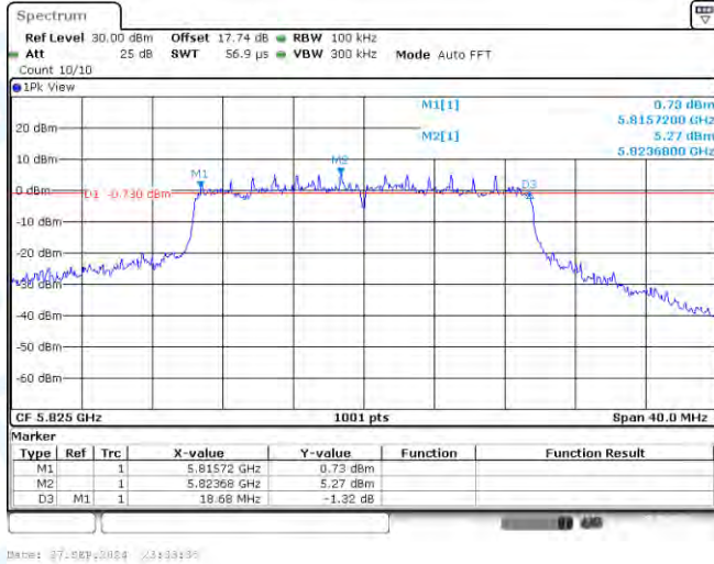
11AX20-CDD-Ant1-5825-PASS
