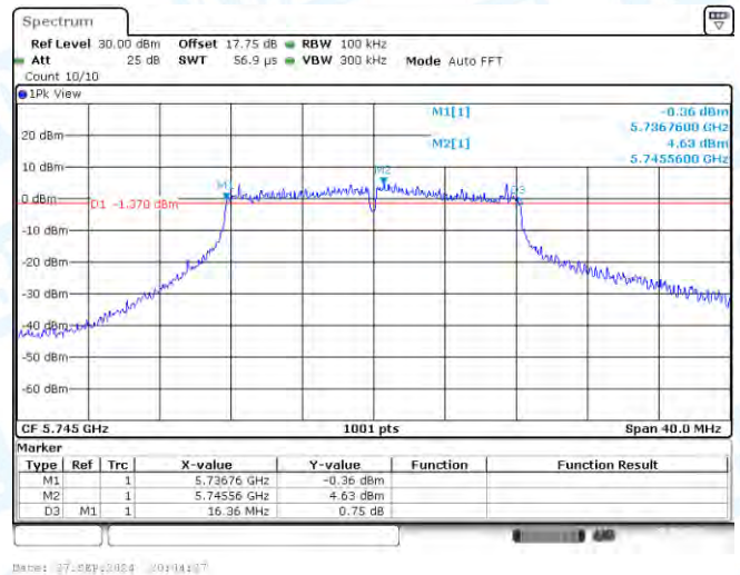
11A-CDD-Ant1-5745-PASS
