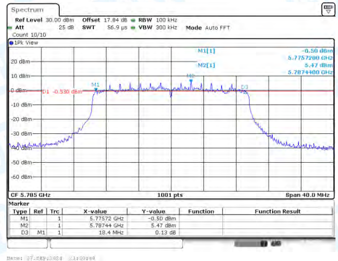
11AX20-CDD-Ant3-5785-PASS
