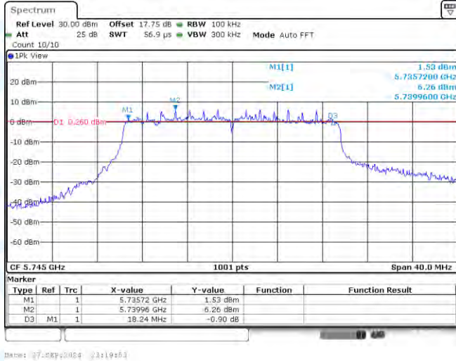
11AX20-CDD-Ant1-5745-PASS
