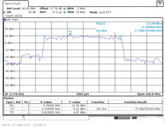
11AX80-CDD-Ant2-5775
