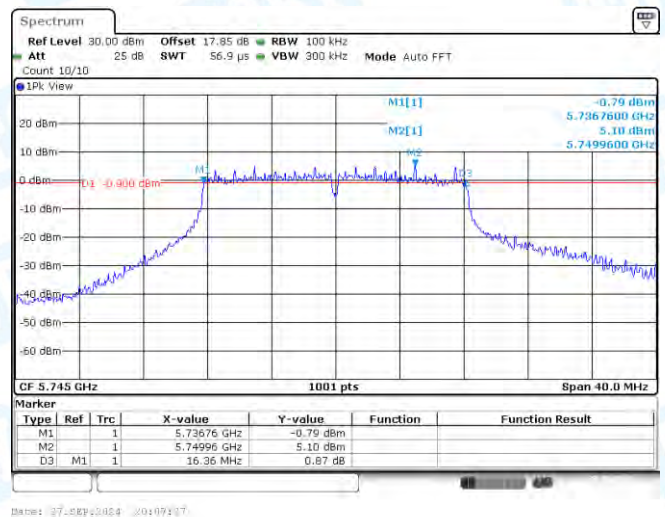
11A-CDD-Ant3-5745-PASS
