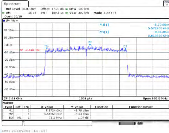
11AX80-CDD-Ant1-5610-PASS
