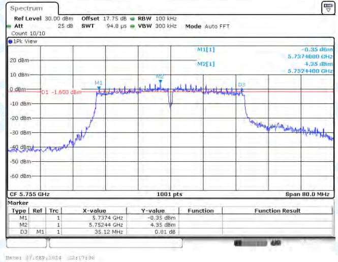
11AC40-CDD-Ant2-5755-PASS
