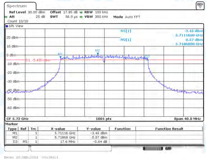
11AC20-CDD-Ant3-5720
