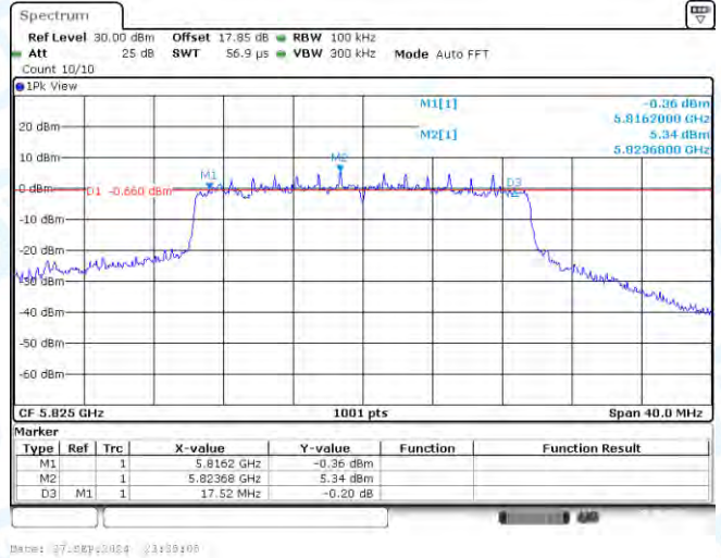
11AX20-CDD-Ant2-5825-PASS
