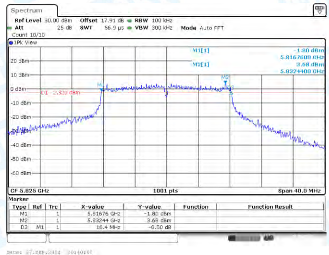
11A-CDD-Ant3-5825-PASS
