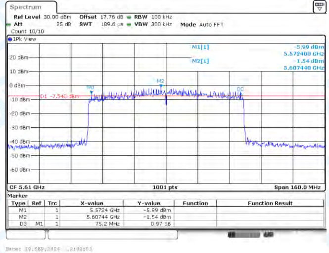
11AX80-CDD-Ant2-5610-PASS
