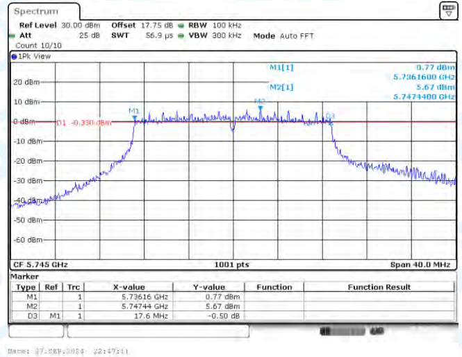
11AC20-CDD-Ant2-5745-PASS
