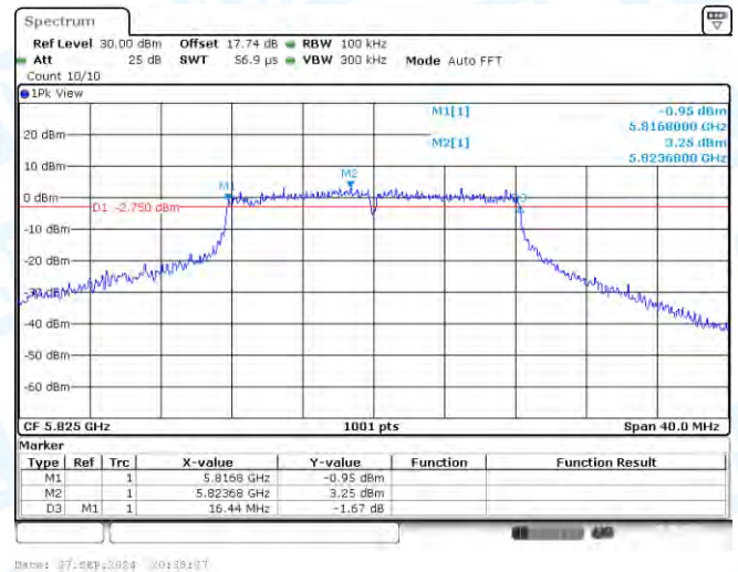
11A-CDD-Ant1-5825-PASS
