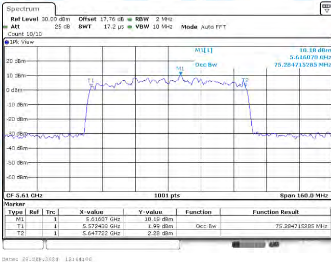
11AC80-CDD-Ant2-5610
