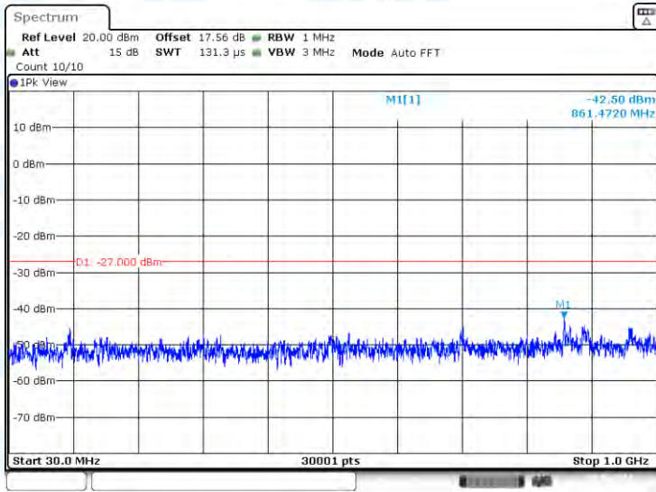
11AX20-CDD-Ant3-5320-30~1000-PASS
