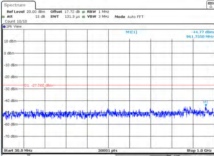
11AX80-CDD-Ant3-5690-30~1000-PASS
