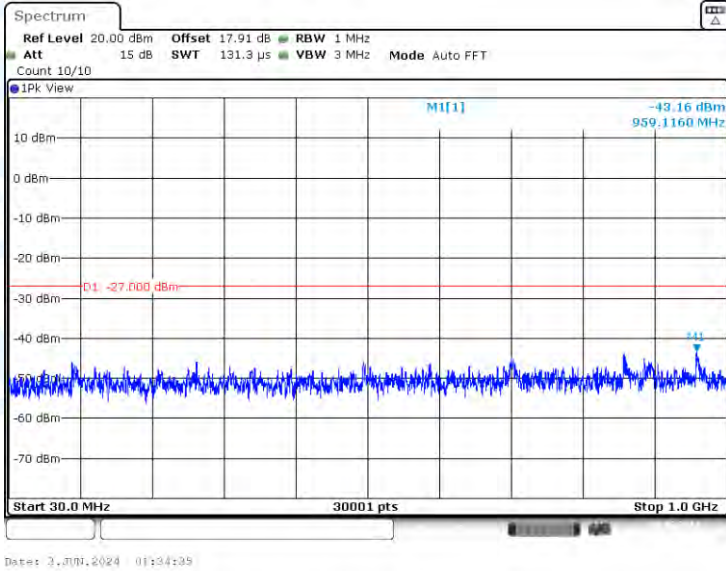
11AX80-CDD-Ant2-5690-30~1000-PASS
