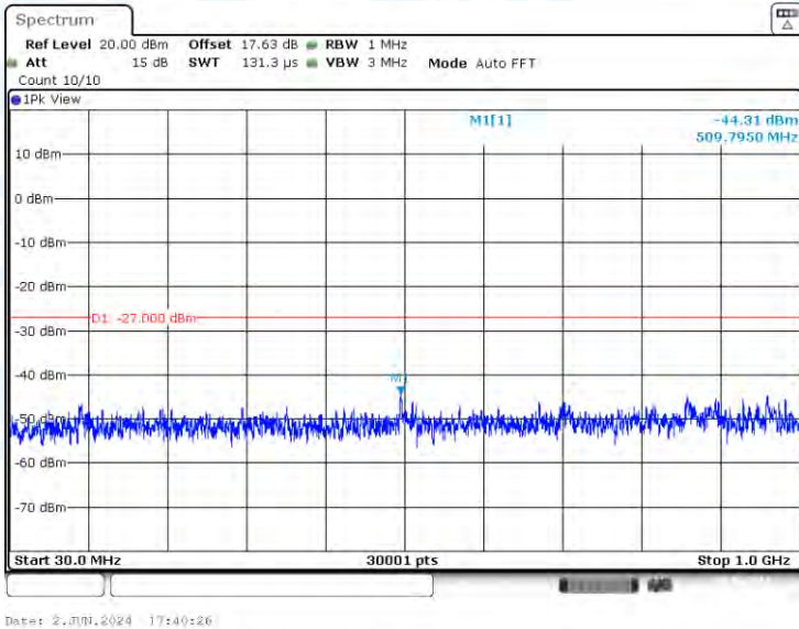
11AX20-CDD-Ant3-5260-30~1000-PASS
