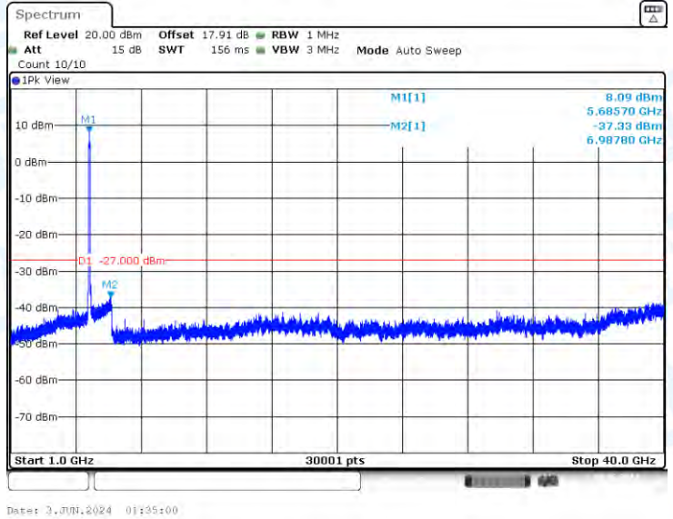
11AX80-CDD-Ant2-5690-1000~40000-PASS
