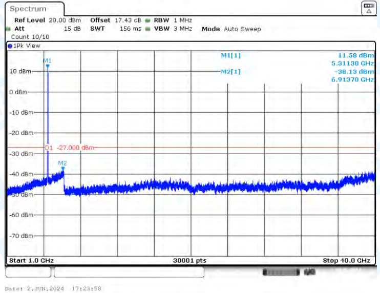
11AX40-CDD-Ant1-5310-1000~40000-PASS
