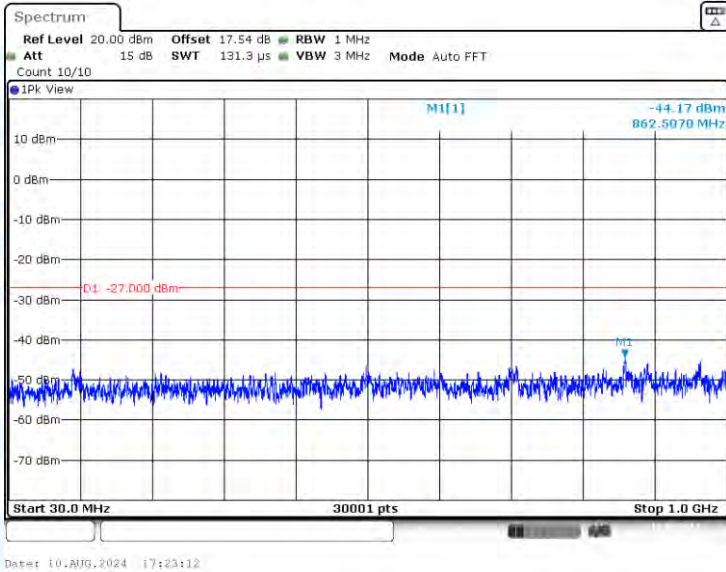
11AX20-CDD-Ant3-5200-30~1000-PASS
