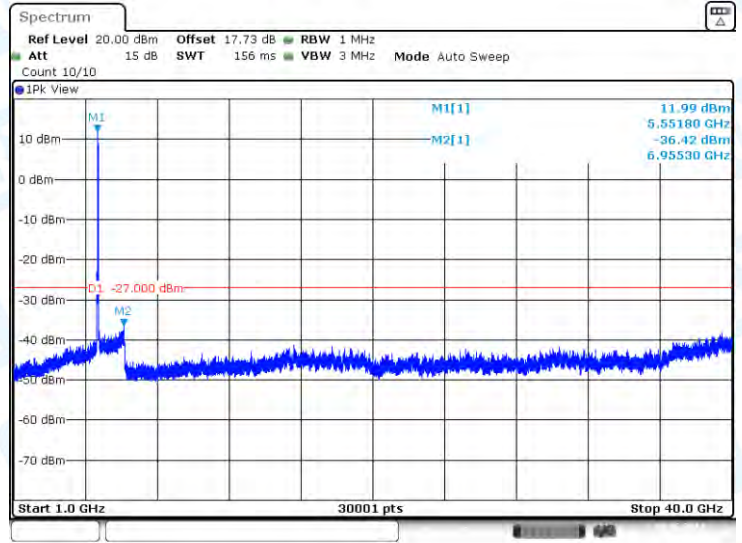
11AX40-CDD-Ant2-5550-1000~40000-PASS
