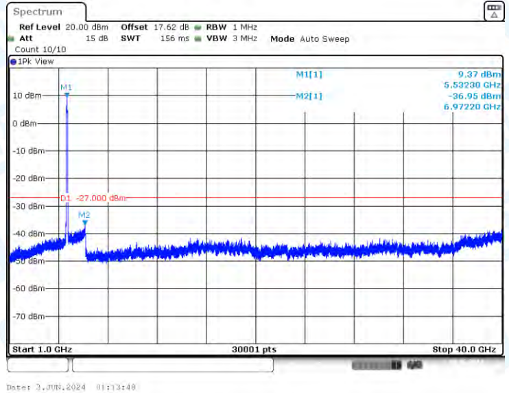
11AX80-CDD-Ant2-5530-1000~40000-PASS
