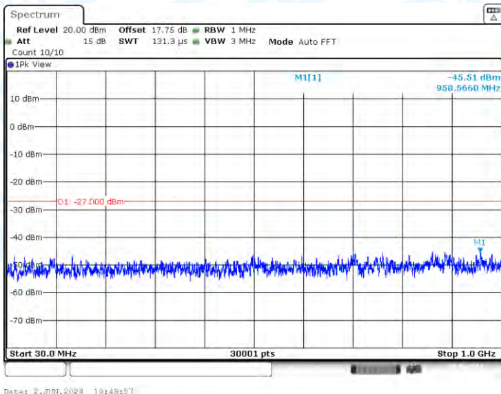
11AX20-CDD-Ant3-5720-30~1000-PASS
