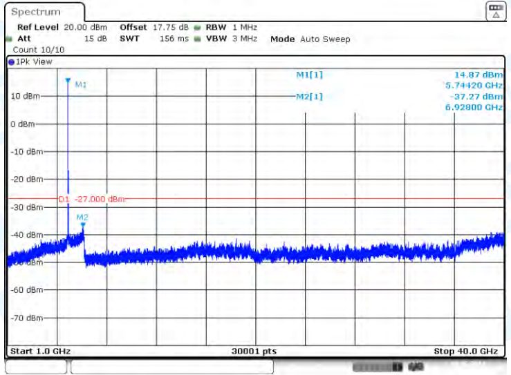
11AX20-CDD-Ant1-5745-1000~40000-PASS
