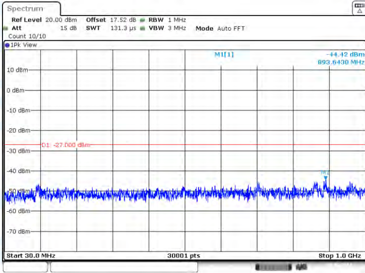
11AX20-CDD-Ant1-5280-30~1000-PASS
