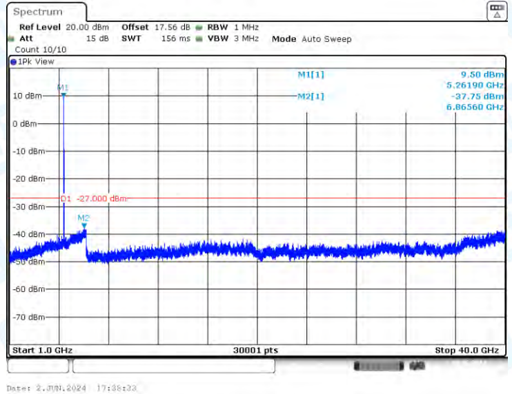
11AX20-CDD-Ant2-5260-1000~40000-PASS
