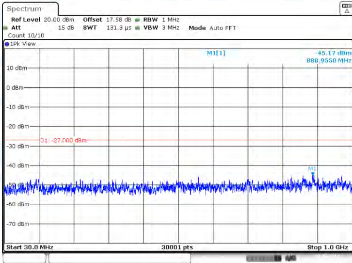
11AX40-CDD-Ant2-5270-30~1000-PASS
