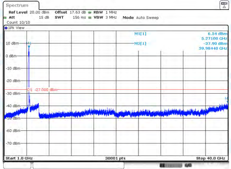
11AX160-CDD-Ant2-5250-1000~40000-PASS
