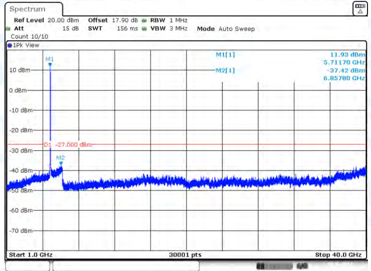
11AX40-CDD-Ant3-5550-1000~40000-PASS
