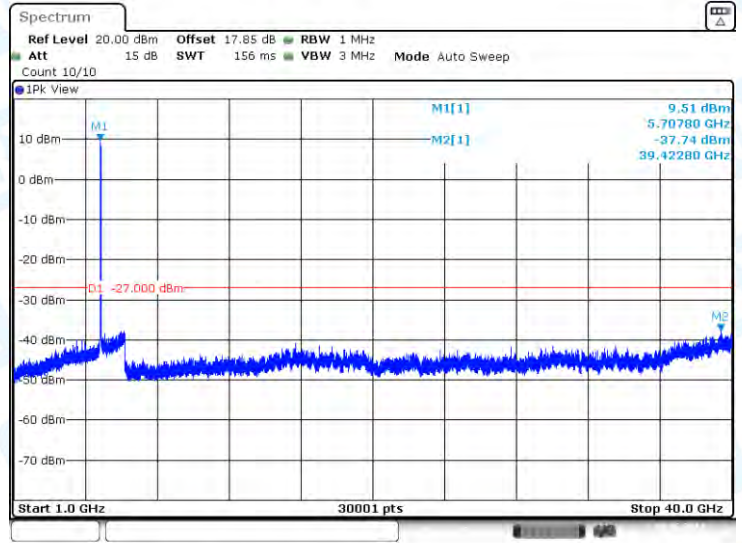
11AC40-CDD-Ant1-5710-1000~40000-PASS
