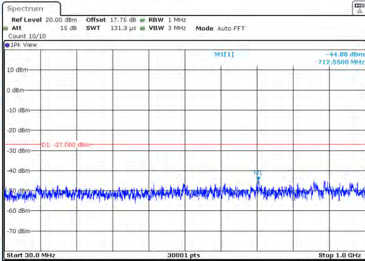
11N40-CDD-Ant1-5755-30~1000-PASS
