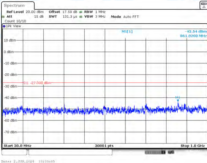
11AC160-CDD-Ant3-5250-30~1000-PASS
