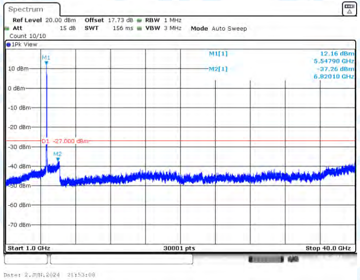
11N40-CDD-Ant3-5550-1000~40000-PASS
