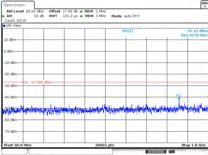
11AC40-CDD-Ant2-5510-30~1000-PASS
