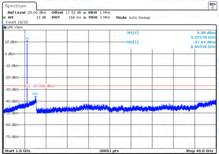
11AC20-CDD-Ant1-5320-1000~40000-PASS
