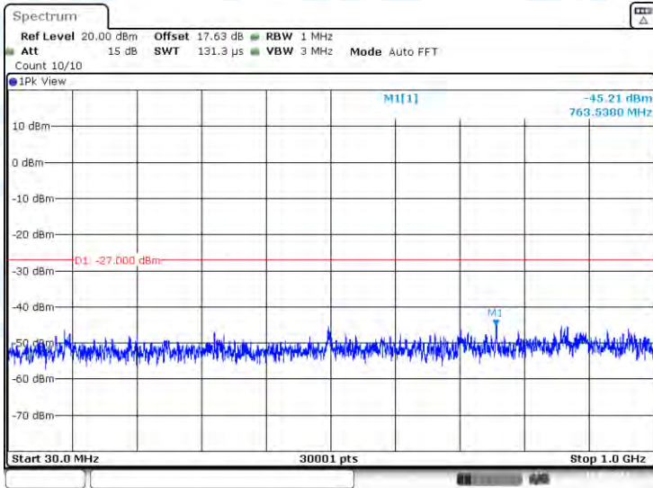
11AC40-CDD-Ant2-5230-30~1000-PASS
