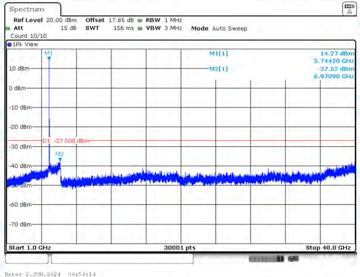
11AC20-CDD-Ant2-5745-1000~40000-PASS
