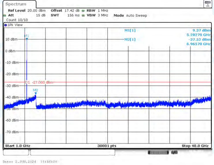
11AC20-CDD-Ant1-5280-1000~40000-PASS
