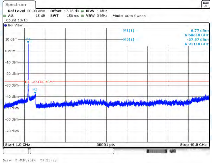
11AC80-CDD-Ant2-5610-1000~40000-PASS
