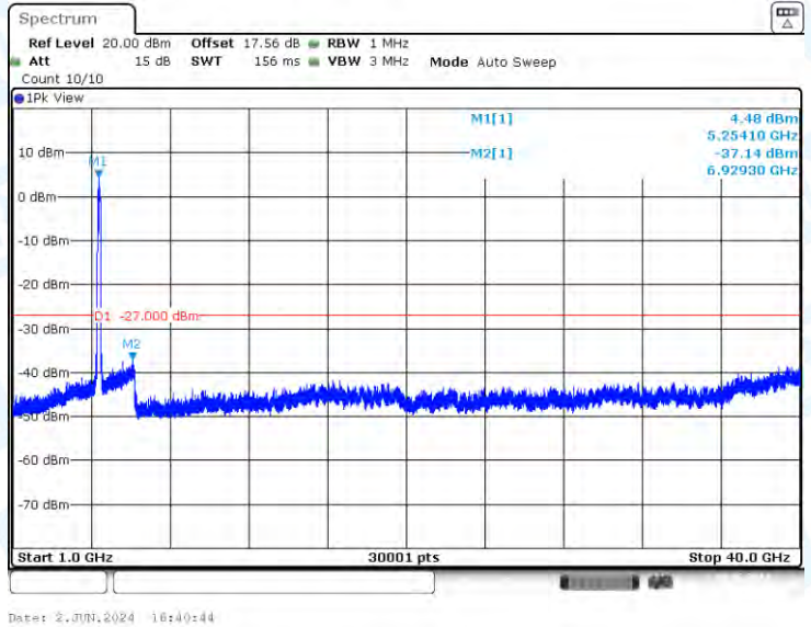
11AC160-CDD-Ant2-5250-1000~40000-PASS
