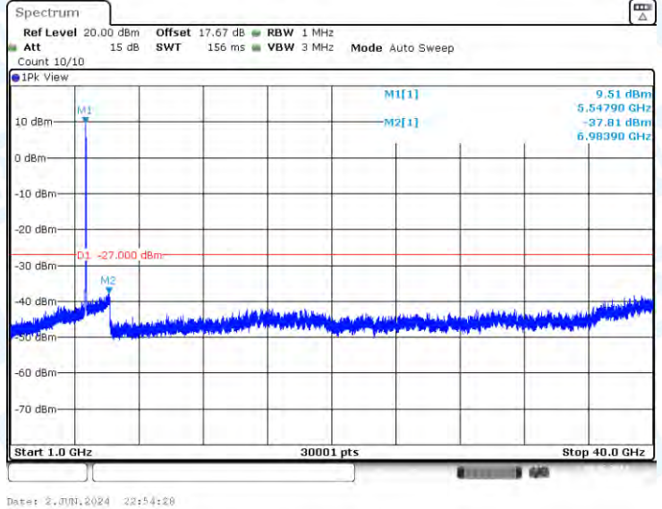
11AC40-CDD-Ant2-5550-1000~40000-PASS
