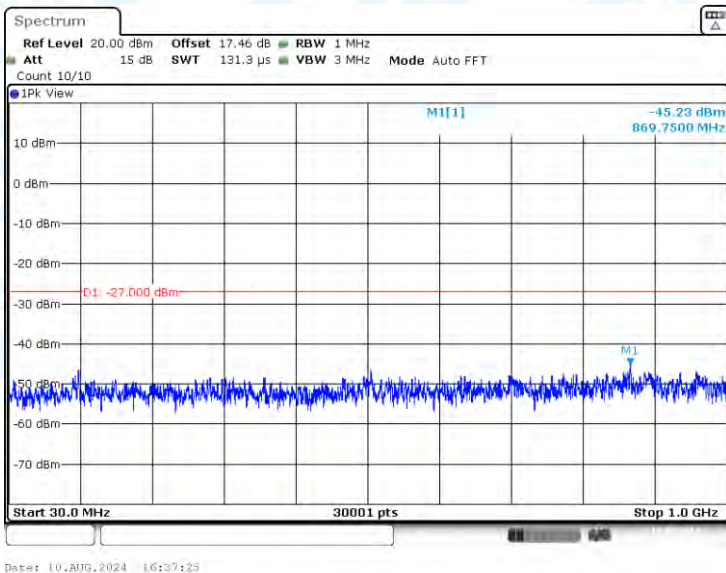
11AC80-CDD-Ant1-5210-30~1000-PASS
