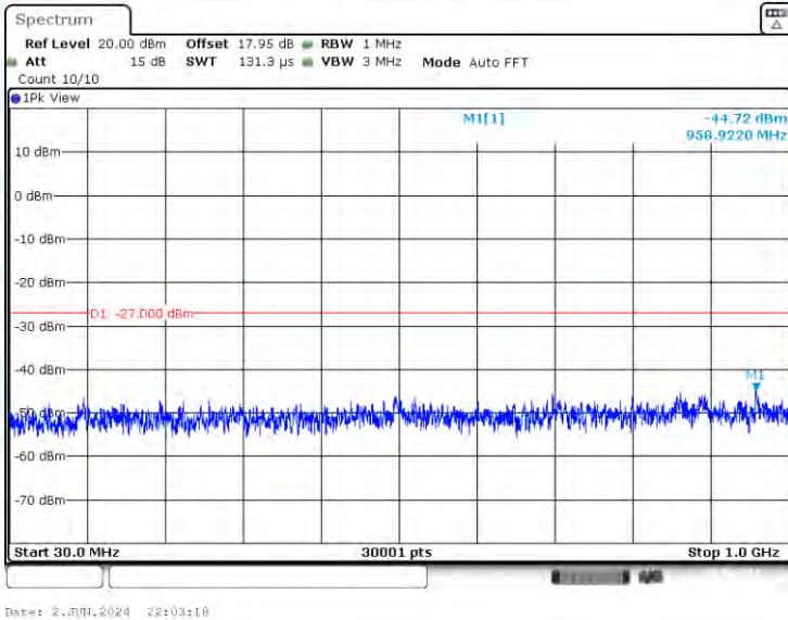
11N40-CDD-Ant3-5710-30~1000-PASS
