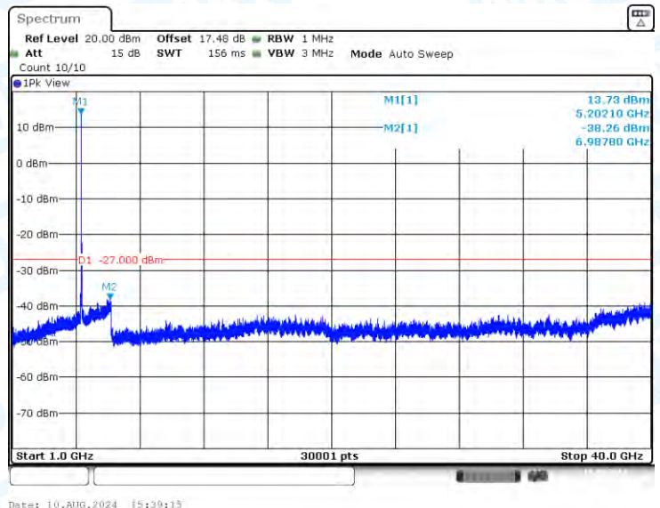
11AC20-CDD-Ant1-5200-1000~40000-PASS
