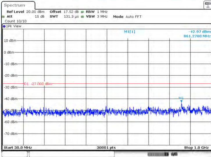
11AC40-CDD-Ant1-5310-30~1000-PASS
