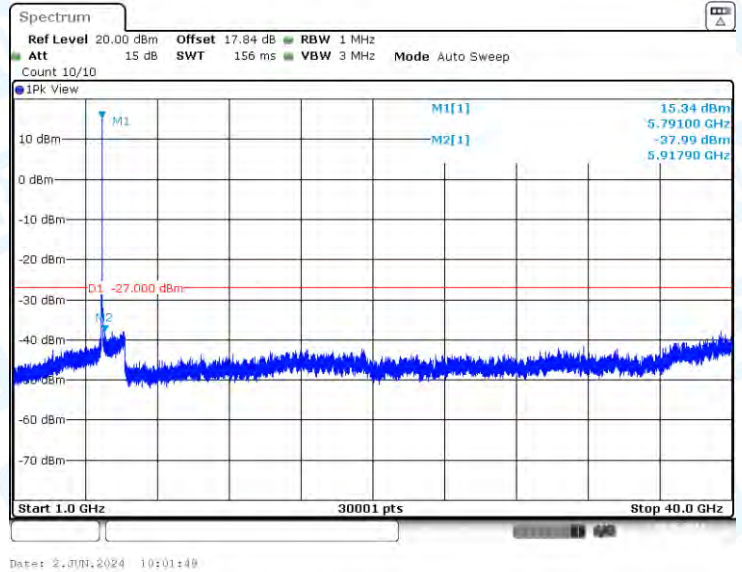
11AC20-CDD-Ant3-5785-1000~40000-PASS
