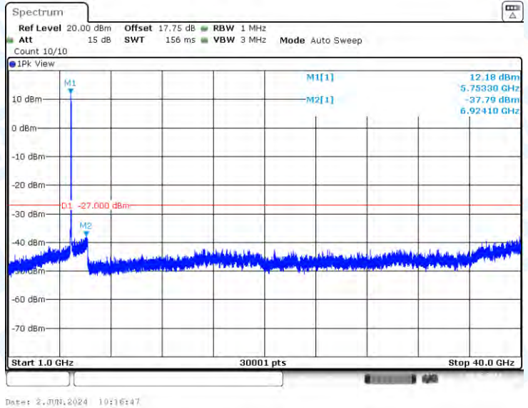
11AC40-CDD-Ant1-5755-1000~40000-PASS
