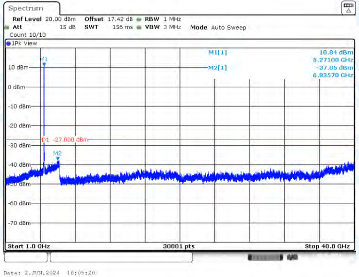
11AC40-CDD-Ant1-5270-1000~40000-PASS
