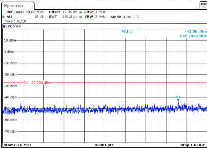
11AC20-CDD-Ant2-5720-30~1000-PASS
