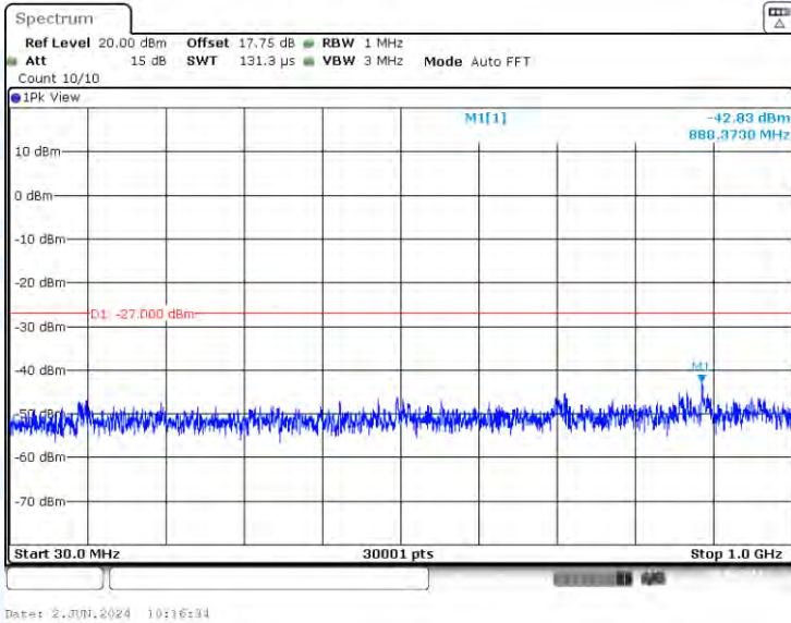
11AC40-CDD-Ant1-5755-30~1000-PASS
