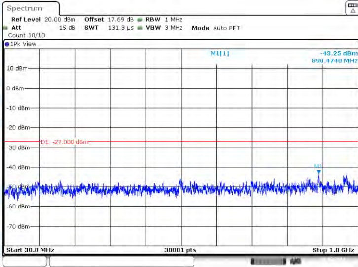
11AC40-CDD-Ant3-5755-30~1000-PASS
