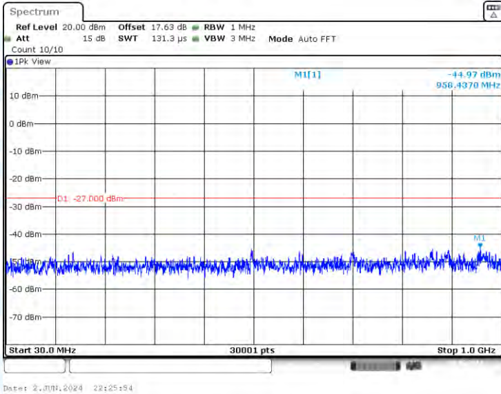
11AC20-CDD-Ant2-5580-30~1000-PASS
