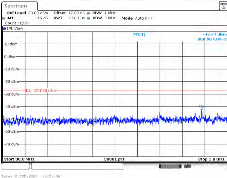
11AC80-CDD-Ant2-5610-30~1000-PASS
