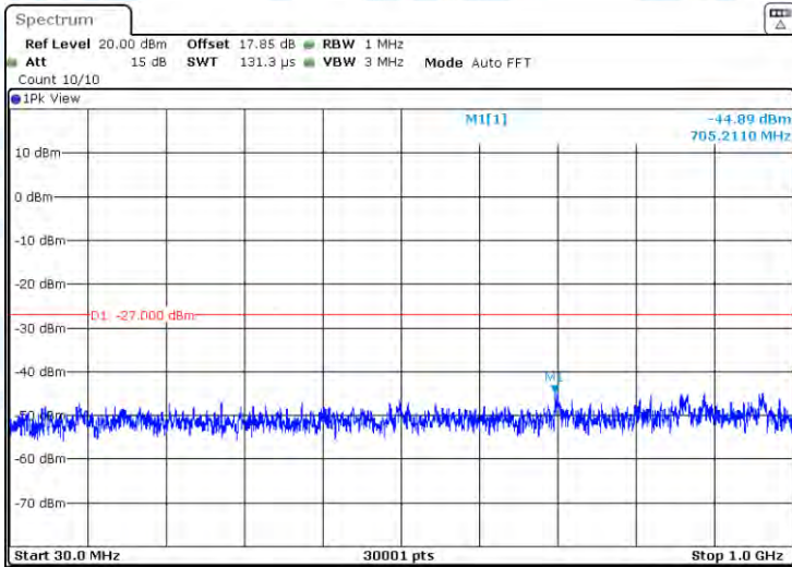
11N40-CDD-Ant2-5755-30~1000-PASS
