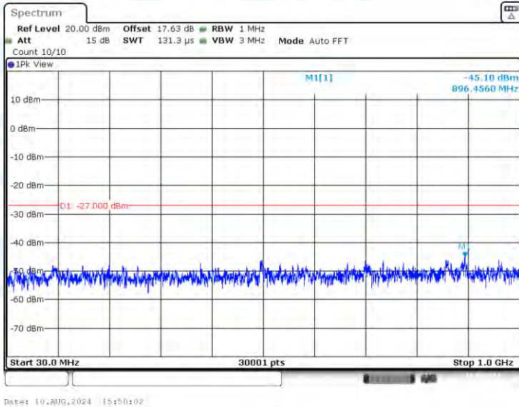
11AC20-CDD-Ant3-5240-30~1000-PASS
