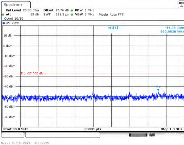
11N40-CDD-Ant2-5795-30~1000-PASS
