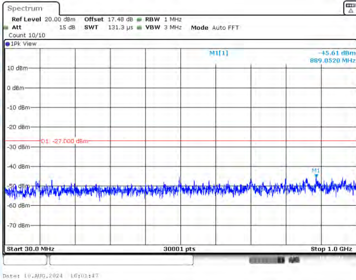
11AC40-CDD-Ant2-5190-30~1000-PASS
