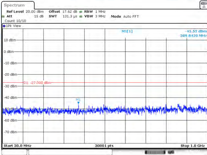
11AC40-CDD-Ant3-5510-30~1000-PASS
