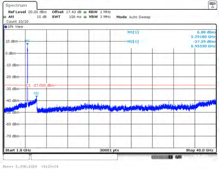
11AC80-CDD-Ant1-5290-1000~40000-PASS
