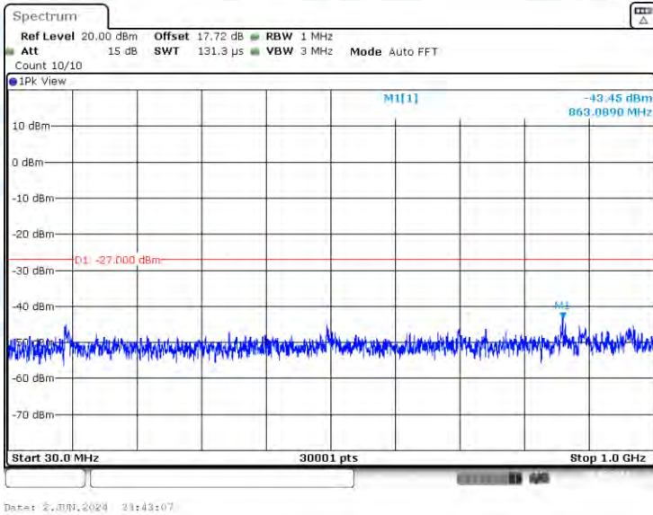
11AC160-CDD-Ant3-5570-30~1000-PASS
