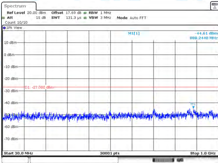
11AC80-CDD-Ant2-5530-30~1000-PASS
