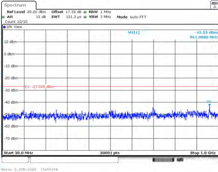
11AC20-CDD-Ant3-5320-30~1000-PASS
