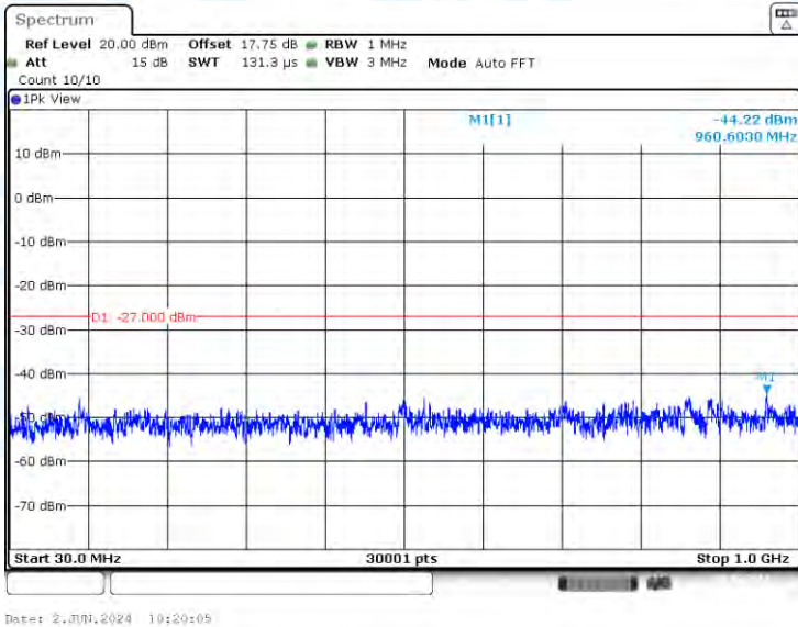
11AC40-CDD-Ant2-5755-30~1000-PASS
