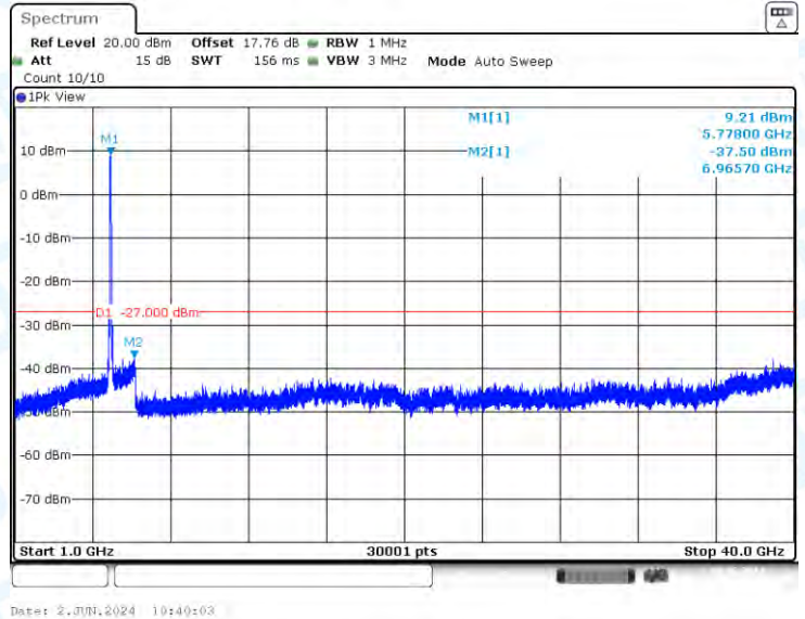
11AC80-CDD-Ant1-5775-1000~40000-PASS
