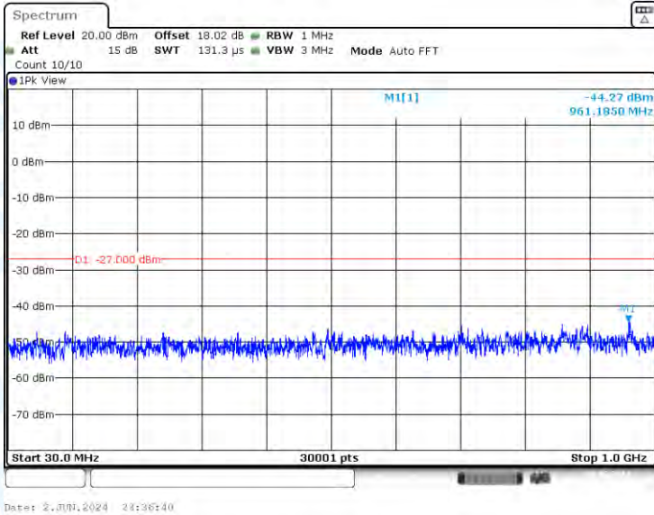
11AC80-CDD-Ant3-5690-30~1000-PASS
