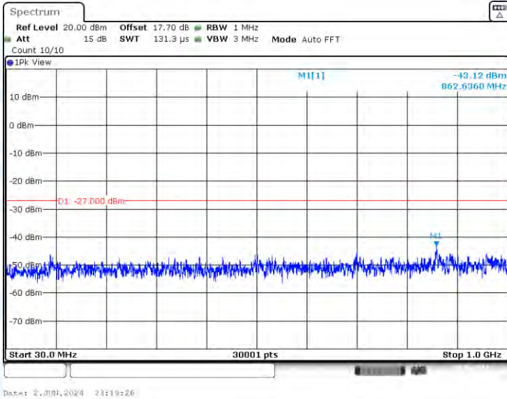
11AC80-CDD-Ant1-5610-30~1000-PASS
