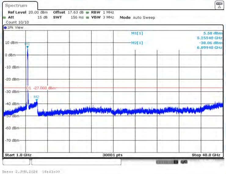
11AC160-CDD-Ant3-5250-1000~40000-PASS
