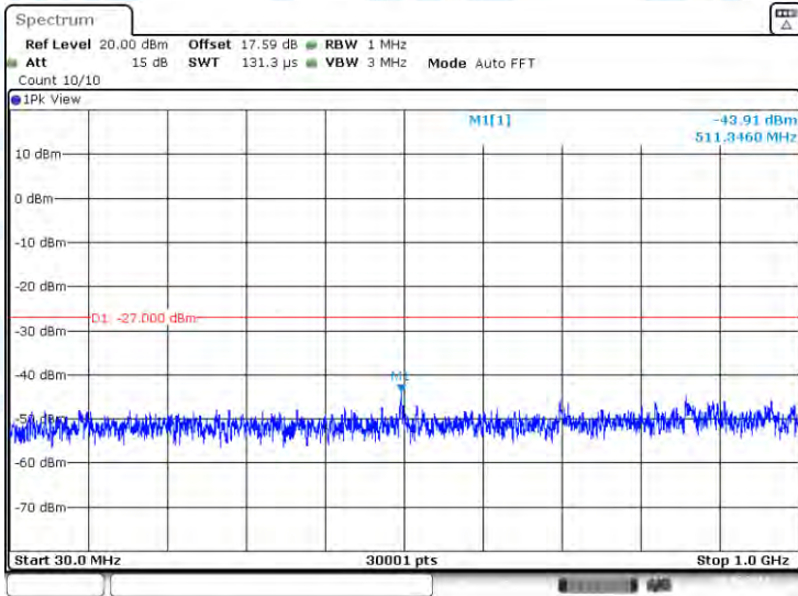
11AC20-CDD-Ant3-5500-30~1000-PASS
