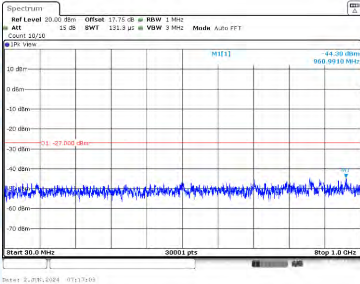
11AC20-CDD-Ant1-5745-30~1000-PASS
