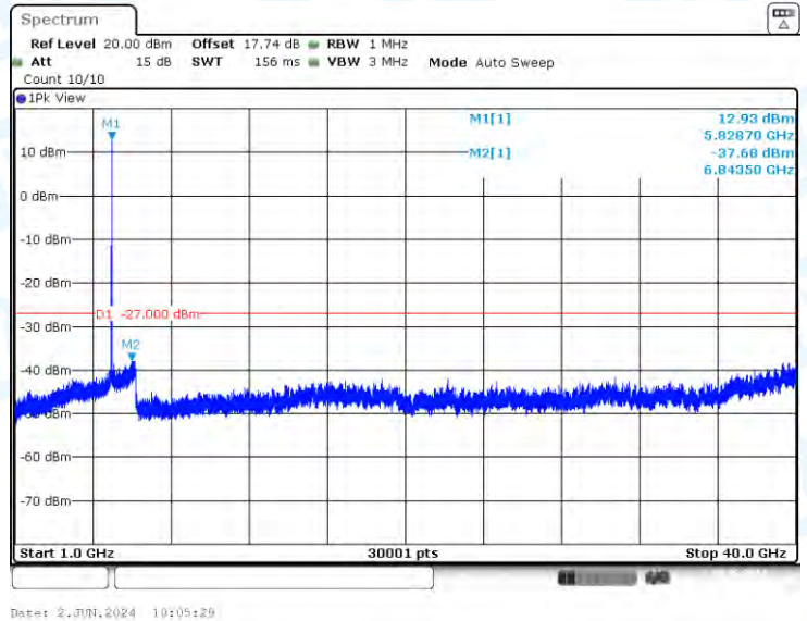
11AC20-CDD-Ant1-5825-1000~40000-PASS
