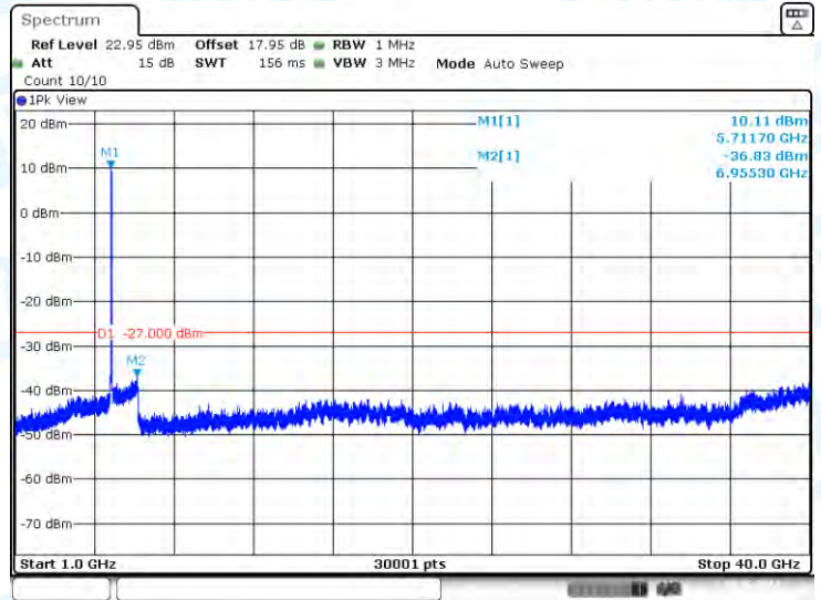
11AC40-CDD-Ant2-5710-1000~40000-PASS
