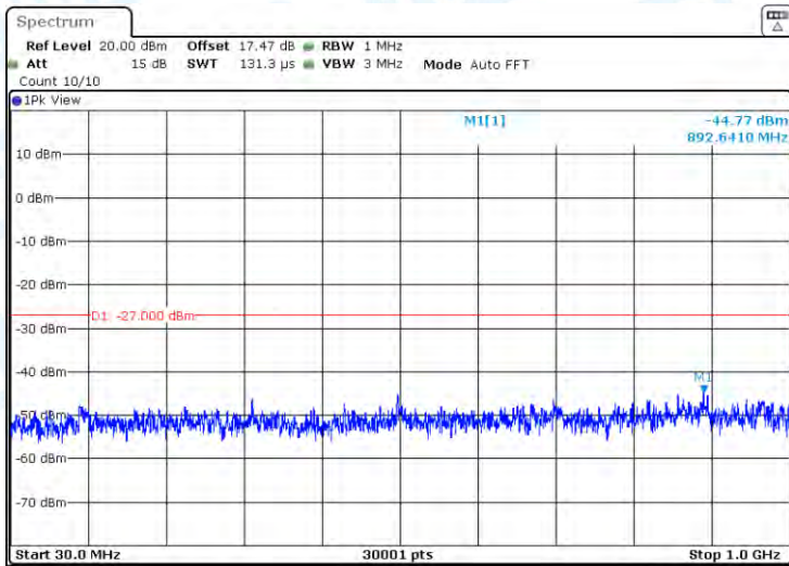
11AC80-CDD-Ant3-5775-30~1000-PASS
