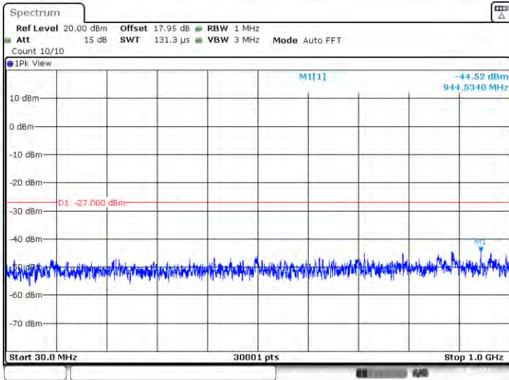
11AC40-CDD-Ant2-5710-30~1000-PASS
