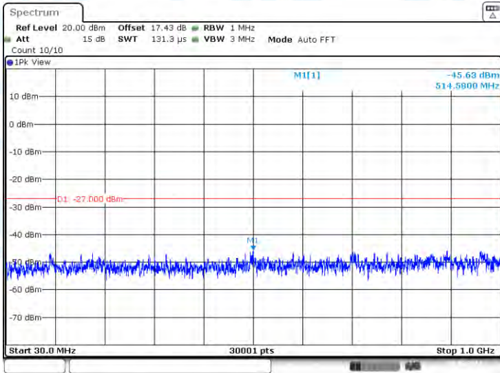
11AC80-CDD-Ant3-5210-30~1000-PASS
