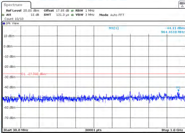
11AC80-CDD-Ant2-5775-30~1000-PASS
