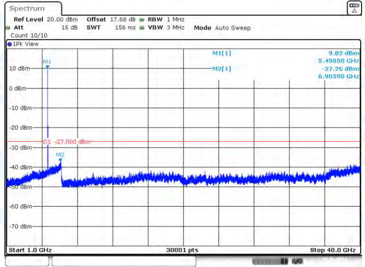
11AC20-CDD-Ant2-5500-1000~40000-PASS
