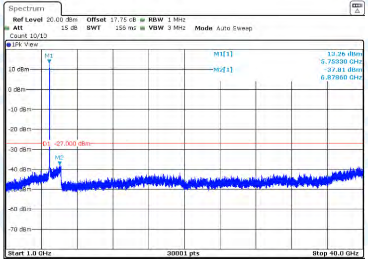
11N40-CDD-Ant1-5755-1000~40000-PASS
