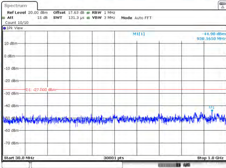
11AC20-CDD-Ant2-5260-30~1000-PASS
