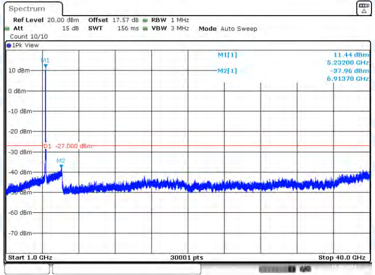
11AC40-CDD-Ant1-5230-1000~40000-PASS
