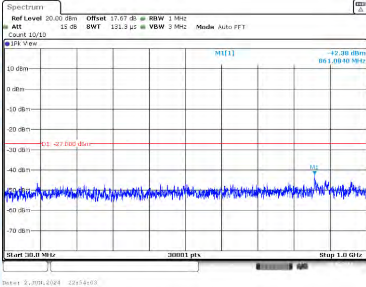
11AC40-CDD-Ant2-5550-30~1000-PASS
