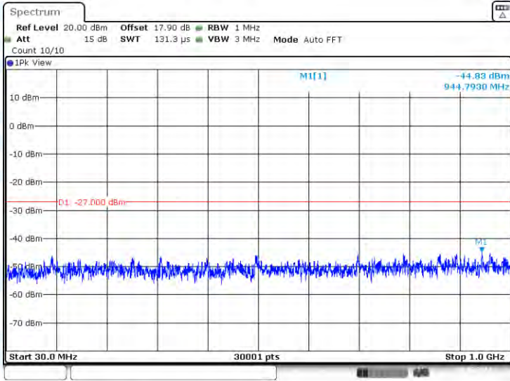
11AC80-CDD-Ant3-5610-30~1000-PASS
