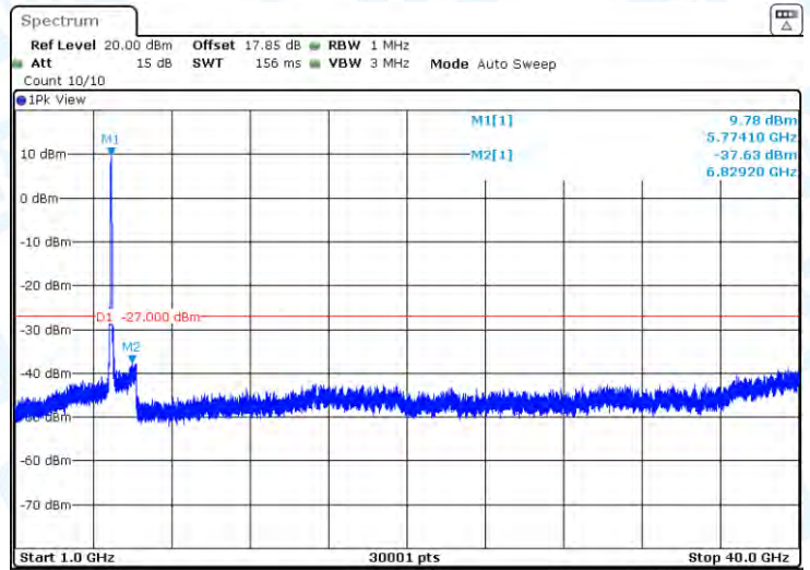
11AC80-CDD-Ant2-5775-1000~40000-PASS
