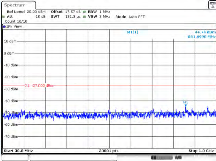
11AC40-CDD-Ant1-5230-30~1000-PASS
