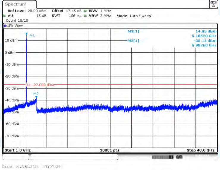
11AX20-CDD-Ant1-5180-1000~40000-PASS
