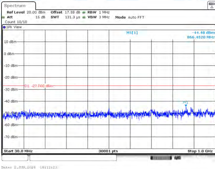
11AC40-CDD-Ant2-5270-30~1000-PASS
