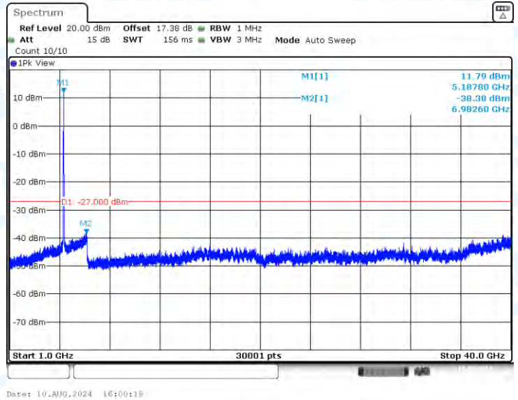
11AC40-CDD-Ant1-5190-1000~40000-PASS
