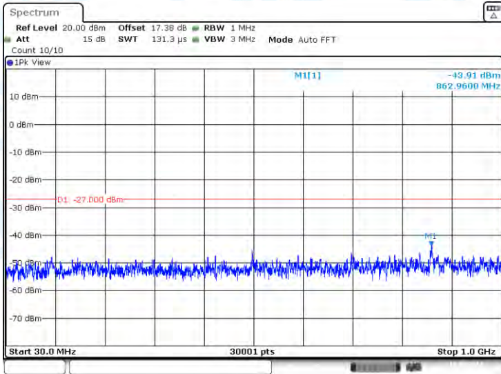
11AC20-CDD-Ant3-5825-30~1000-PASS
