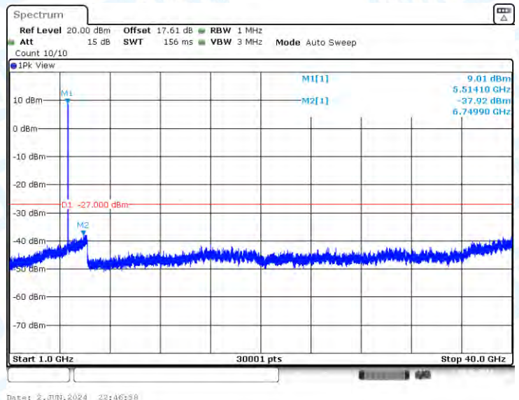
11AC40-CDD-Ant1-5510-1000~40000-PASS
