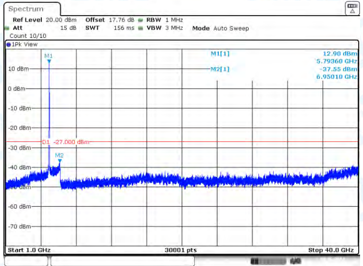
11AC40-CDD-Ant1-5795-1000~40000-PASS
