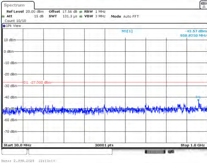
11AC20-CDD-Ant1-5500-30~1000-PASS
