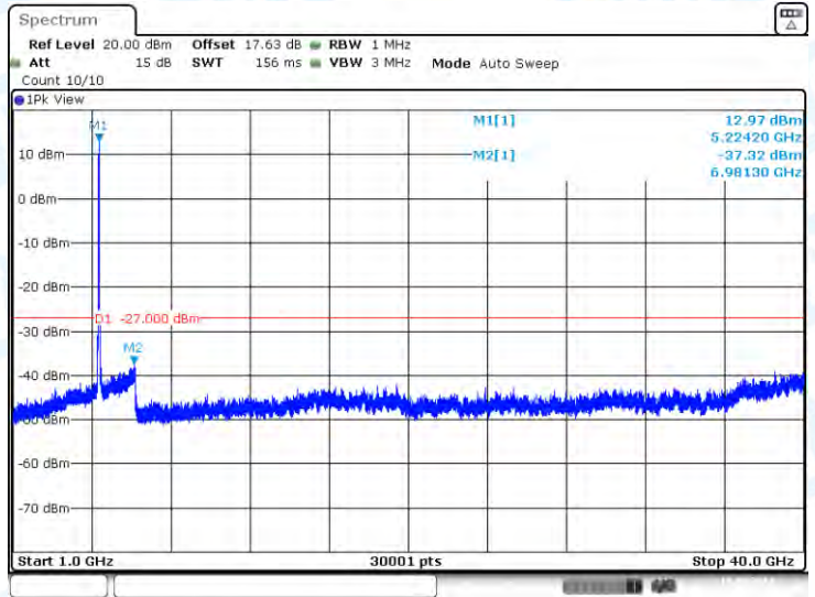
11AC40-CDD-Ant2-5230-1000~40000-PASS
