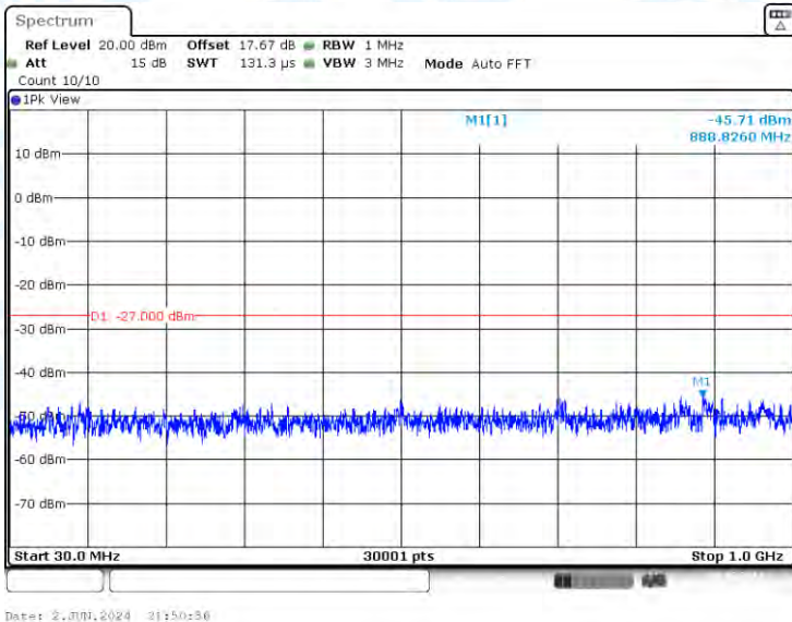
11N40-CDD-Ant1-5550-30~1000-PASS
