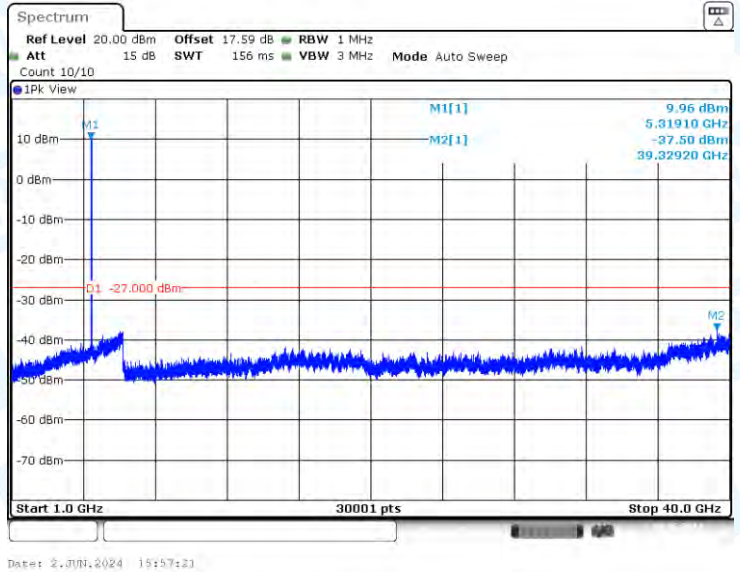
11AC20-CDD-Ant3-5320-1000~40000-PASS
