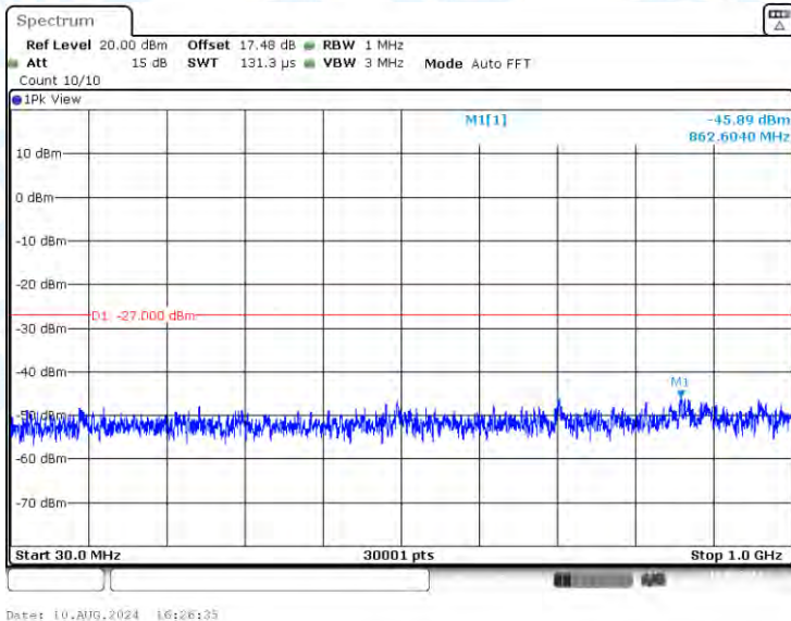
11AC40-CDD-Ant3-5190-30~1000-PASS
