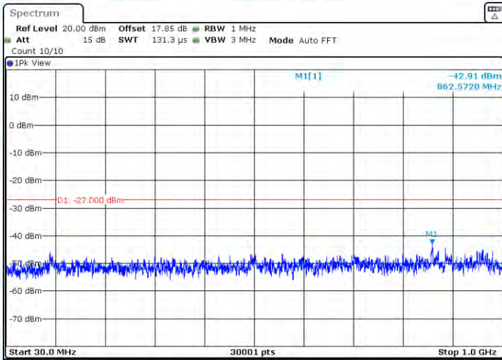
11AC20-CDD-Ant1-5720-30~1000-PASS
