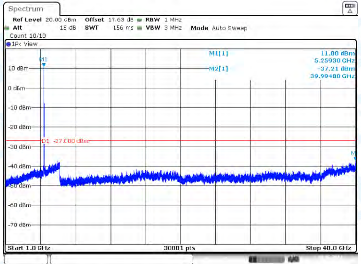
11AC20-CDD-Ant2-5260-1000~40000-PASS
