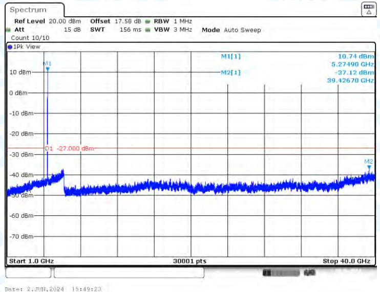
11AC20-CDD-Ant2-5280-1000~40000-PASS
