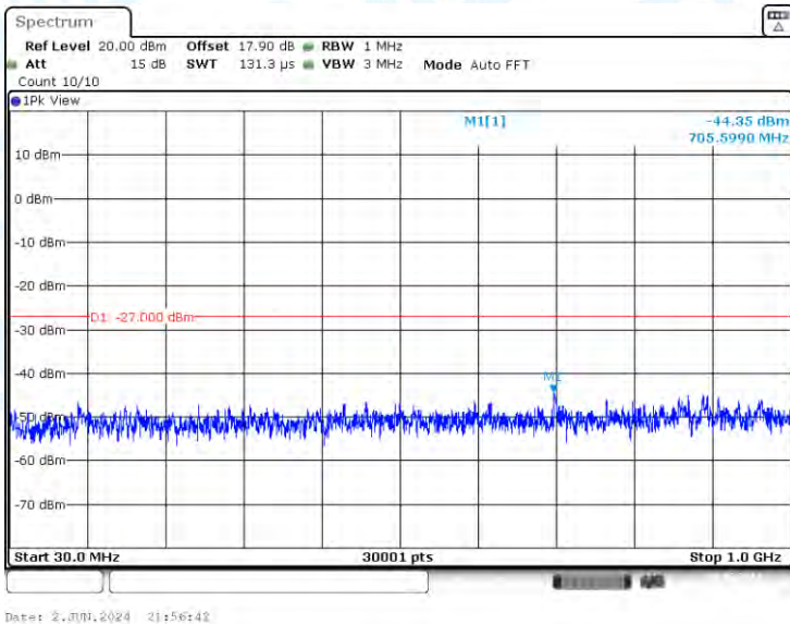
11N40-CDD-Ant1-5710-30~1000-PASS
