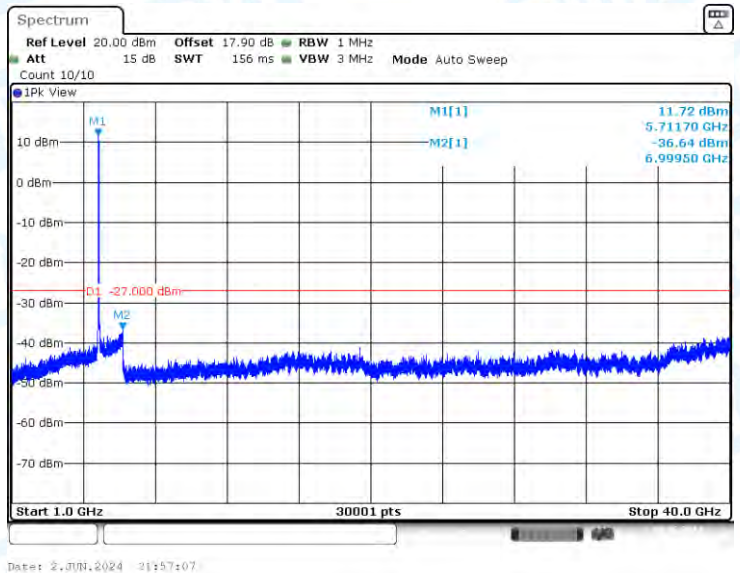
11N40-CDD-Ant1-5710-1000~40000-PASS
