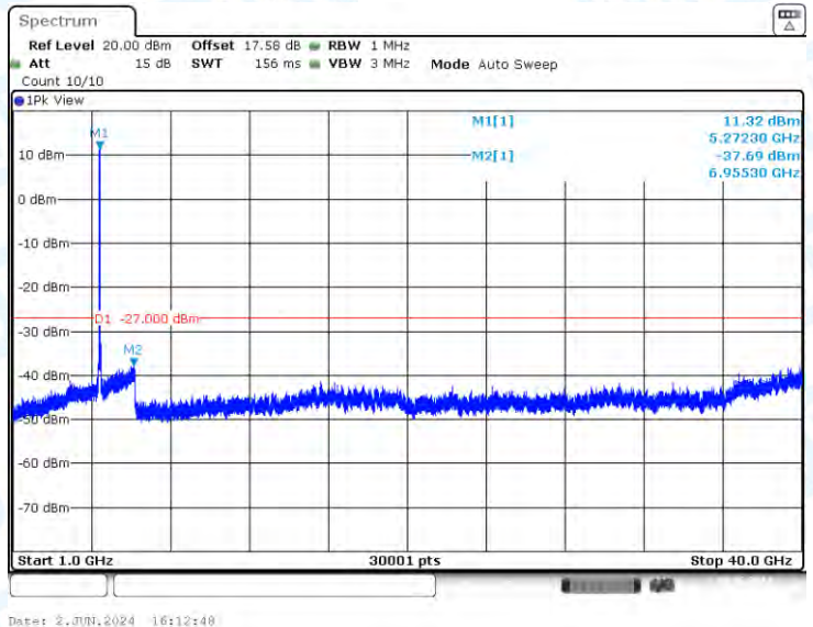
11AC40-CDD-Ant2-5270-1000~40000-PASS
