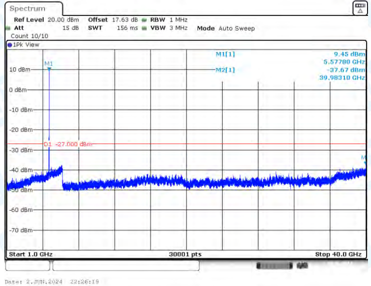
11AC20-CDD-Ant2-5580-1000~40000-PASS
