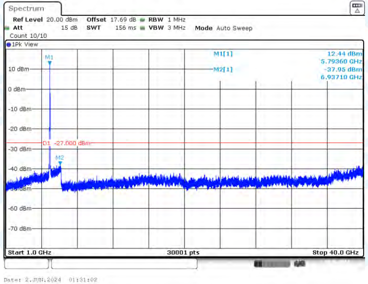
11N40-CDD-Ant1-5795-1000~40000-PASS
