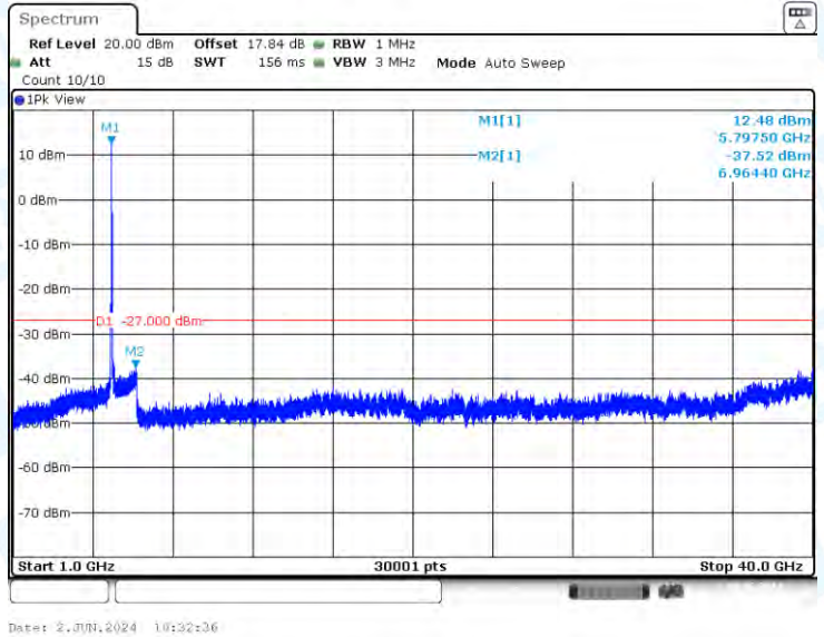
11AC40-CDD-Ant3-5795-1000~40000-PASS
