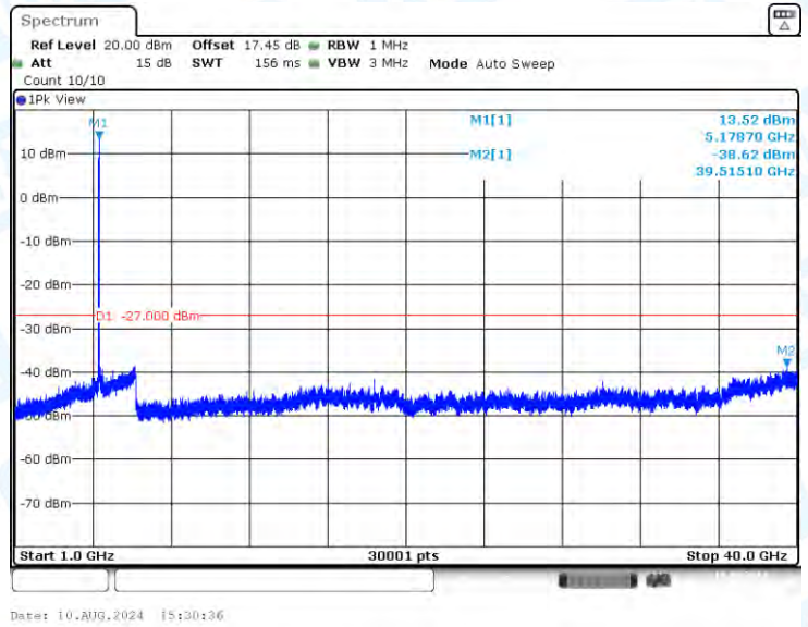
11AC20-CDD-Ant1-5180-1000~40000-PASS
