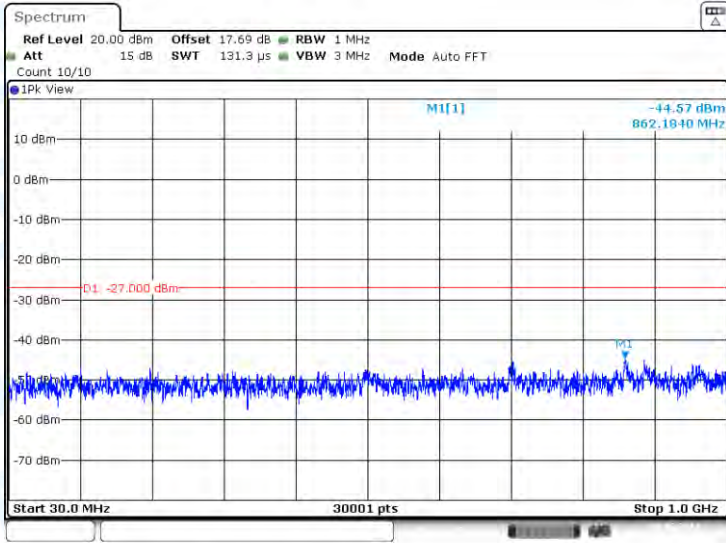
11AC20-CDD-Ant3-5745-30~1000-PASS
