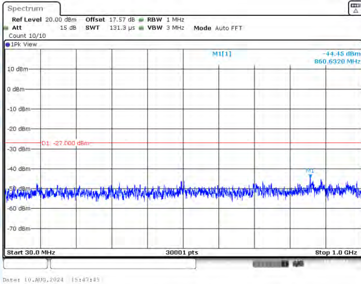
11AC20-CDD-Ant2-5240-30~1000-PASS
