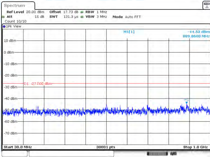
11N40-CDD-Ant2-5550-30~1000-PASS
