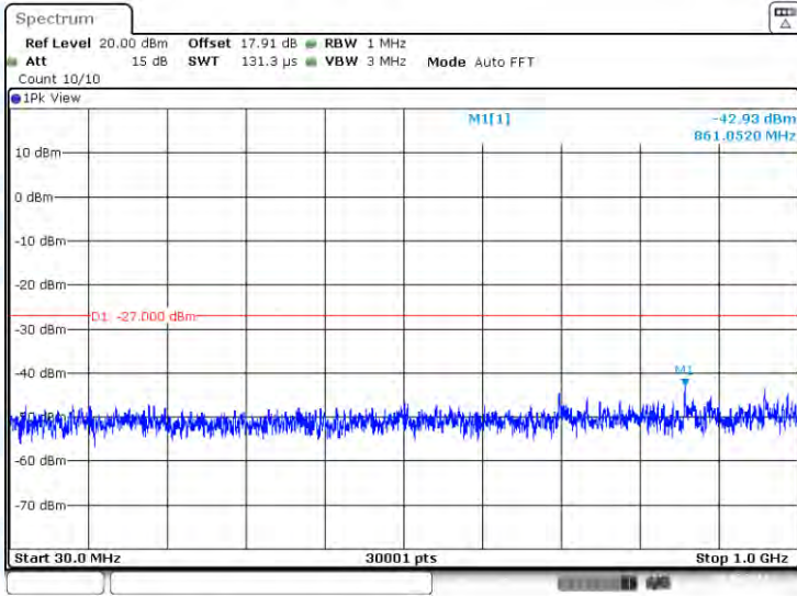
11AC20-CDD-Ant2-5825-30~1000-PASS
