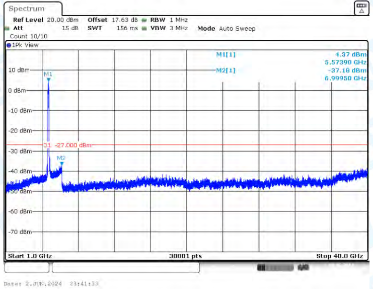
11AC160-CDD-Ant2-5570-1000~40000-PASS
