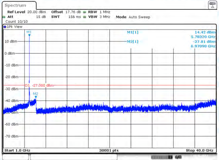
11AC20-CDD-Ant1-5785-1000~40000-PASS
