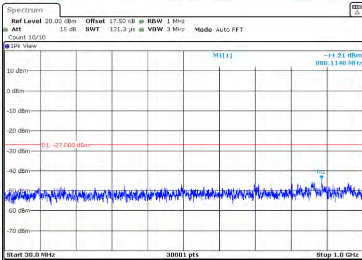
11AC20-CDD-Ant1-5180-30~1000-PASS
