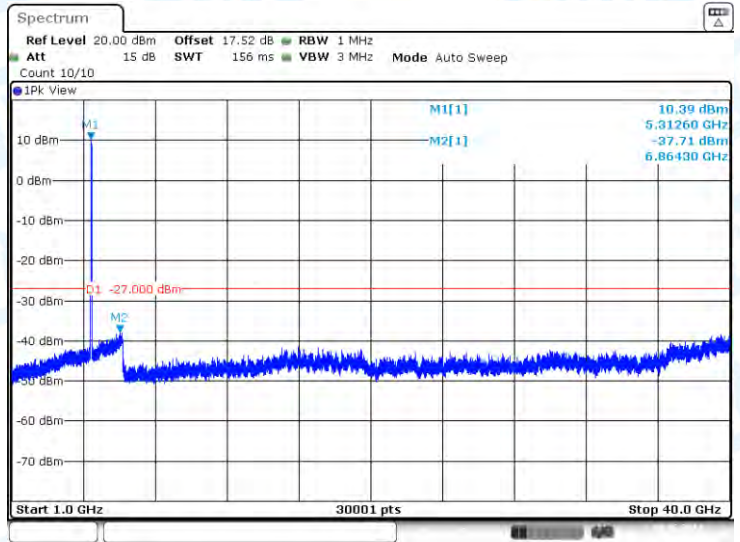
11AC40-CDD-Ant1-5310-1000~40000-PASS
