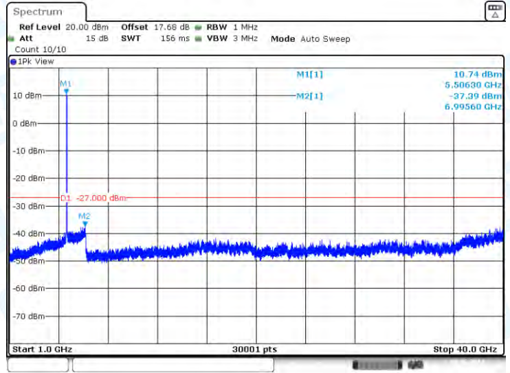
11AC40-CDD-Ant2-5510-1000~40000-PASS
