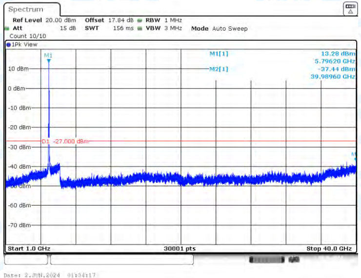
11N40-CDD-Ant2-5795-1000~40000-PASS
