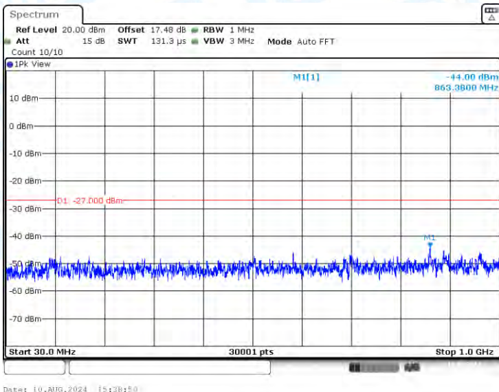
11AC20-CDD-Ant1-5200-30~1000-PASS
