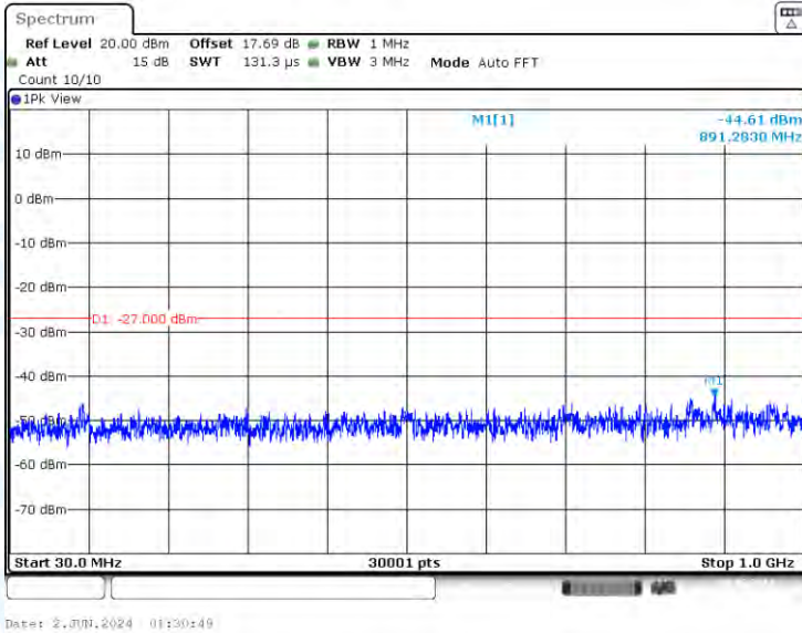
11N40-CDD-Ant1-5795-30~1000-PASS
