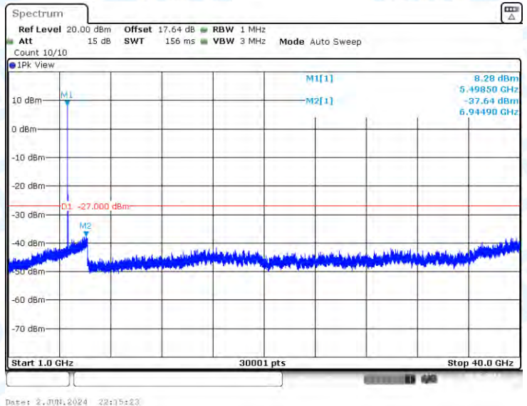
11AC20-CDD-Ant1-5500-1000~40000-PASS
