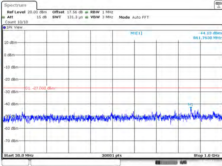
11AC20-CDD-Ant1-5260-30~1000-PASS
