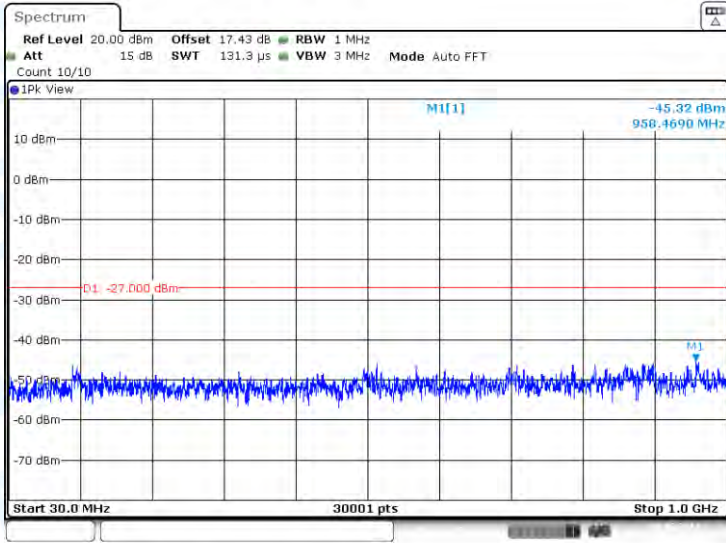
11AC40-CDD-Ant3-5270-30~1000-PASS
