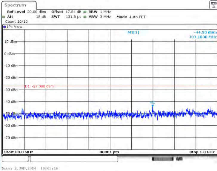
11AC20-CDD-Ant3-5785-30~1000-PASS
