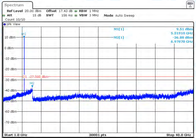
11AC20-CDD-Ant3-5280-1000~40000-PASS
