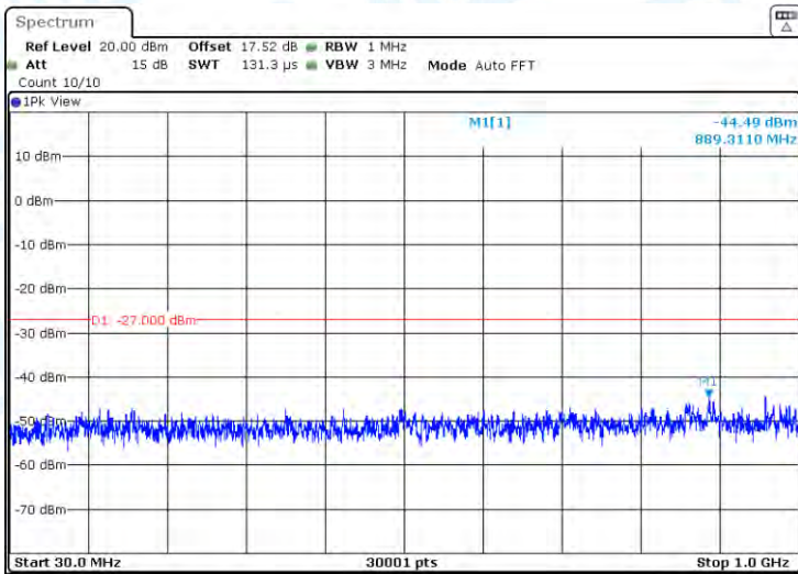
11AC20-CDD-Ant1-5320-30~1000-PASS
