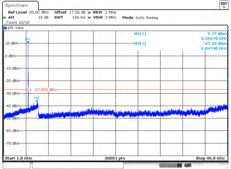
11AC20-CDD-Ant1-5260-1000~40000-PASS
