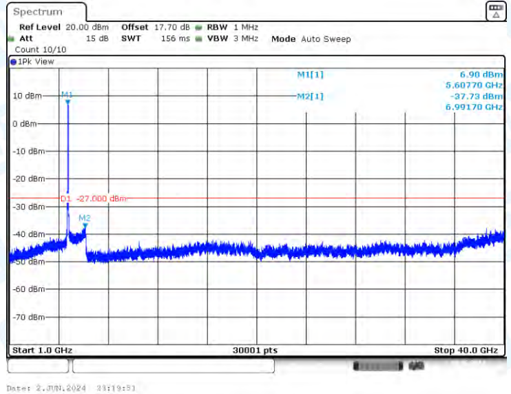
11AC80-CDD-Ant1-5610-1000~40000-PASS
