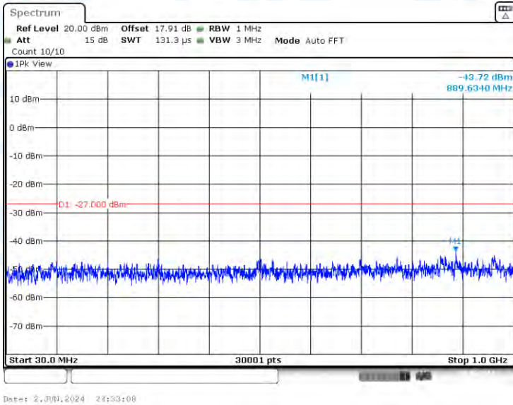
11AC80-CDD-Ant2-5690-30~1000-PASS
