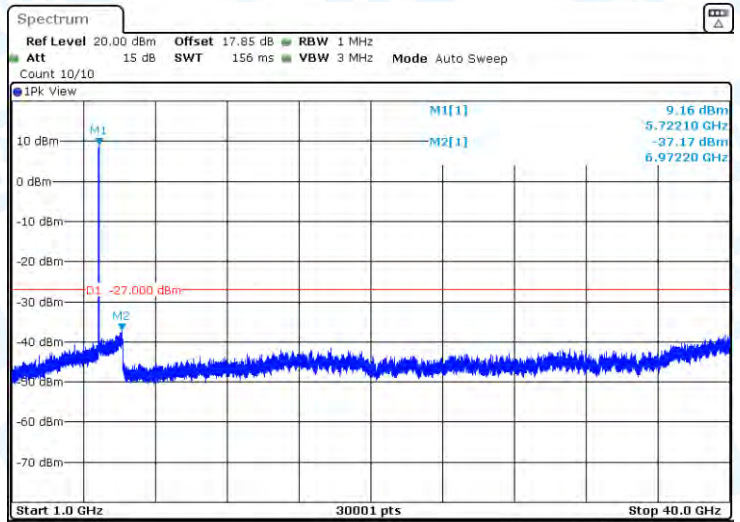
11AC20-CDD-Ant1-5720-1000~40000-PASS
