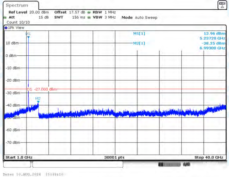
11AC20-CDD-Ant2-5240-1000~40000-PASS
