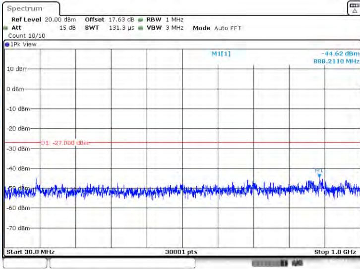
11AC160-CDD-Ant1-5570-30~1000-PASS
