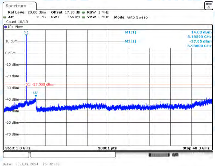
11AC20-CDD-Ant2-5180-1000~40000-PASS
