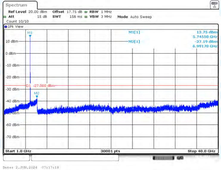
11AC20-CDD-Ant1-5745-1000~40000-PASS
