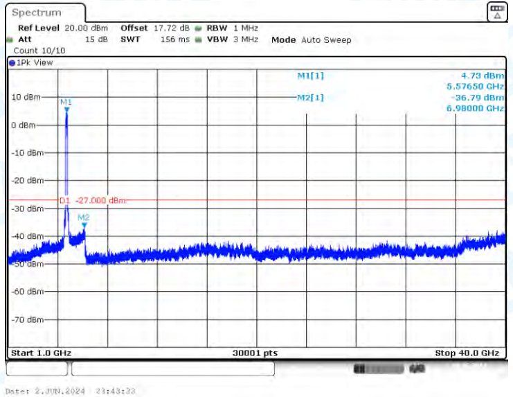
11AC160-CDD-Ant3-5570-1000~40000-PASS
