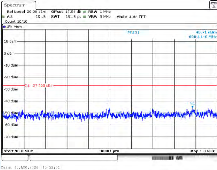
11AC20-CDD-Ant3-5180-30~1000-PASS
