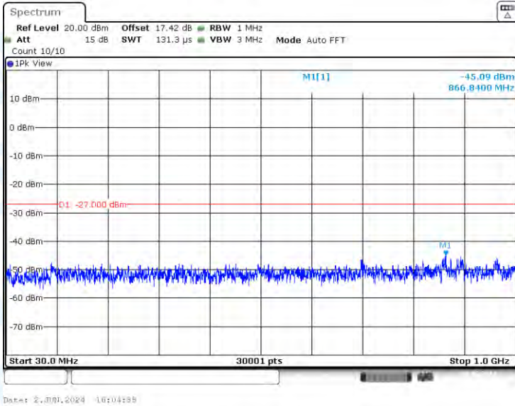
11AC40-CDD-Ant1-5270-30~1000-PASS
