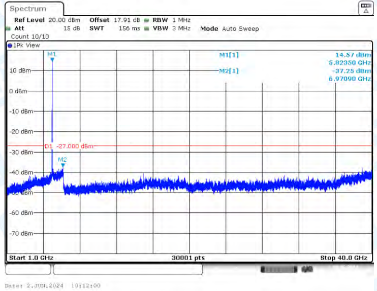
11AC20-CDD-Ant3-5825-1000~40000-PASS
