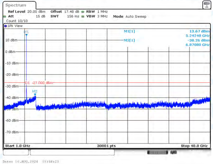
11AC20-CDD-Ant1-5240-1000~40000-PASS
