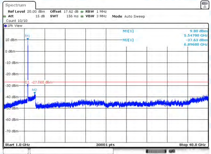
11AC40-CDD-Ant3-5510-1000~40000-PASS
