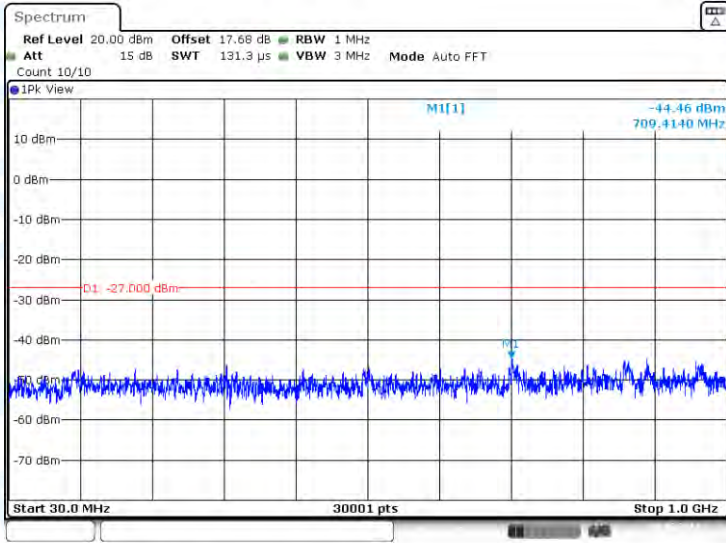
11AC20-CDD-Ant2-5500-30~1000-PASS
