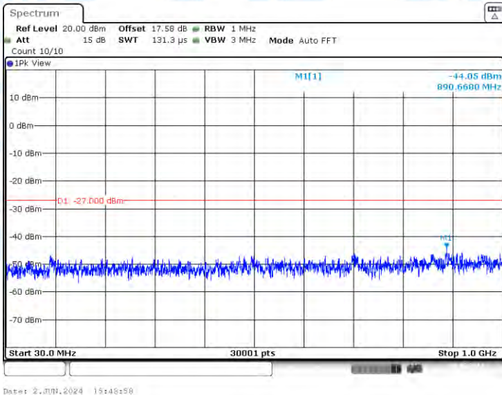
11AC20-CDD-Ant2-5280-30~1000-PASS
