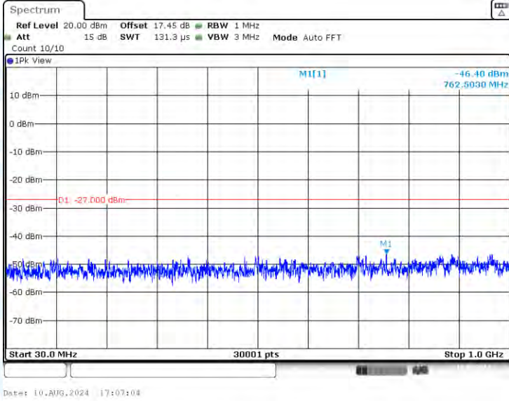
11AX20-CDD-Ant1-5180-30~1000-PASS
