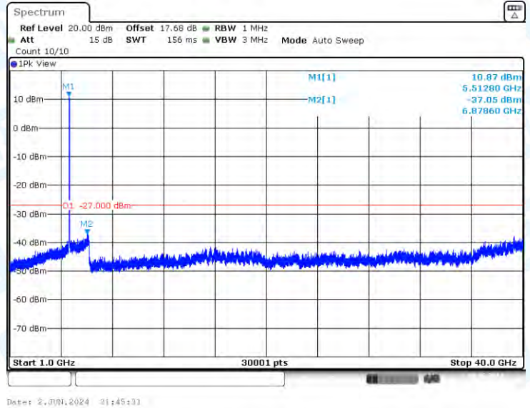
11N40-CDD-Ant3-5510-1000~40000-PASS
