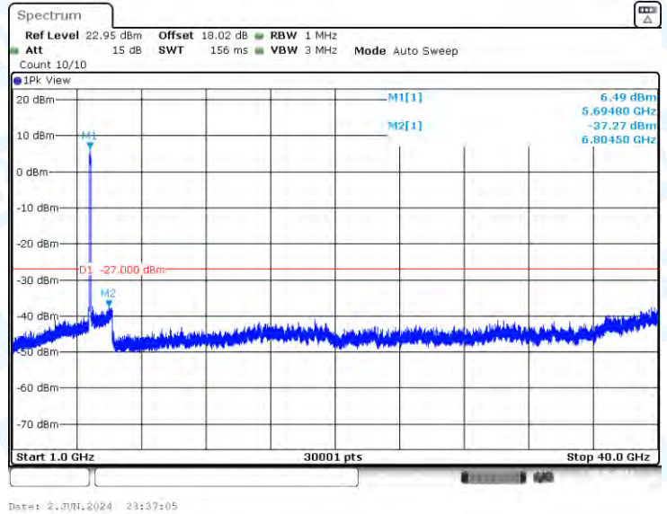
11AC80-CDD-Ant3-5690-1000~40000-PASS
