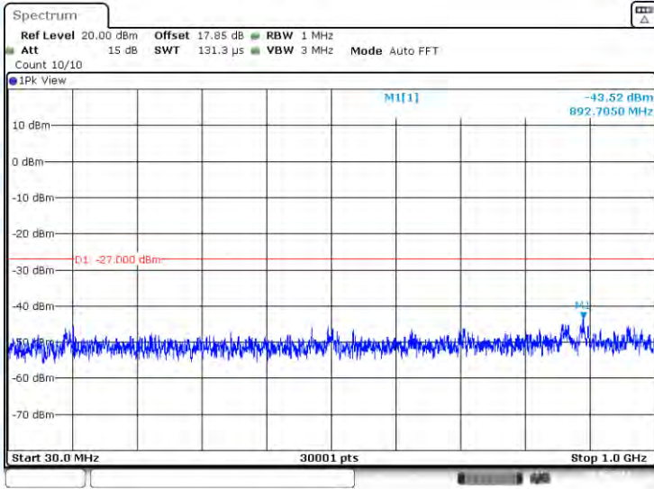
11AC40-CDD-Ant1-5710-30~1000-PASS
