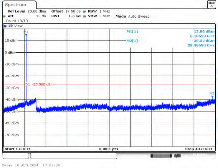
11AX20-CDD-Ant2-5180-1000~40000-PASS
