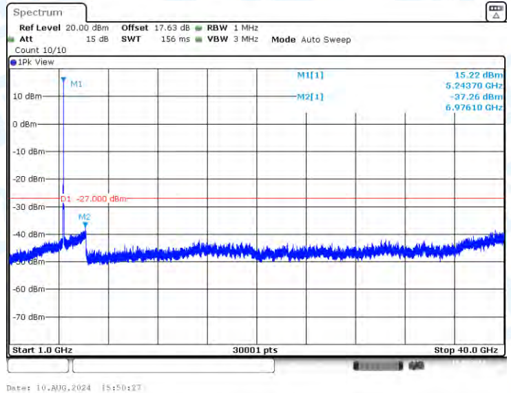
11AC20-CDD-Ant3-5240-1000~40000-PASS
