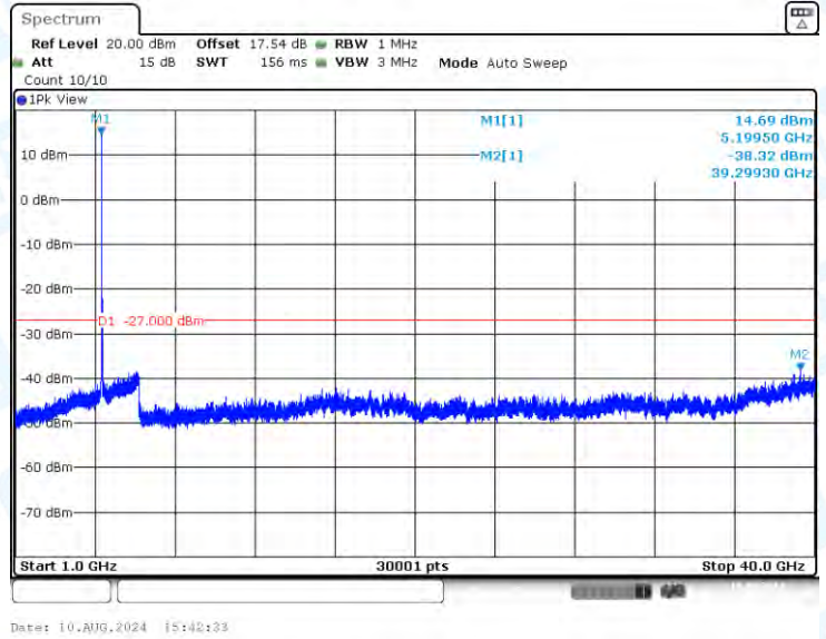
11AC20-CDD-Ant3-5200-1000~40000-PASS
