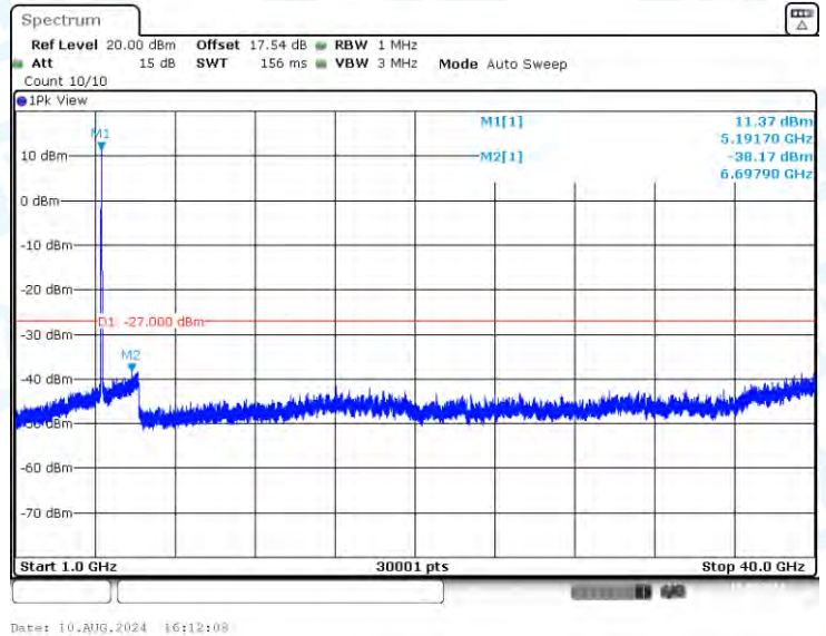
11AC40-CDD-Ant3-5190-1000~40000-PASS
