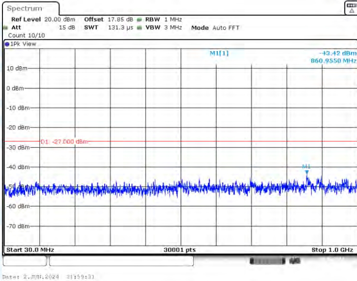
11N40-CDD-Ant2-5710-30~1000-PASS
