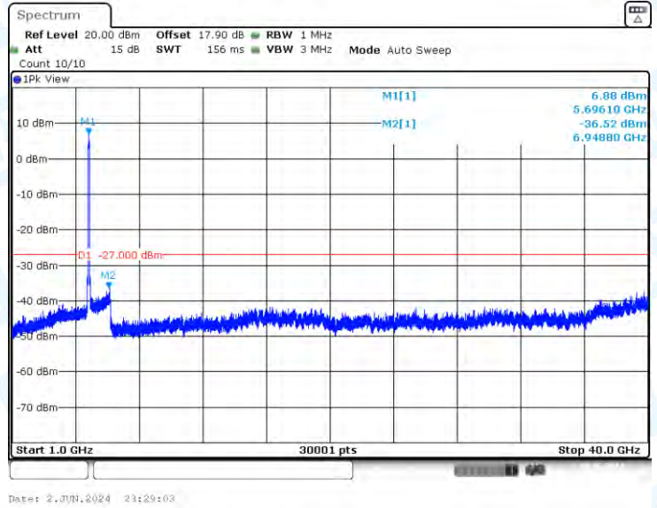
11AC80-CDD-Ant1-5690-1000~40000-PASS
