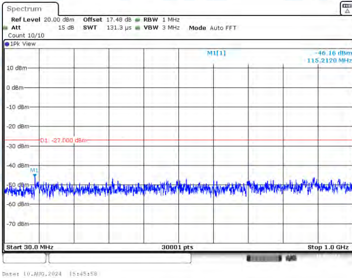
11AC20-CDD-Ant1-5240-30~1000-PASS
