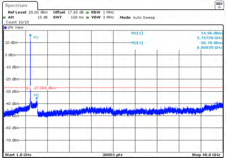
11N40-CDD-Ant2-5755-1000~40000-PASS
