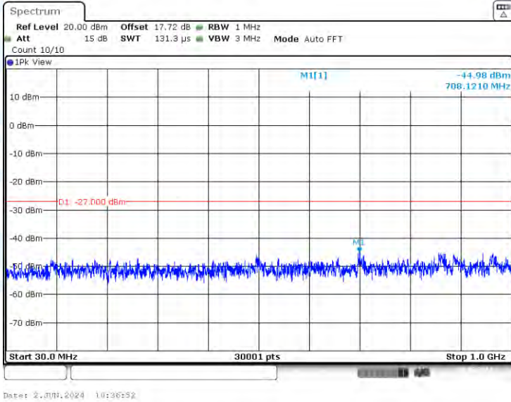
11AC80-CDD-Ant1-5775-30~1000-PASS
