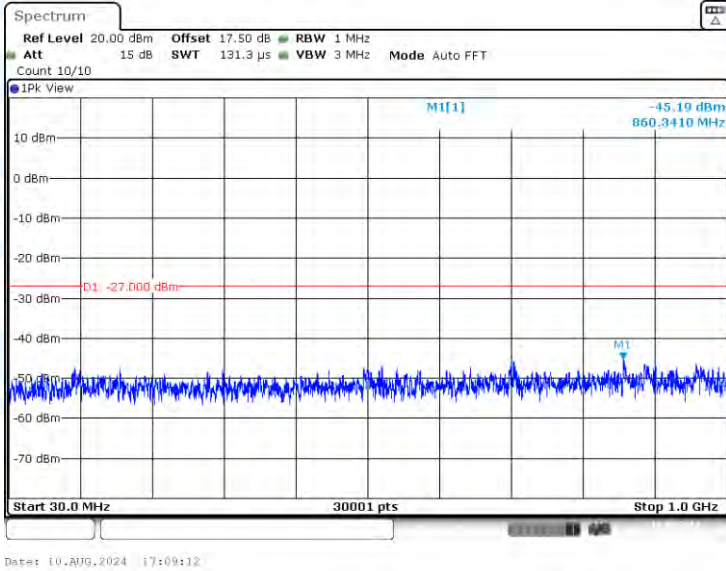
11AX20-CDD-Ant2-5180-30~1000-PASS
