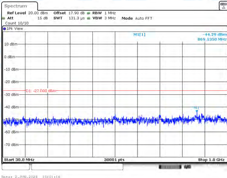
11AC40-CDD-Ant3-5550-30~1000-PASS
