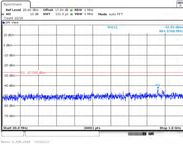
11AC40-CDD-Ant3-5795-30~1000-PASS
