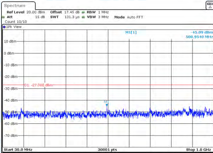
11N40-CDD-Ant3-5795-30~1000-PASS
