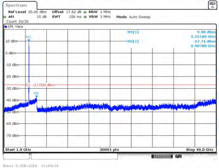
11N40-CDD-Ant1-5550-1000~40000-PASS
