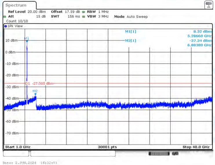
11AC80-CDD-Ant3-5290-1000~40000-PASS
