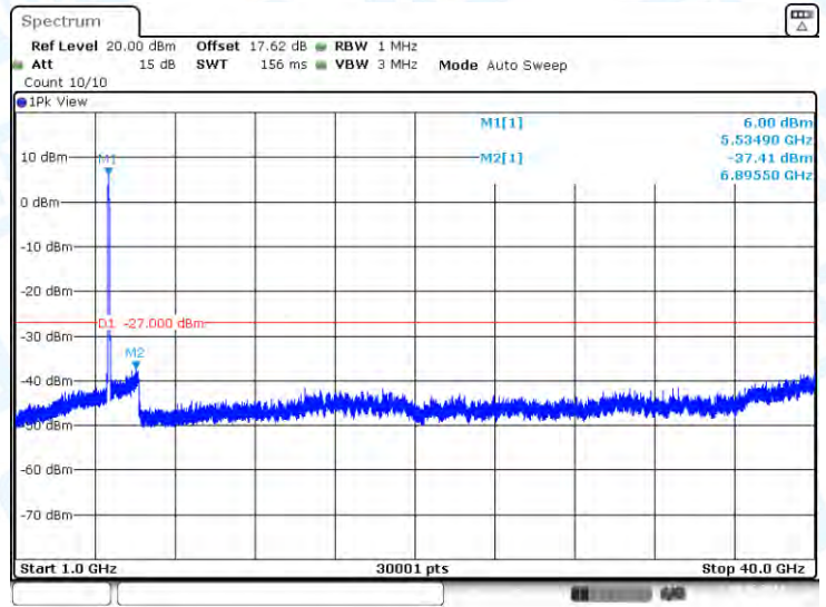
11AC80-CDD-Ant1-5530-1000~40000-PASS
