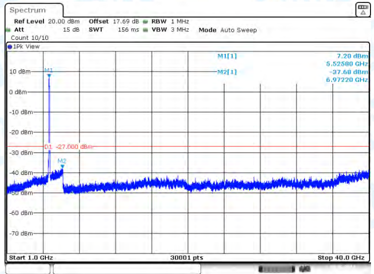
11AC80-CDD-Ant2-5530-1000~40000-PASS
