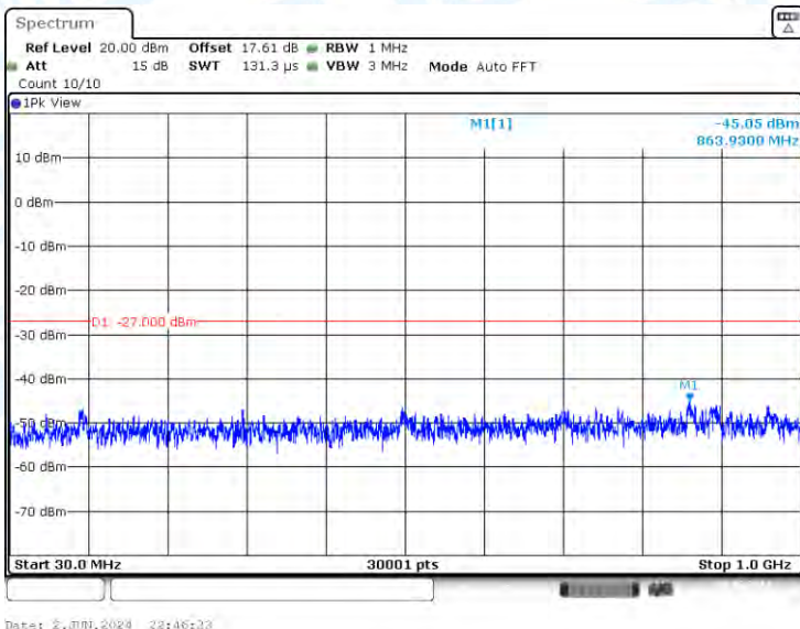
11AC40-CDD-Ant1-5510-30~1000-PASS
