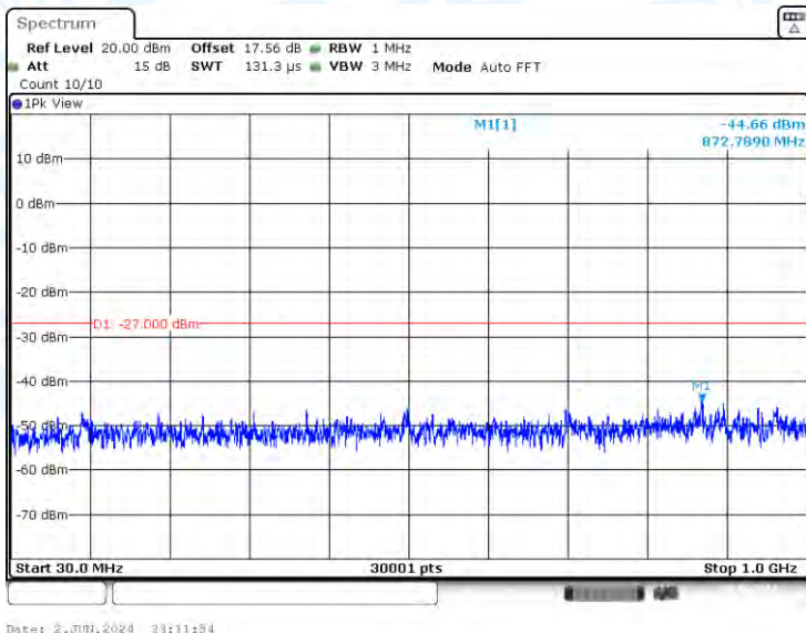
11AC80-CDD-Ant3-5290-30~1000-PASS
