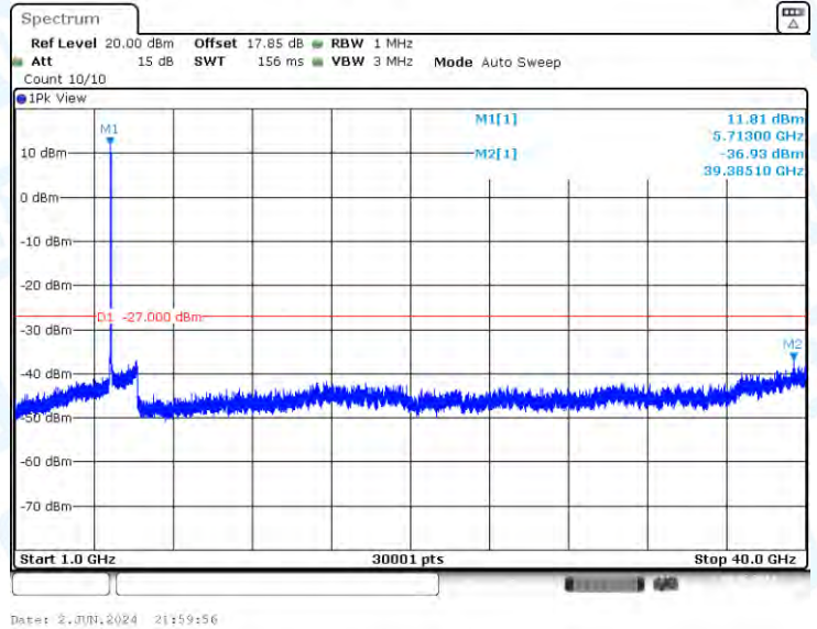
11N40-CDD-Ant2-5710-1000~40000-PASS
