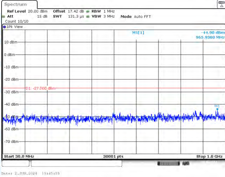
11AC20-CDD-Ant1-5280-30~1000-PASS
