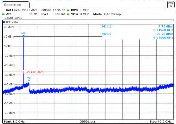
11AC20-CDD-Ant2-5720-1000~40000-PASS
