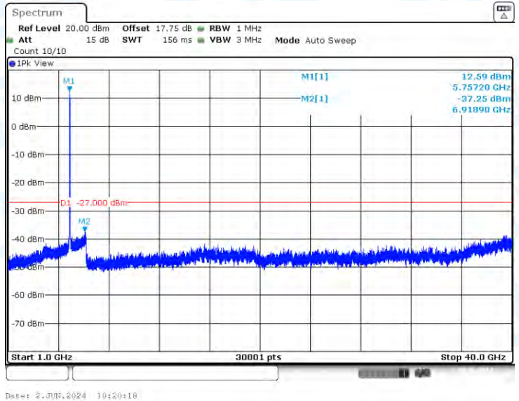
11AC40-CDD-Ant2-5755-1000~40000-PASS
