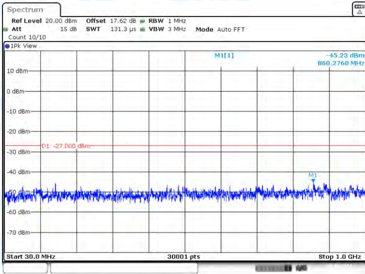
11AC80-CDD-Ant1-5530-30~1000-PASS
