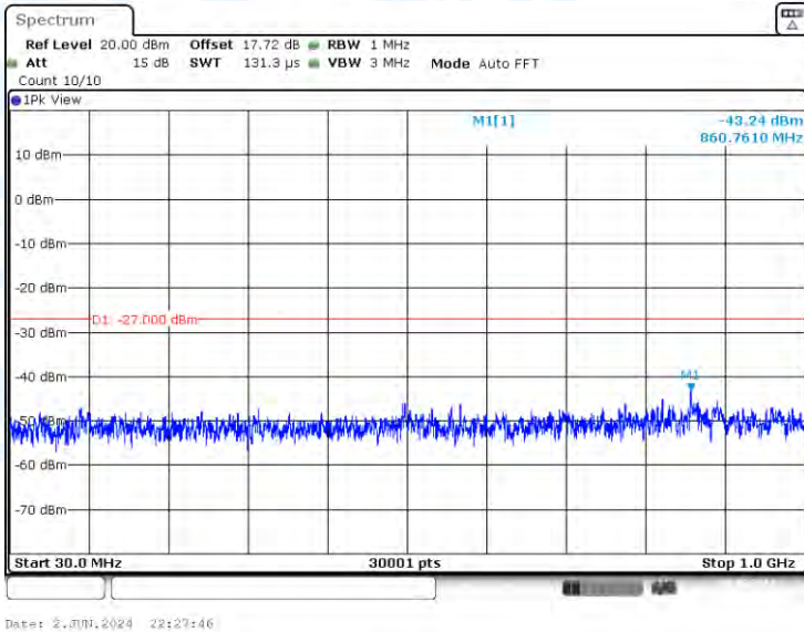
11AC20-CDD-Ant3-5580-30~1000-PASS
