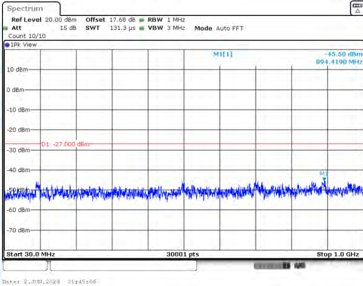
11N40-CDD-Ant3-5510-30~1000-PASS
