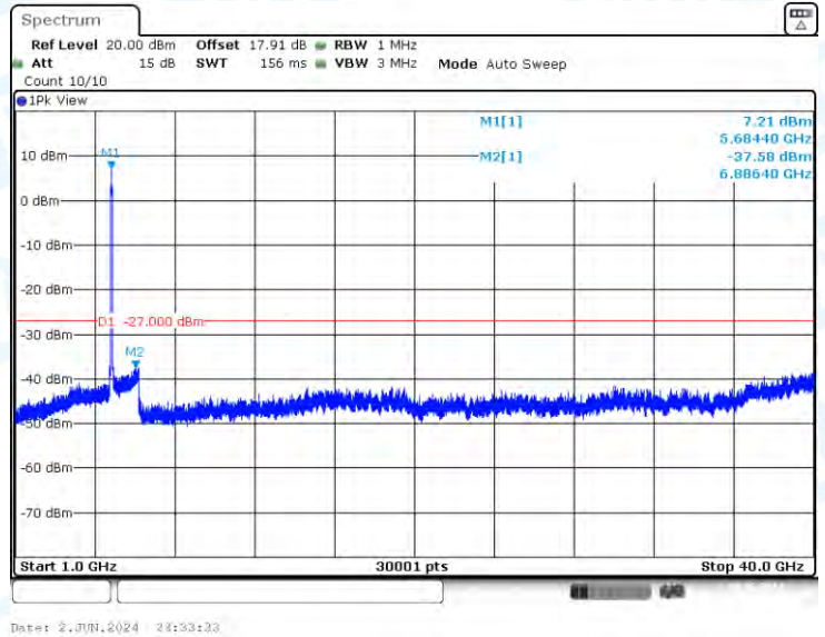
11AC80-CDD-Ant2-5690-1000~40000-PASS
