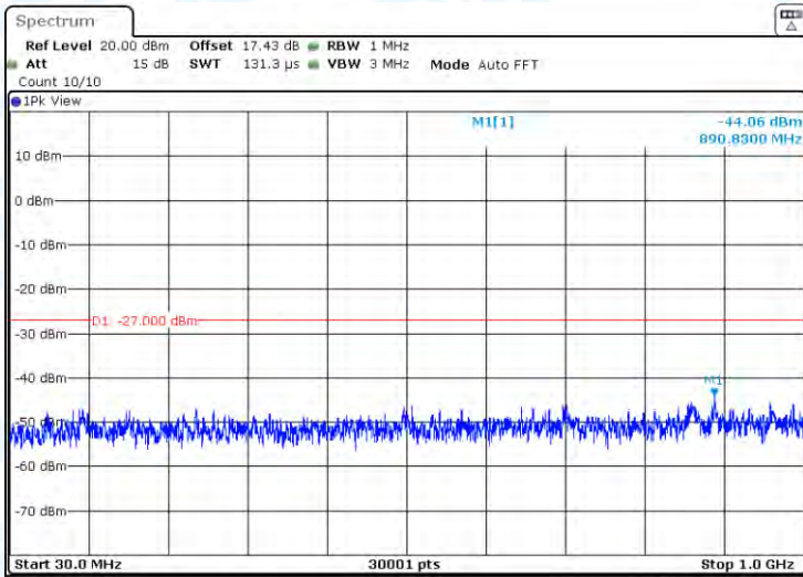
11AC20-CDD-Ant3-5280-30~1000-PASS
