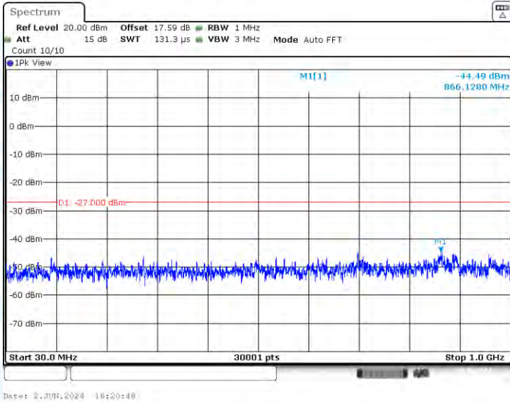
11AC40-CDD-Ant3-5310-30~1000-PASS
