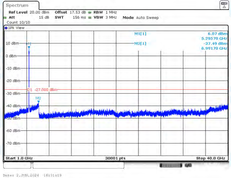
11AC80-CDD-Ant2-5290-1000~40000-PASS
