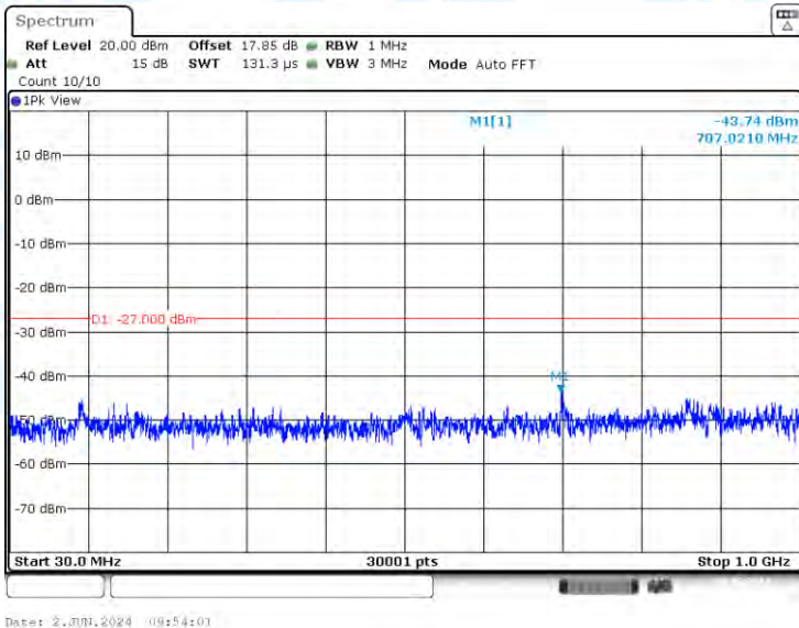
11AC20-CDD-Ant2-5745-30~1000-PASS
