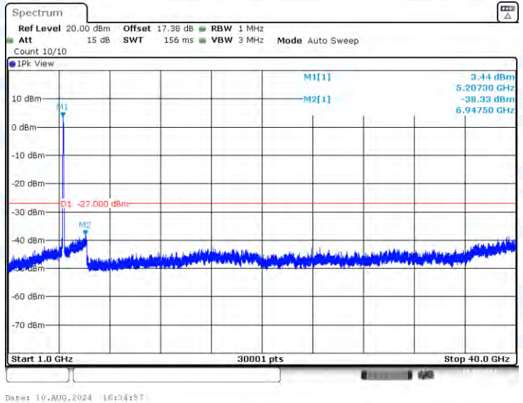
11AC80-CDD-Ant1-5210-1000~40000-PASS
