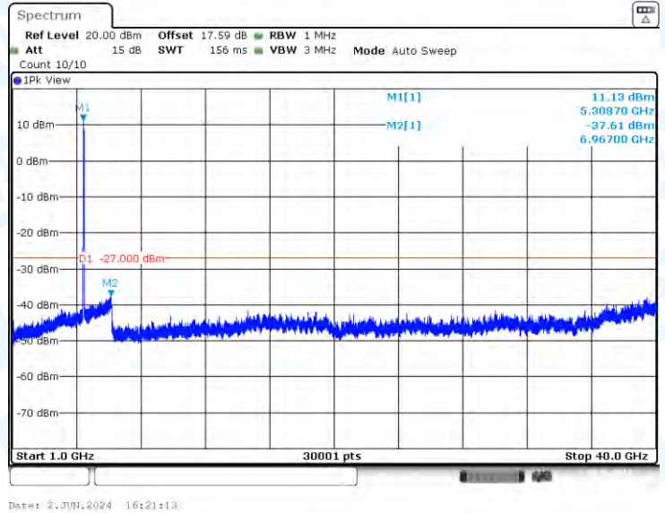
11AC40-CDD-Ant3-5310-1000~40000-PASS
