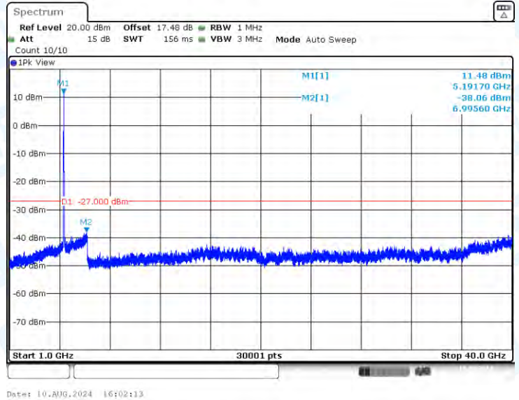
11AC40-CDD-Ant2-5190-1000~40000-PASS
