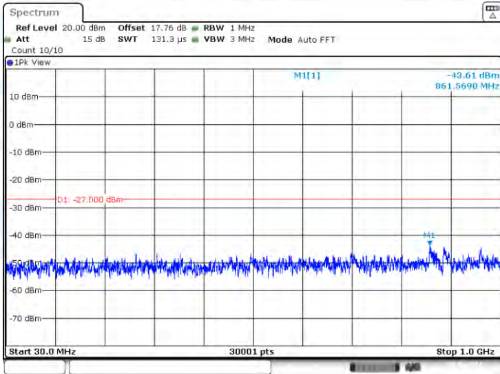
11AC20-CDD-Ant1-5785-30~1000-PASS
