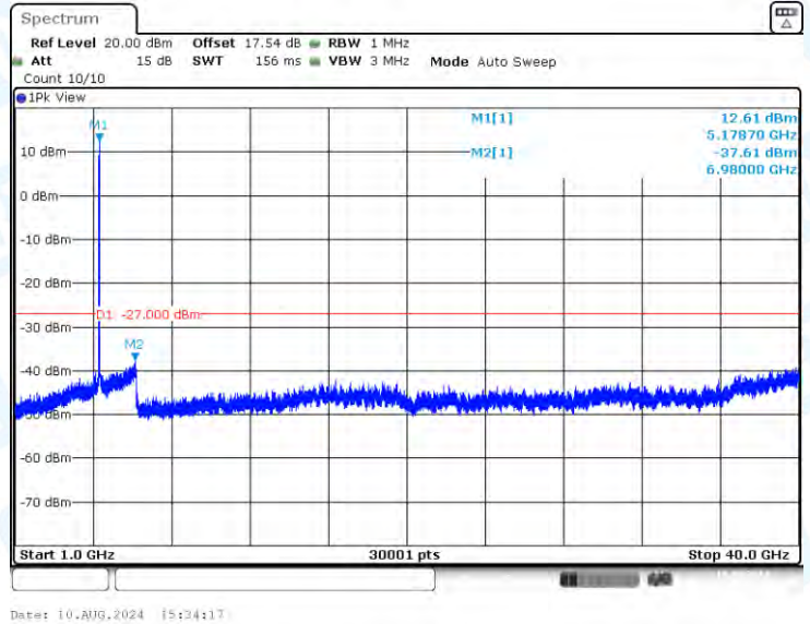
11AC20-CDD-Ant3-5180-1000~40000-PASS
