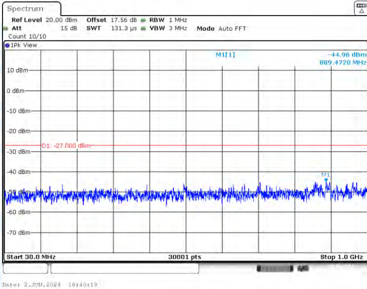
11AC160-CDD-Ant2-5250-30~1000-PASS
