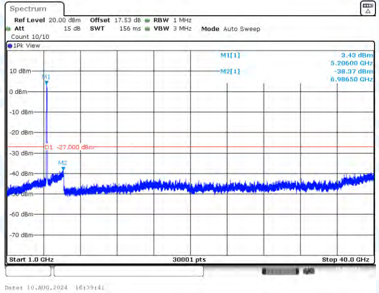
11AC80-CDD-Ant3-5210-1000~40000-PASS
