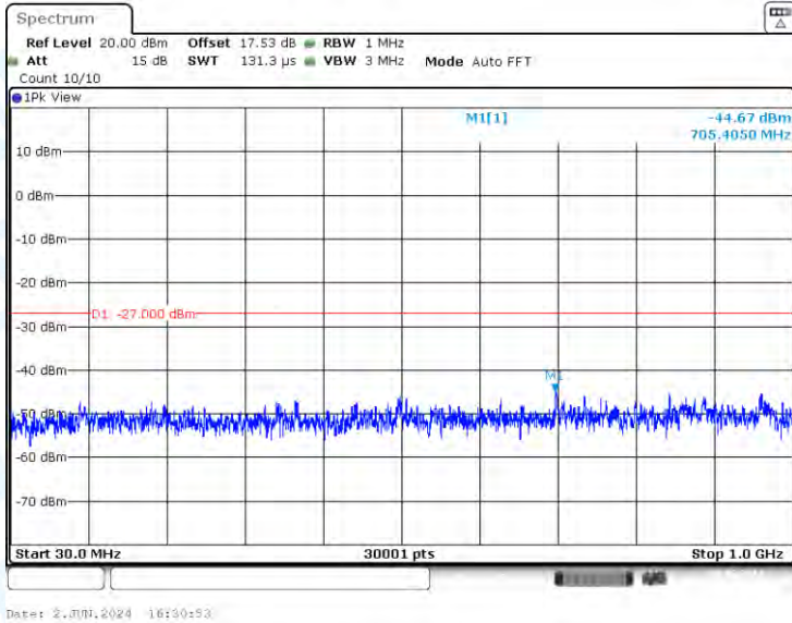
11AC80-CDD-Ant2-5290-30~1000-PASS
