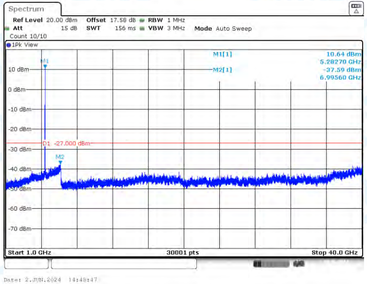
11N20-CDD-Ant3-5280-1000~40000-PASS
