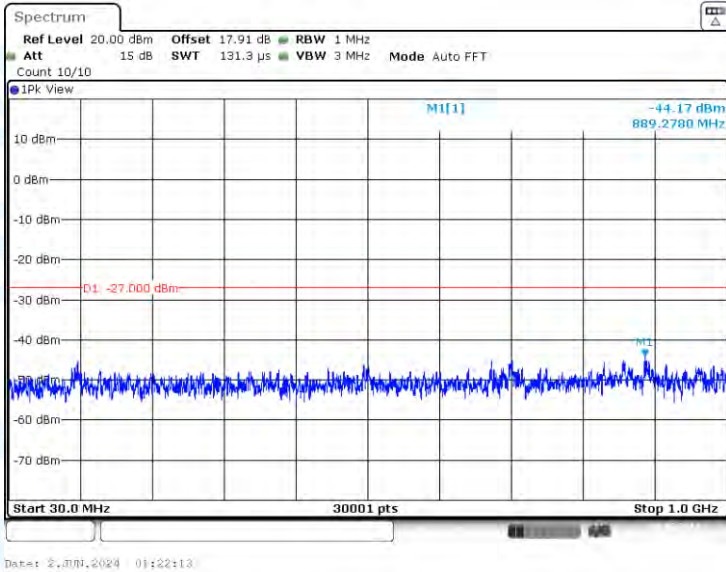
11N20-CDD-Ant3-5825-30~1000-PASS
