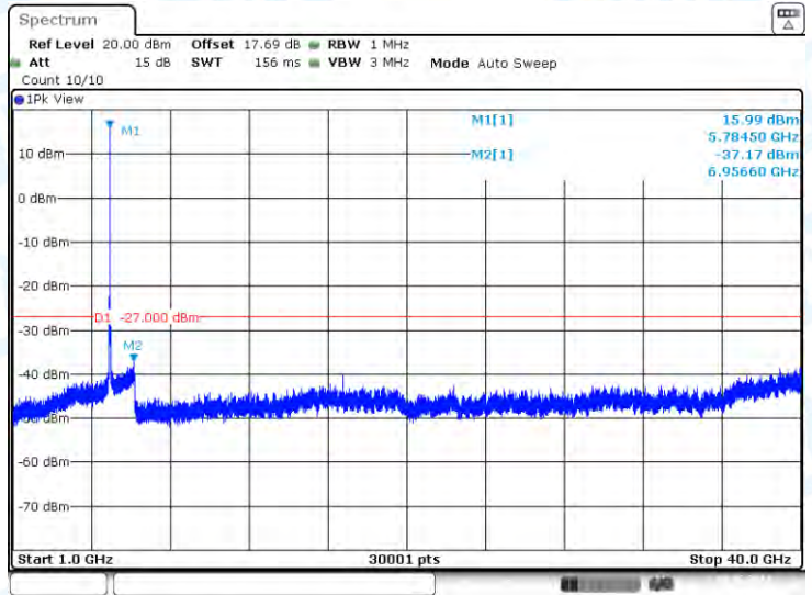
11A-CDD-Ant3-5745-1000~40000-PASS
