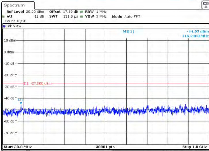
11A-Ant3-5500-30~1000-PASS
