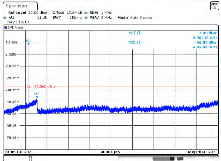
11N20-CDD-Ant1-5500-1000~40000-PASS
