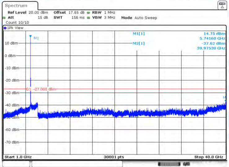
11N20-CDD-Ant2-5745-1000~40000-PASS
