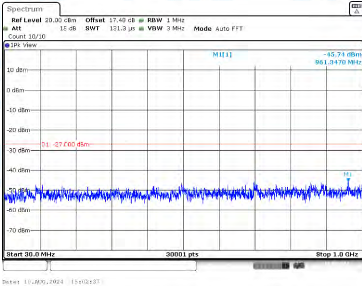
11N20-CDD-Ant2-5200-30~1000-PASS
