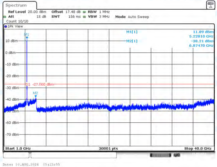
11N40-CDD-Ant1-5230-1000~40000-PASS
