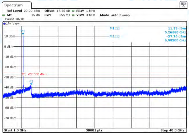
11N40-CDD-Ant2-5270-1000~40000-PASS
