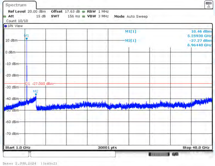
11A-CDD-Ant3-5260-1000~40000-PASS
