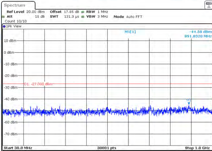
11N20-CDD-Ant1-5825-30~1000-PASS
