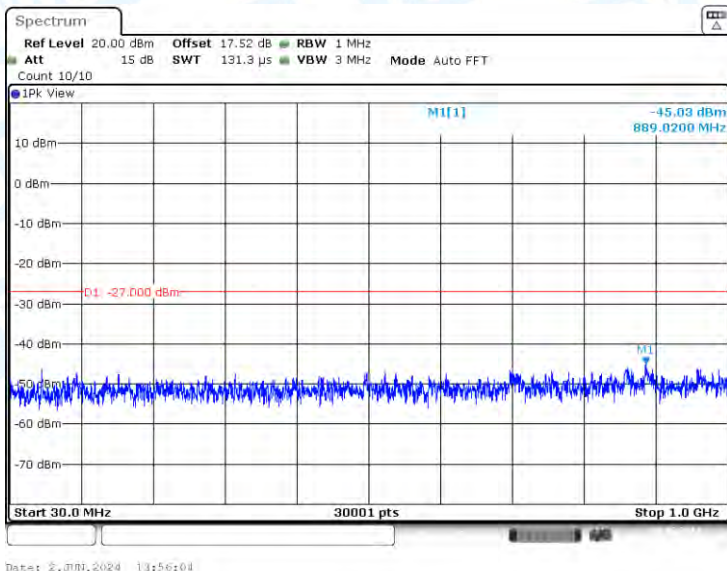
11A-CDD-Ant1-5280-30~1000-PASS
