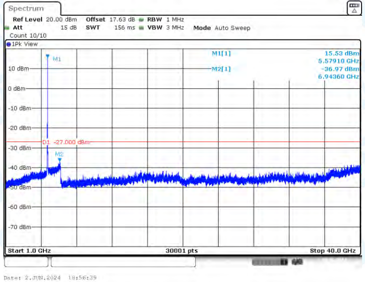
11A-Ant2-5580-1000~40000-PASS
