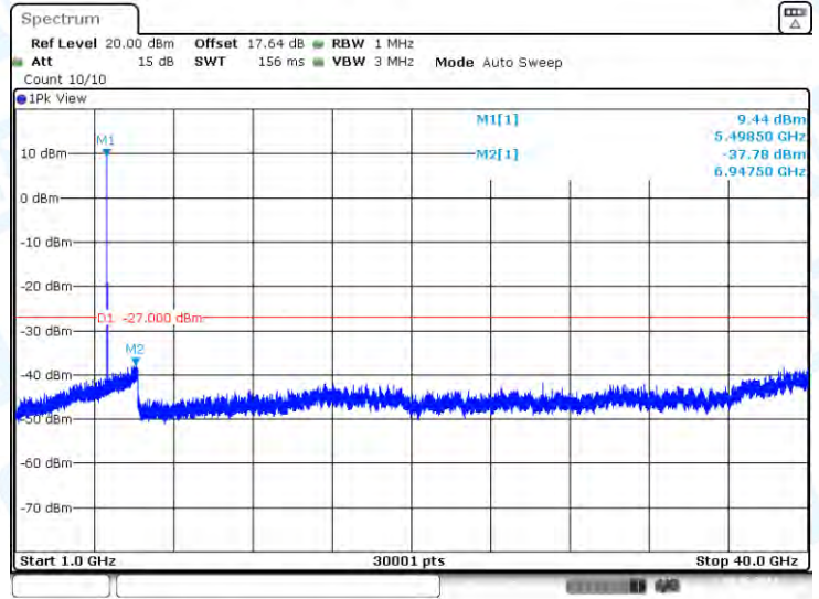
11A-CDD-Ant1-5500-1000~40000-PASS
