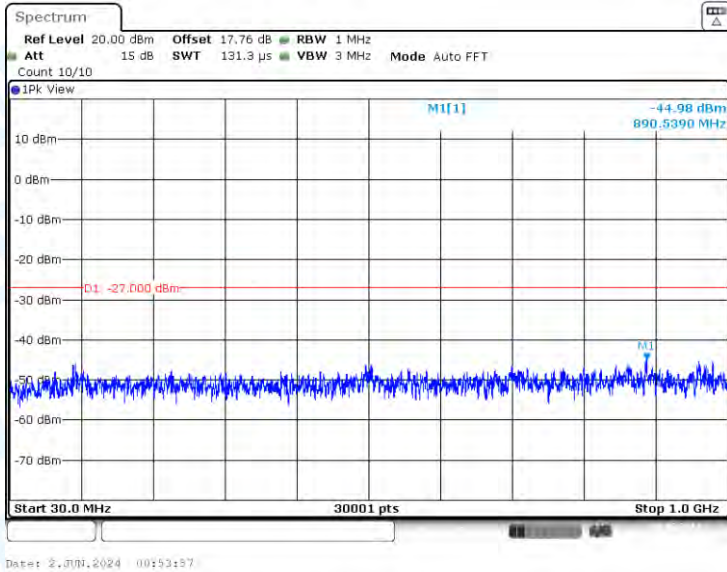
11A-CDD-Ant2-5785-30~1000-PASS
