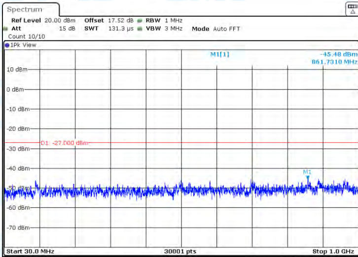
11N40-CDD-Ant1-5270-30~1000-PASS
