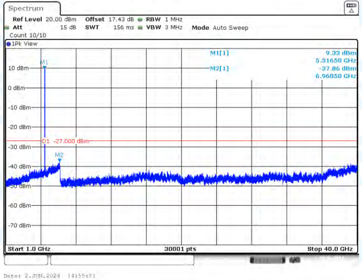
11N20-CDD-Ant1-5320-1000~40000-PASS
