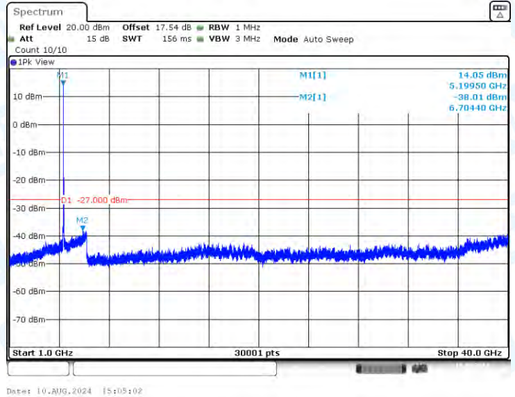
11N20-CDD-Ant3-5200-1000~40000-PASS
