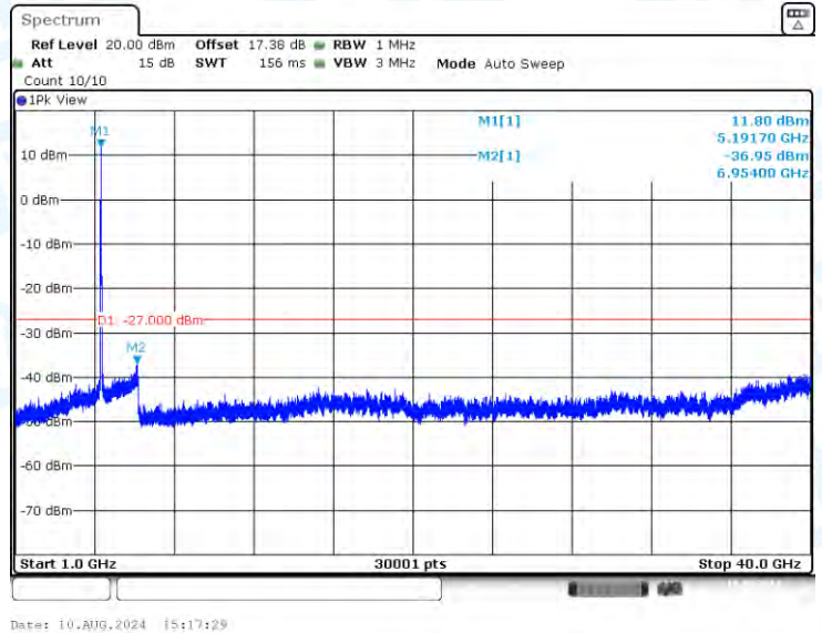
11N40-CDD-Ant1-5190-1000~40000-PASS
