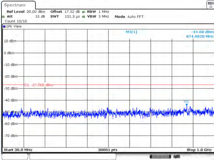
11N20-CDD-Ant1-5280-30~1000-PASS
