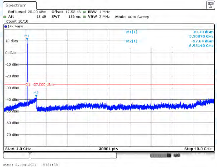
11N40-CDD-Ant2-5310-1000~40000-PASS
