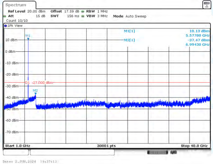
11A-CDD-Ant1-5580-1000~40000-PASS
