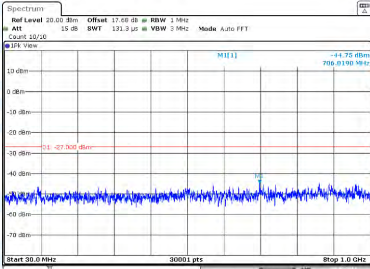
11A-Ant2-5500-30~1000-PASS
