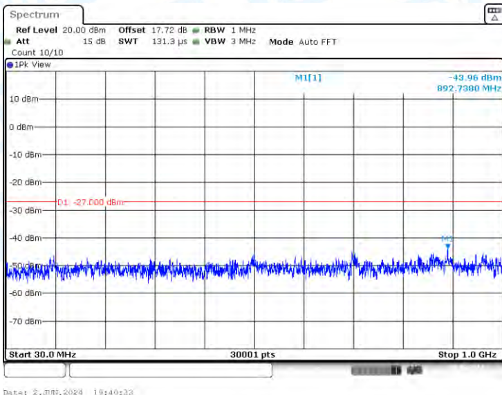
11A-CDD-Ant2-5580-30~1000-PASS
