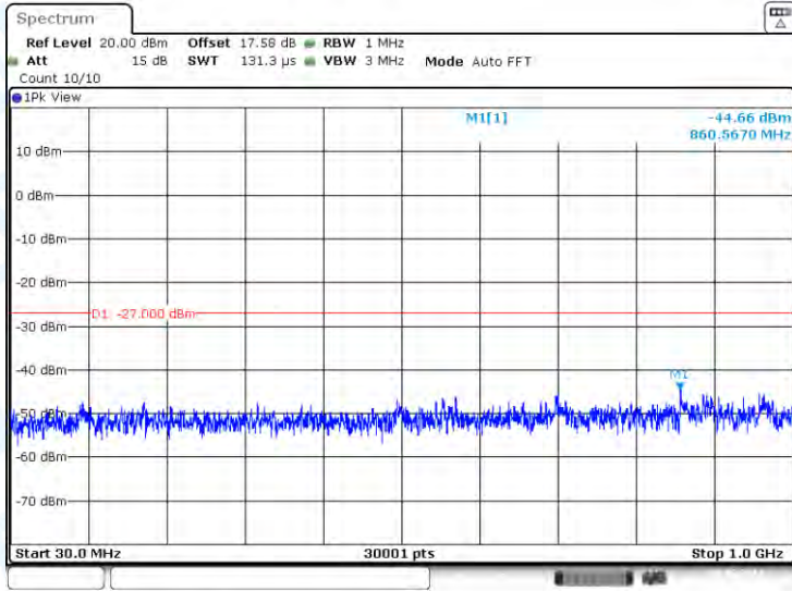
11A-CDD-Ant2-5280-30~1000-PASS
