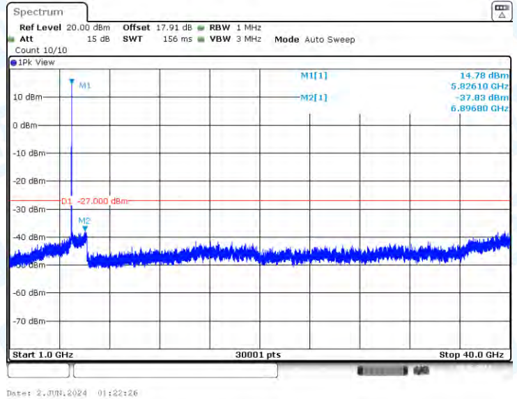
11N20-CDD-Ant3-5825-1000~40000-PASS
