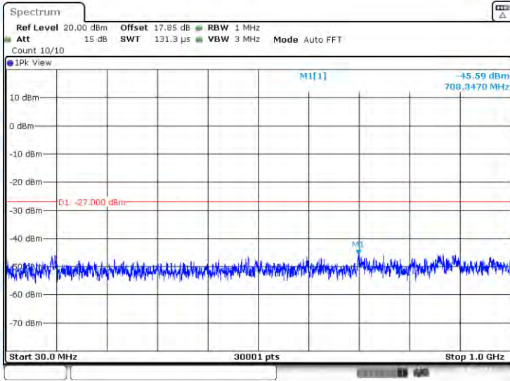
11A-Ant1-5720-30~1000-PASS
