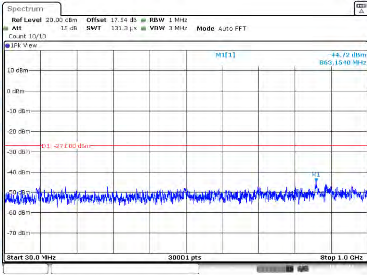
11N40-CDD-Ant2-5190-30~1000-PASS
