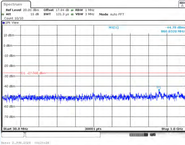
11A-Ant3-5785-30~1000-PASS
