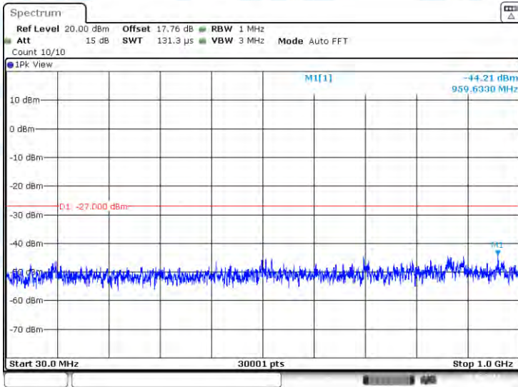
11A-Ant1-5785-30~1000-PASS
