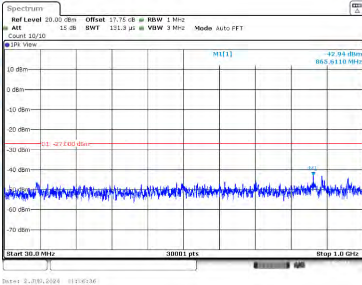
11N20-CDD-Ant3-5720-30~1000-PASS
