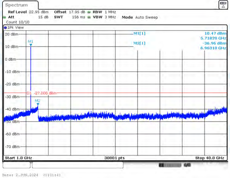
11N20-CDD-Ant3-5720-1000~40000-PASS
