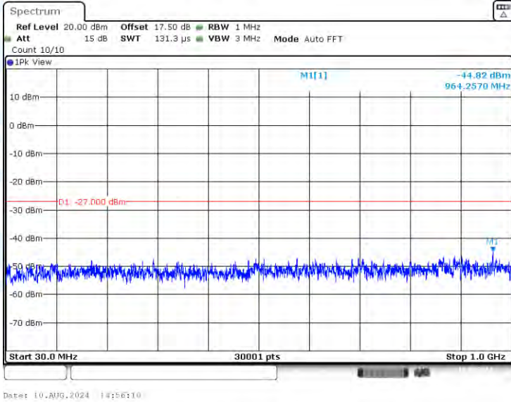
11N20-CDD-Ant2-5180-30~1000-PASS
