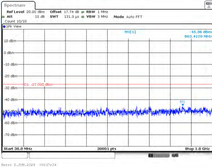
11A-Ant1-5825-30~1000-PASS
