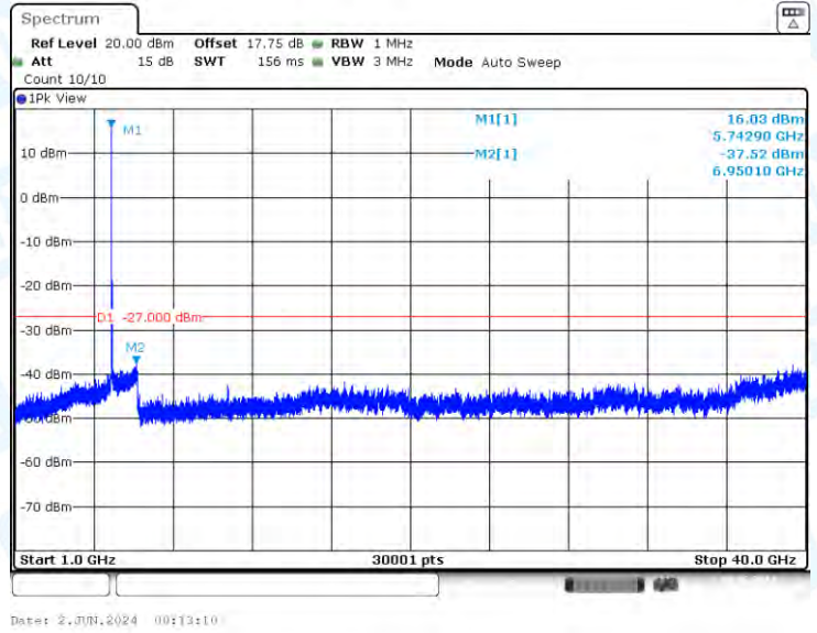
11A-Ant1-5745-1000~40000-PASS
