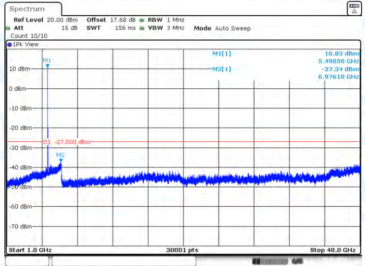
11A-CDD-Ant2-5500-1000~40000-PASS
