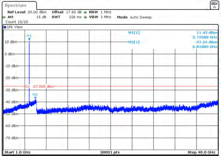
11A-CDD-Ant1-5720-1000~40000-PASS
