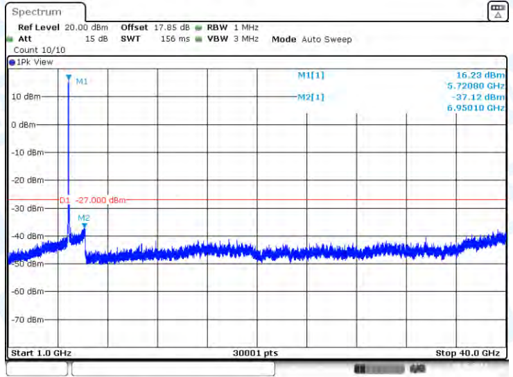
11A-Ant1-5720-1000~40000-PASS
