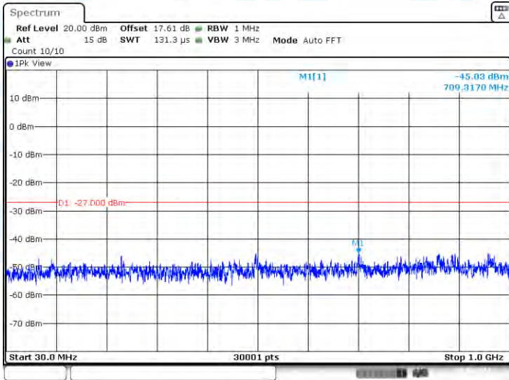
11N40-CDD-Ant1-5510-30~1000-PASS
