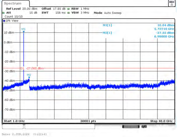
11N20-CDD-Ant2-5720-1000~40000-PASS
