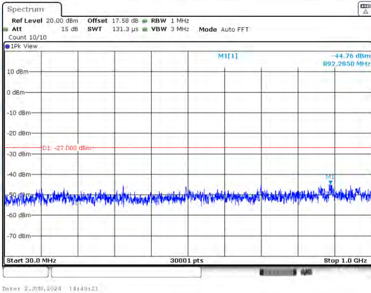
11N20-CDD-Ant3-5280-30~1000-PASS
