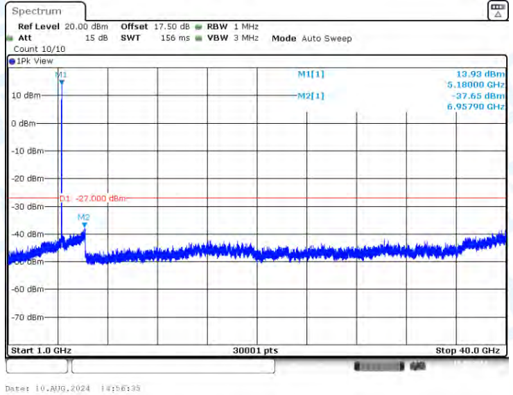
11N20-CDD-Ant2-5180-1000~40000-PASS
