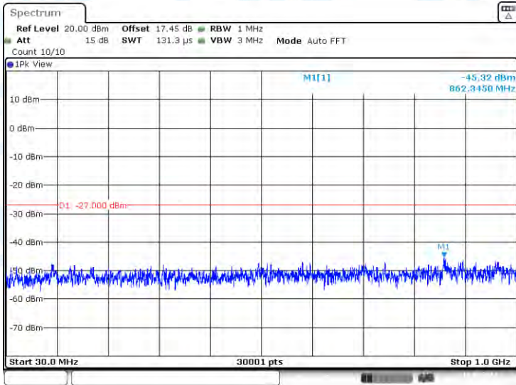
11A-Ant3-5825-30~1000-PASS
