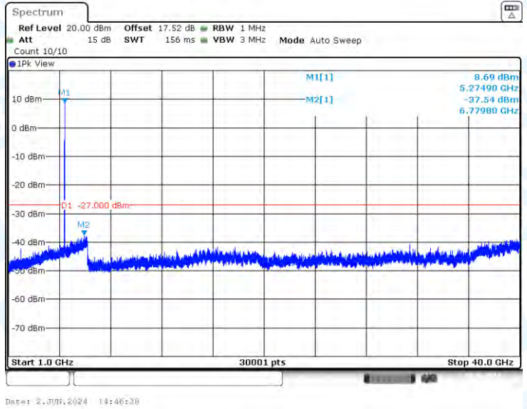
11N20-CDD-Ant2-5280-1000~40000-PASS
