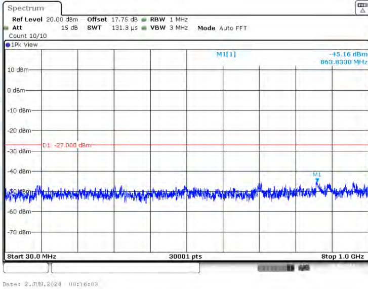
11A-Ant2-5745-30~1000-PASS
