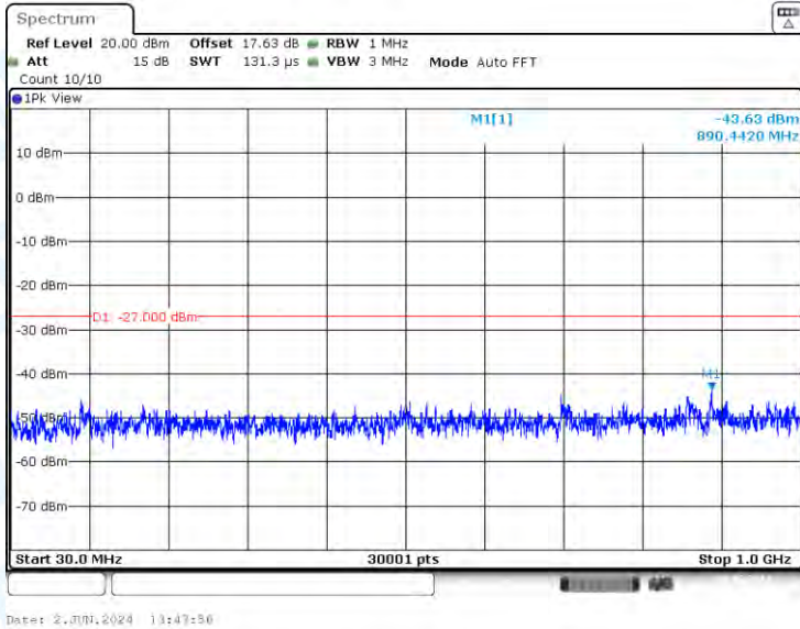
11A-CDD-Ant3-5260-30~1000-PASS
