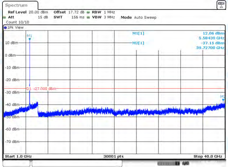
11N20-CDD-Ant2-5580-1000~40000-PASS
