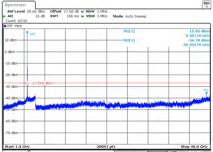
11A-Ant2-5500-1000~40000-PASS
