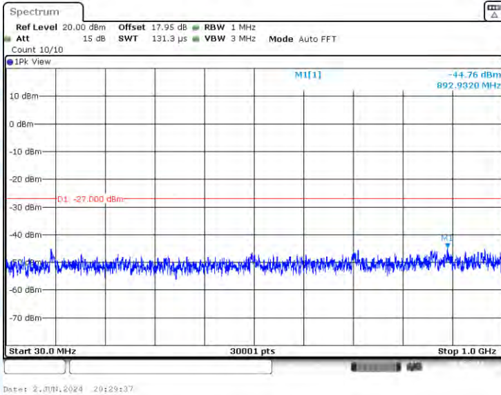
11A-CDD-Ant3-5720-30~1000-PASS
