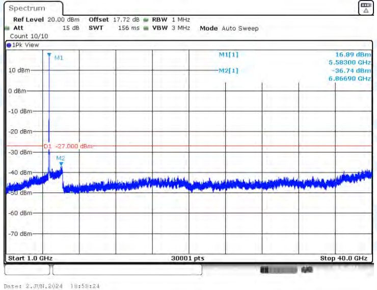
11A-Ant3-5580-1000~40000-PASS
