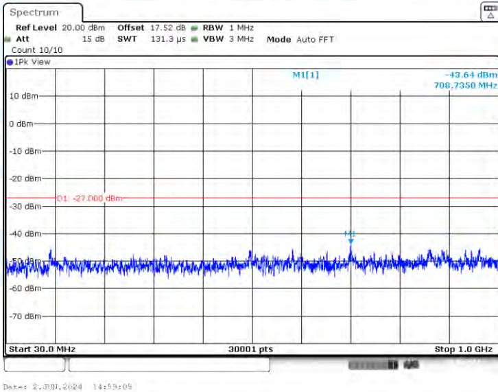
11N20-CDD-Ant2-5320-30~1000-PASS
