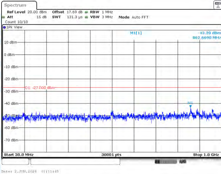
11N20-CDD-Ant1-5785-30~1000-PASS
