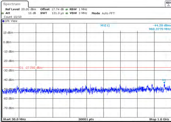
11N20-CDD-Ant3-5785-30~1000-PASS
