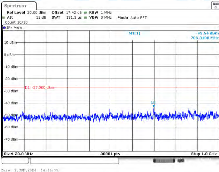
11N20-CDD-Ant3-5260-30~1000-PASS
