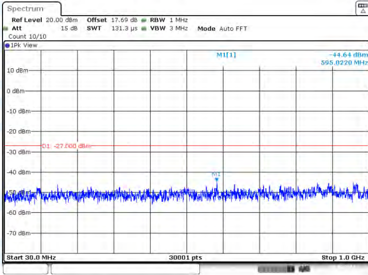
11A-Ant3-5745-30~1000-PASS
