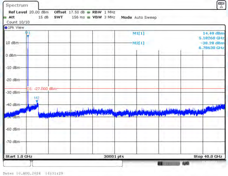
11A-CDD-Ant2-5180-1000~40000-PASS
