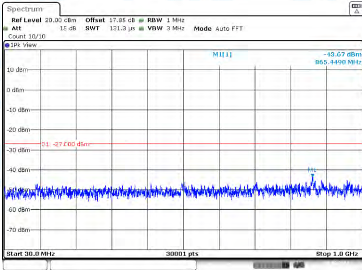
11N20-CDD-Ant2-5745-30~1000-PASS
