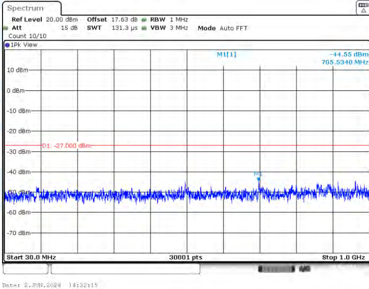
11N20-CDD-Ant3-5260-30~1000-PASS
