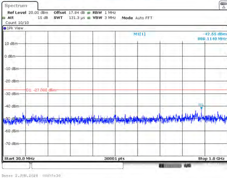
11A-CDD-Ant3-5785-30~1000-PASS
