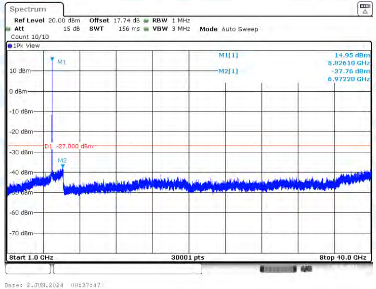
11A-Ant1-5825-1000~40000-PASS
