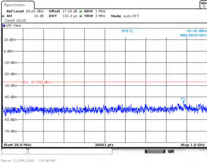
11A-CDD-Ant1-5580-30~1000-PASS
