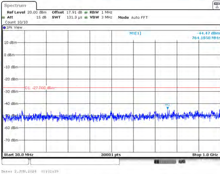
11A-CDD-Ant3-5825-30~1000-PASS
