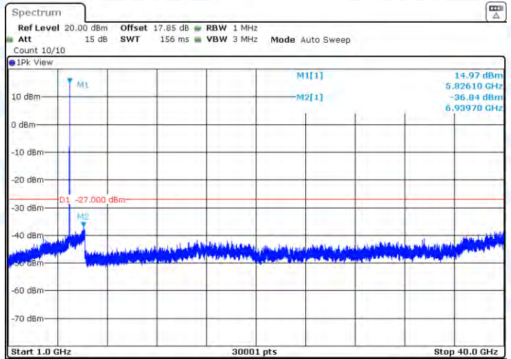
11N20-CDD-Ant1-5825-1000~40000-PASS
