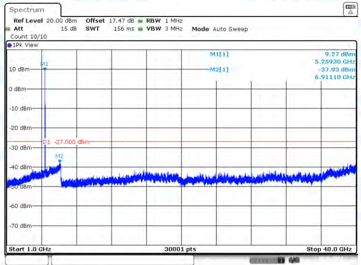
11N20-CDD-Ant3-5240-1000~40000-PASS
