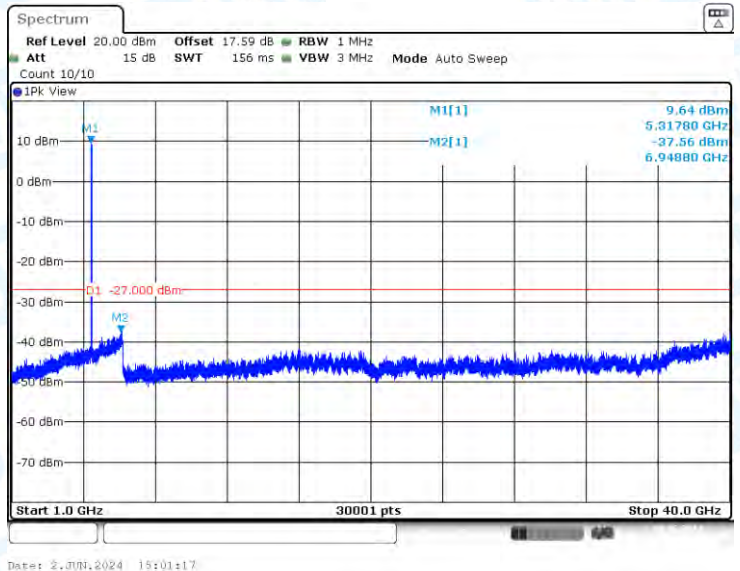
11N20-CDD-Ant2-5320-1000~40000-PASS
