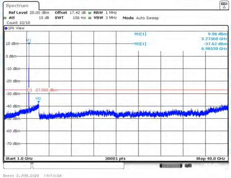
11A-CDD-Ant1-5280-1000~40000-PASS
