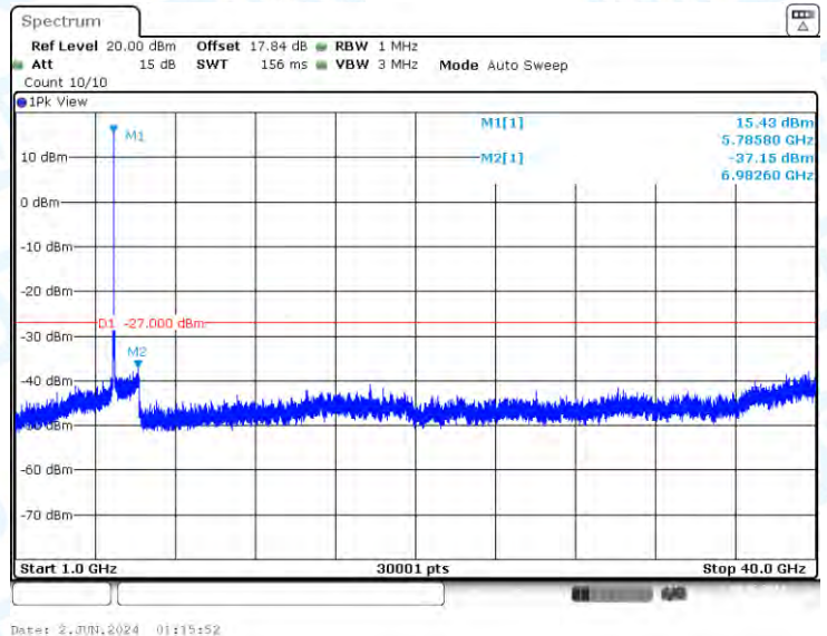
11N20-CDD-Ant2-5785-1000~40000-PASS
