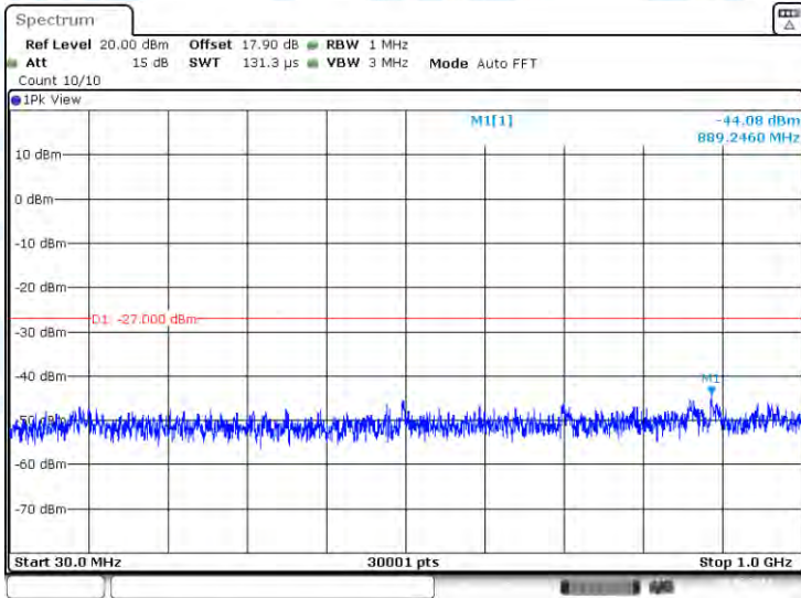
11N20-CDD-Ant3-5580-30~1000-PASS
