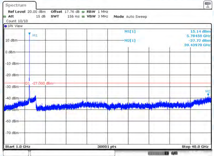
11A-Ant1-5785-1000~40000-PASS
