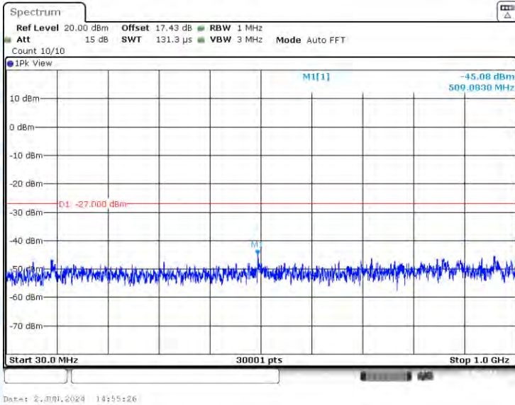
11N20-CDD-Ant1-5320-30~1000-PASS
