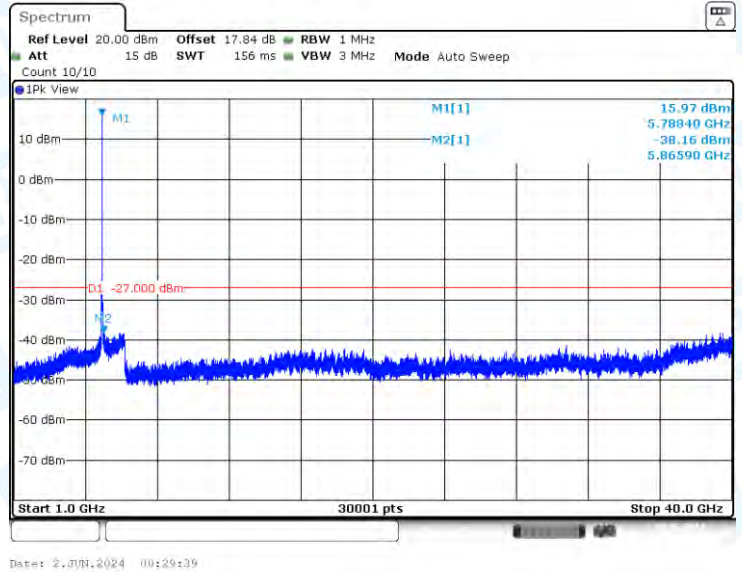
11A-Ant3-5785-1000~40000-PASS
