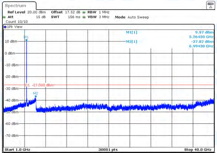
11N40-CDD-Ant1-5270-1000~40000-PASS
