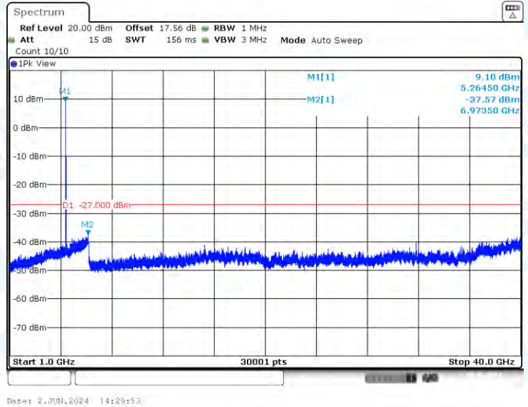
11N20-CDD-Ant2-5260-1000~40000-PASS
