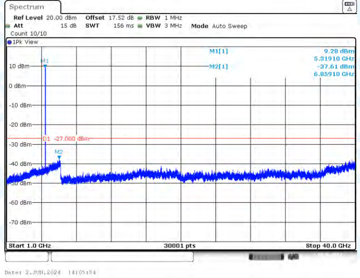
11A-CDD-Ant2-5320-1000~40000-PASS
