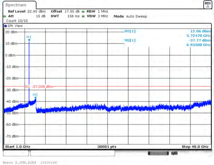
11A-CDD-Ant3-5720-1000~40000-PASS
