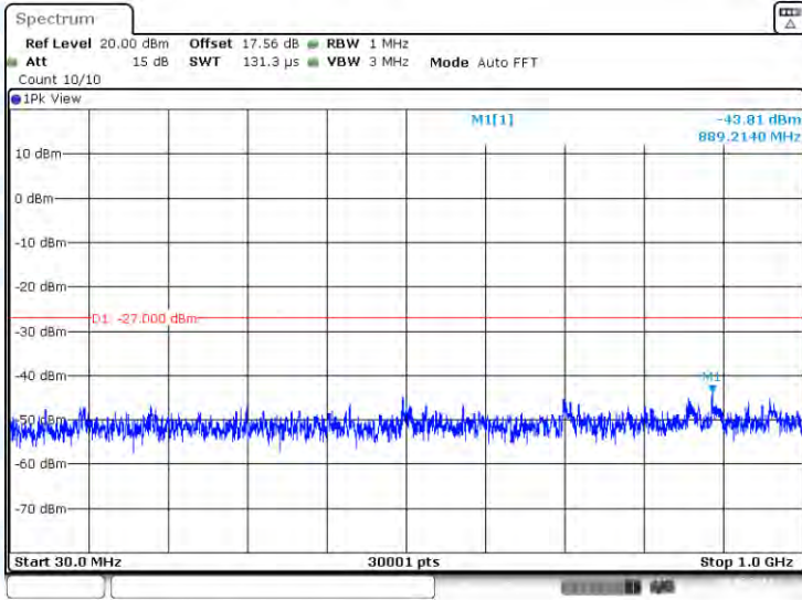
11N20-CDD-Ant3-5320-30~1000-PASS
