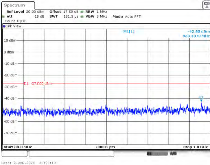
11N20-CDD-Ant1-5580-30~1000-PASS
