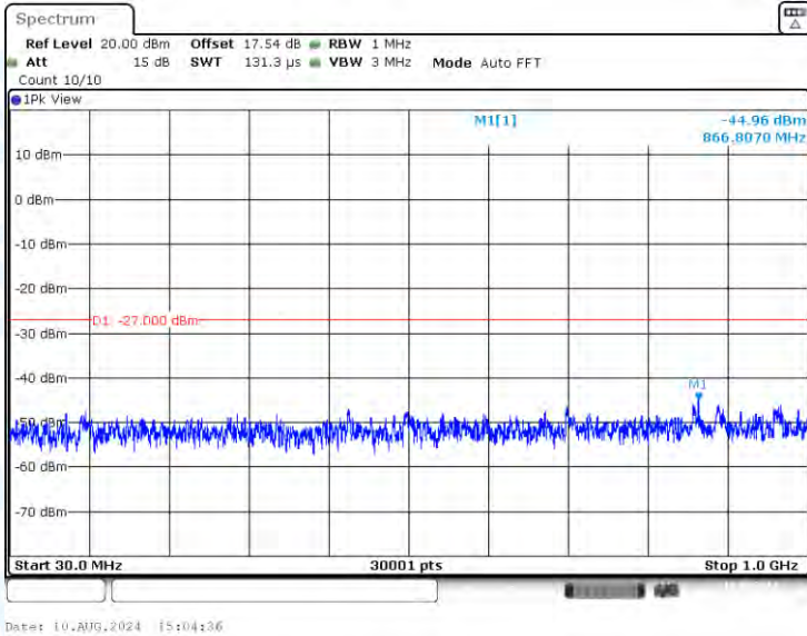
11N20-CDD-Ant3-5200-30~1000-PASS
