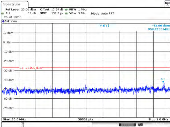
11A-CDD-Ant3-5745-30~1000-PASS
