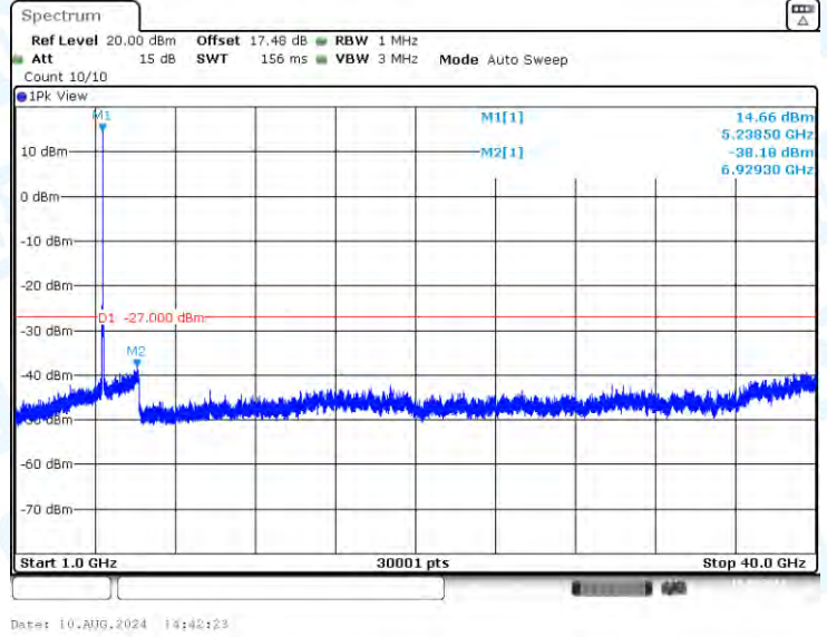
11A-CDD-Ant1-5240-1000~40000-PASS
