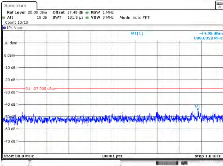
11N40-CDD-Ant3-5190-30~1000-PASS
