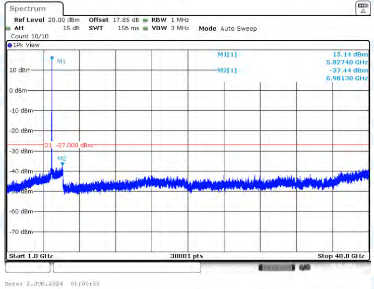
11A-CDD-Ant2-5825-1000~40000-PASS
