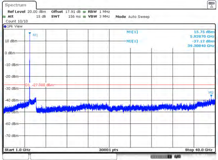
11A-Ant2-5825-1000~40000-PASS
