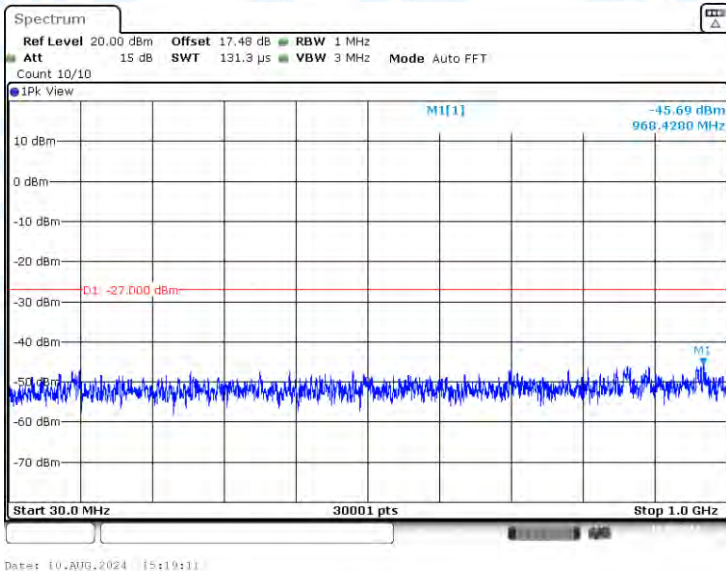
11N40-CDD-Ant1-5190-30~1000-PASS
