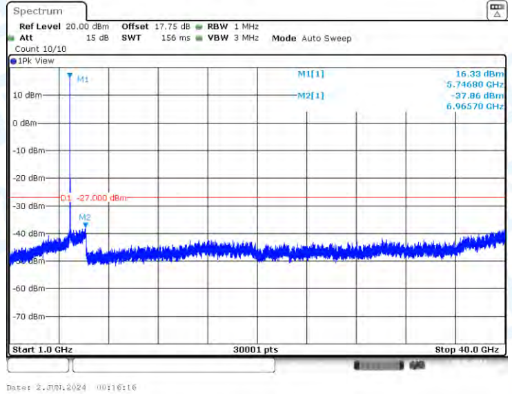
11A-Ant2-5745-1000~40000-PASS
