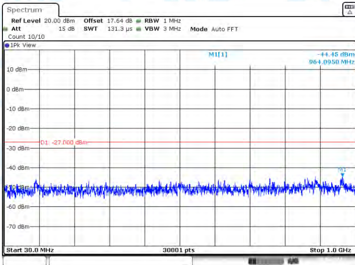
11N20-CDD-Ant1-5500-30~1000-PASS
