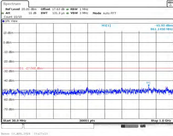
11N40-CDD-Ant3-5230-30~1000-PASS
