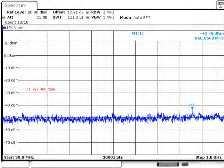
11A-Ant2-5825-30~1000-PASS
