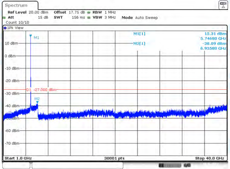
11N20-CDD-Ant1-5745-1000~40000-PASS
