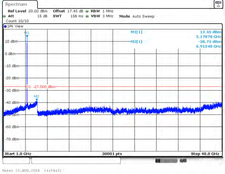
11N20-CDD-Ant1-5180-1000~40000-PASS
