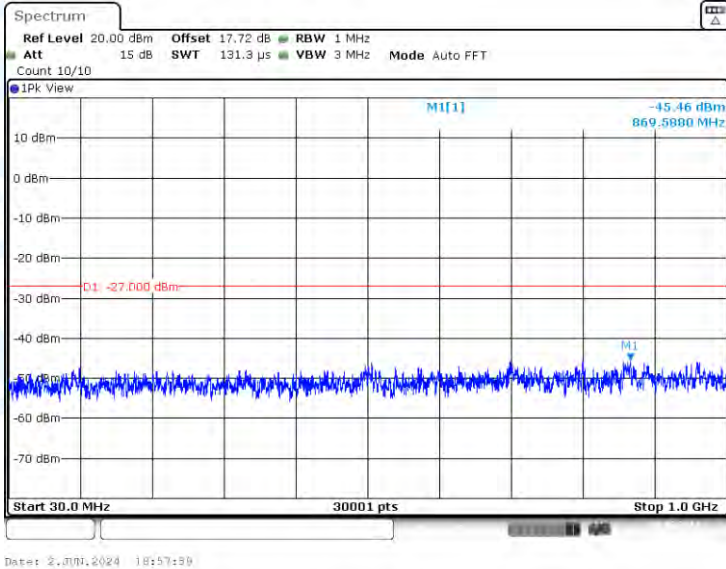
11A-Ant3-5580-30~1000-PASS
