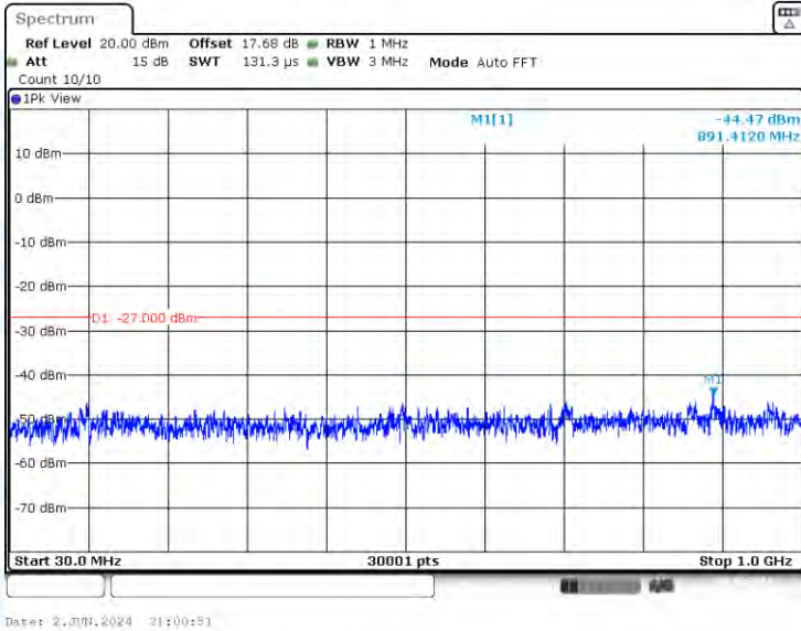
11N20-CDD-Ant3-5500-30~1000-PASS
