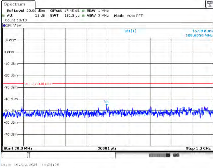
11N20-CDD-Ant1-5180-30~1000-PASS
