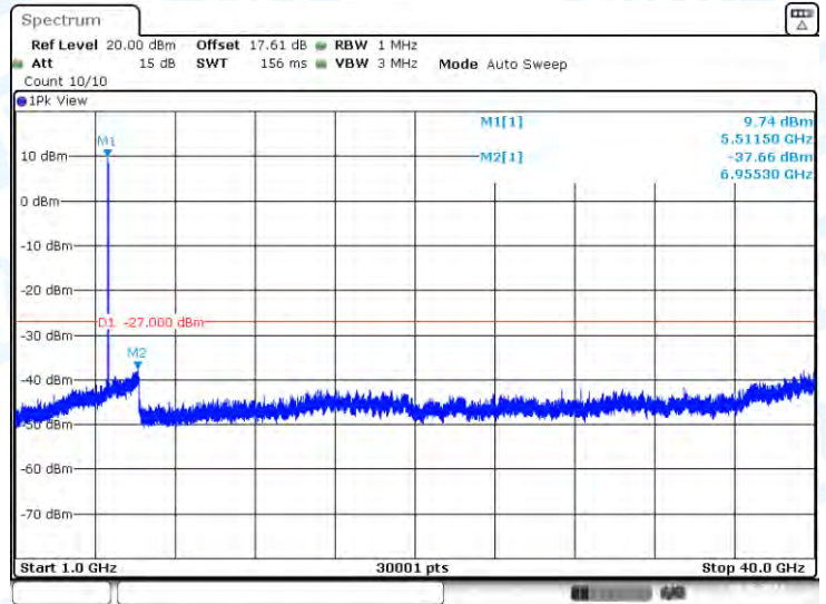
11N40-CDD-Ant1-5510-1000~40000-PASS
