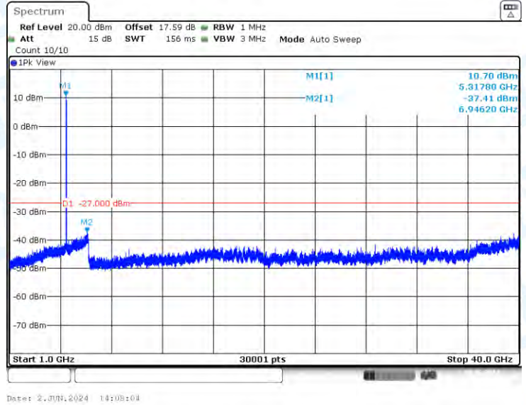
11A-CDD-Ant3-5320-1000~40000-PASS
