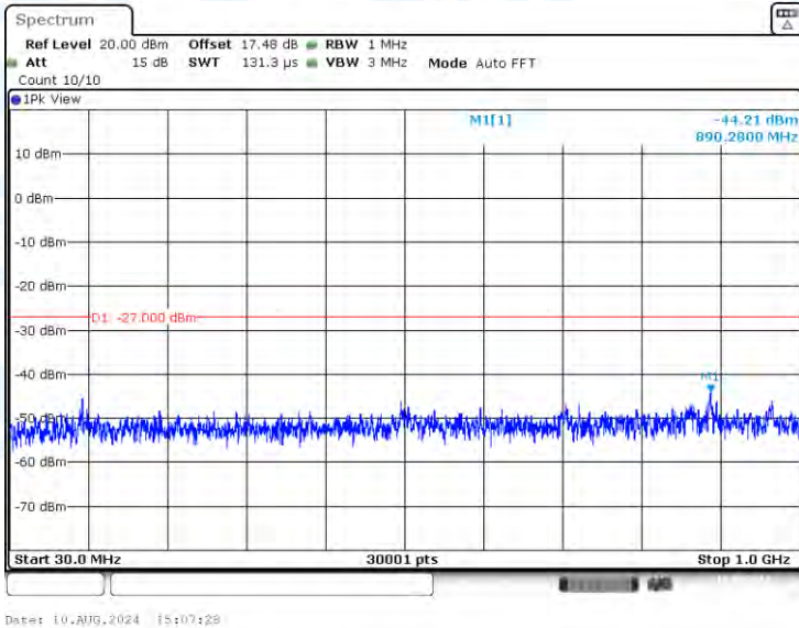
11N20-CDD-Ant1-5240-30~1000-PASS
