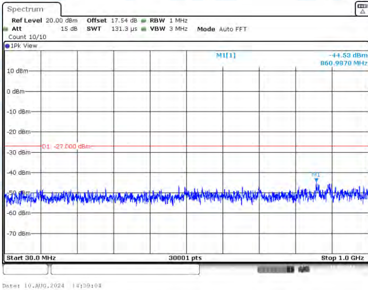
11A-CDD-Ant3-5200-30~1000-PASS
