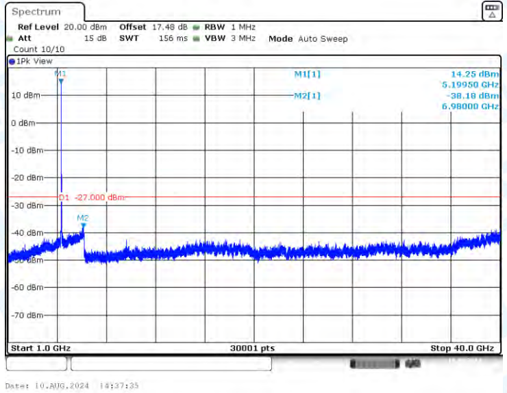
11A-CDD-Ant2-5200-1000~40000-PASS
