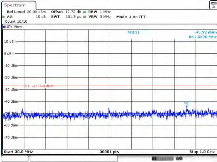
11N20-CDD-Ant2-5580-30~1000-PASS
