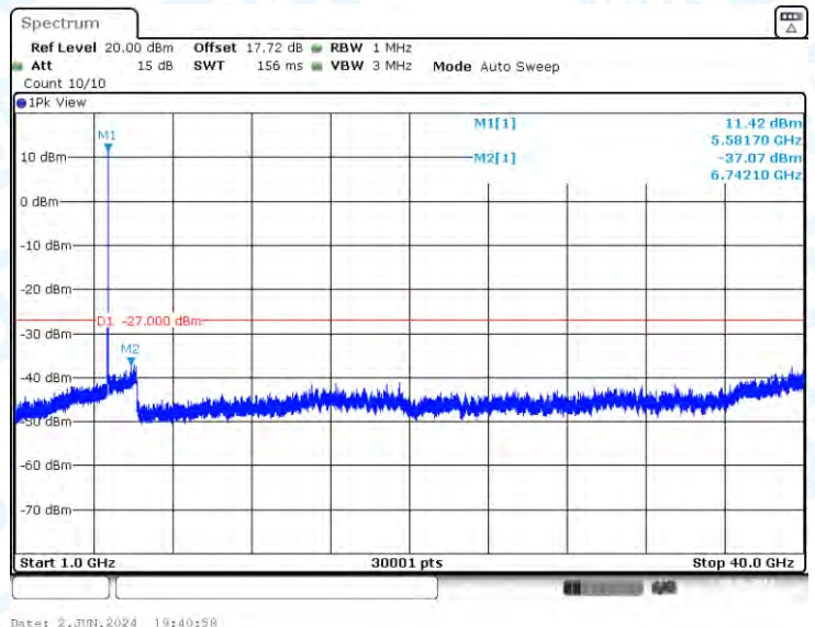
11A-CDD-Ant2-5580-1000~40000-PASS
