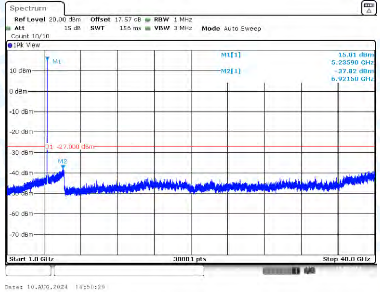
11A-CDD-Ant2-5240-1000~40000-PASS
