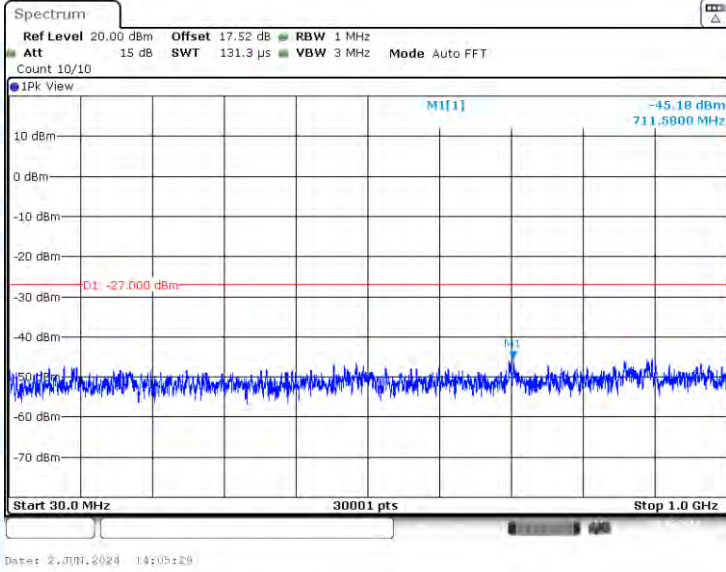
11A-CDD-Ant2-5320-30~1000-PASS
