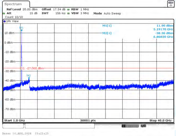
11N40-CDD-Ant3-5190-1000~40000-PASS
