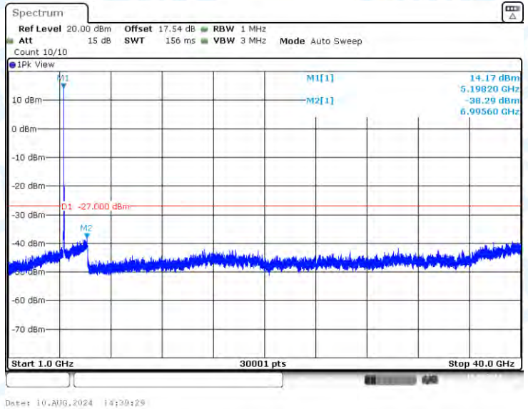
11A-CDD-Ant3-5200-1000~40000-PASS
