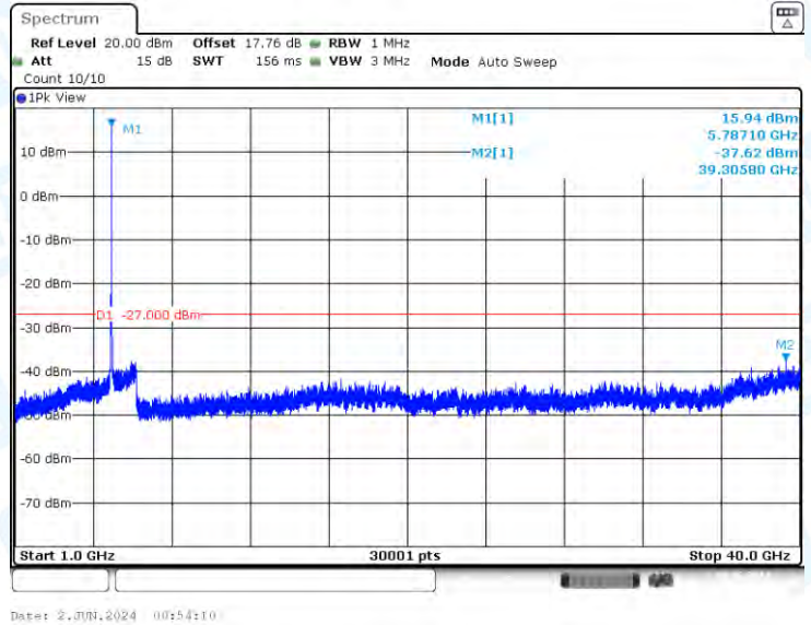
11A-CDD-Ant2-5785-1000~40000-PASS
