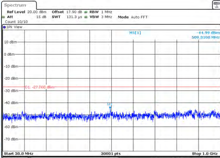
11A-CDD-Ant3-5580-30~1000-PASS
