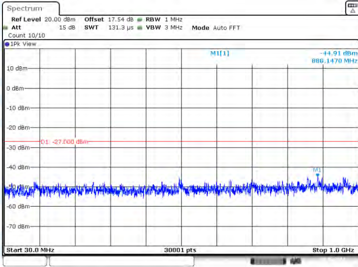
11N40-CDD-Ant3-5310-30~1000-PASS
