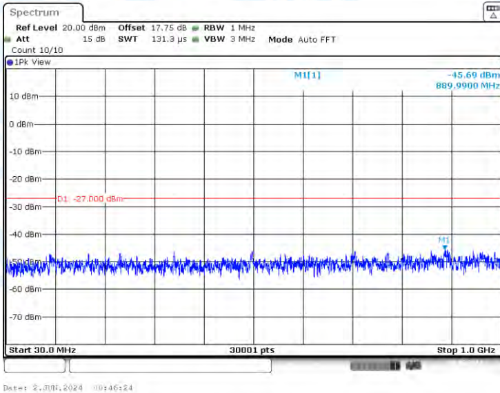
11A-CDD-Ant1-5745-30~1000-PASS
