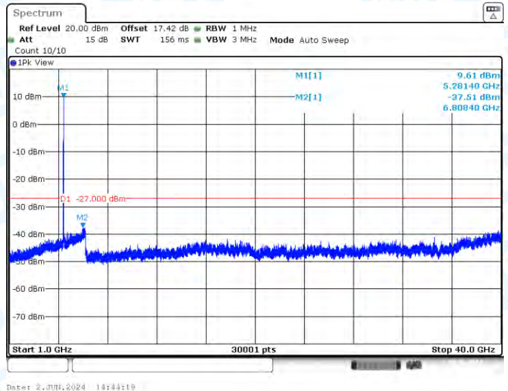
11N20-CDD-Ant3-5260-1000~40000-PASS
