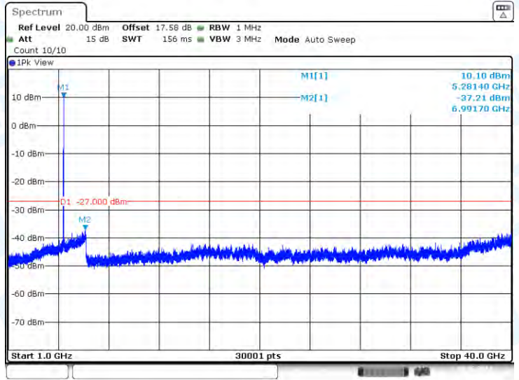
11A-CDD-Ant2-5280-1000~40000-PASS
