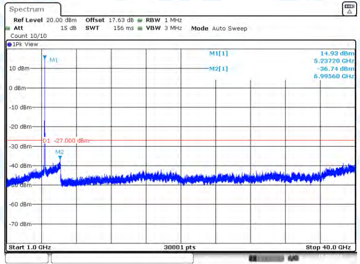
11N20-CDD-Ant2-5240-1000~40000-PASS
