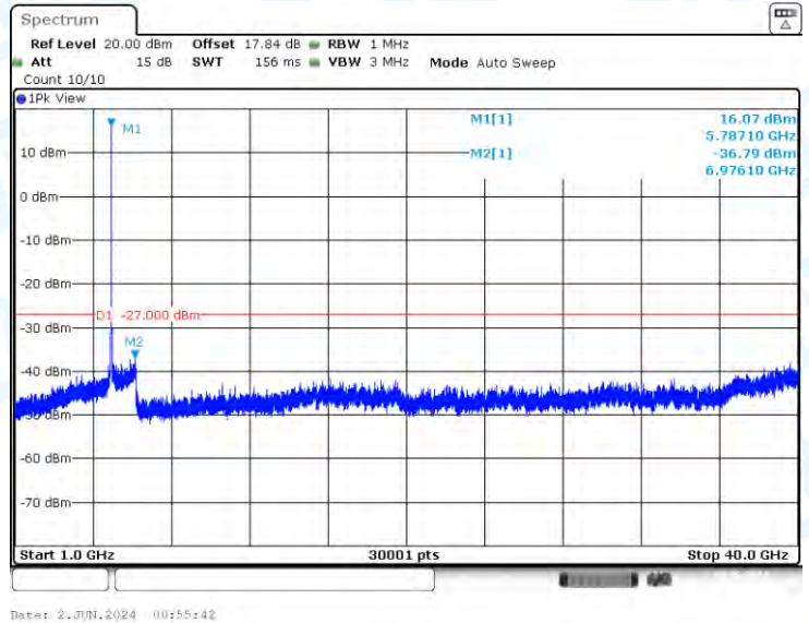
11A-CDD-Ant3-5785-1000~40000-PASS
