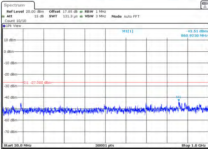
11A-CDD-Ant1-5720-30~1000-PASS
