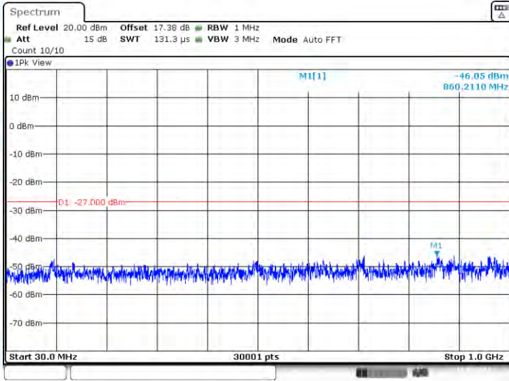
11N20-CDD-Ant3-5180-30~1000-PASS
