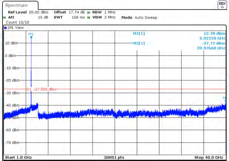
11N20-CDD-Ant3-5785-1000~40000-PASS
