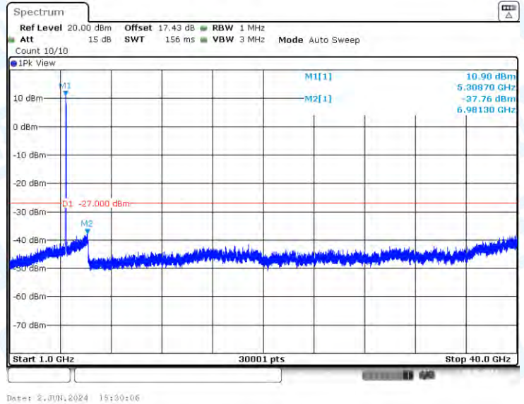
11N40-CDD-Ant1-5310-1000~40000-PASS
