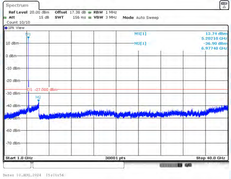
11N20-CDD-Ant1-5200-1000~40000-PASS
