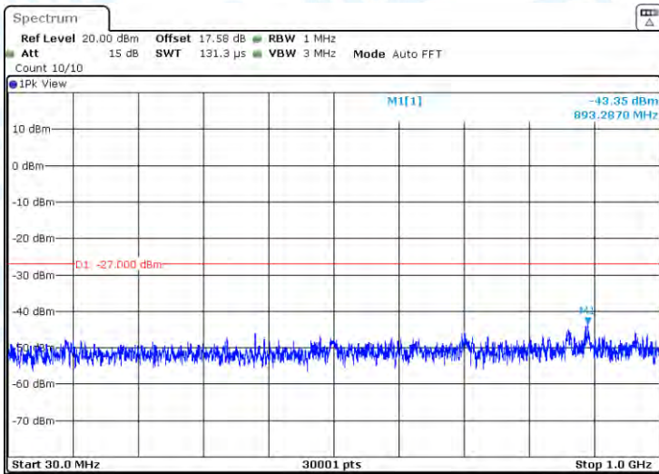
11N40-CDD-Ant2-5270-30~1000-PASS
