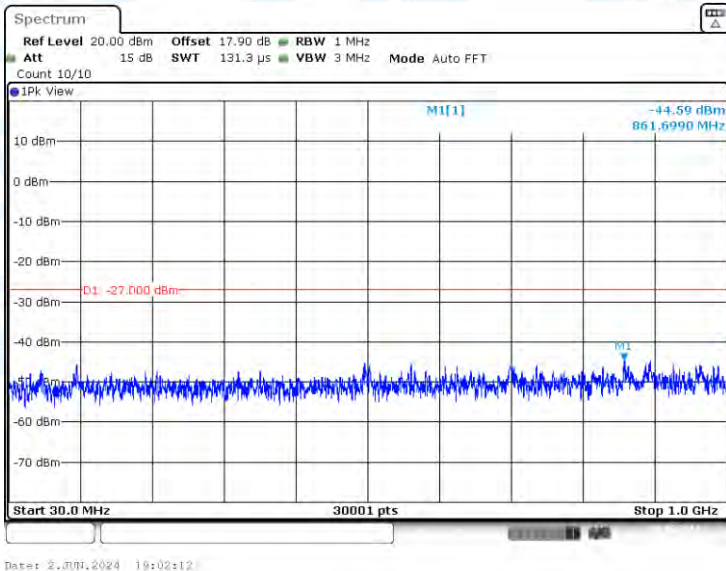
11A-Ant3-5580-30~1000-PASS
