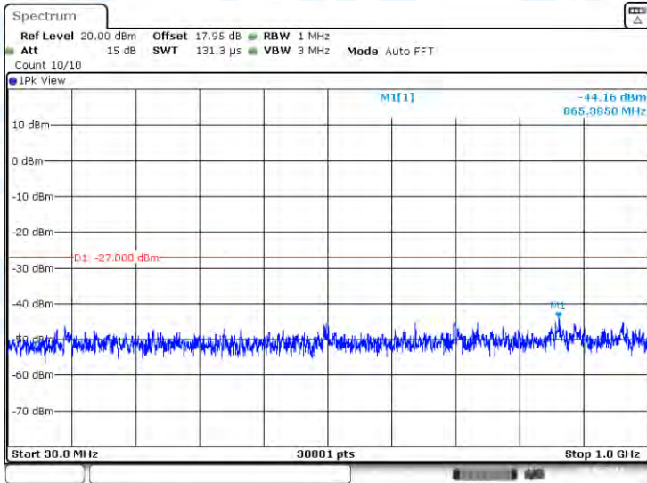
11A-Ant2-5720-30~1000-PASS
