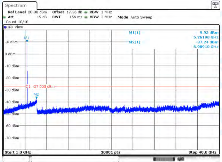
11A-CDD-Ant1-5260-1000~40000-PASS
