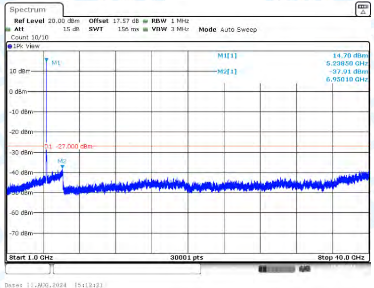
11N20-CDD-Ant1-5240-1000~40000-PASS
