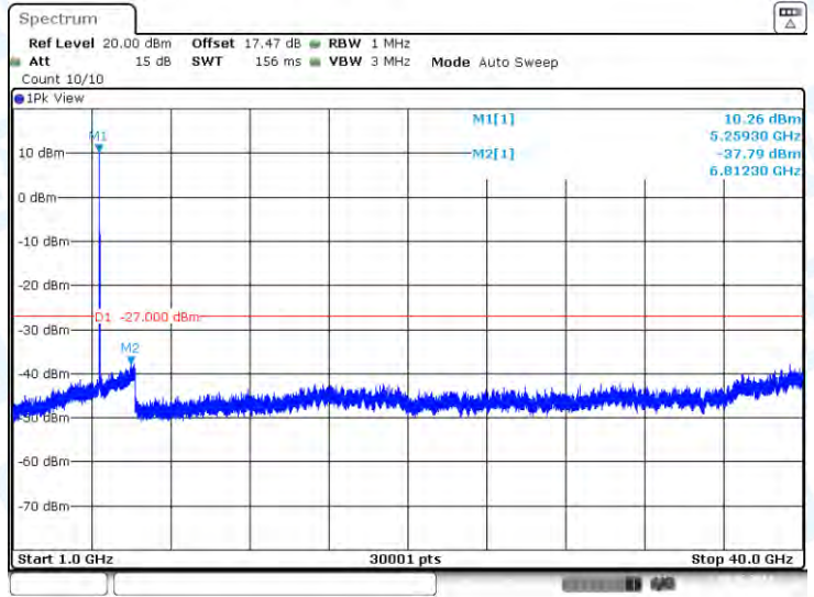
11A-CDD-Ant3-5240-1000~40000-PASS
