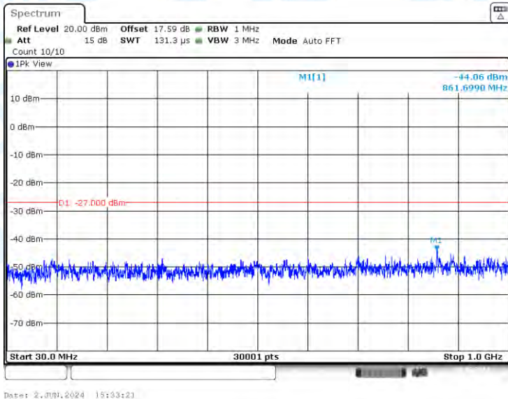
11N40-CDD-Ant2-5310-30~1000-PASS
