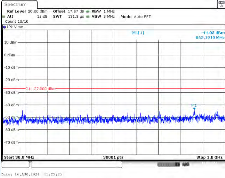
11N40-CDD-Ant2-5230-30~1000-PASS
