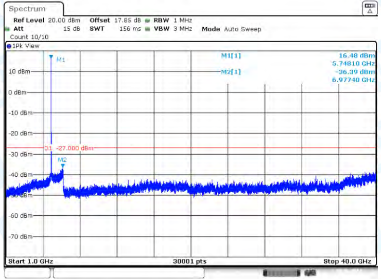
11A-CDD-Ant2-5745-1000~40000-PASS
