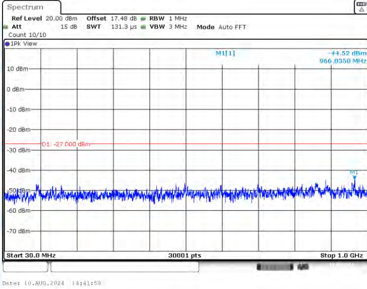
11A-CDD-Ant1-5240-30~1000-PASS
