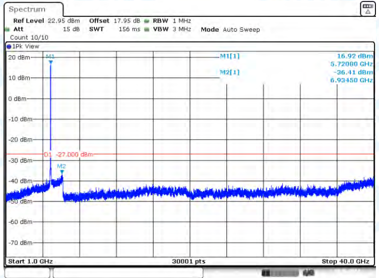
11A-Ant2-5720-1000~40000-PASS
