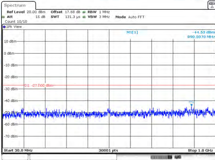
11A-CDD-Ant2-5500-30~1000-PASS
