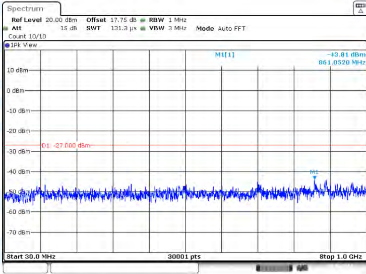
11N20-CDD-Ant1-5745-30~1000-PASS
