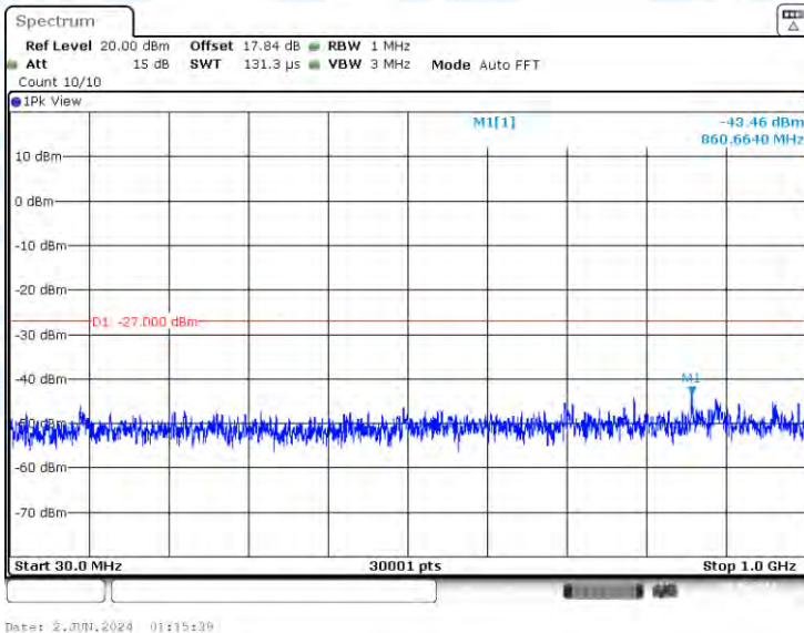
11N20-CDD-Ant2-5785-30~1000-PASS
