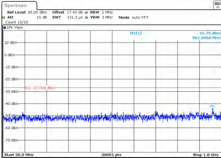
11A-CDD-Ant3-5280-30~1000-PASS
