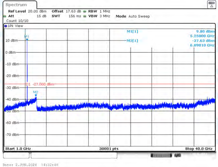
11N20-CDD-Ant3-5260-1000~40000-PASS
