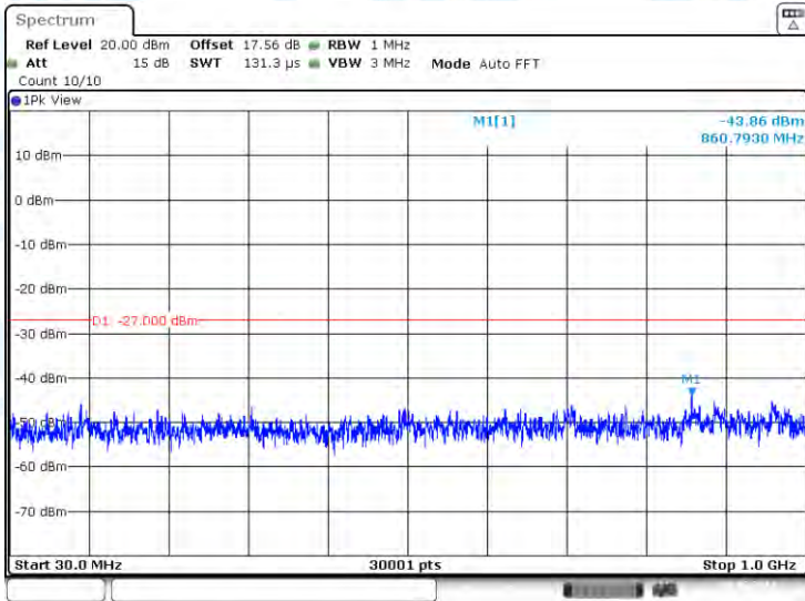
11A-CDD-Ant1-5260-30~1000-PASS
