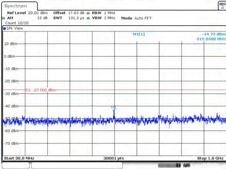
11N20-CDD-Ant2-5240-30~1000-PASS
