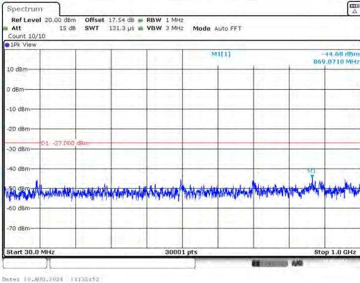
11A-CDD-Ant3-5180-30~1000-PASS
