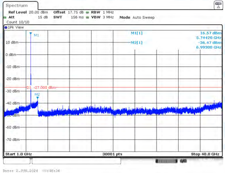
11A-CDD-Ant1-5745-1000~40000-PASS
