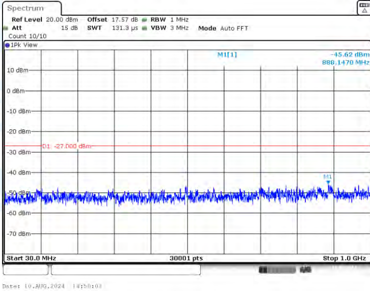
11A-CDD-Ant2-5240-30~1000-PASS
