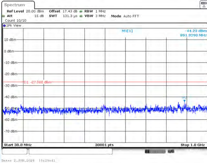
11N40-CDD-Ant1-5310-30~1000-PASS
