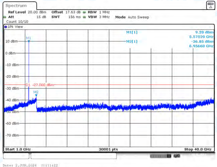
11N20-CDD-Ant1-5580-1000~40000-PASS
