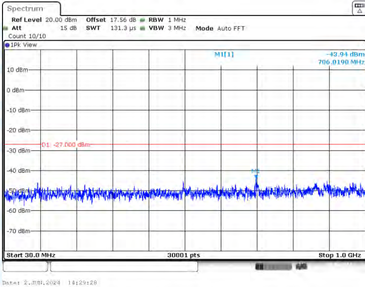
11N20-CDD-Ant2-5260-30~1000-PASS
