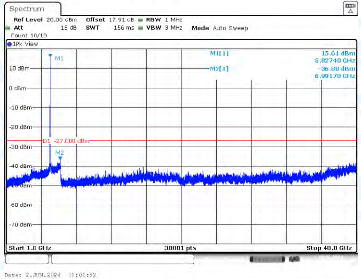
11A-CDD-Ant3-5825-1000~40000-PASS
