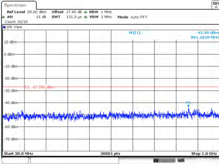
11A-CDD-Ant1-5825-30~1000-PASS
