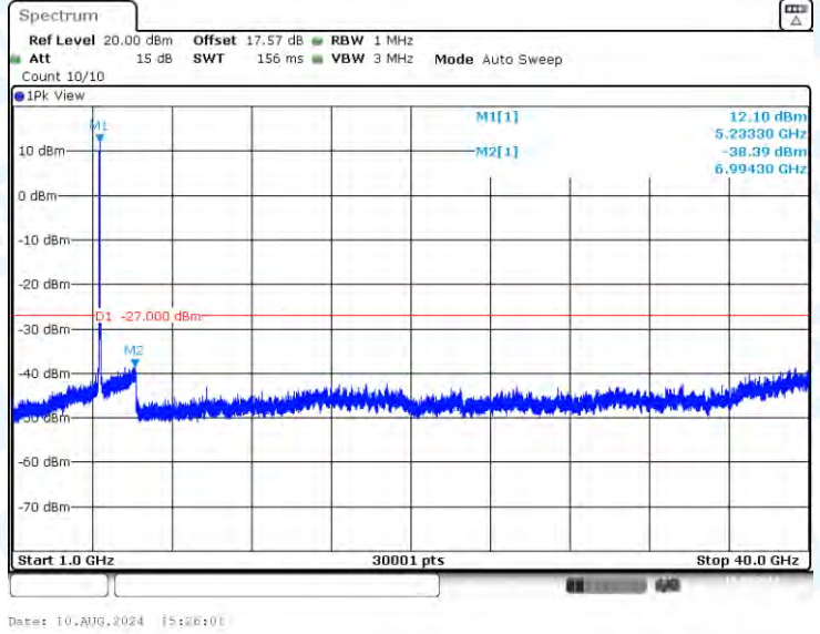
11N40-CDD-Ant2-5230-1000~40000-PASS
