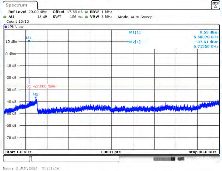
11N20-CDD-Ant3-5500-1000~40000-PASS
