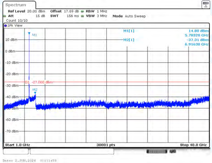
11N20-CDD-Ant1-5785-1000~40000-PASS
