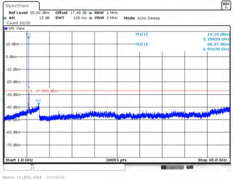
11N20-CDD-Ant2-5200-1000~40000-PASS
