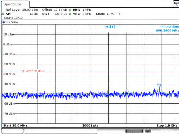
11A-CDD-Ant1-5500-30~1000-PASS
