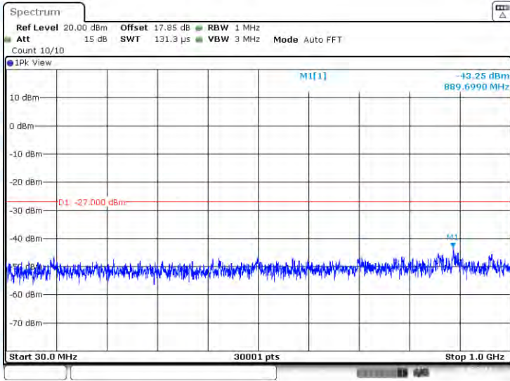
11A-CDD-Ant2-5745-30~1000-PASS
