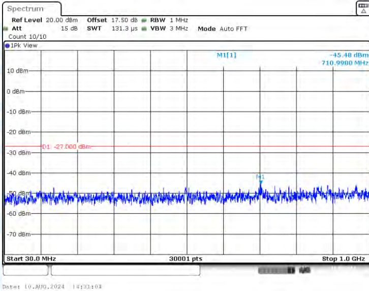
11A-CDD-Ant2-5180-30~1000-PASS
