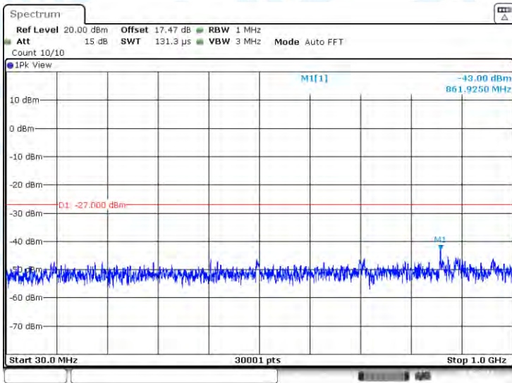
11N20-CDD-Ant3-5240-30~1000-PASS
