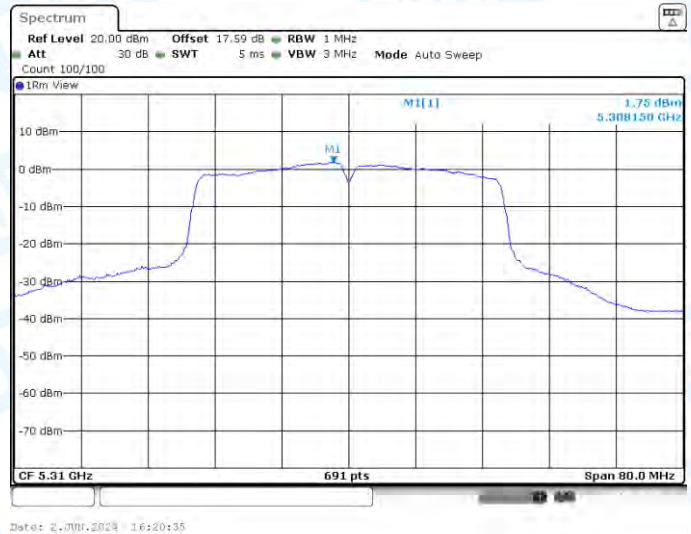
11AC40-CDD-Ant3-5310-PASS
