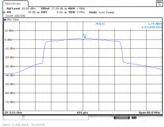
11AX40-CDD-Ant1-5510-PASS
