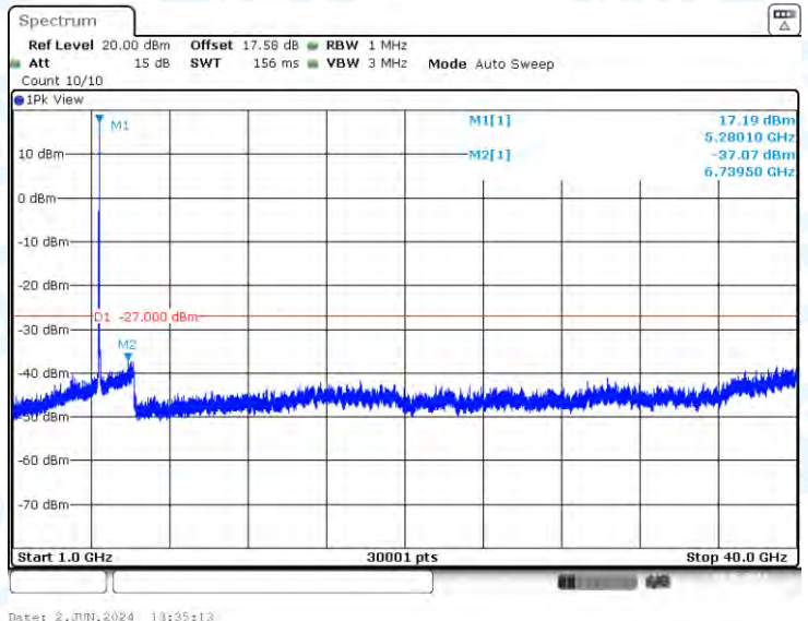
11A-Ant2-5280-1000~40000-PASS
