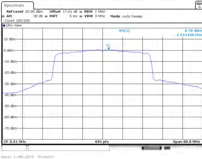
11AX40-CDD-Ant2-5510-PASS
