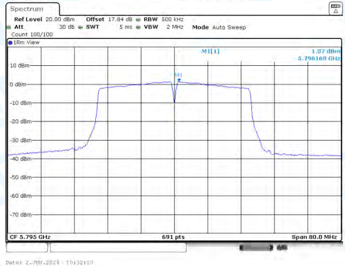
11AC40-CDD-Ant3-5795-PASS
