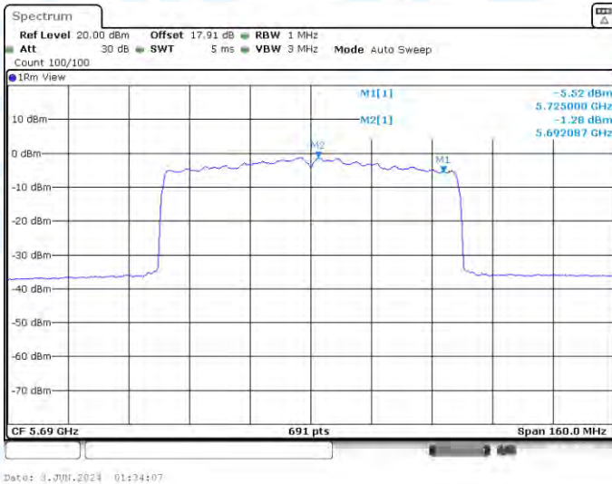
11AX80-CDD-Ant2-5690_UNII-2C-PASS
