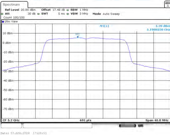
11AX20-CDD-Ant2-5200-PASS
