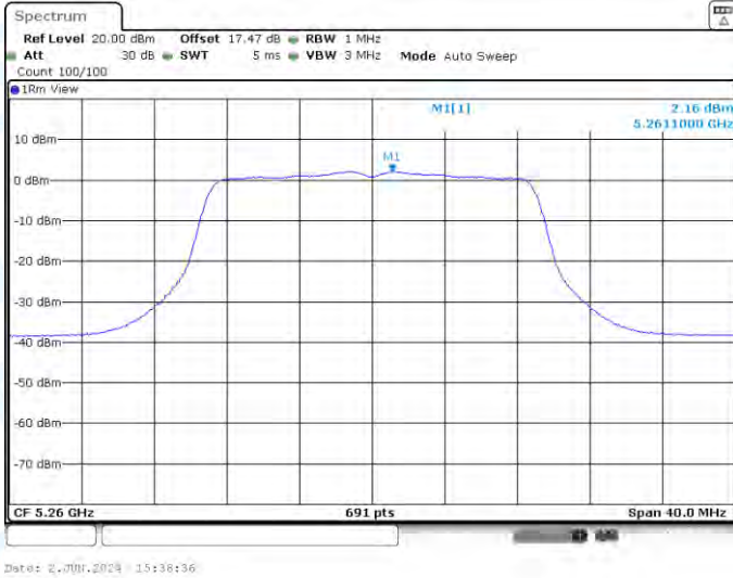
11AC20-CDD-Ant1-5260-PASS
