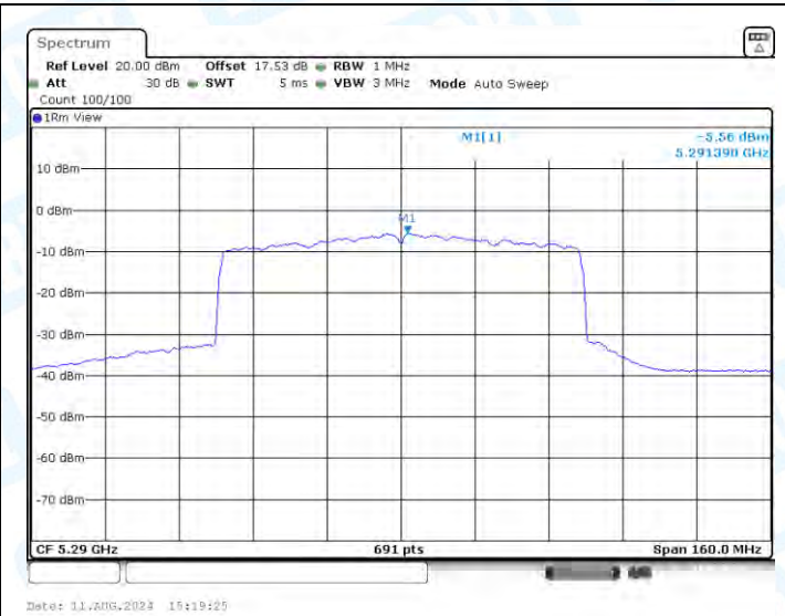
11AX80-CDD-Ant2-5290-PASS
