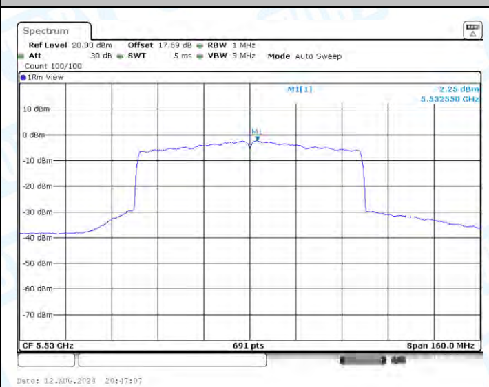
11AX80-CDD-Ant1-5530-PASS
