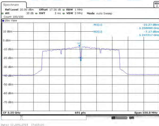
11AC160-CDD-Ant2-5250_UNII-1-PASS
