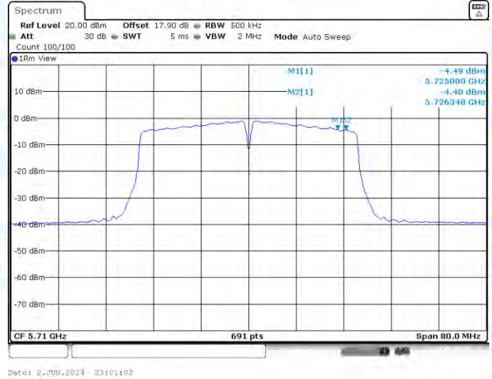
11AC40-CDD-Ant1-5710_UNII-3-PASS
