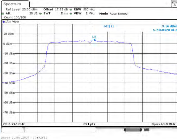
11AX20-CDD-Ant3-5745-PASS
