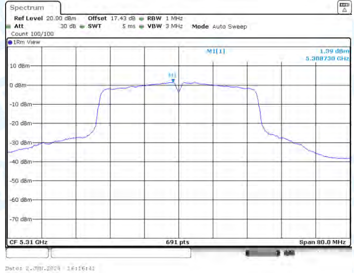
11AC40-CDD-Ant1-5310-PASS
