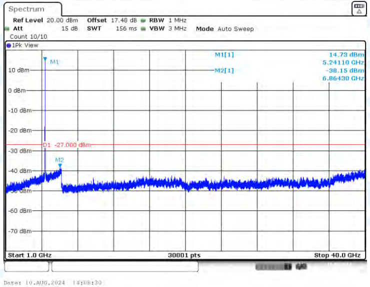
11A-Ant1-5240-1000~40000-PASS
