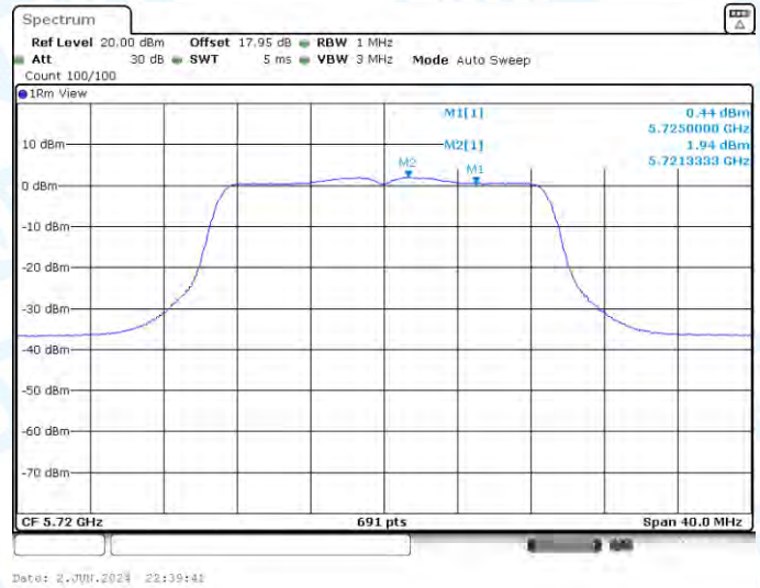
11AC20-CDD-Ant3-5720_UNII-2C-PASS
