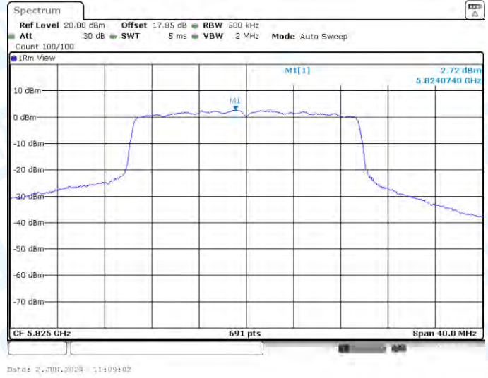
11AX20-CDD-Ant2-5825-PASS
