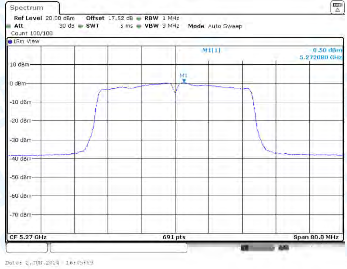
11AC40-CDD-Ant2-5270-PASS
