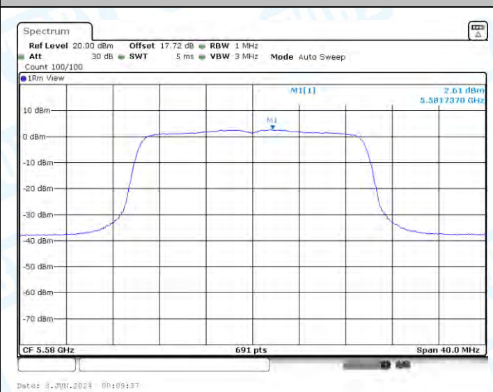
11AX20-CDD-Ant1-5580-PASS
