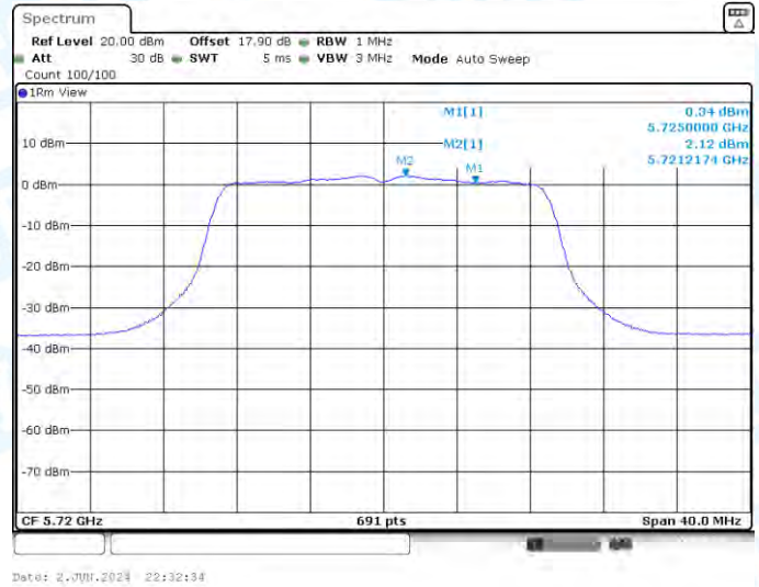
11AC20-CDD-Ant1-5720_UNII-2C-PASS
