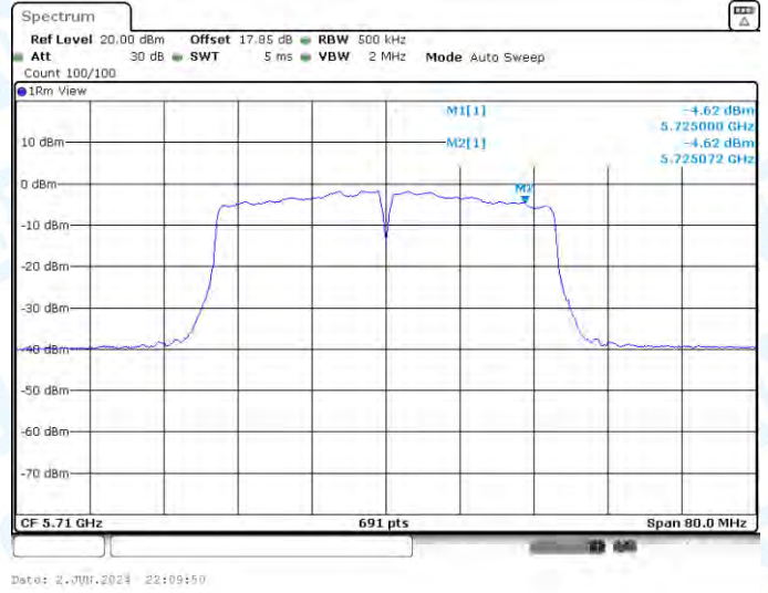
11N40-CDD-Ant2-5710_UNII-3-PASS
