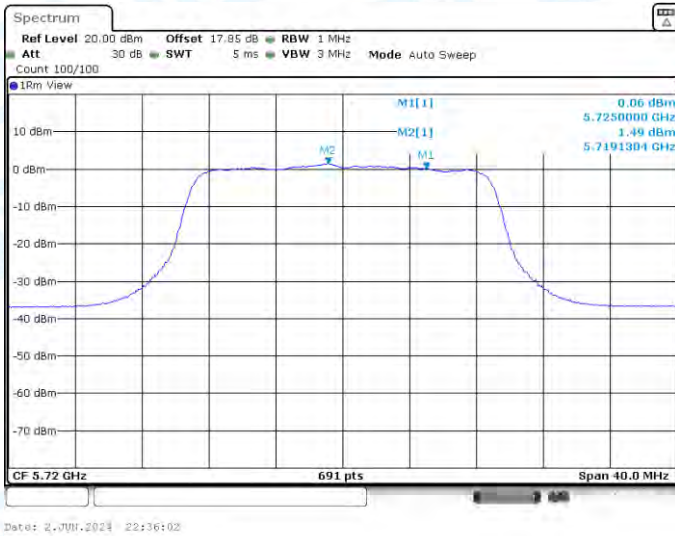
11AC20-CDD-Ant2-5720_UNII-2C-PASS
