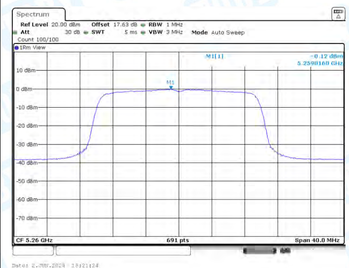
11AX20-CDD-Ant3-5260-PASS
