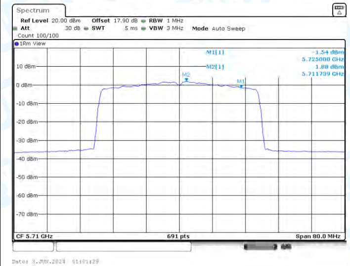
11AX40-CDD-Ant1-5710_UNII-2C-PASS
