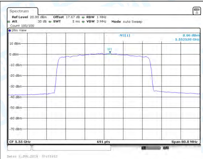
11AX40-CDD-Ant2-5550-PASS
