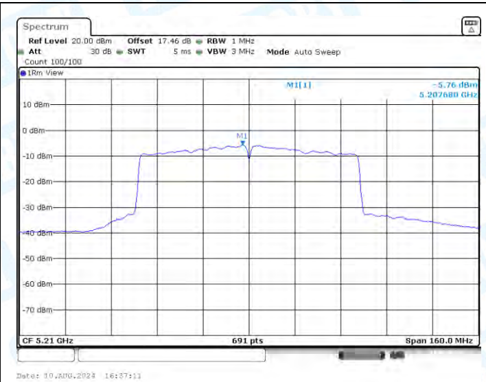
11AC80-CDD-Ant2-5210-PASS
