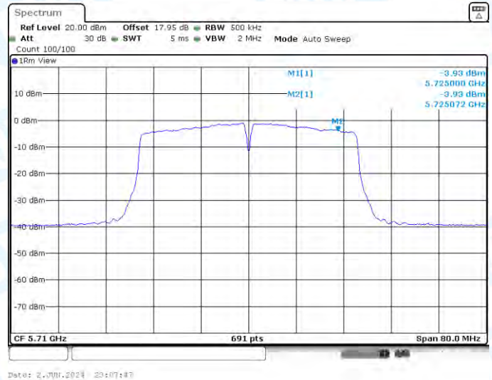
11AC40-CDD-Ant3-5710_UNII-3-PASS
