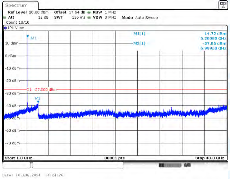
11A-Ant3-5200-1000~40000-PASS
