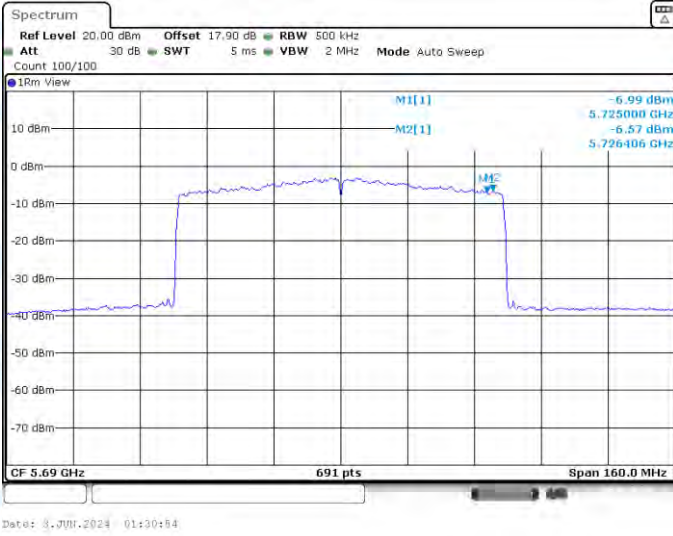
11AX80-CDD-Ant1-5690_UNII-3-PASS
