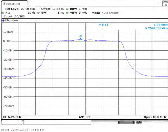
11AC20-CDD-Ant3-5260-PASS
