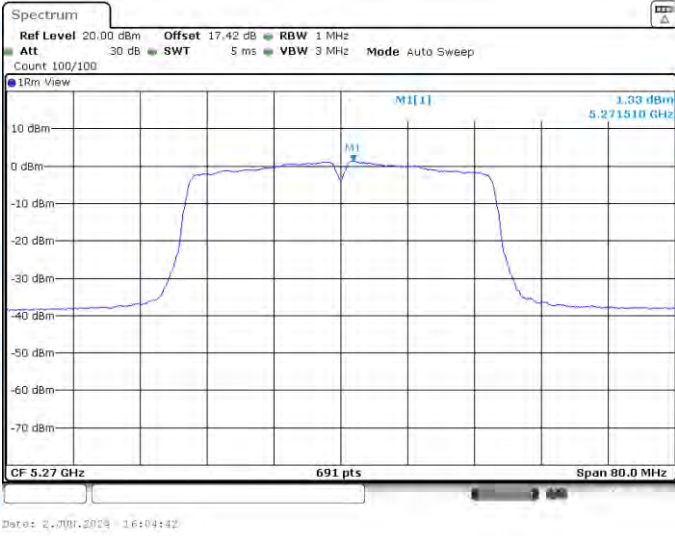
11AC40-CDD-Ant1-5270-PASS
