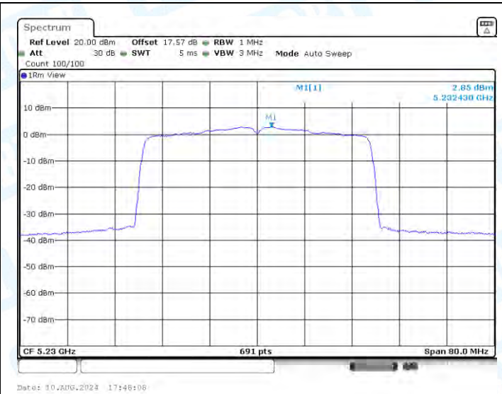
11AX40-CDD-Ant2-5230-PASS
