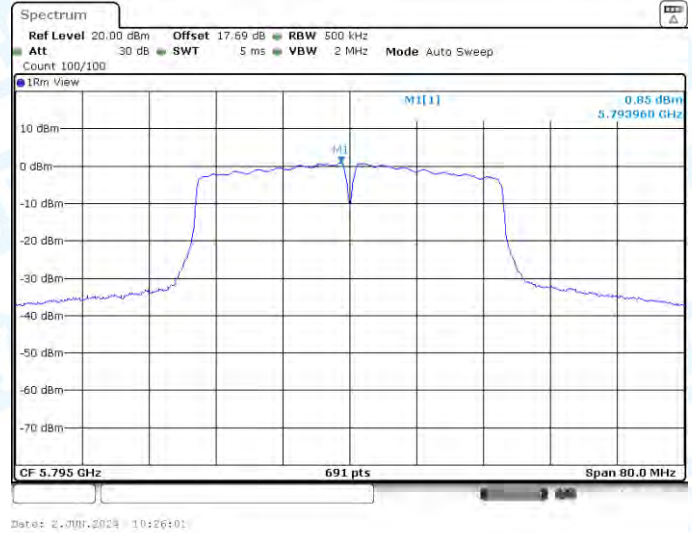
11AC40-CDD-Ant1-5795-PASS
