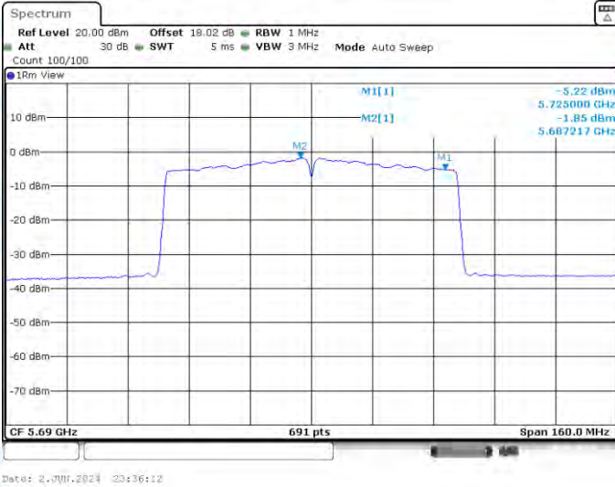
11AC80-CDD-Ant3-5690_UNII-2C-PASS
