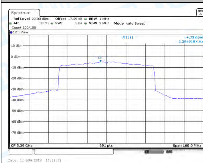
11AX80-CDD-Ant1-5290-PASS
