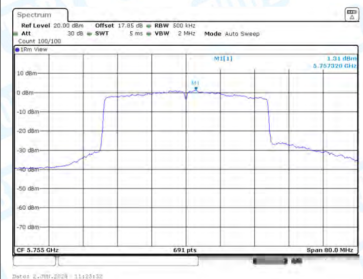
11AX40-CDD-Ant3-5755-PASS
