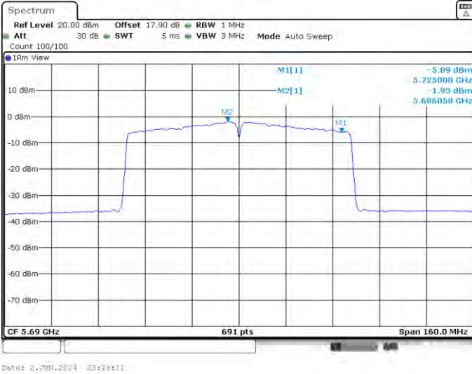
11AC80-CDD-Ant1-5690_UNII-2C-PASS
