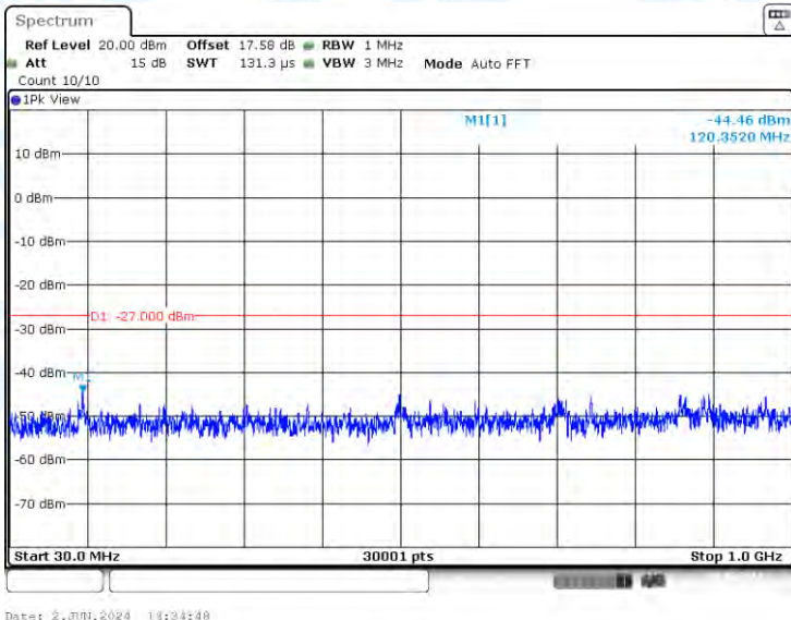
11A-Ant2-5280-30~1000-PASS
