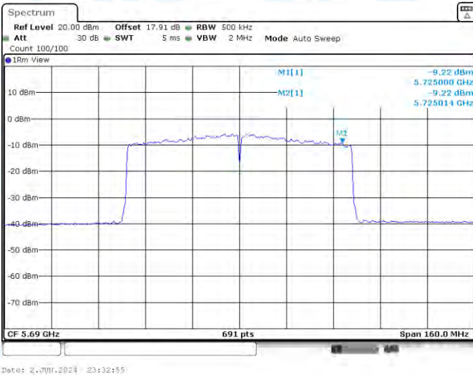
11AC80-CDD-Ant2-5690_UNII-3-PASS
