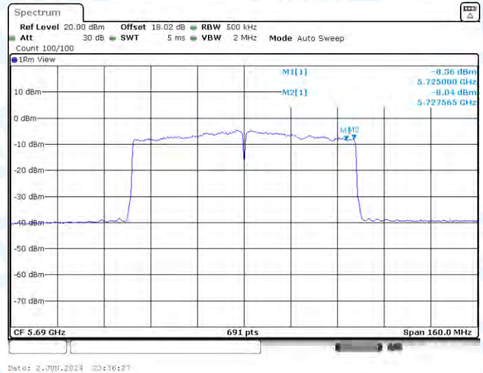
11AC80-CDD-Ant3-5690_UNII-3-PASS
