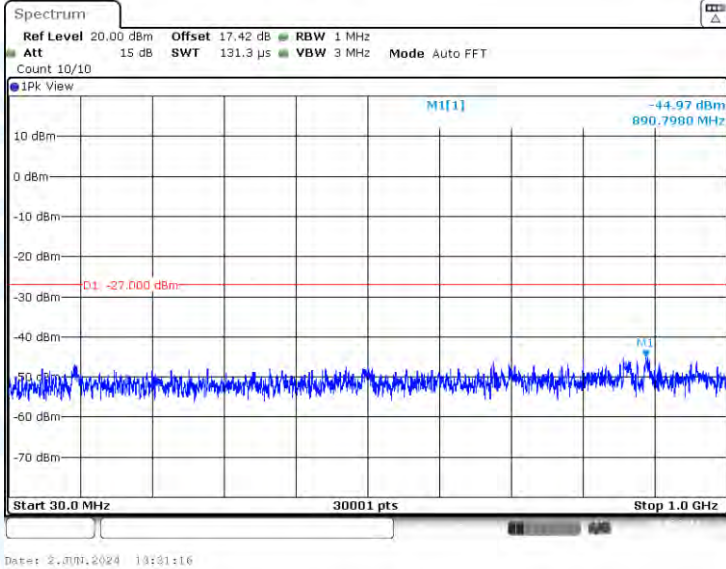
11A-Ant1-5280-30~1000-PASS
