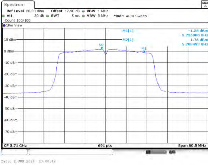
11AC40-CDD-Ant1-5710_UNII-2C-PASS
