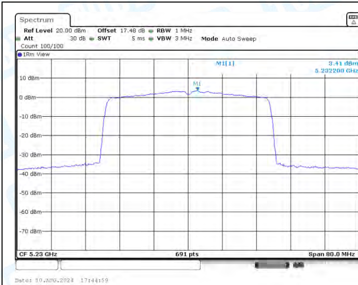
11AX40-CDD-Ant1-5230-PASS
