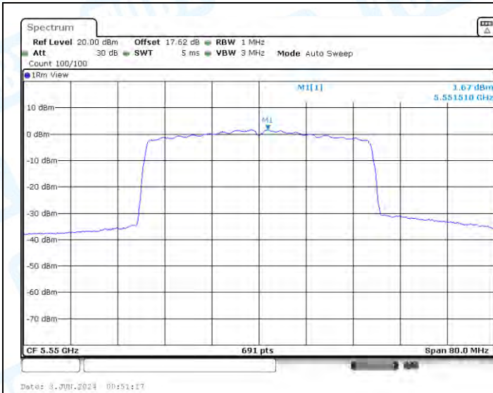
11AX40-CDD-Ant1-5550-PASS
