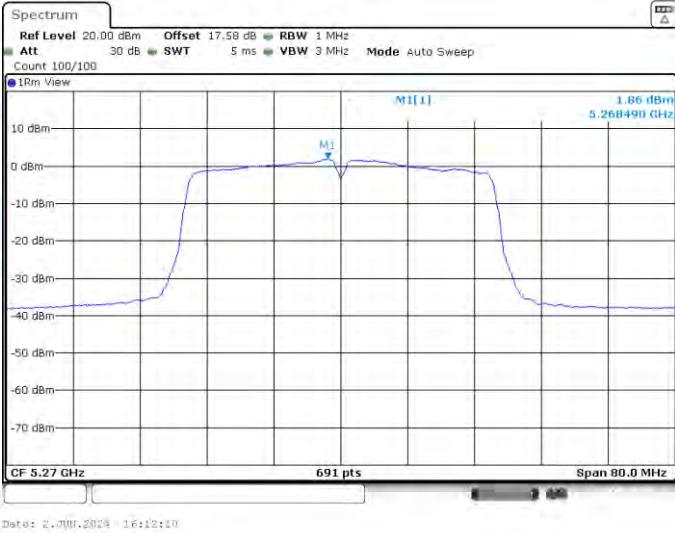
11AC40-CDD-Ant3-5270-PASS
