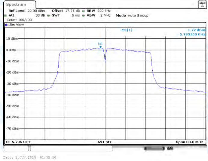
11N40-CDD-Ant2-5795-PASS
