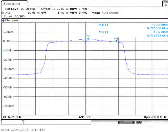
11AC40-CDD-Ant3-5710_UNII-2C-PASS
