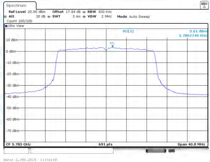
11AX20-CDD-Ant3-5785-PASS
