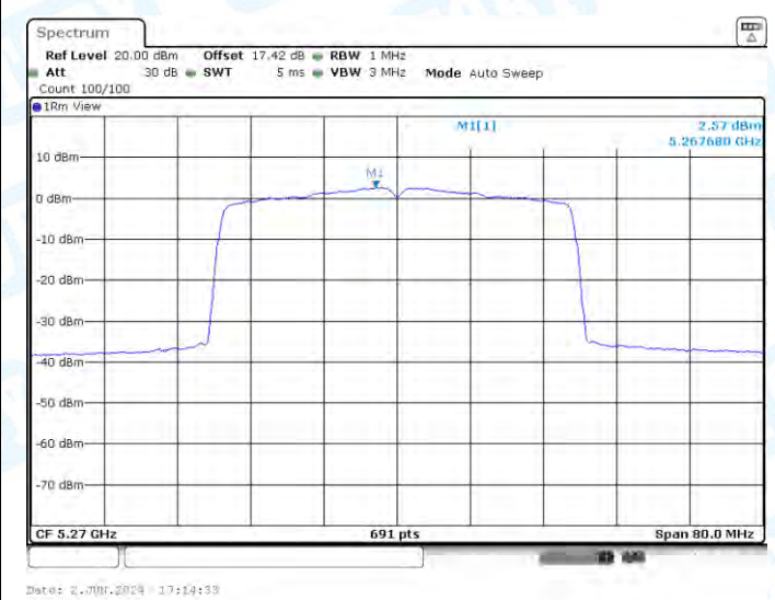
11AX40-CDD-Ant1-5270-PASS
