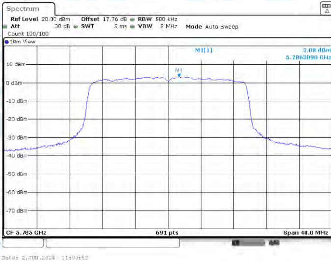
11AX20-CDD-Ant2-5785-PASS
