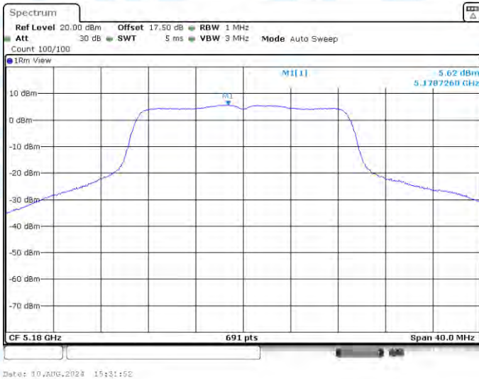
11AC20-CDD-Ant2-5180-PASS
