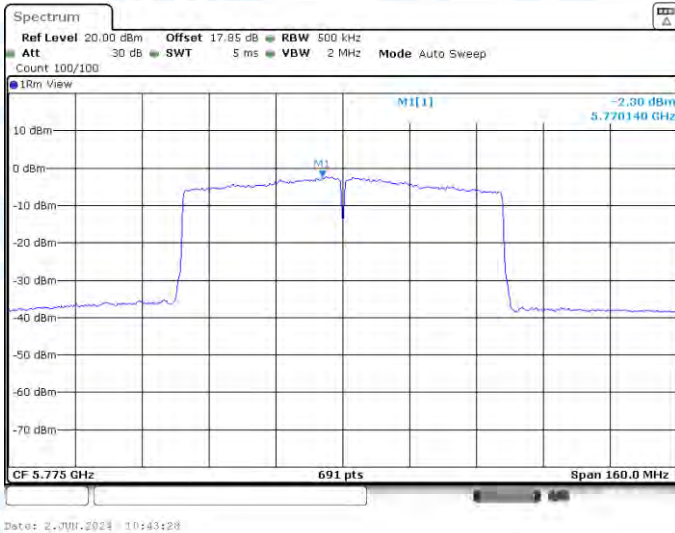
11AC80-CDD-Ant3-5775-PASS
