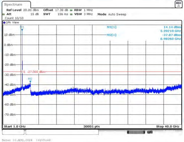
11A-Ant1-5200-1000~40000-PASS
