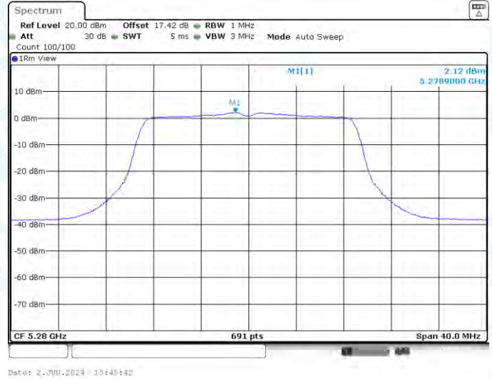
11AC20-CDD-Ant1-5280-PASS
