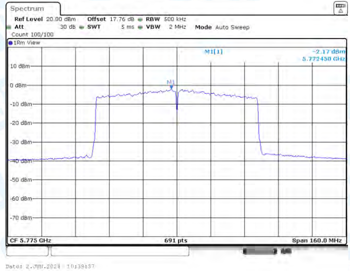
11AC80-CDD-Ant2-5775-PASS
