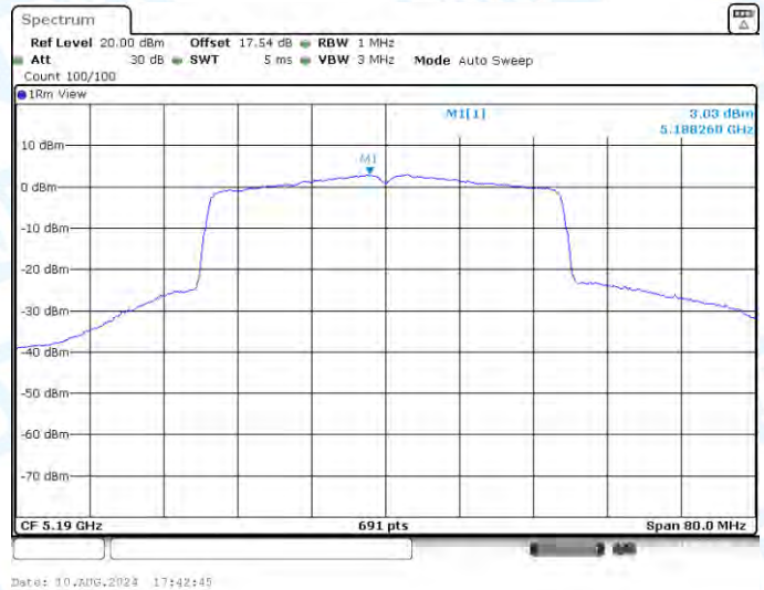
11AX40-CDD-Ant3-5190-PASS
