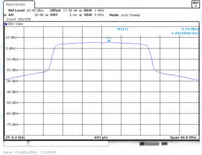
11AX20-CDD-Ant1-5200-PASS
