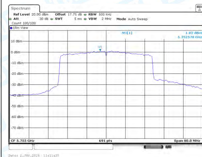
11AX40-CDD-Ant2-5755-PASS
