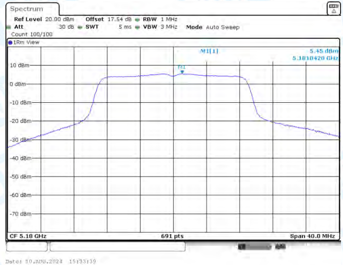
11AC20-CDD-Ant3-5180-PASS
