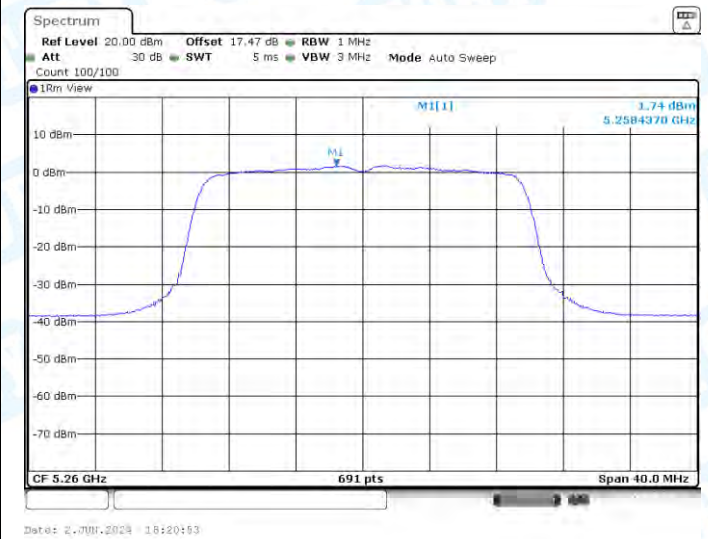
11AX20-CDD-Ant1-5260-PASS
