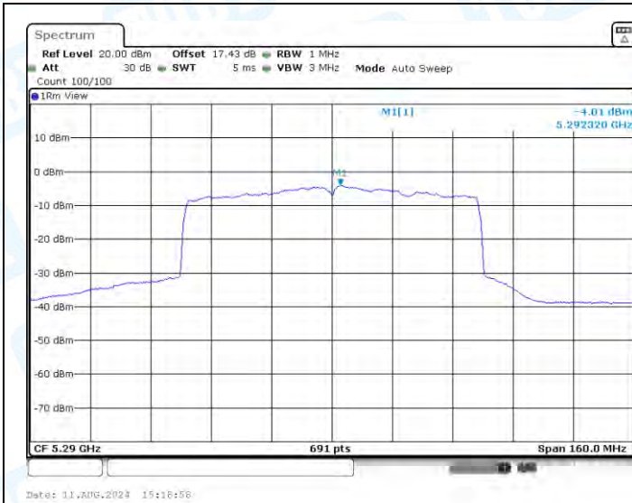
11AX80-CDD-Ant1-5290-PASS
