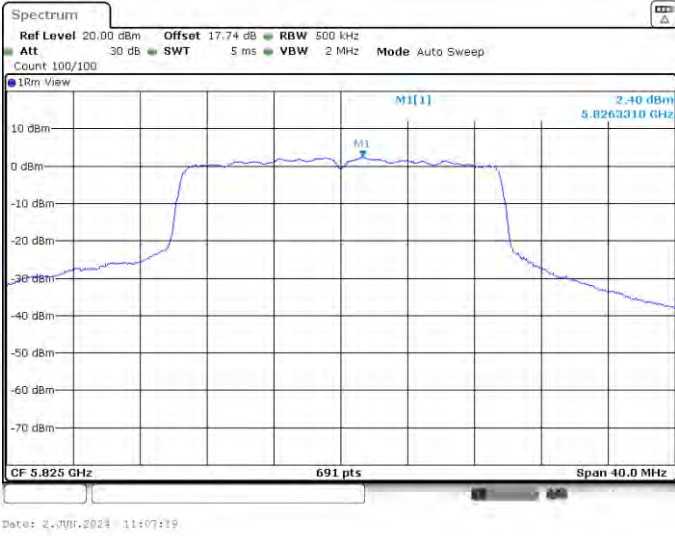
11AX20-CDD-Ant1-5825-PASS
