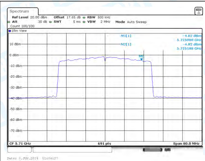
11AX40-CDD-Ant2-5710_UNII-3-PASS
