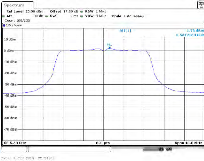
11AC20-CDD-Ant1-5580-PASS
