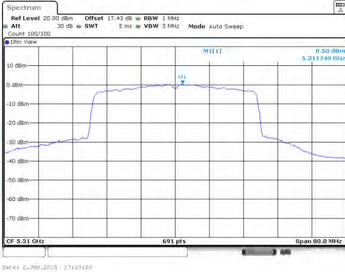
11AX40-CDD-Ant1-5310-PASS
