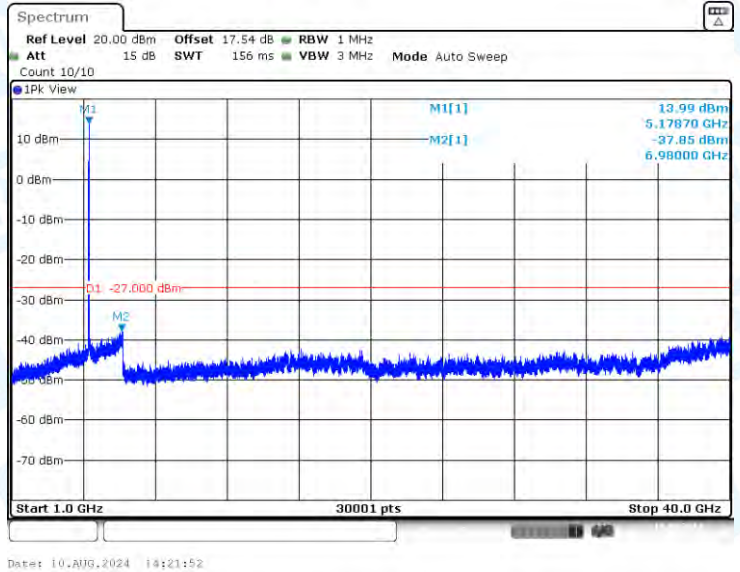
11A-Ant3-5180-1000~40000-PASS
