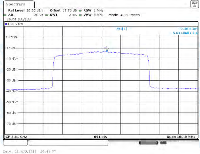
11AX80-CDD-Ant2-5610-PASS
