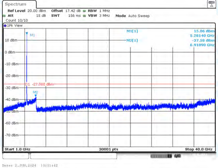
11A-Ant1-5280-1000~40000-PASS
