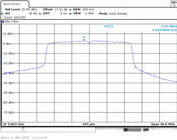
11AX20-CDD-Ant3-5825-PASS
