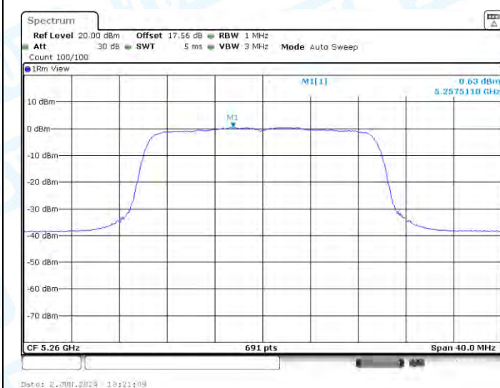
11AX20-CDD-Ant2-5260-PASS
