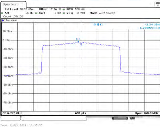
11AX80-CDD-Ant2-5775-PASS
