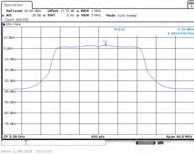
11AC20-CDD-Ant3-5580-PASS
