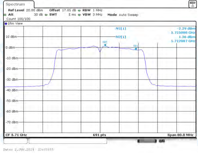
11AC40-CDD-Ant2-5710_UNII-2C-PASS
