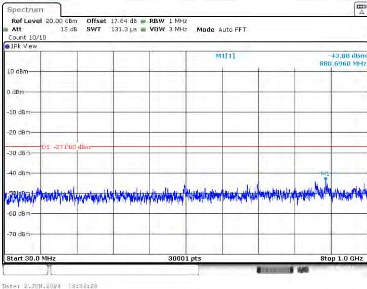
11A-Ant1-5500-30~1000-PASS
