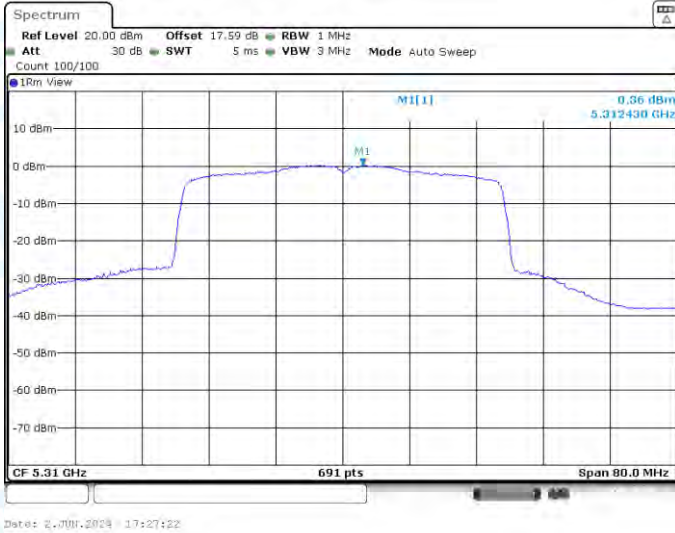
11AX40-CDD-Ant3-5310-PASS
