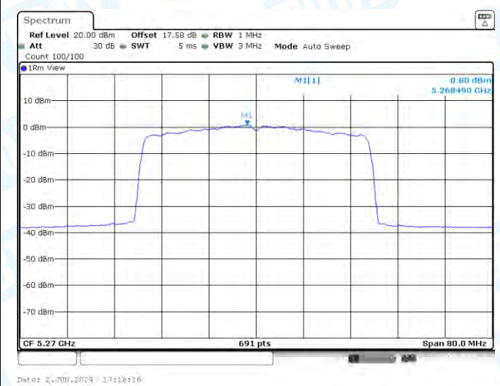
11AX40-CDD-Ant3-5270-PASS
