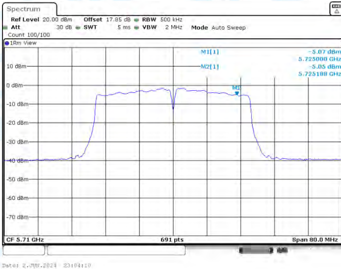
11AC40-CDD-Ant2-5710_UNII-3-PASS
