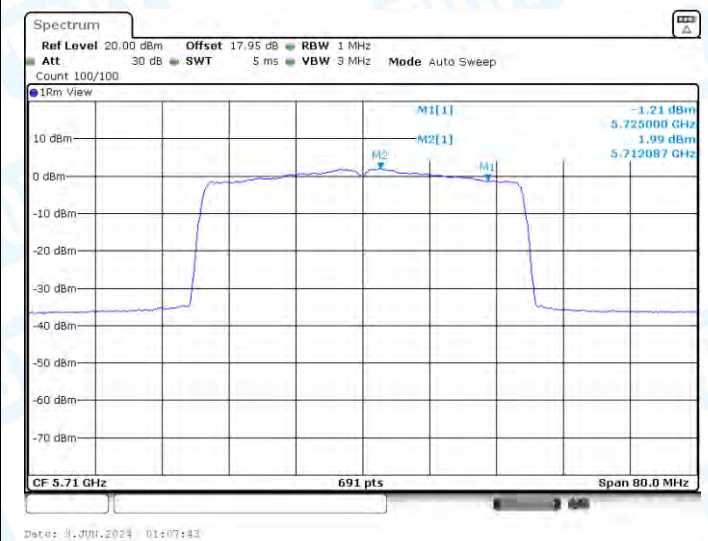
11AX40-CDD-Ant3-5710_UNII-2C-PASS
