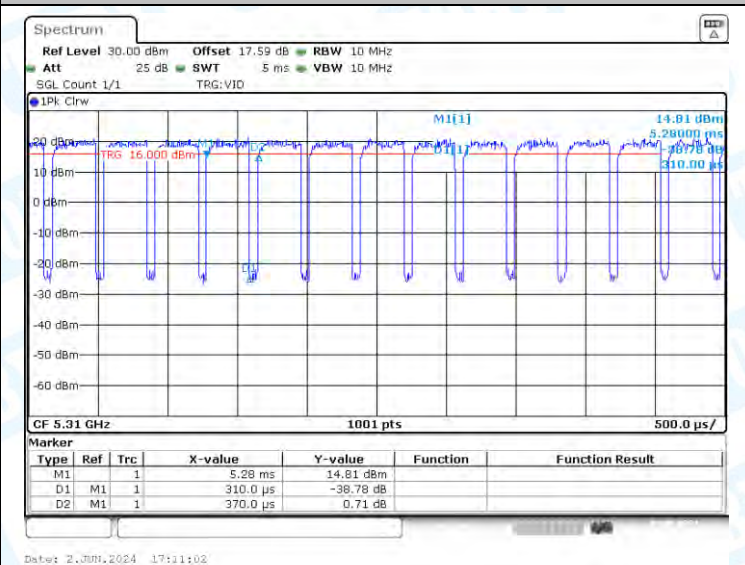
NTNV-11AX40-CDD-Ant3-5310
