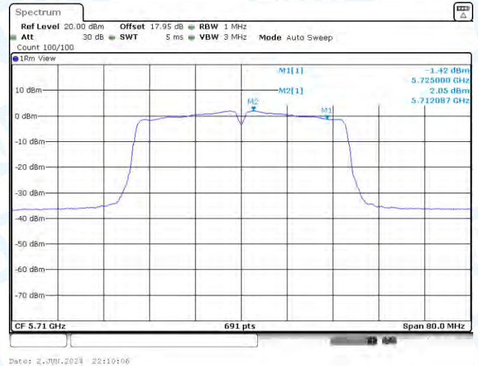
11N40-CDD-Ant3-5710_UNII-2C-PASS
