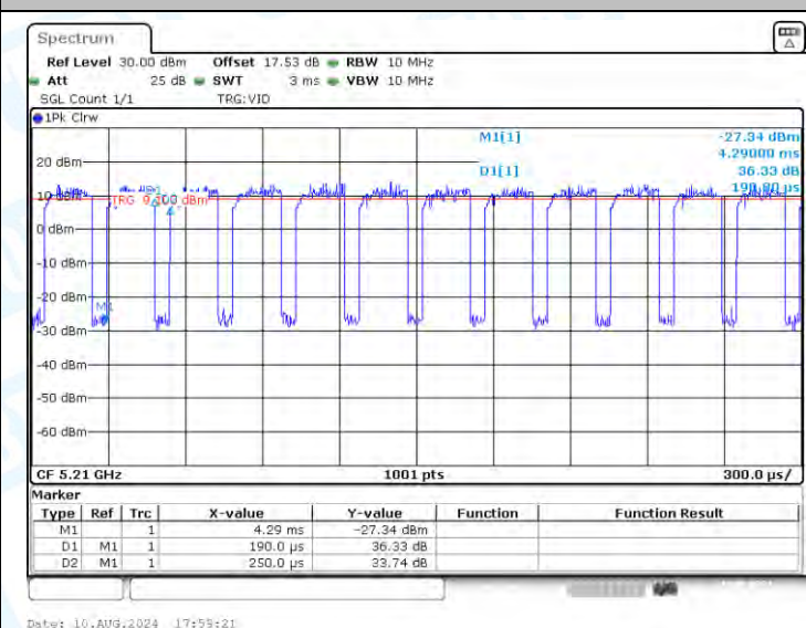
NTVN-11AX80-CDD-Ant3-5210
