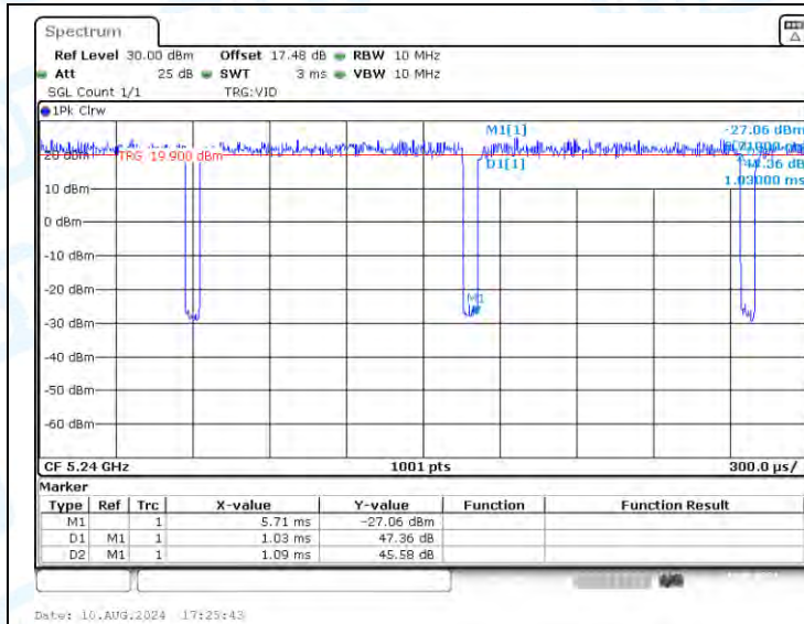
NTNV-11AX20-CDD-Ant1-5240
