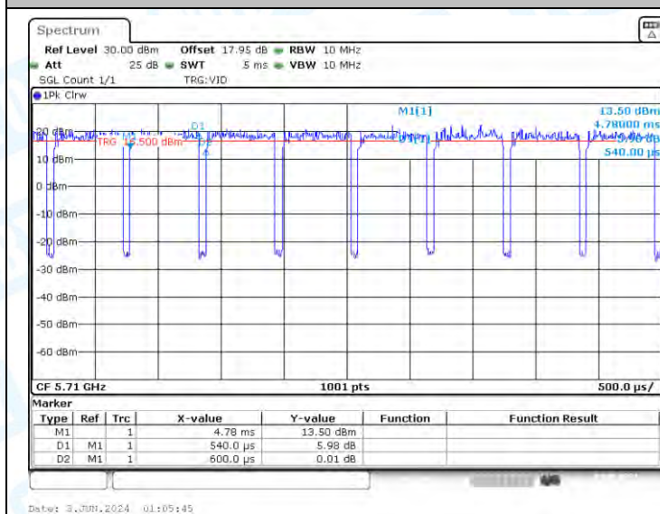
NTNV-11AX40-CDD-Ant3-5710
