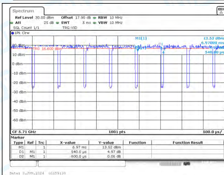
NTNV-11AX40-CDD-Ant1-5710
