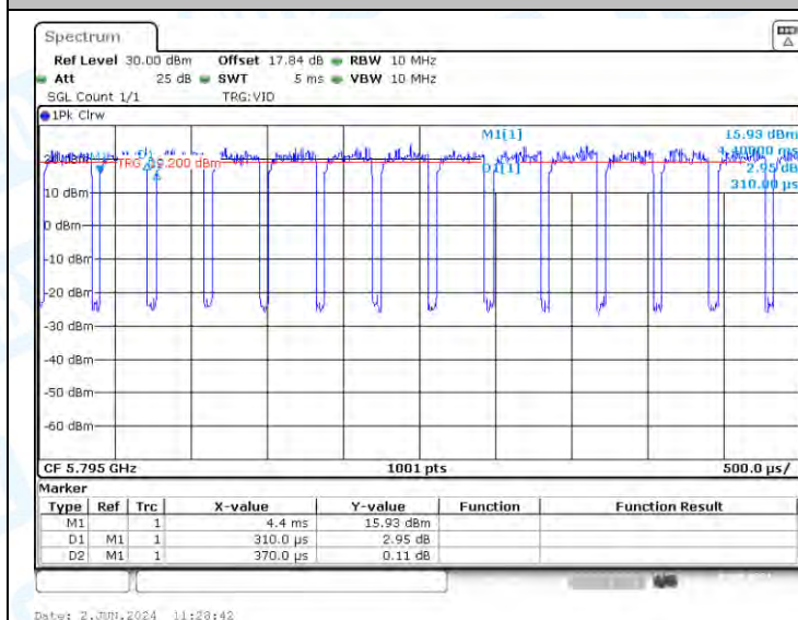
NTVN-11AX40-CDD-Ant3-5795
