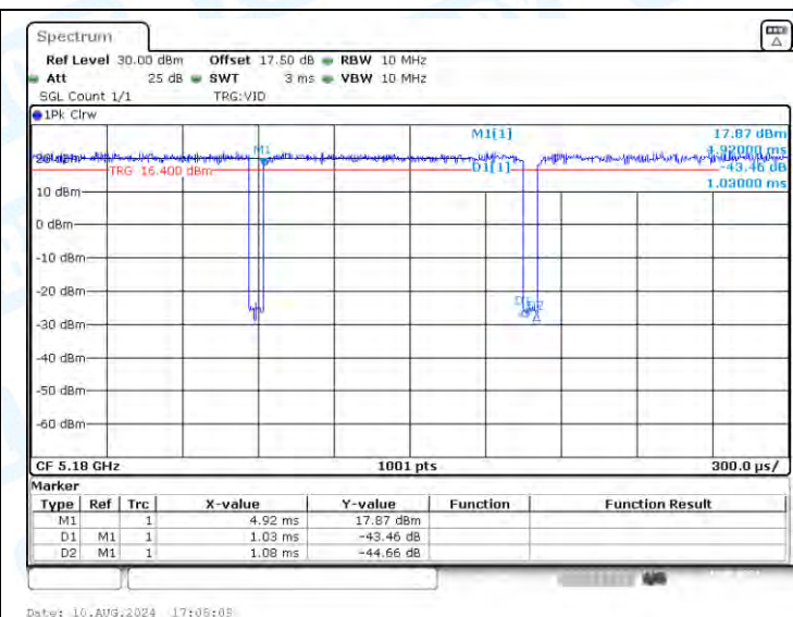
NTNV-11AX20-CDD-Ant2-5180
