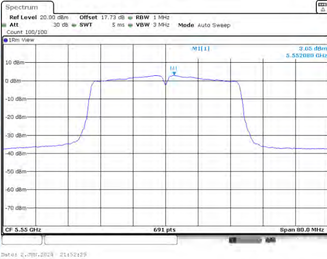
11N40-CDD-Ant3-5550-PASS
