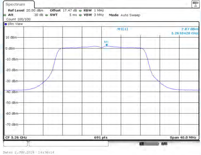
11N20-CDD-Ant1-5260-PASS
