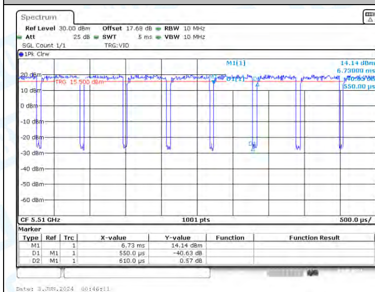
NTNV-11AX40-CDD-Ant3-5510
