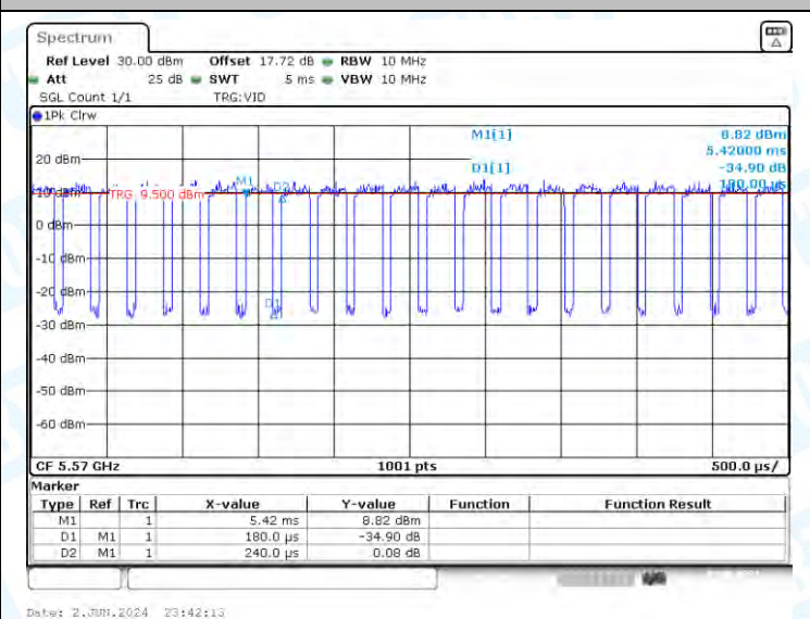
NTNV-11AC160-CDD-Ant3-5570
