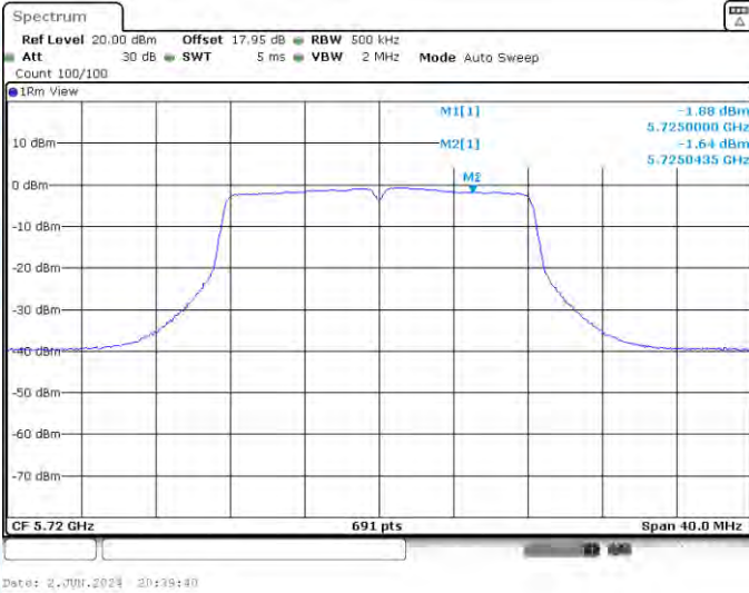
11A-CDD-Ant3-5720_UNII-3-PASS
