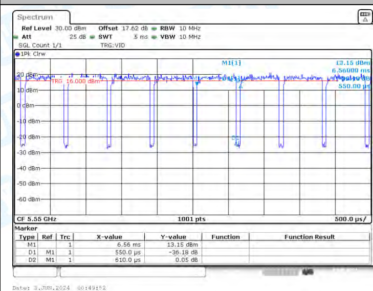
NTNV-11AX40-CDD-Ant1-5550
