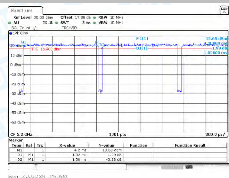
NTNV-11AX20-CDD-Ant1-5200
