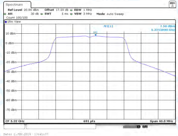
11A-Ant3-5320-PASS
