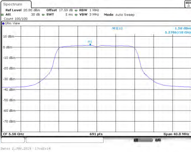
11A-CDD-Ant1-5580-PASS
