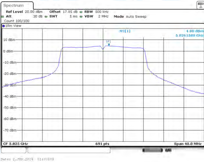
11A-CDD-Ant2-5825-PASS
