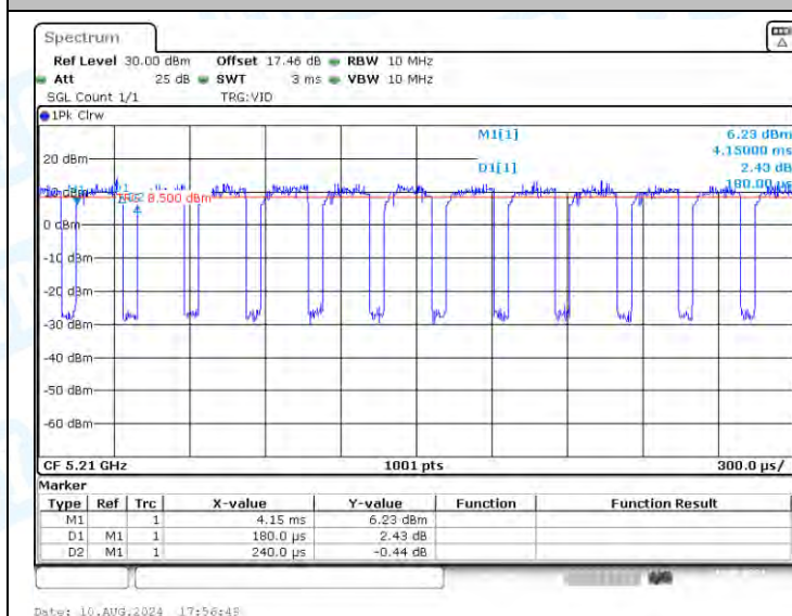
NTVN-11AX80-CDD-Ant2-5210
