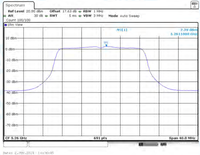
11N20-CDD-Ant3-5260-PASS
