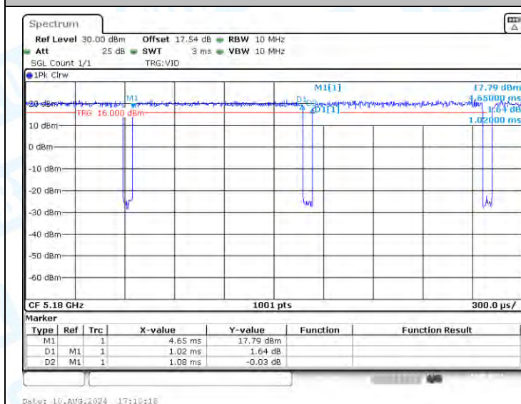
NTNV-11AX20-CDD-Ant3-5180
