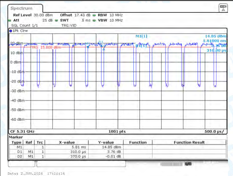
NTNV-11AX40-CDD-Ant1-5310
