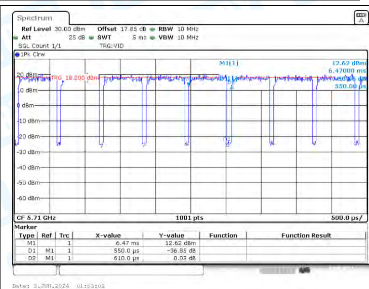
NTNV-11AX40-CDD-Ant2-5710
