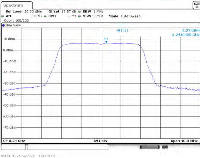
11A-CDD-Ant2-5240-PASS
