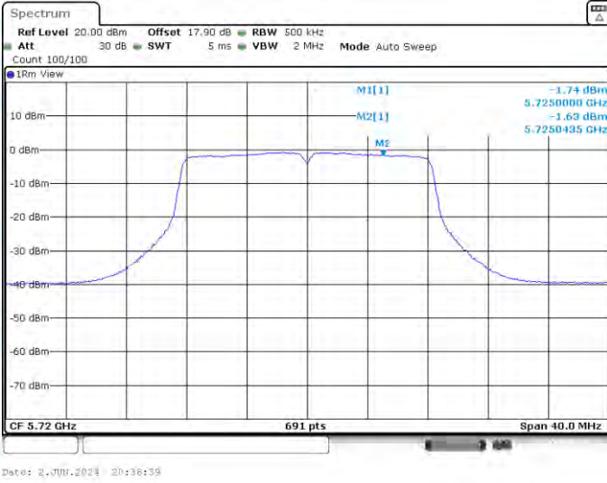
11A-CDD-Ant1-5720_UNII-3-PASS
