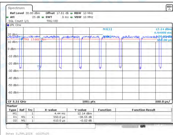
NTNV-11AX40-CDD-Ant2-5510
