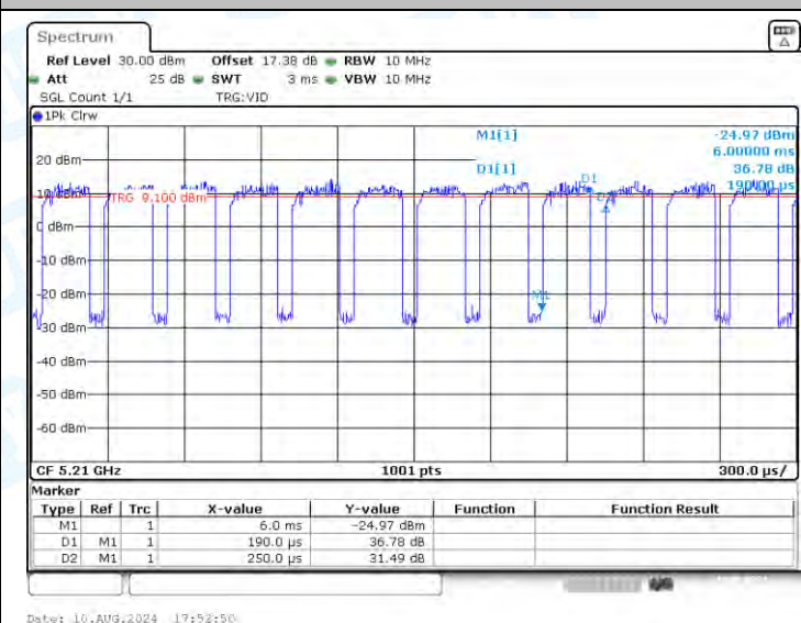
NTVN-11AX80-CDD-Ant1-5210
