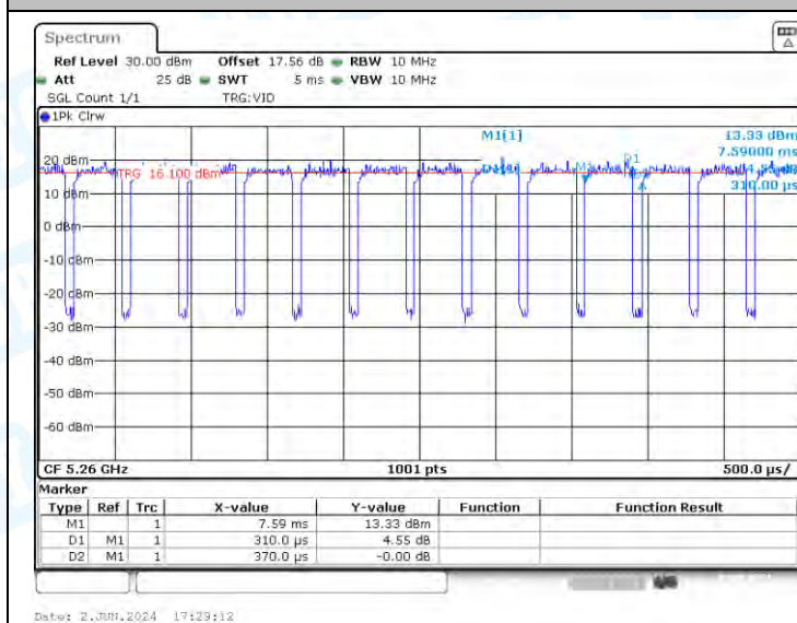
NTNV-11AX20-CDD-Ant2-5260
