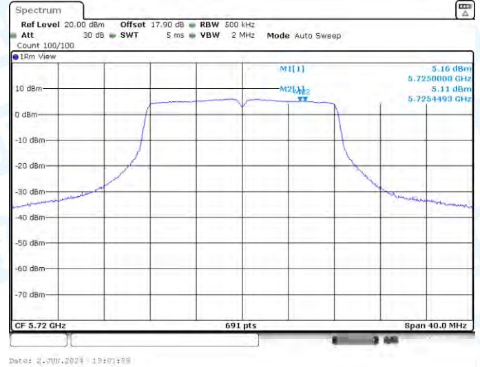
11A-Ant1-5720_UNII-3-PASS
