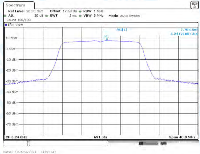
11A-CDD-Ant3-5240-PASS
