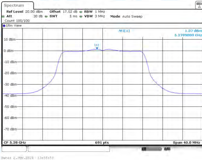
11A-CDD-Ant2-5280-PASS
