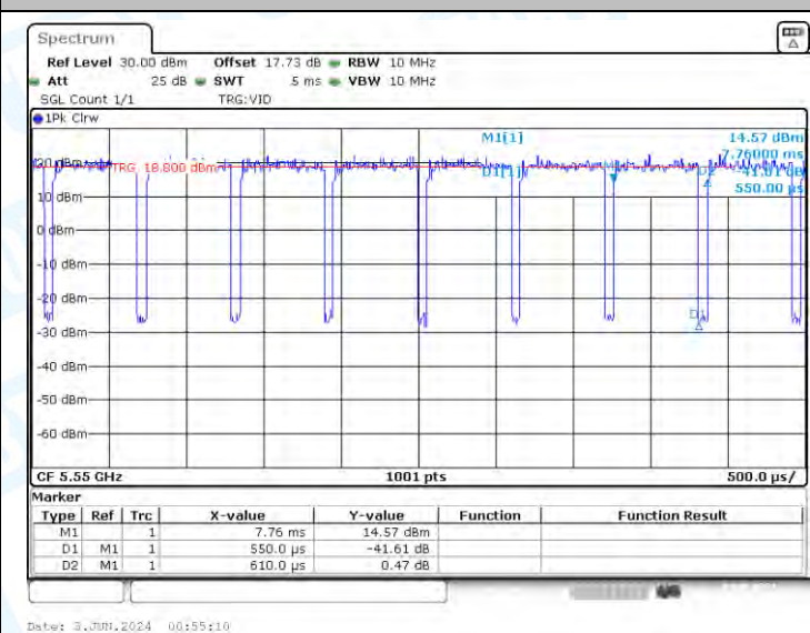
NTNV-11AX40-CDD-Ant3-5550
