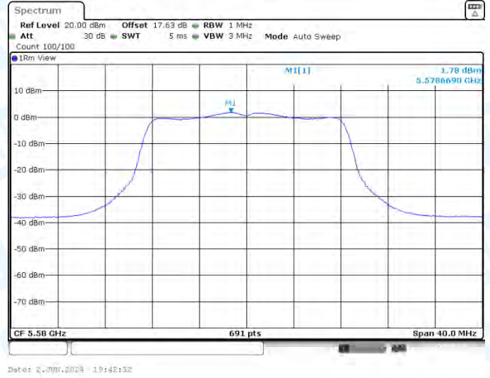
11A-CDD-Ant2-5580-PASS
