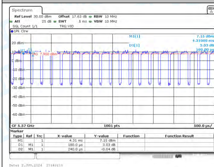
NTNV-11AC160-CDD-Ant2-5570
