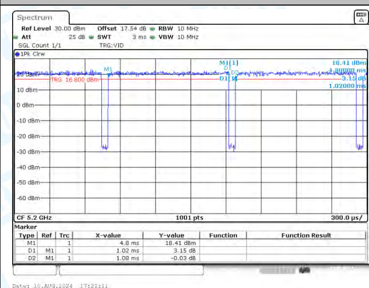
NTNV-11AX20-CDD-Ant3-5200
