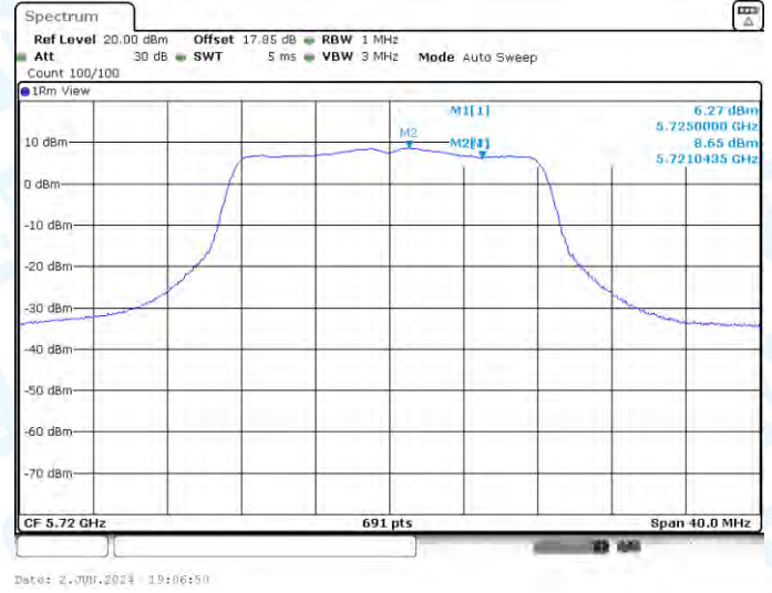
11A-Ant2-5720_UNII-2C-PASS
