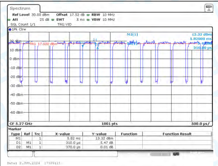
NTNV-11AX40-CDD-Ant2-5270
