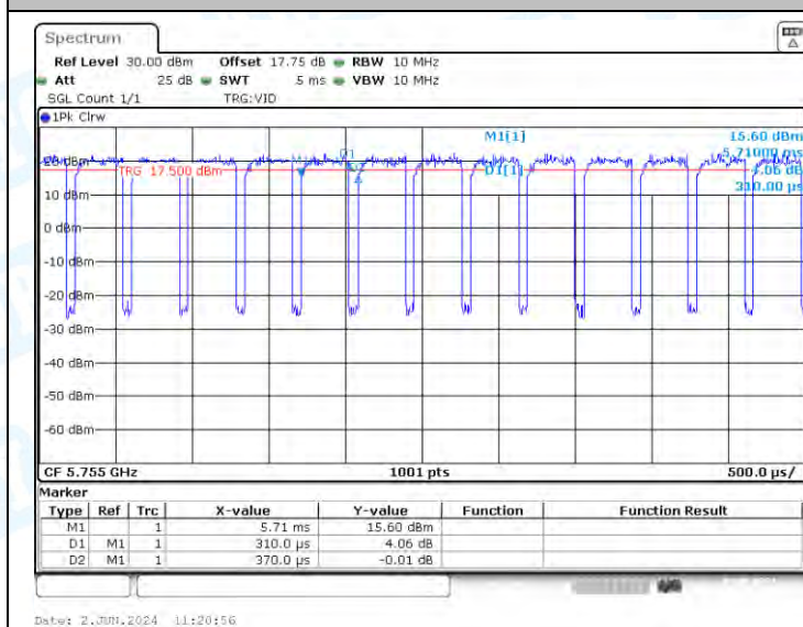
NTNV-11AX40-CDD-Ant2-5755
