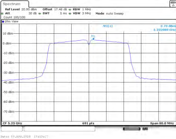
11N40-CDD-Ant1-5230-PASS
