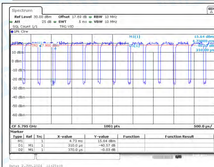
NTVN-11AX40-CDD-Ant1-5795
