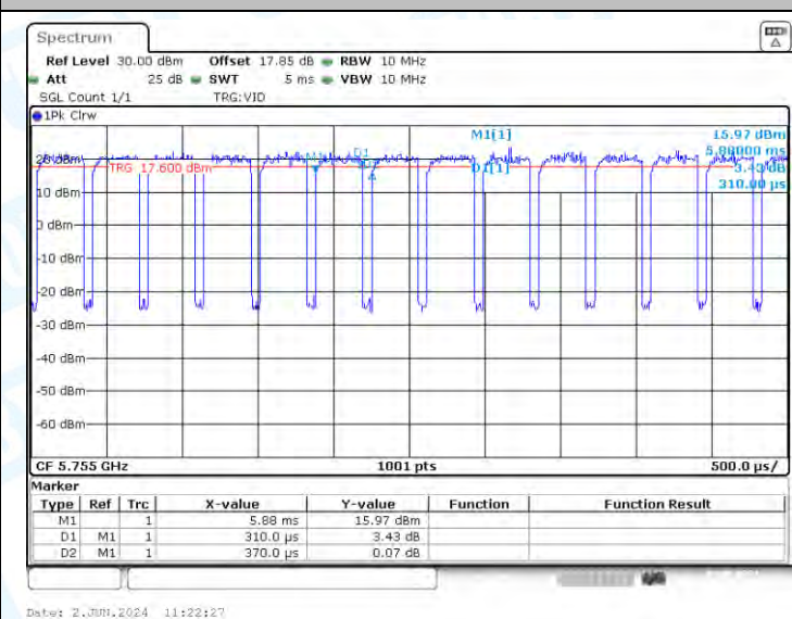
NTNV-11AX40-CDD-Ant3-5755
