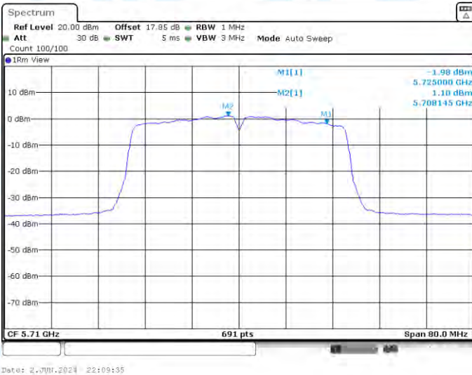
11N40-CDD-Ant2-5710_UNII-2C-PASS
