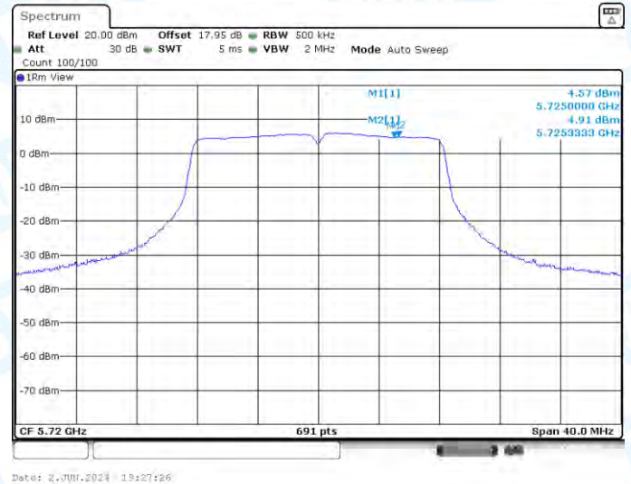
11A-Ant3-5720_UNII-3-PASS
