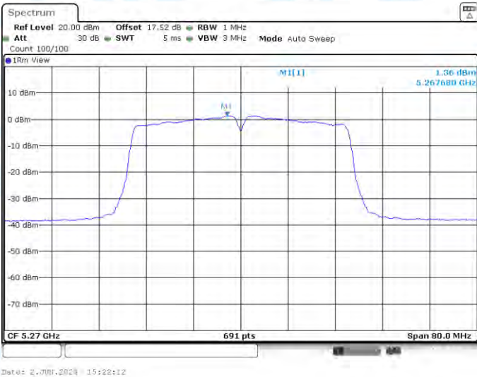
11N40-CDD-Ant2-5270-PASS
