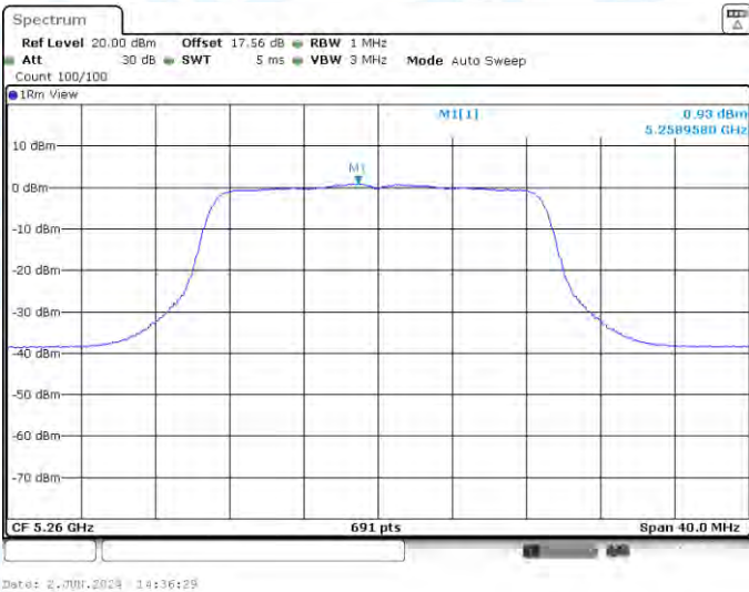
11N20-CDD-Ant2-5260-PASS
