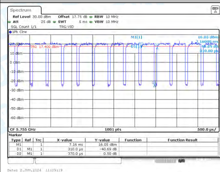
NTNV-11AX40-CDD-Ant1-5755
