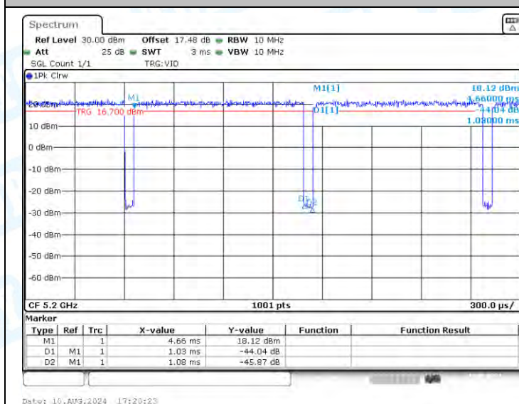
NTNV-11AX20-CDD-Ant2-5200
