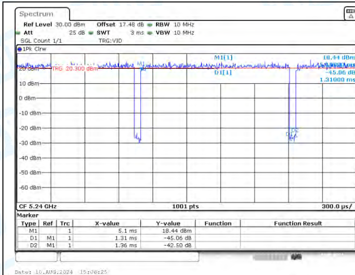
NTVN-11N20-CDD-Ant1-5240
