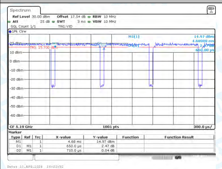
NTNV-11AC40-CDD-Ant3-5190
