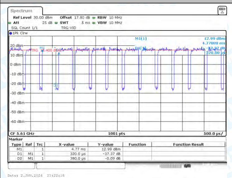
NTNV-11AC80-CDD-Ant3-5610
