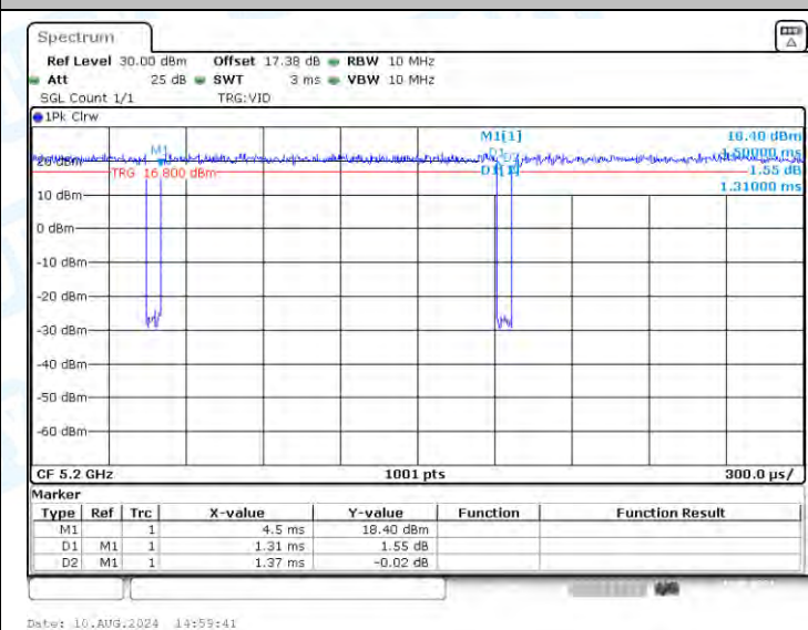
NTNV-11N20-CDD-Ant1-5200
