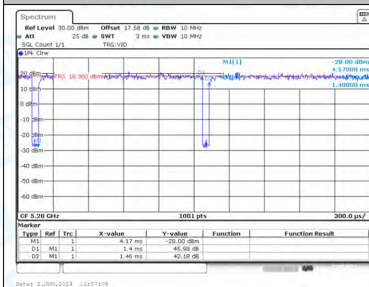
NTNV-11A-CDD-Ant3-5280
