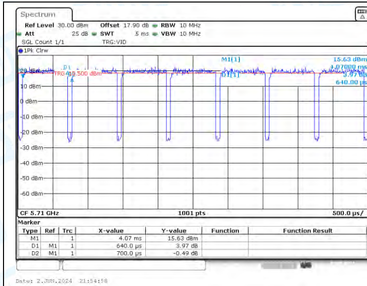
NTNV-11N40-CDD-Ant1-5710
