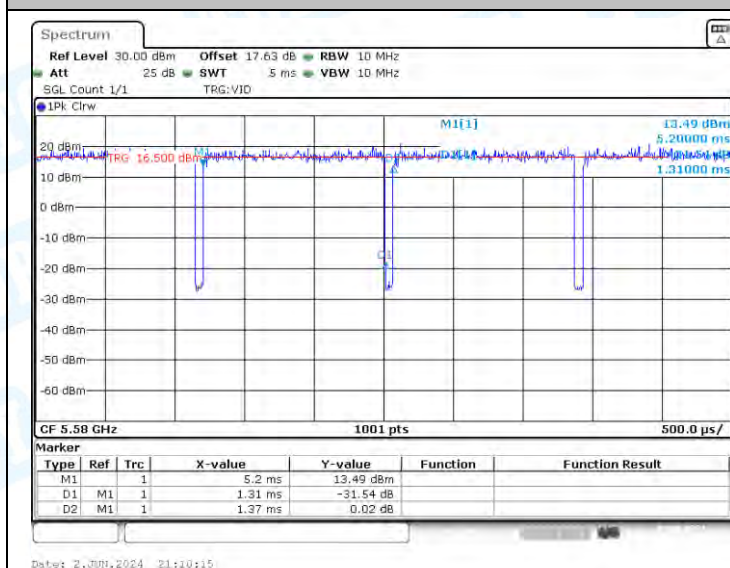
NTNV-11N20-CDD-Ant2-5580
