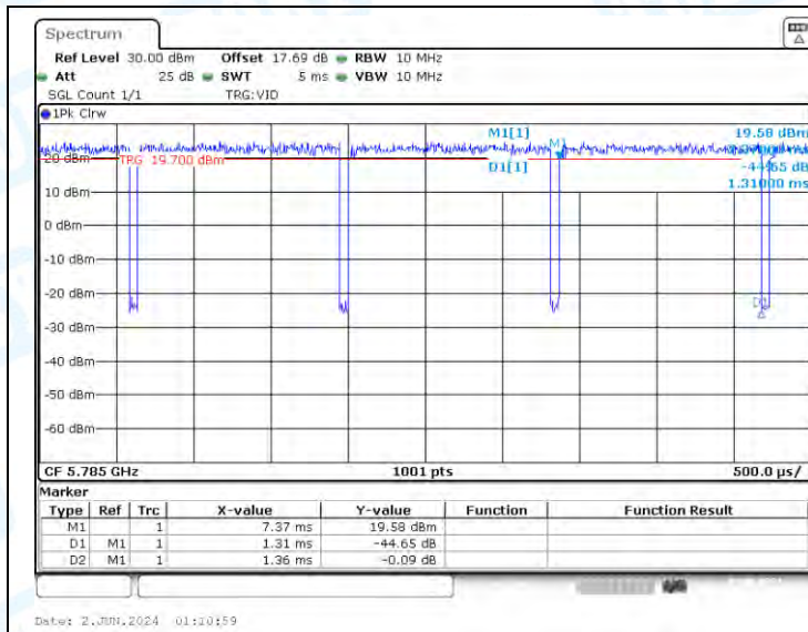
NTNV-11N20-CDD-Ant1-5785
