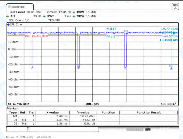
NTNV-11N20-CDD-Ant3-5745
