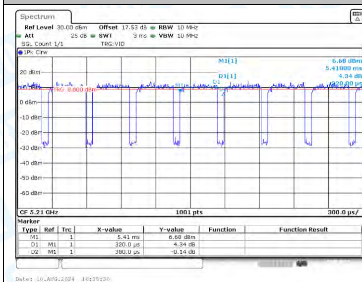
NTNV-11AC80-CDD-Ant3-5210
