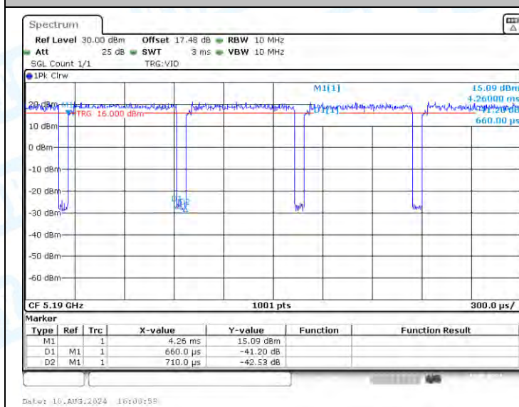
NTNV-11AC40-CDD-Ant2-5190
