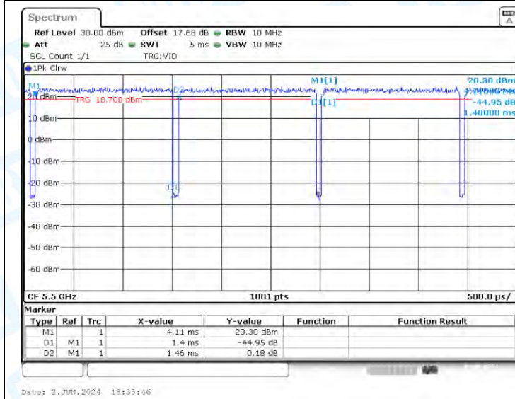
NTNV-11A-Ant3-5500
