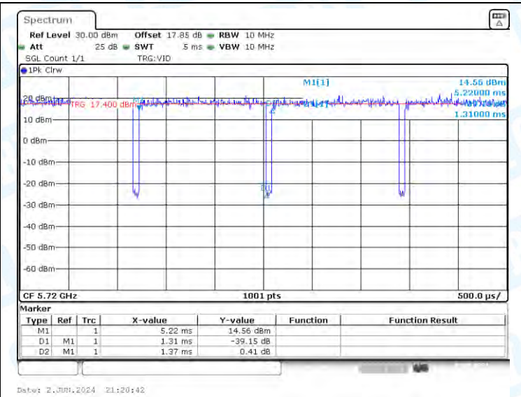
NTNV-11N20-CDD-Ant2-5720
