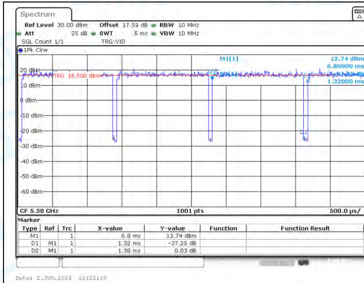
NTNV-11AC20-CDD-Ant1-5580
