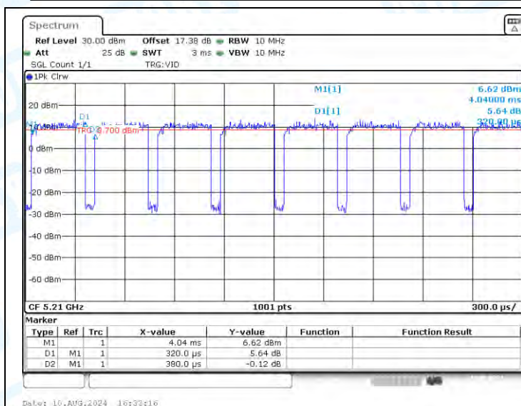
NTNV-11AC80-CDD-Ant1-5210
