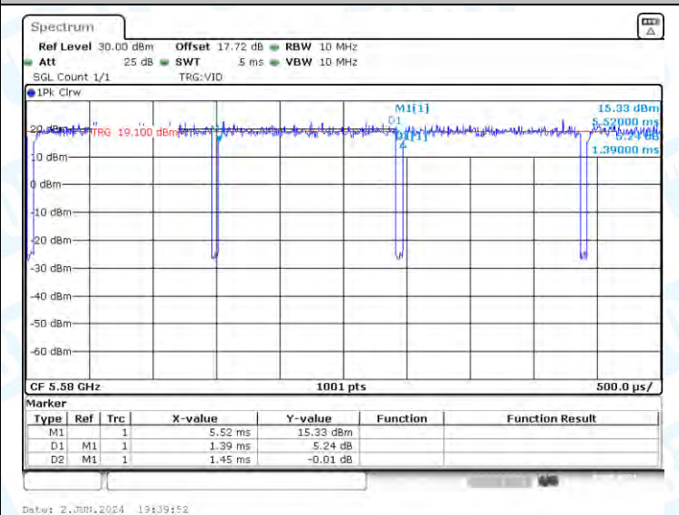
NTNV-11A-CDD-Ant3-5580
