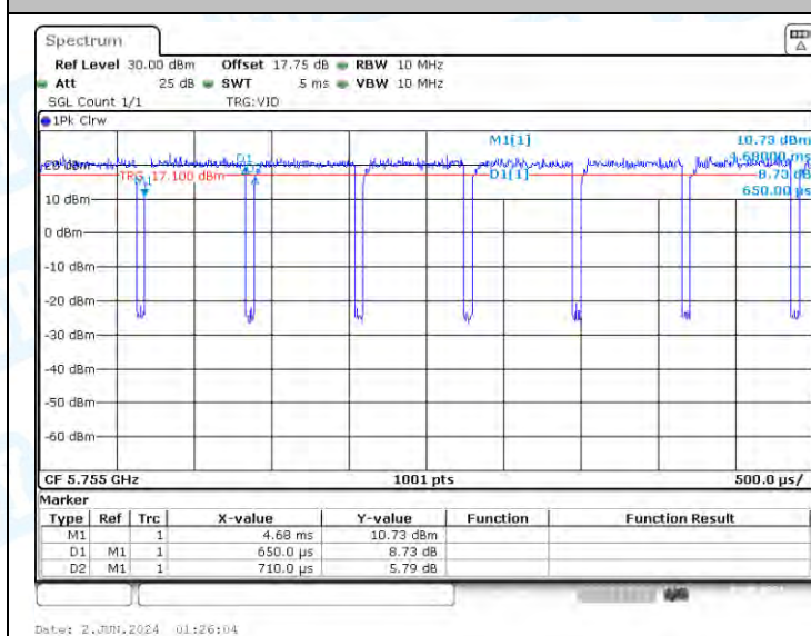
NTNV-11N40-CDD-Ant2-5755
