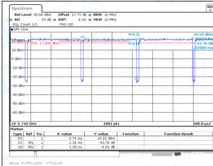
NTNV-11AC20-CDD-Ant1-5745
