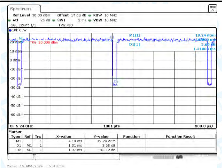
NTNV-11AC20-CDD-Ant3-5240
