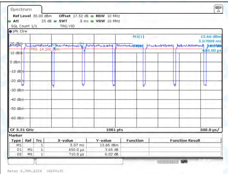
NTNV-11AC40-CDD-Ant2-5310
