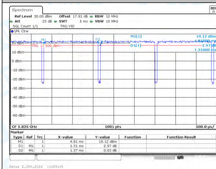
NTNV-11AC20-CDD-Ant3-5825
