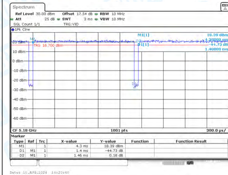
NTNV-11A-Ant3-5180
