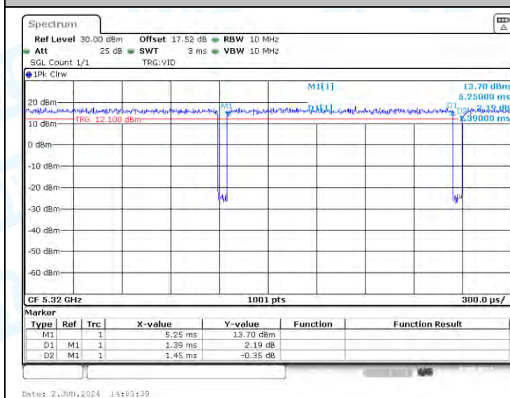
NTNV-11A-CDD-Ant2-5320
