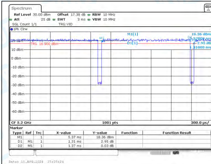
NTNV-11AC20-CDD-Ant1-5200
