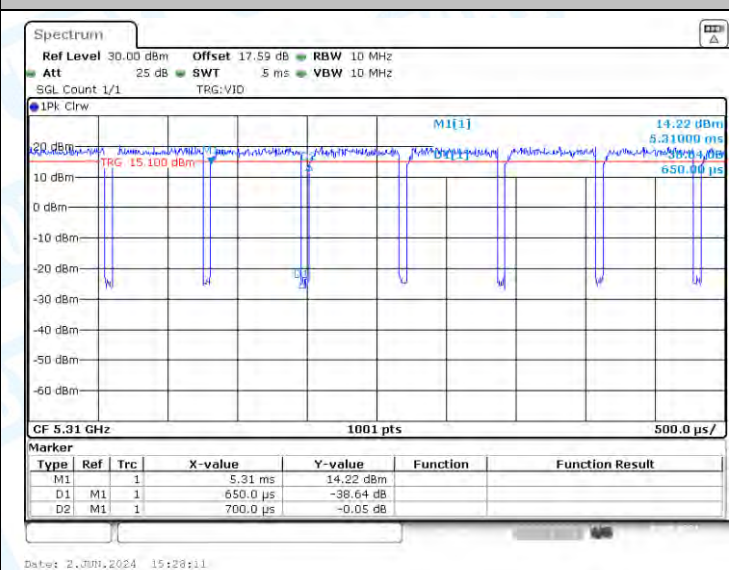
NTNV-11N40-CDD-Ant3-5310
