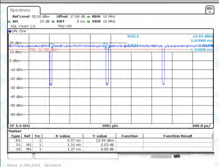
NTNV-11AC20-CDD-Ant3-5500
