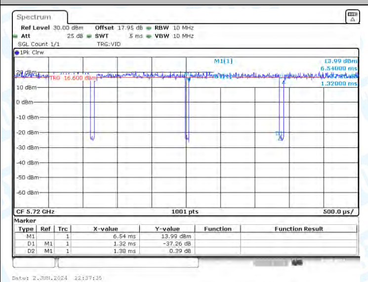
NTNV-11AC20-CDD-Ant3-5720
