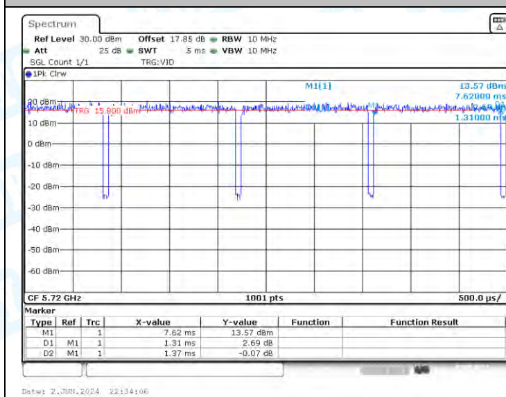
NTNV-11AC20-CDD-Ant2-5720
