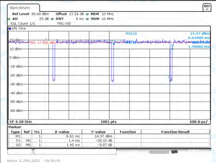
NTNV-11A-CDD-Ant1-5580
