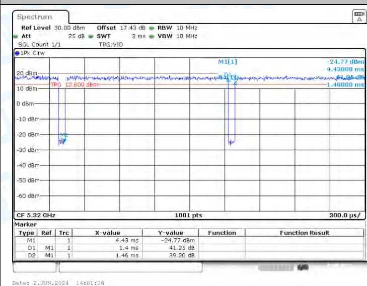
NTNV-11A-CDD-Ant1-5320
