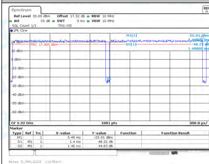
NTNV-11A-Ant2-5320
