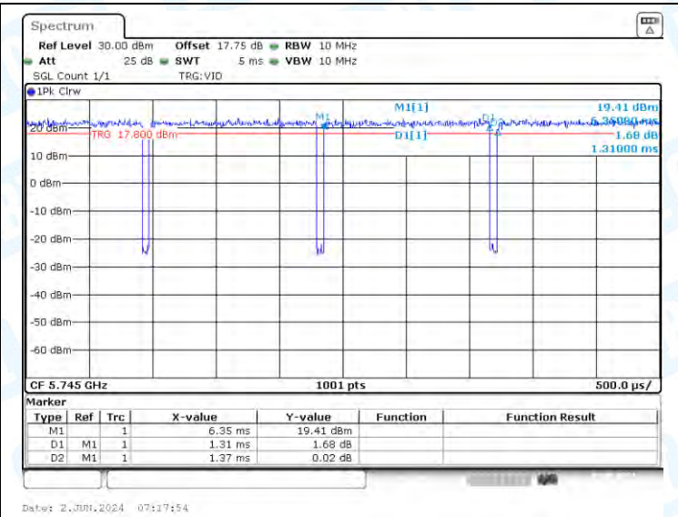
NTNV-11AC20-CDD-Ant2-5745
