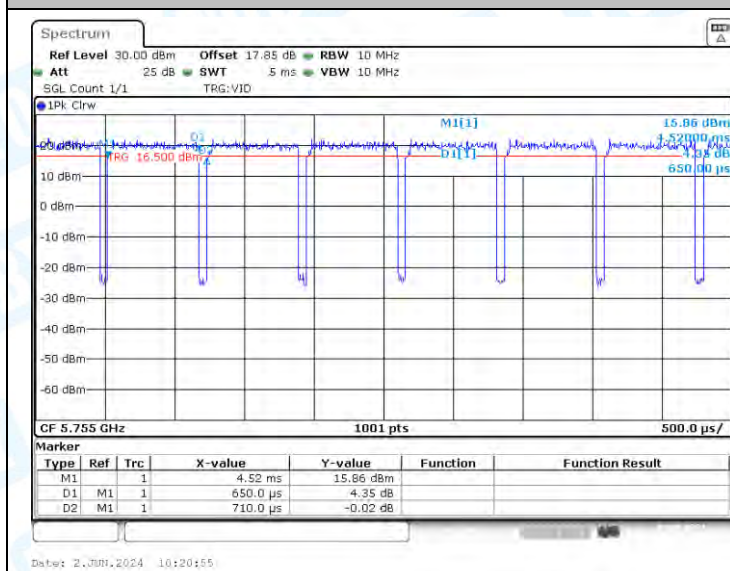
NTNV-11AC40-CDD-Ant3-5755
