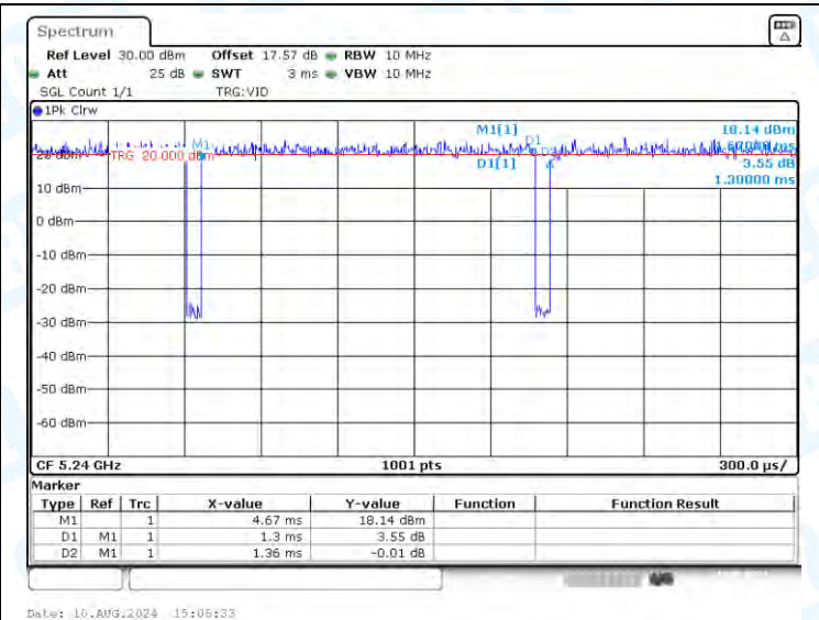
NTVN-11N20-CDD-Ant2-5240
