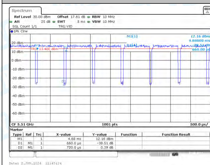
NTNV-11AC40-CDD-Ant2-5510
