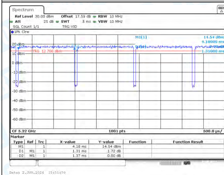
NTNV-11AC20-CDD-Ant3-5320
