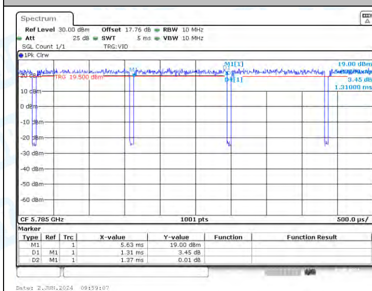
NTNV-11AC20-CDD-Ant2-5785
