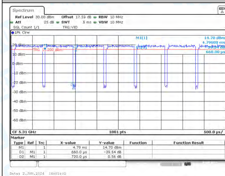
NTNV-11AC40-CDD-Ant3-5310
