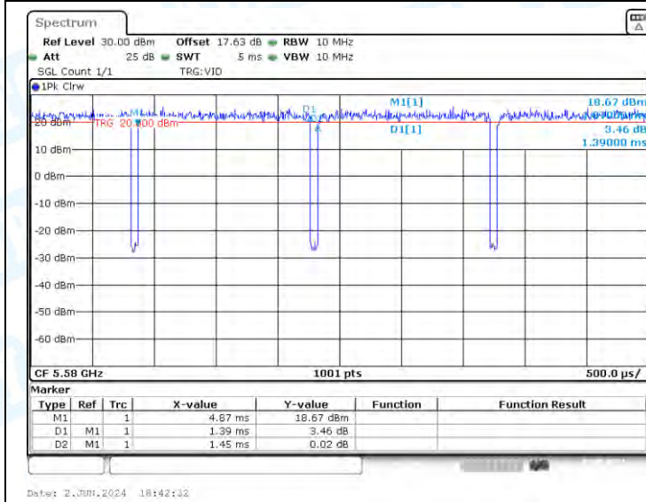
NTNV-11A-Ant2-5580
