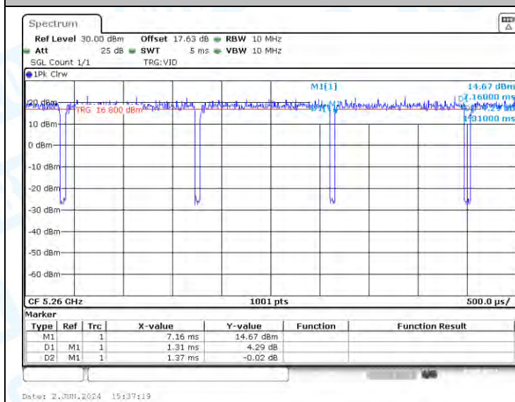
NTNV-11AC20-CDD-Ant3-5260
