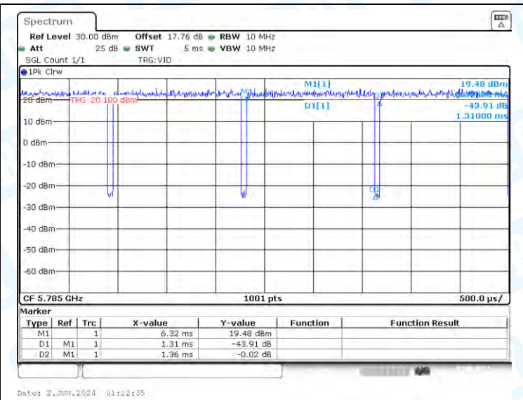
NTNV-11N20-CDD-Ant2-5785
