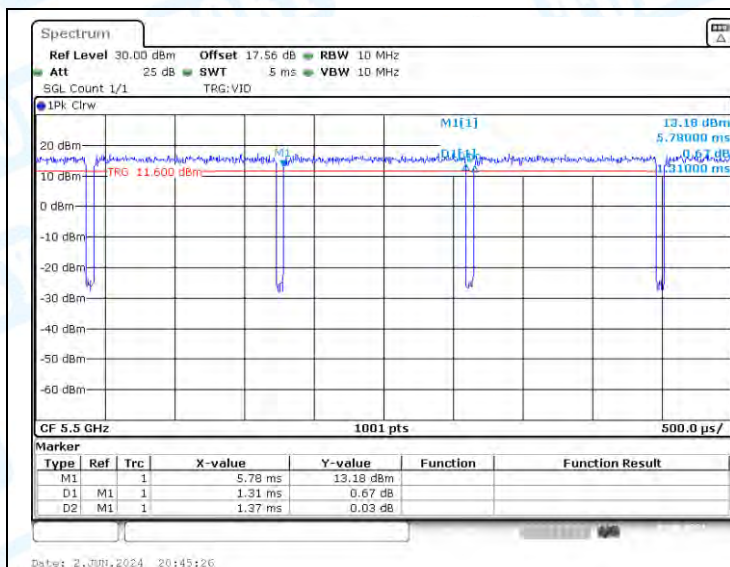
NTNV-11N20-CDD-Ant1-5500
