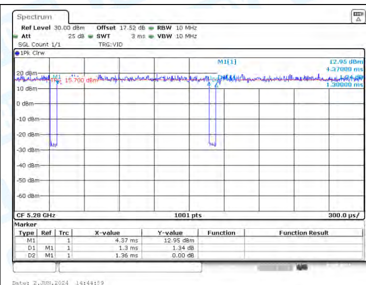
NTVN-11N20-CDD-Ant2-5280
