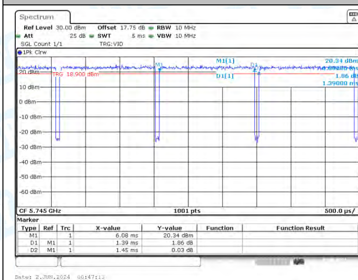
NTNV-11A-CDD-Ant2-5745
