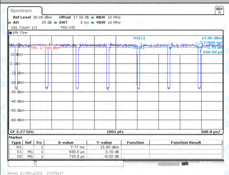
NTNV-11AC40-CDD-Ant3-5270
