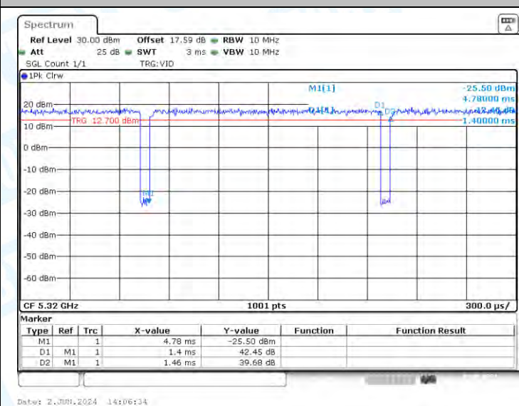
NTNV-11A-CDD-Ant3-5320
