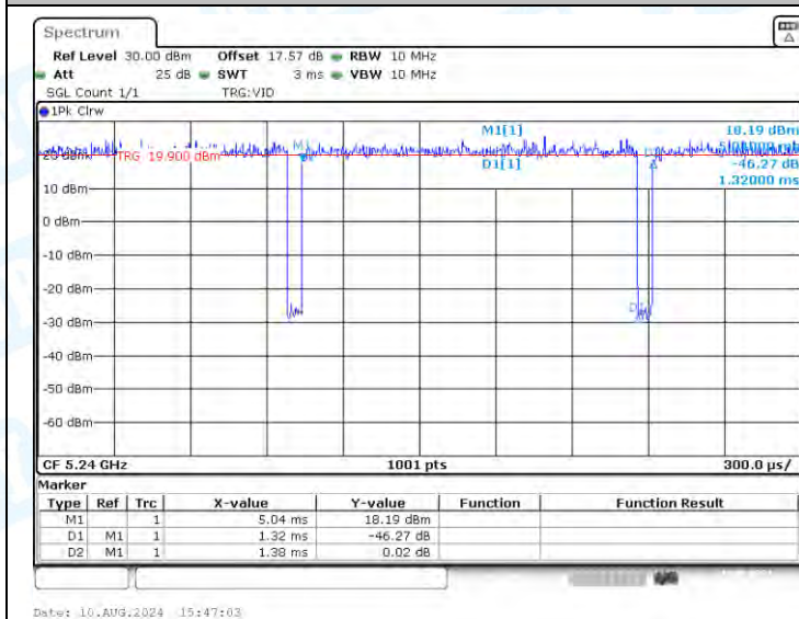
NTNV-11AC20-CDD-Ant2-5240
