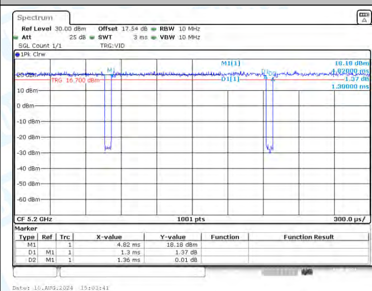
NTNV-11N20-CDD-Ant3-5200
