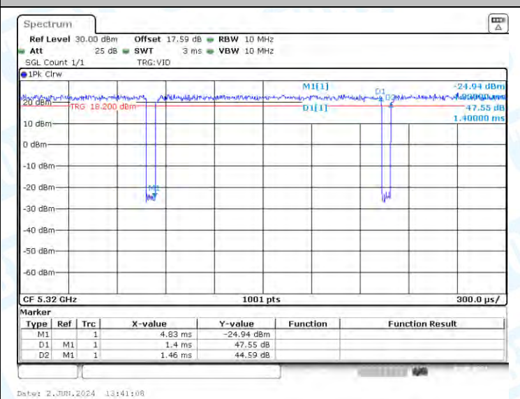
NTNV-11A-Ant3-5320
