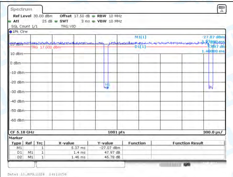
NTNV-11A-Ant2-5180
