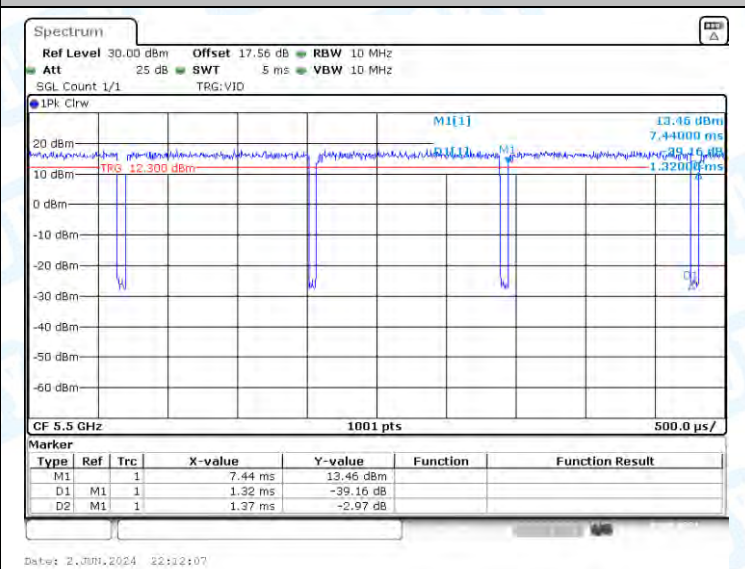
NTNV-11AC20-CDD-Ant1-5500
