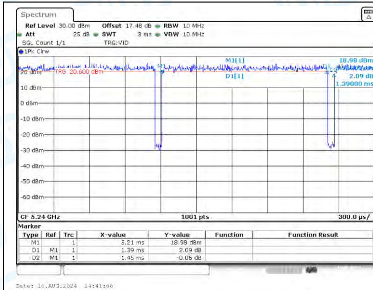
NTNV-11A-CDD-Ant1-5240
