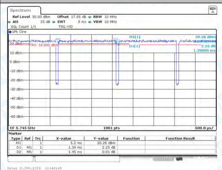
NTNV-11A-CDD-Ant3-5745
