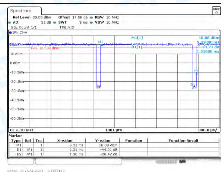
NTNV-11N20-CDD-Ant2-5180
