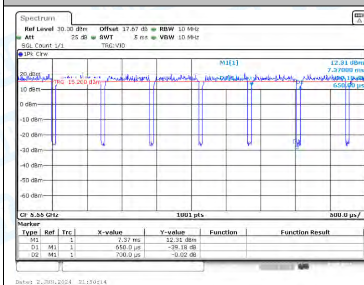
NTNV-11N40-CDD-Ant2-5550
