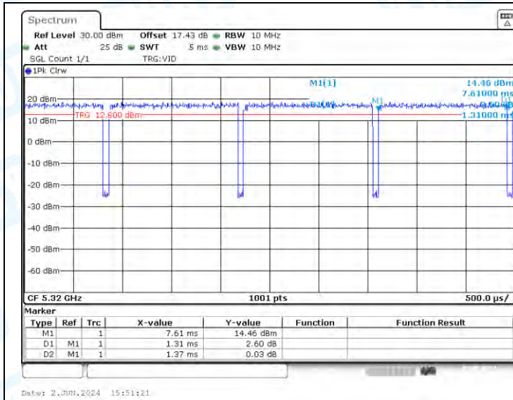
NTNV-11AC20-CDD-Ant1-5320
