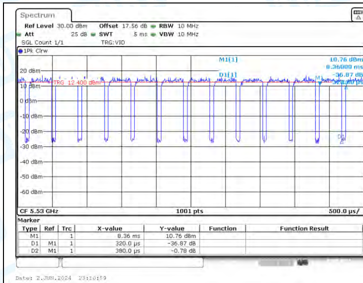
NTNV-11AC80-CDD-Ant1-5530
