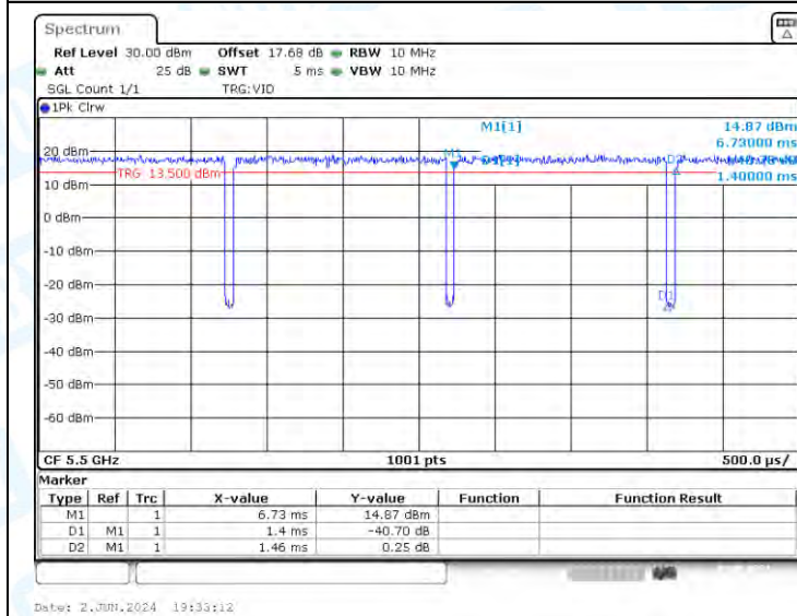
NTNV-11A-CDD-Ant3-5500
