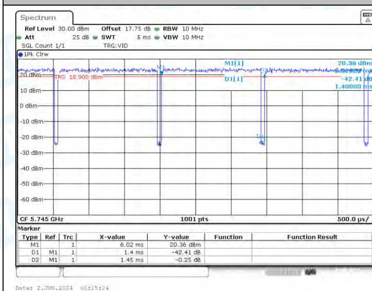
NTNV-11A-Ant2-5745
