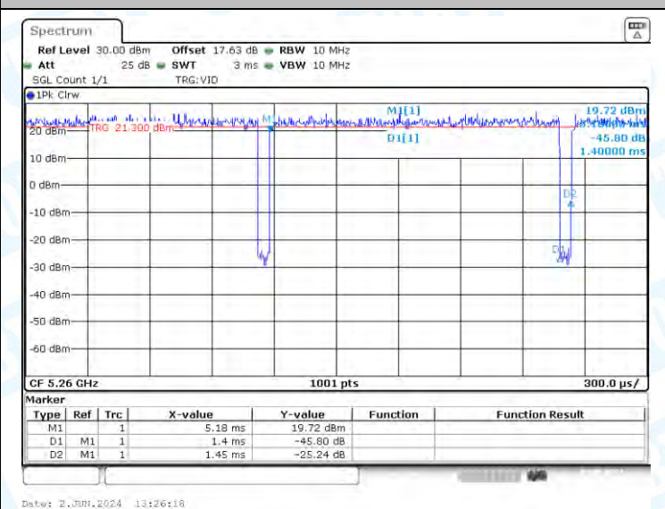
NTNV-11A-Ant3-5260
