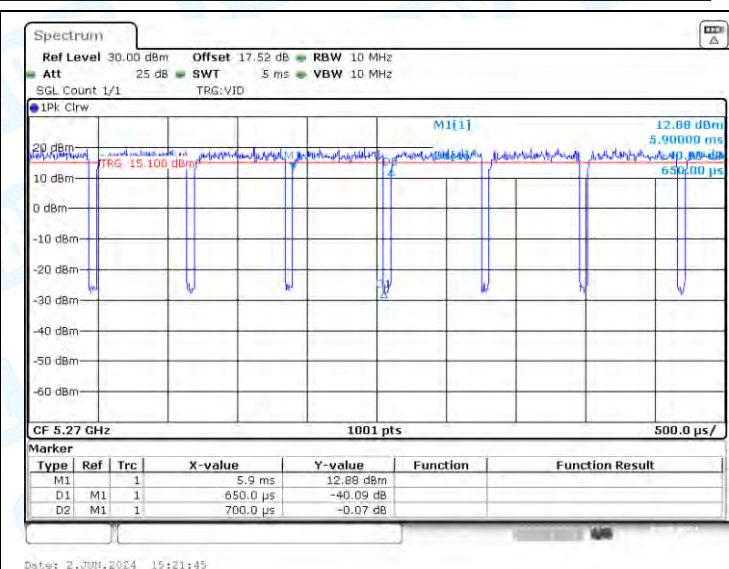
NTNV-11N40-CDD-Ant2-5270
