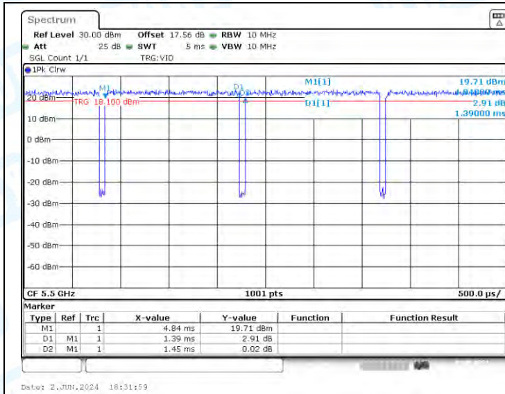
NTNV-11A-Ant1-5500
