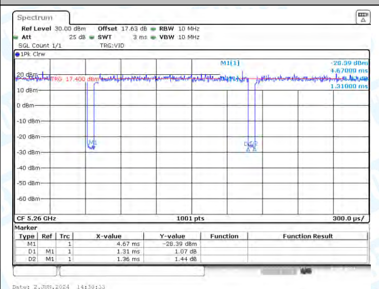
NTVN-11N20-CDD-Ant3-5260
