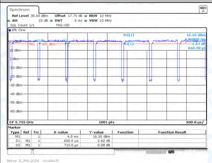
NTNV-11N40-CDD-Ant1-5755
