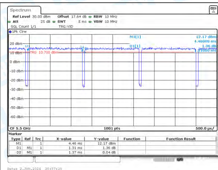
NTNV-11N20-CDD-Ant2-5500
