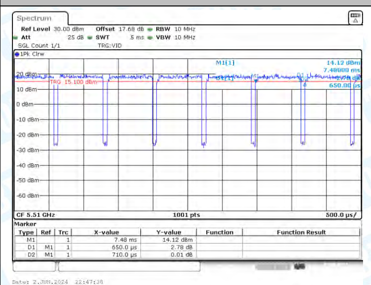
NTNV-11AC40-CDD-Ant3-5510
