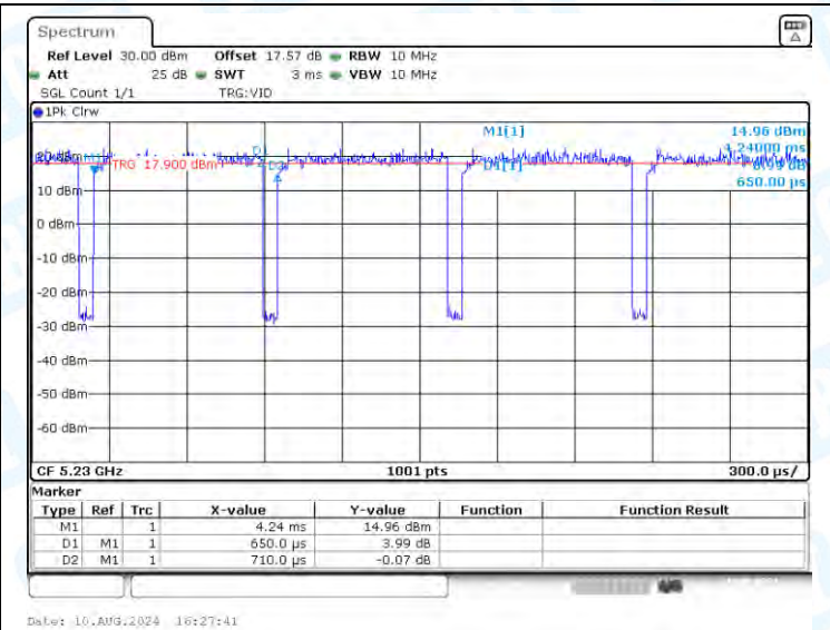
NTNV-11AC40-CDD-Ant2-5230
