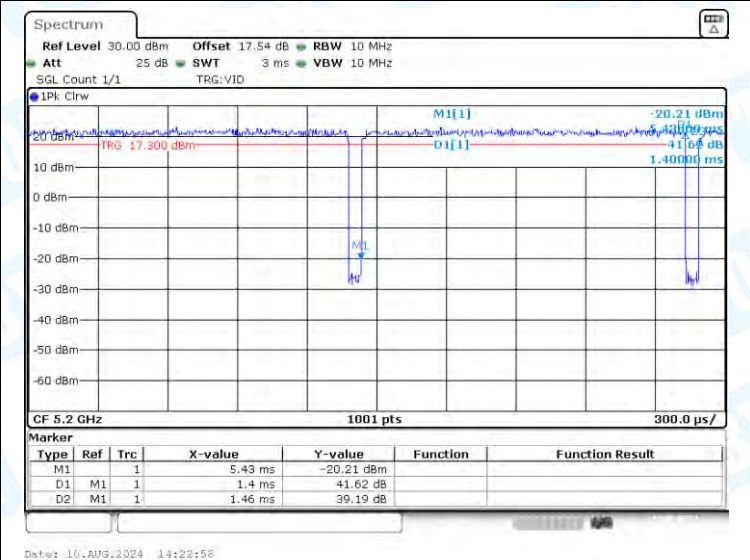
NTNV-11A-Ant3-5200
