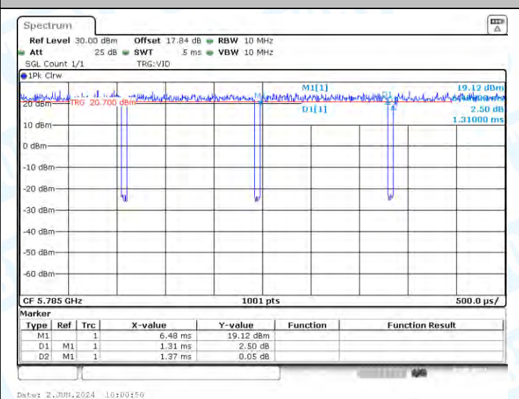
NTNV-11AC20-CDD-Ant3-5785
