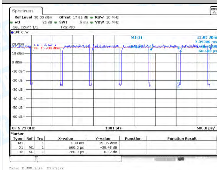
NTNV-11AC40-CDD-Ant2-5710
