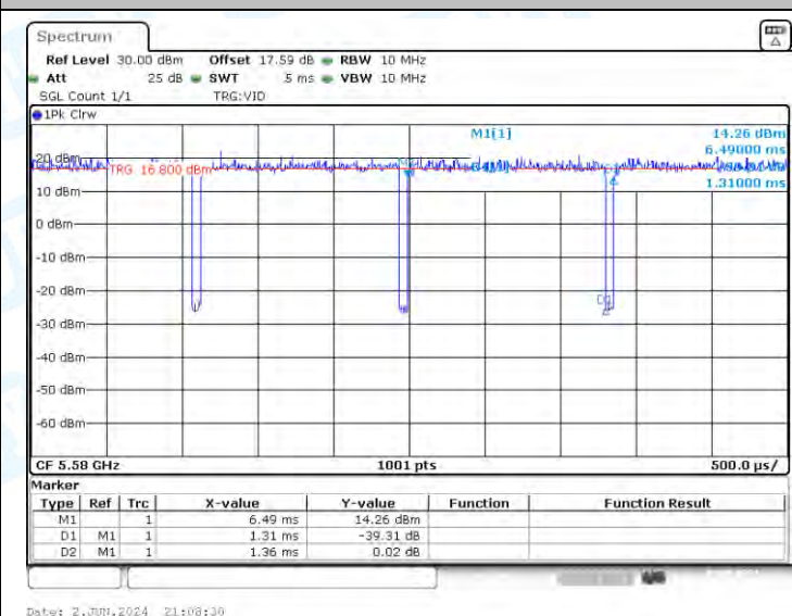
NTNV-11N20-CDD-Ant1-5580
