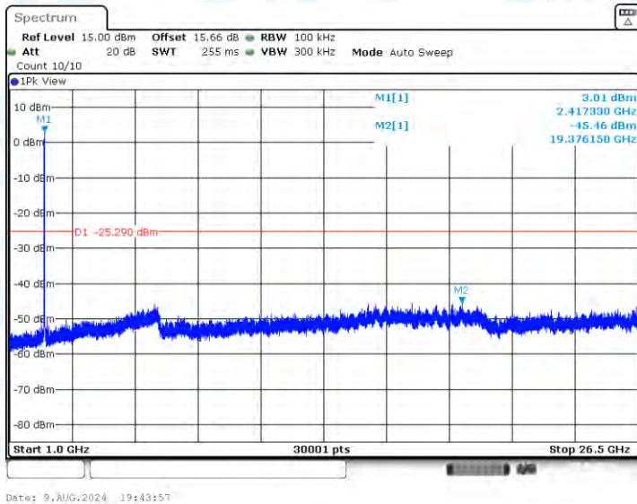
11AX20-CDD-Ant1-2412-1000~26500-PASS
