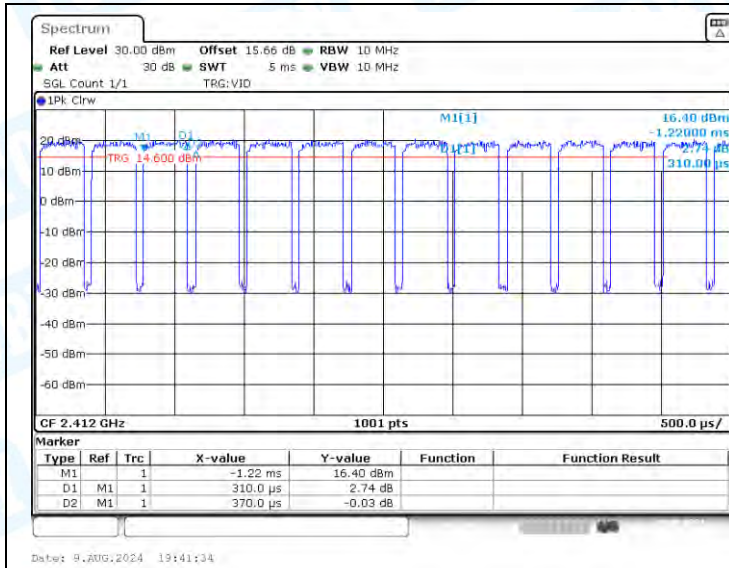
NTNV-11AX20-CDD-Ant1-2412
