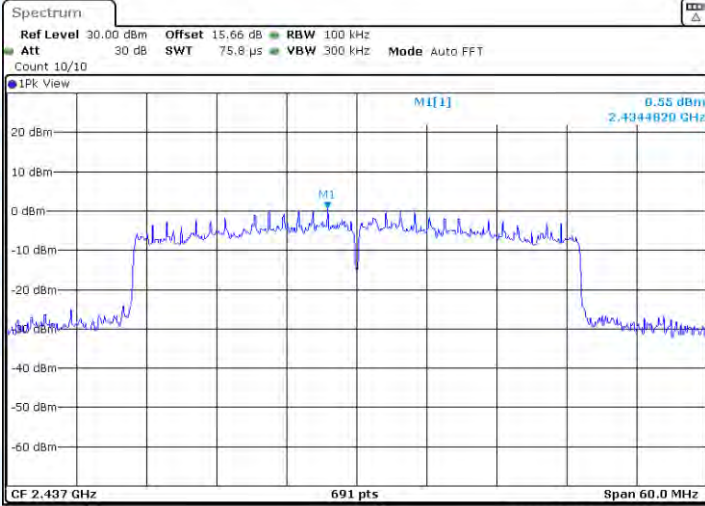
11AX40-CDD-Ant1-2437-0~Reference-PASS
