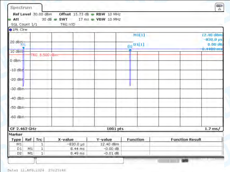
NTNV-11B-Ant2-2462
