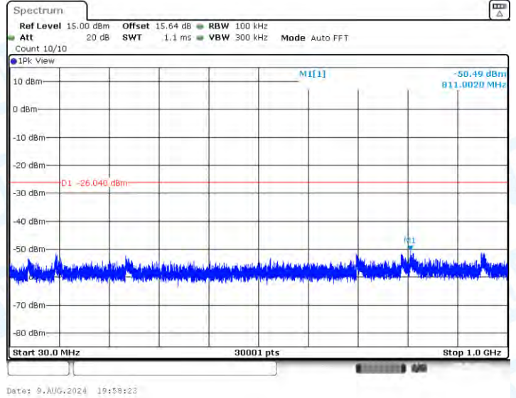
11AX20-CDD-Ant1-2462-30~1000-PASS
