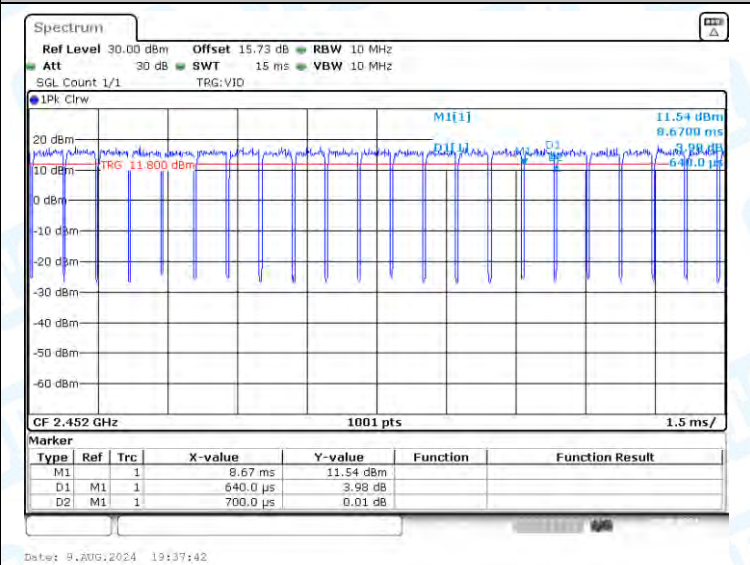
NTNV-11N40-CDD-Ant2-2452
