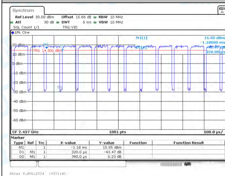
NTNV-11AX20-CDD-Ant1-2437
