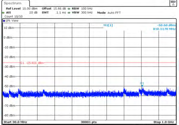
11AX20-CDD-Ant1-2437-30~1000-PASS
