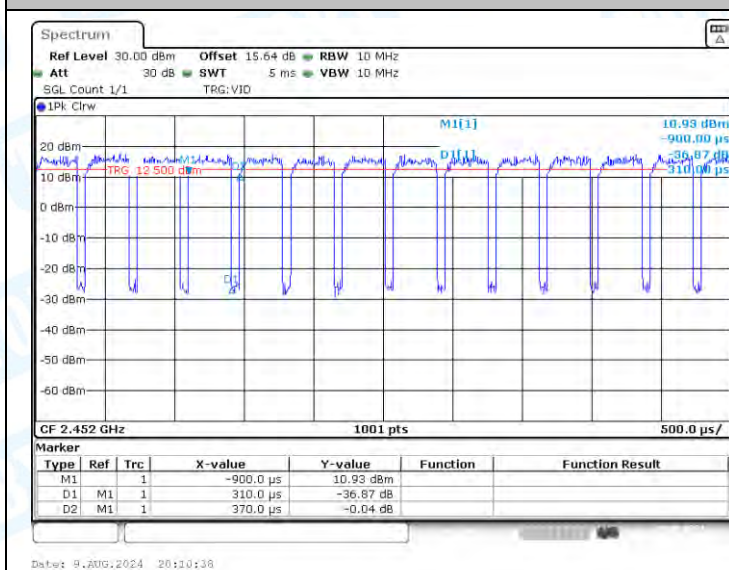
NTNV-11AX40-CDD-Ant1-2452
