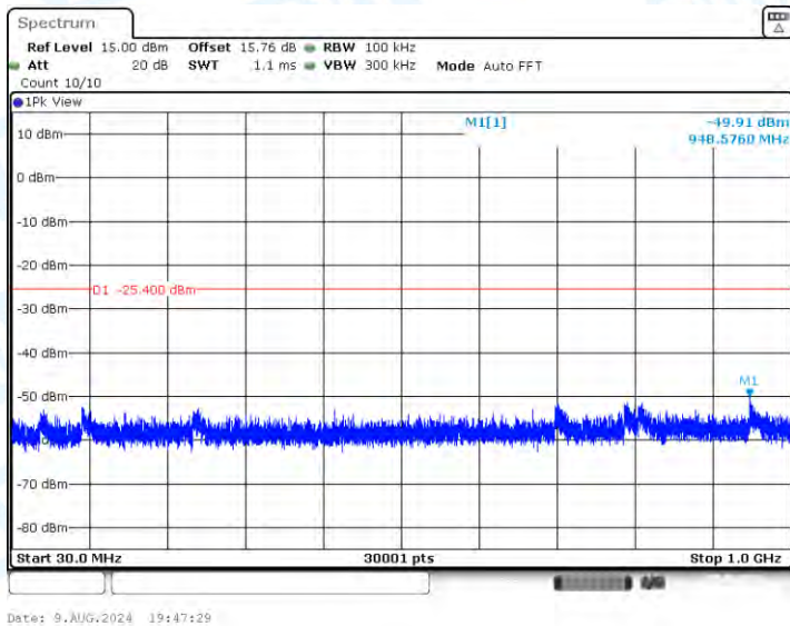
11AX20-CDD-Ant2-2412-30~1000-PASS
