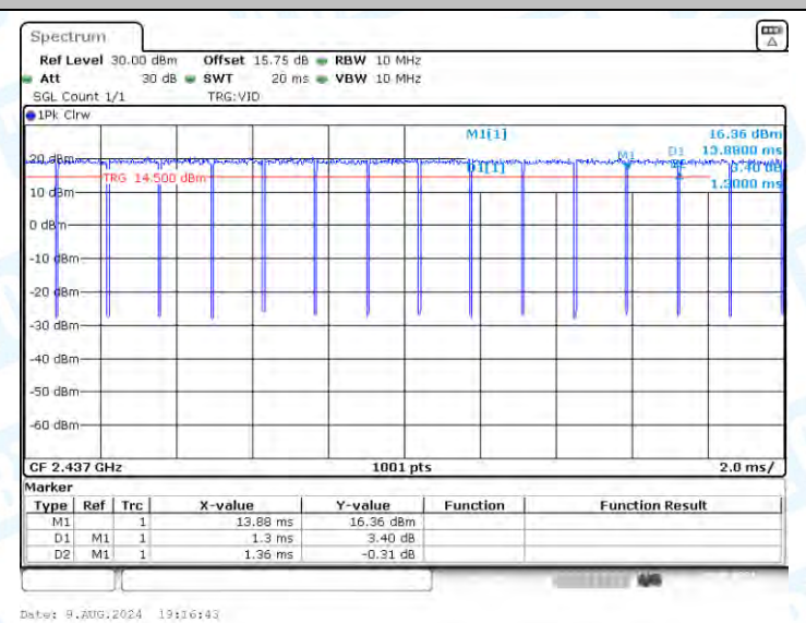
NTNV-11N20-CDD-Ant2-2437
