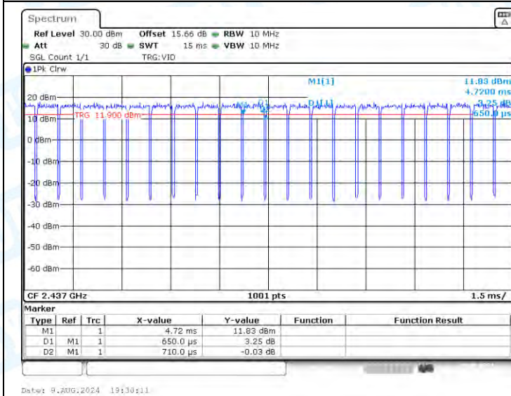
NTNV-11N40-CDD-Ant1-2437
