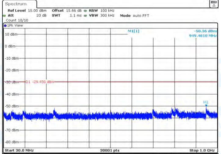
11AX40-CDD-Ant1-2437-30~1000-PASS
