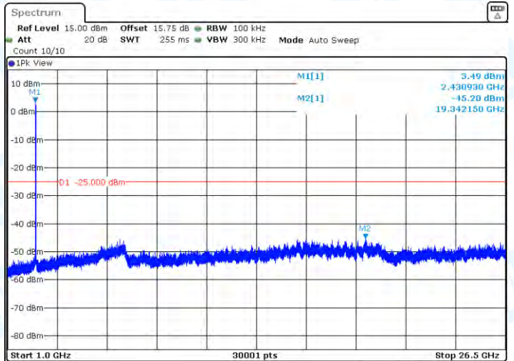
11G-CDD-Ant2-2437-0~Reference-PASS
