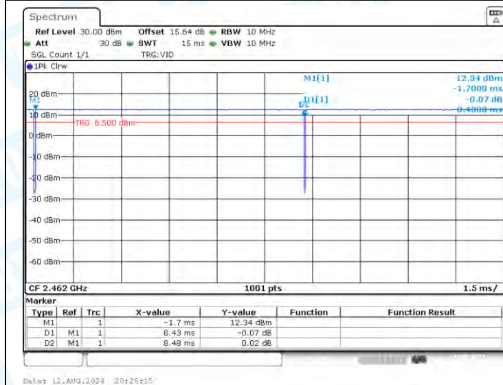
NTNV-11B-Ant1-2462
