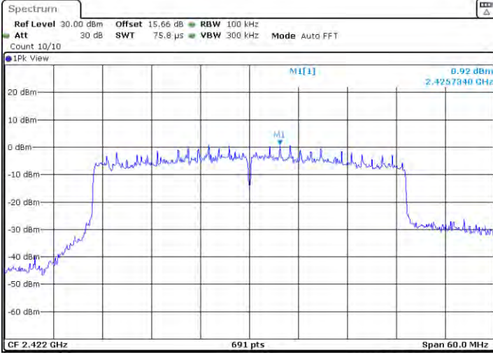
11AX40-CDD-Ant1-2422-0~Reference-PASS
