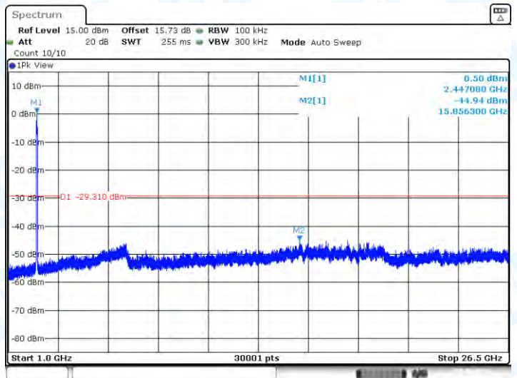
11AX40-CDD-Ant2-2452-0~Reference-PASS
