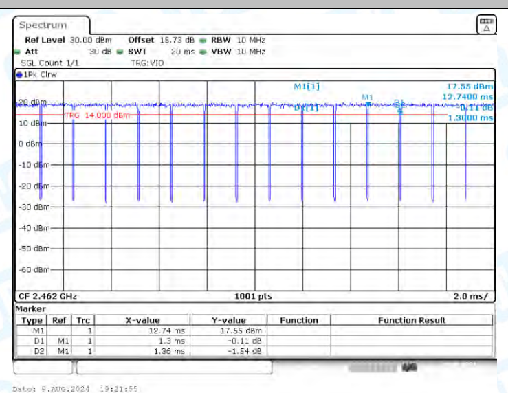
NTNV-11N20-CDD-Ant2-2462
