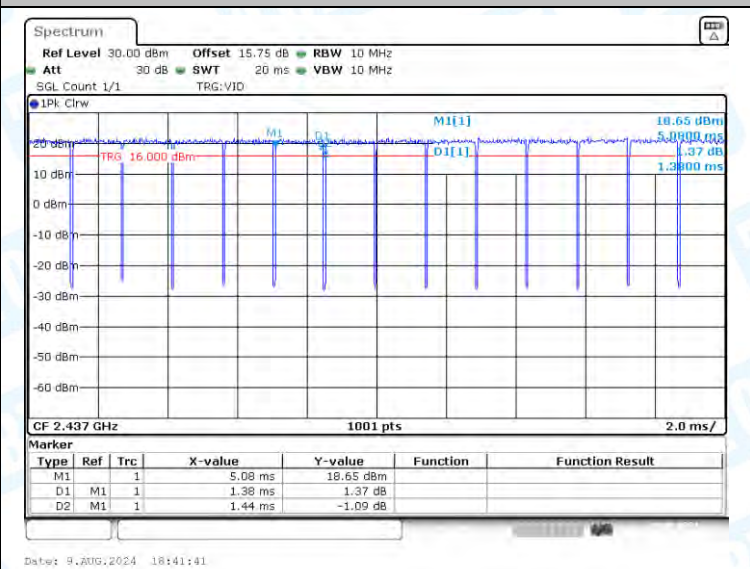
NTNV-11G-Ant2-2437
