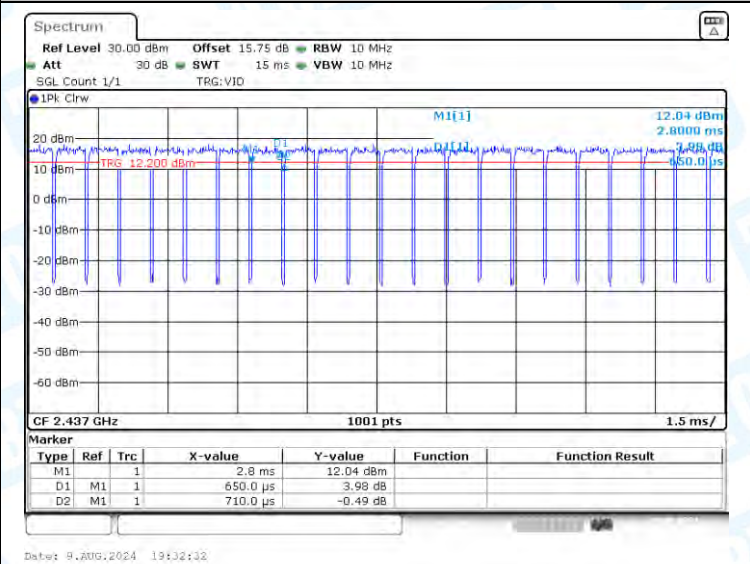
NTNV-11N40-CDD-Ant2-2437
