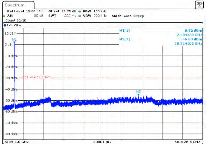
11AX40-CDD-Ant2-2437-0~Reference-PASS
