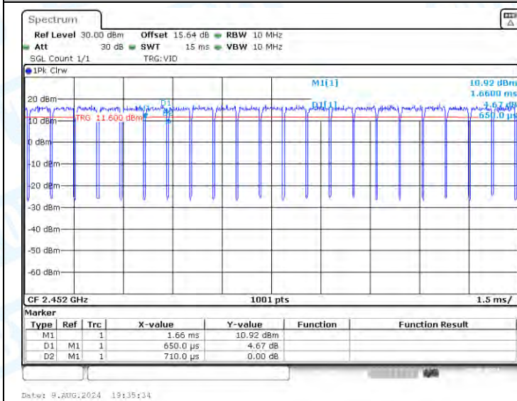
NTNV-11N40-CDD-Ant1-2452
