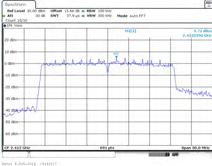
11AX20-CDD-Ant1-2412-0~Reference-PASS
