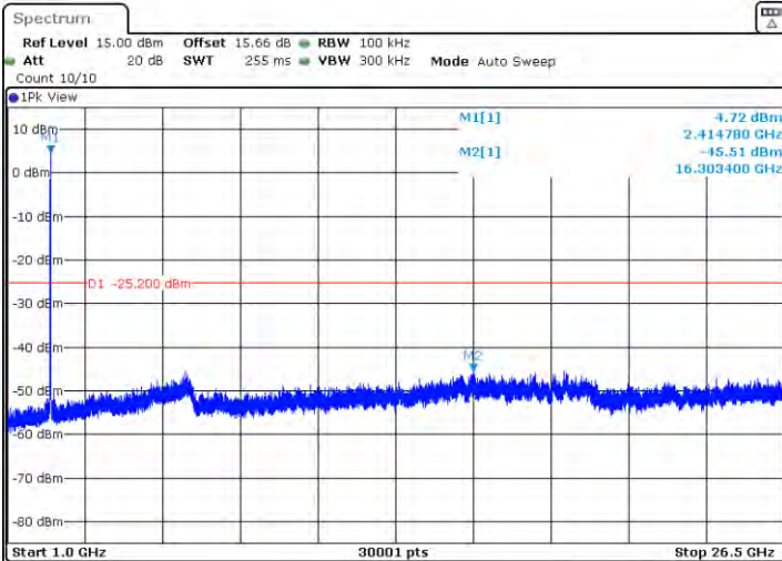
11G-CDD-Ant1-2412-0~Reference-PASS
