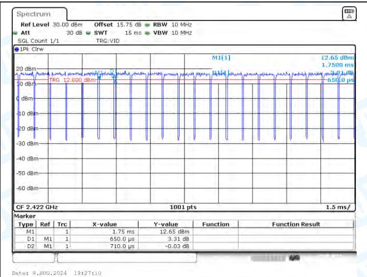
NTNV-11N40-CDD-Ant2-2422
