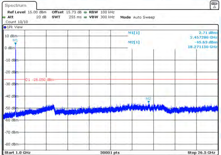
11N20-CDD-Ant2-2462-0~Reference-PASS
