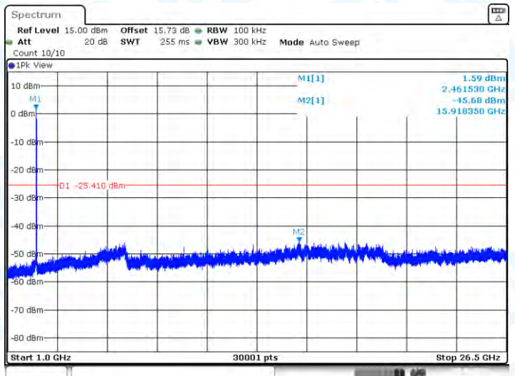
11G-CDD-Ant2-2462-0~Reference-PASS
