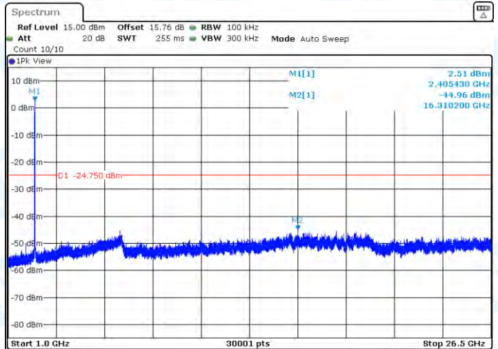
11G-CDD-Ant2-2412-0~Reference-PASS
