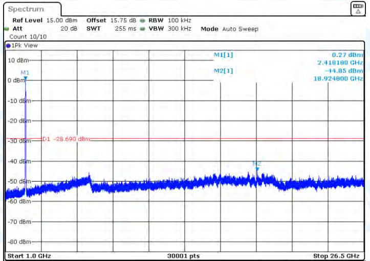
11N40-CDD-Ant2-2422-1000~26500-PASS
