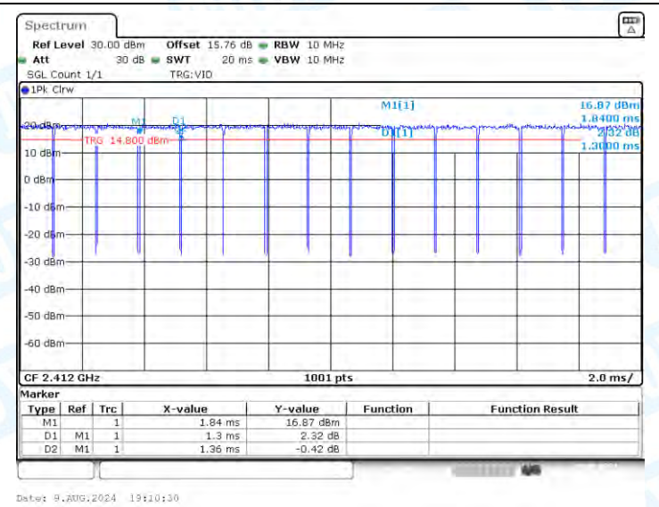
NTNV-11N20-CDD-Ant2-2412
