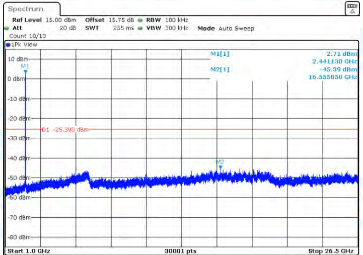
11N20-CDD-Ant2-2437-1000~26500-PASS
