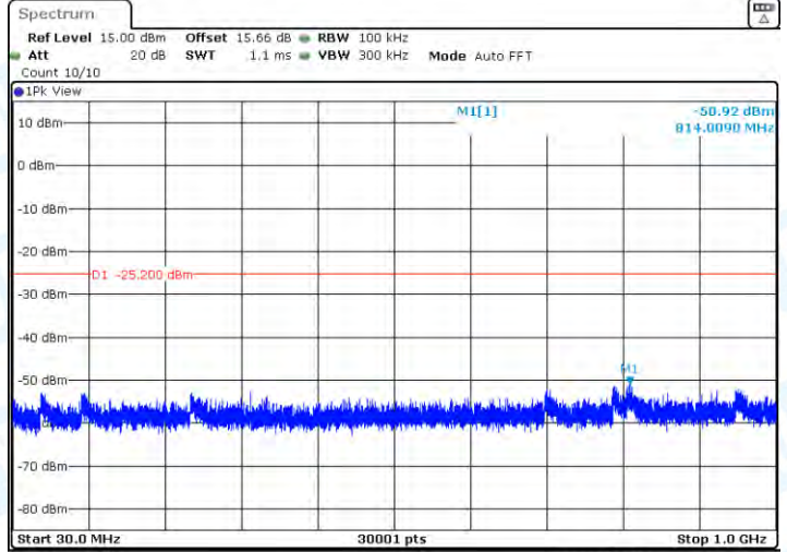
11G-CDD-Ant1-2412-30~1000-PASS
