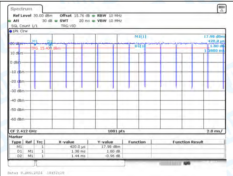
NTNV-11G-CDD-Ant2-2412
