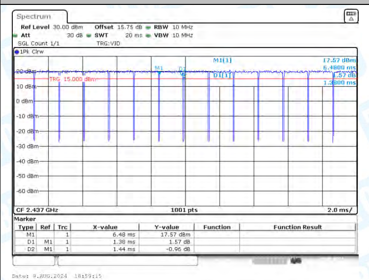
NTNV-11G-CDD-Ant2-2437
