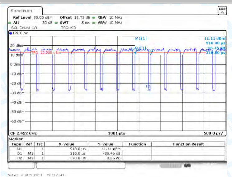
NTNV-11AX40-CDD-Ant2-2452
