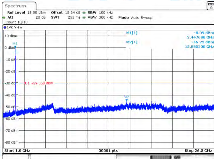
11AX40-CDD-Ant1-2452-0~Reference-PASS
