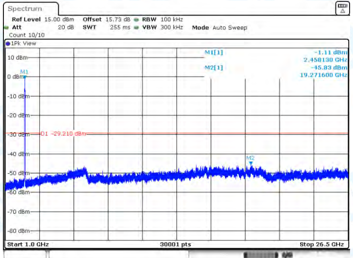
11N40-CDD-Ant2-2452-1000~26500-PASS
