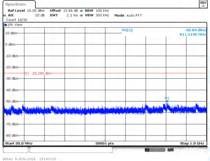
11AX20-CDD-Ant1-2412-30~1000-PASS
