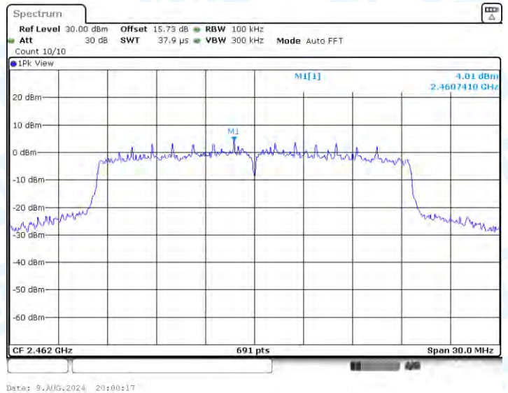
11AX20-CDD-Ant2-2462-0~Reference-PASS
