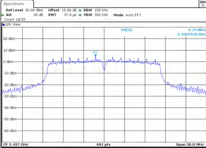
11G-CDD-Ant1-2437-0~Reference-PASS
