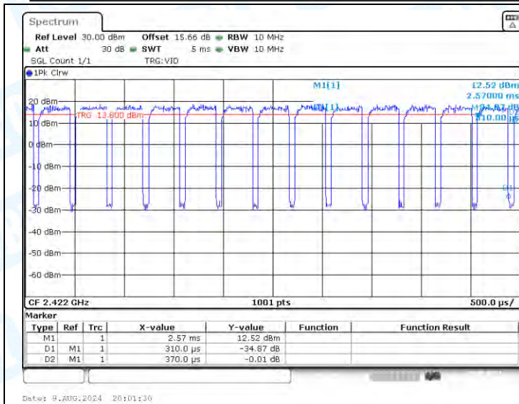
NTNV-11AX40-CDD-Ant1-2422
