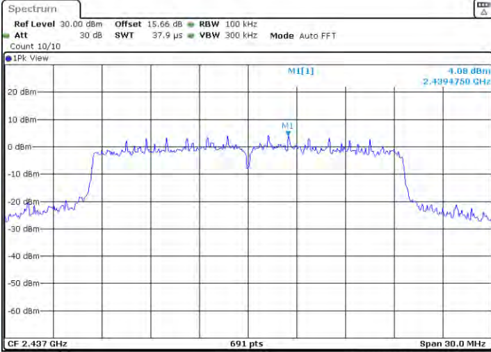
11AX20-CDD-Ant1-2437-0~Reference-PASS
