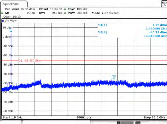
11G-CDD-Ant1-2462-0~Reference-PASS
