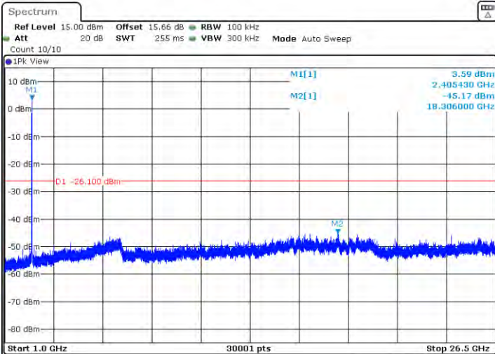
11N20-CDD-Ant1-2412-0~Reference-PASS
