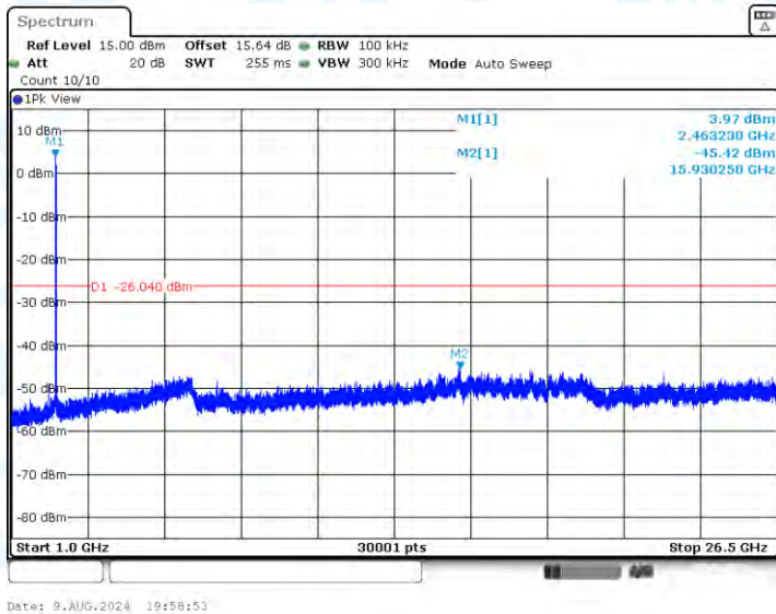
11AX20-CDD-Ant1-2462-1000~26500-PASS
