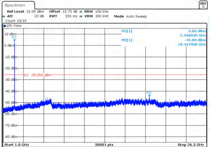
11AX20-CDD-Ant2-2437-0~Reference-PASS
