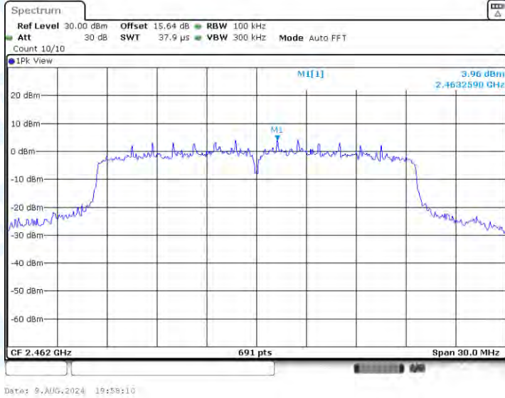
11AX20-CDD-Ant1-2462-0~Reference-PASS
