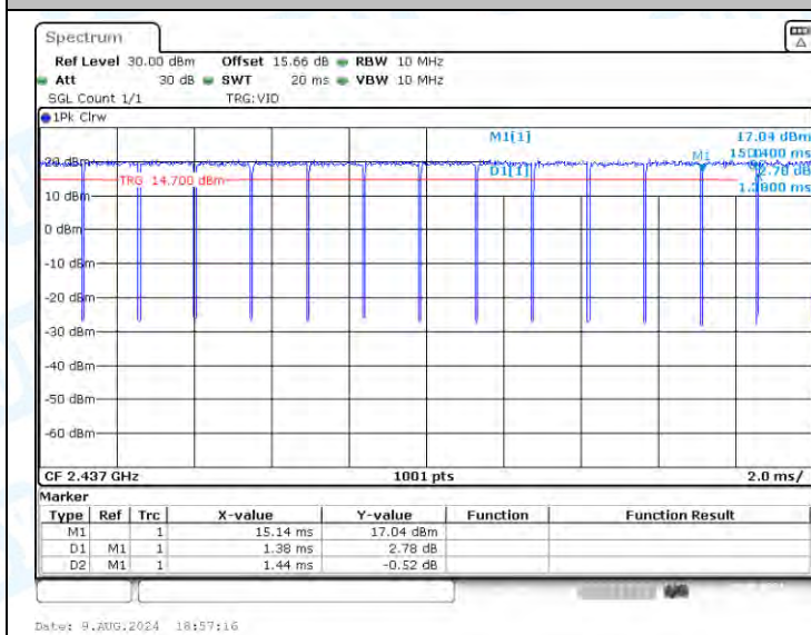
NTNV-11G-CDD-Ant1-2437
