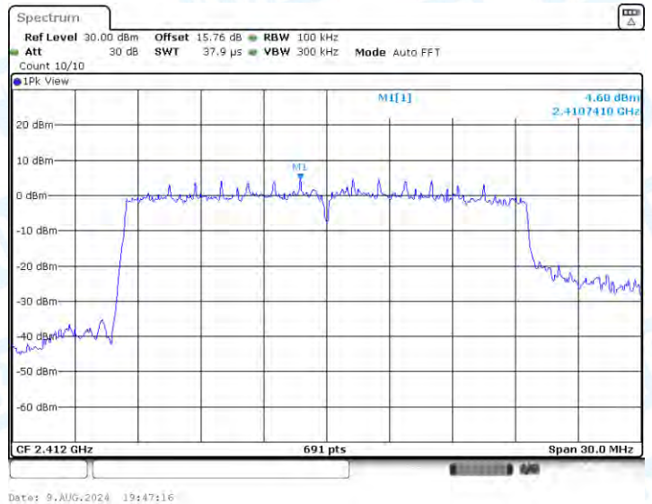
11AX20-CDD-Ant2-2412-0~Reference-PASS
