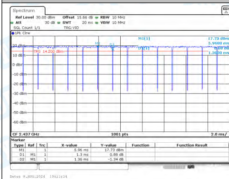
NTNV-11N20-CDD-Ant1-2437
