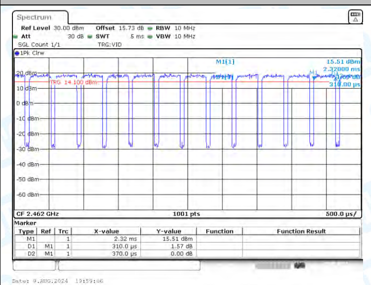
NTNV-11AX20-CDD-Ant2-2462
