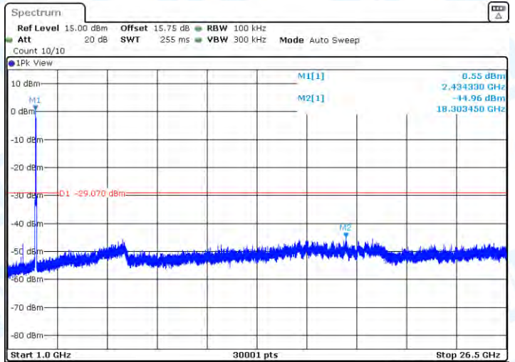
11N40-CDD-Ant2-2437-1000~26500-PASS
