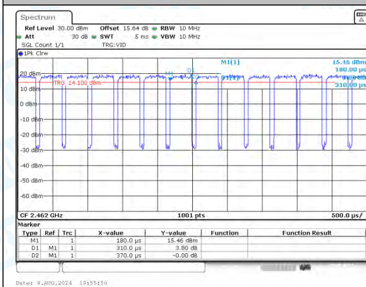
NTNV-11AX20-CDD-Ant1-2462
