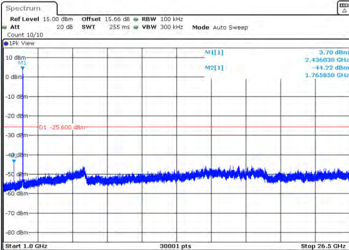
11N20-CDD-Ant1-2437-0~Reference-PASS
