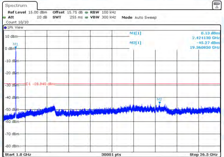
11AX40-CDD-Ant2-2422-0~Reference-PASS
