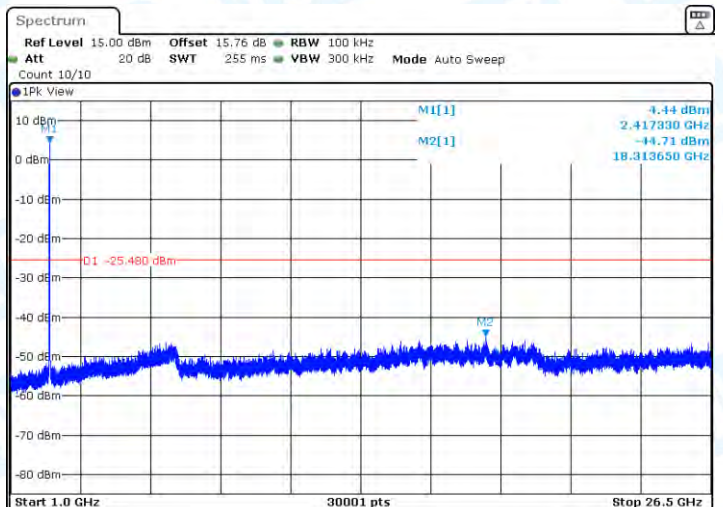
11N20-CDD-Ant2-2412-1000~26500-PASS
