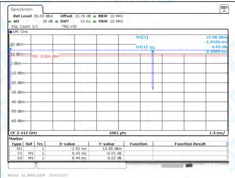
NTNV-11B-Ant2-2412
