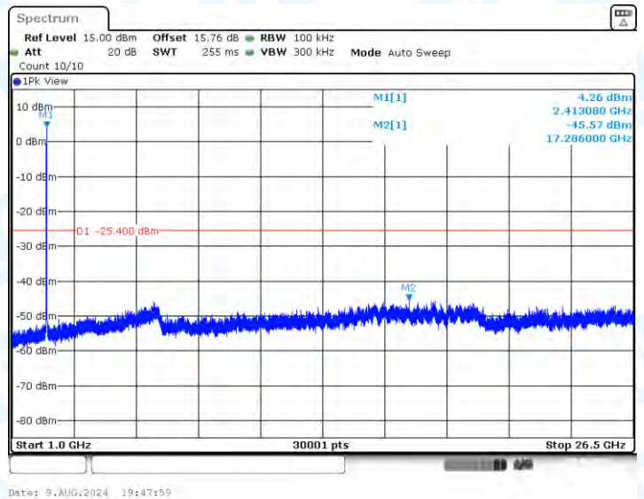
11AX20-CDD-Ant2-2412-1000~26500-PASS
