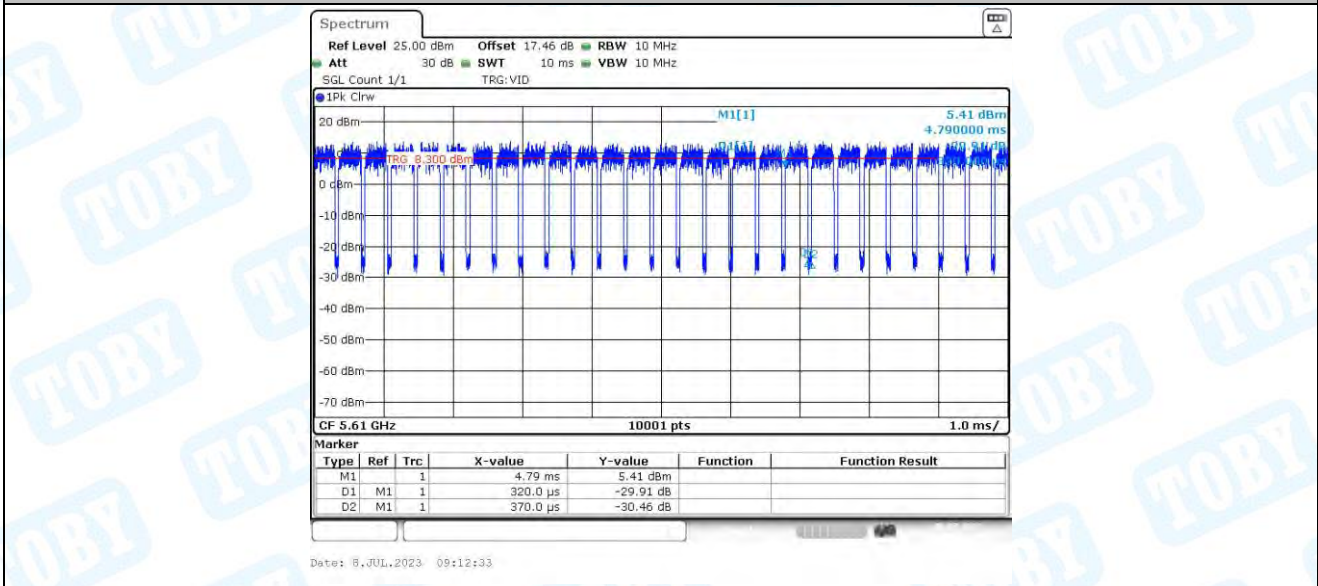
11AC80-CDD_Ant3_5610
