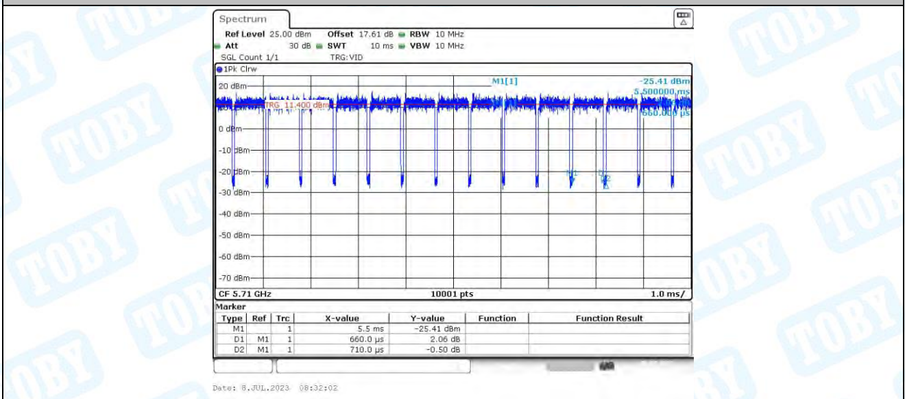
11AC40-CDD_Ant4_5710
