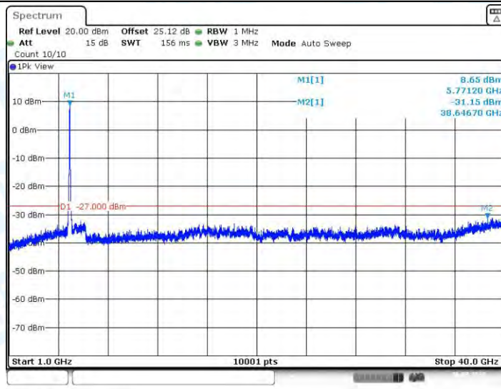
11AC80-CDD_Ant4_5775_1000~40000
