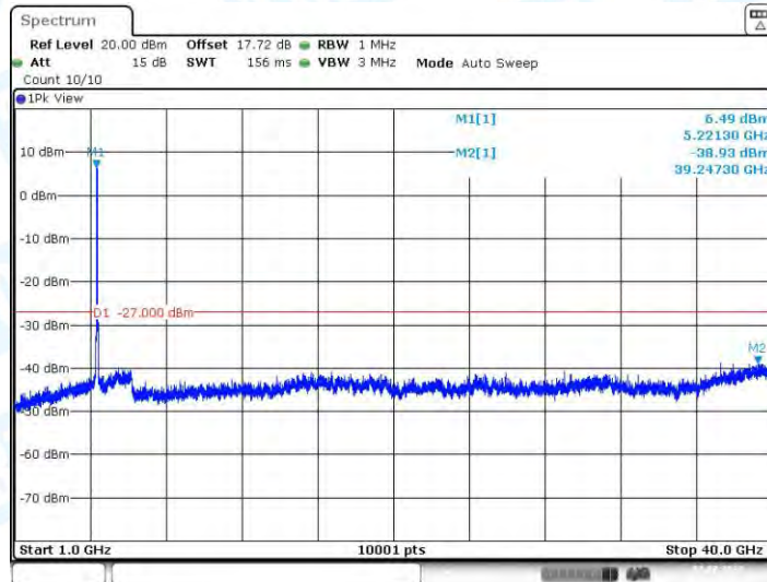
11N40-CDD_Ant4_5230_1000~40000
