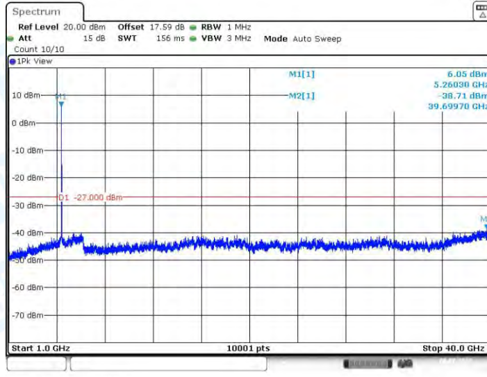
11AC20-CDD_Ant3_5260_1000~40000
