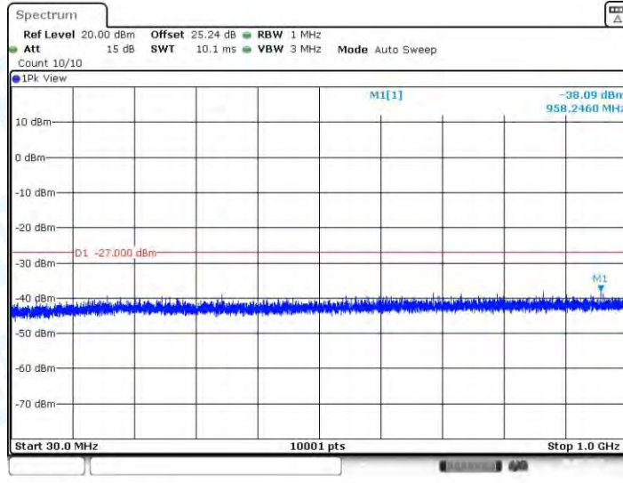
11AC20-CDD_Ant3_5825_30~1000
