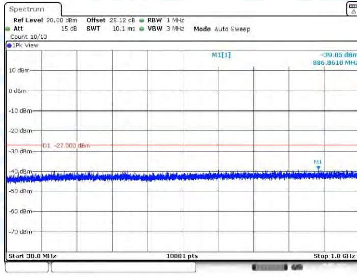
11AC80-CDD_Ant4_5775_30~1000
