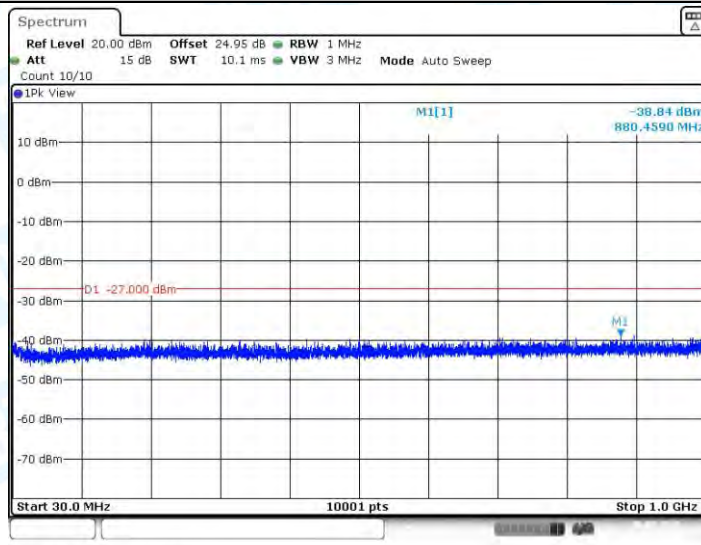
11AC40-CDD_Ant1_5795_30~1000
