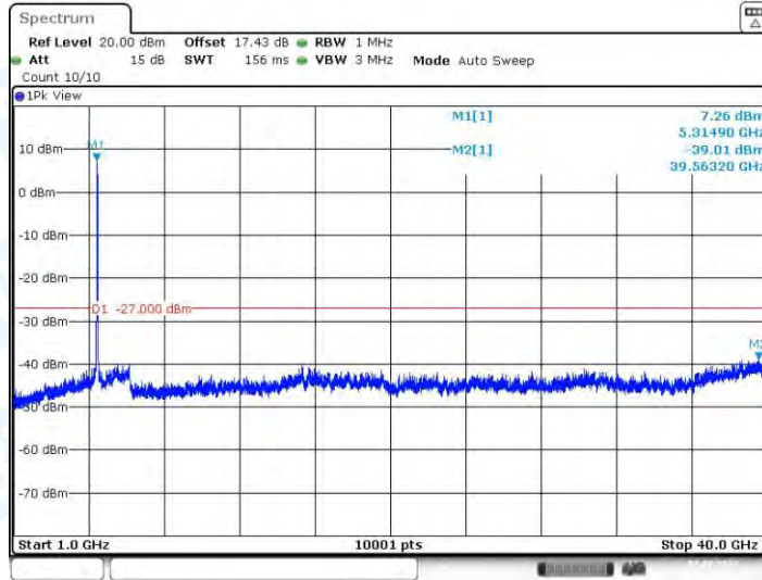
11N40-CDD_Ant2_5310_1000~40000
