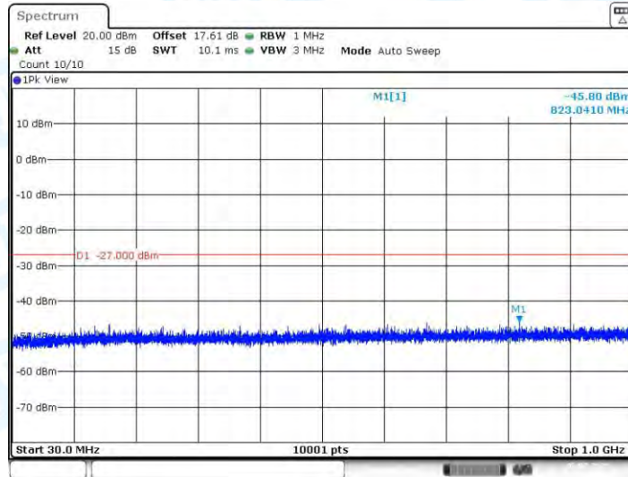
11N40-CDD_Ant3_5270_30~1000
