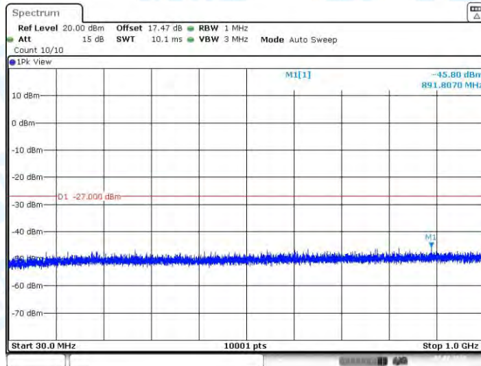
11N40-CDD_Ant4_5310_30~1000
