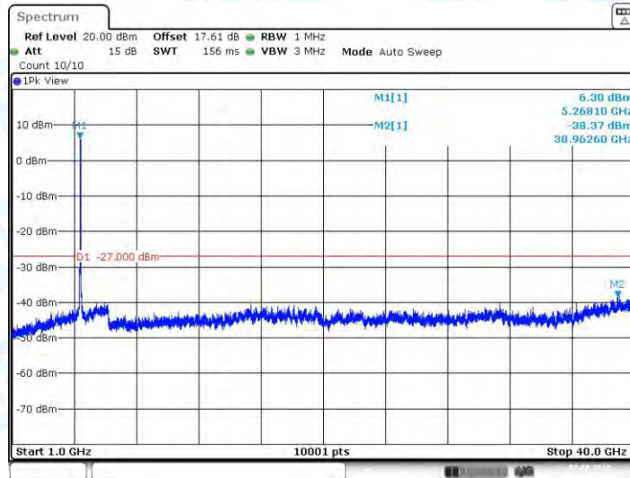
11N40-CDD_Ant3_5270_1000~40000
