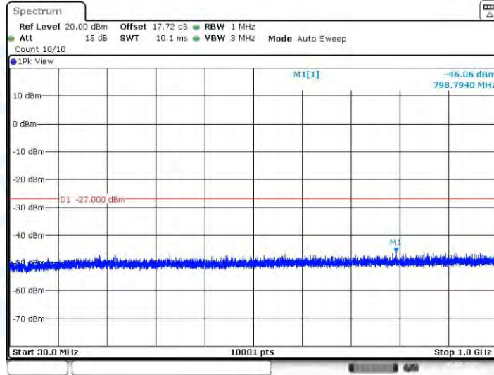
11N40-CDD_Ant4_5230_30~1000
