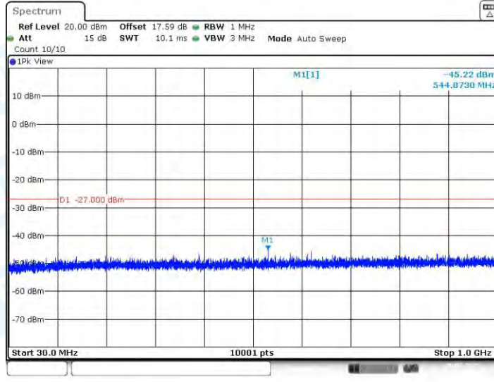
11AC20-CDD_Ant3_5260_30~1000
