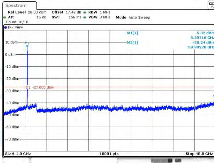
11N40-CDD_Ant3_5310_1000~40000
