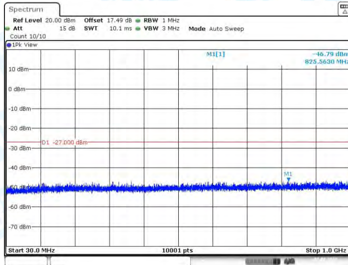
11N40-CDD_Ant3_5510_30~1000
