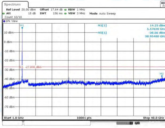
11A_Ant2_5580_1000~40000
