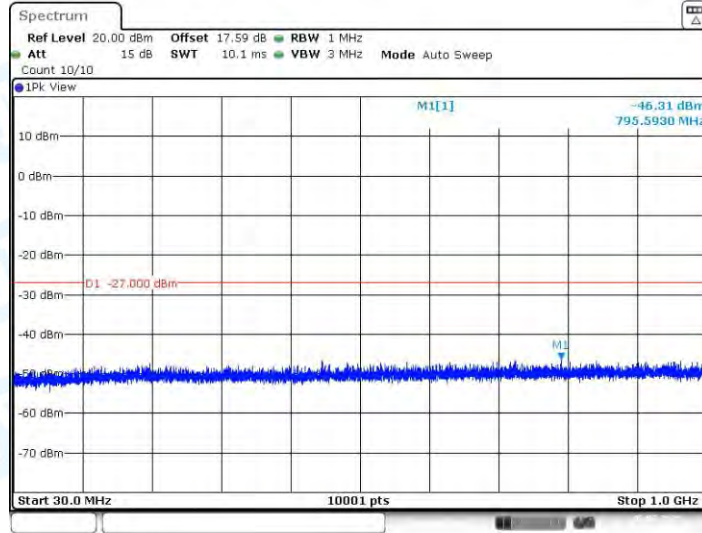
11N20-CDD_Ant3_5260_30~1000
