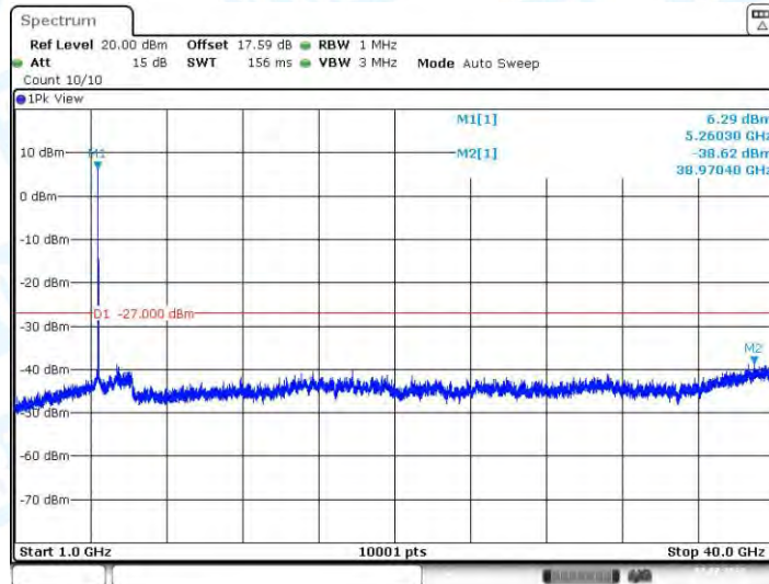
11N20-CDD_Ant3_5260_1000~40000
