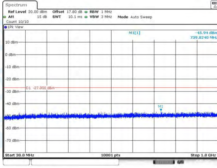
11N20-CDD_Ant4_5700_30~1000
