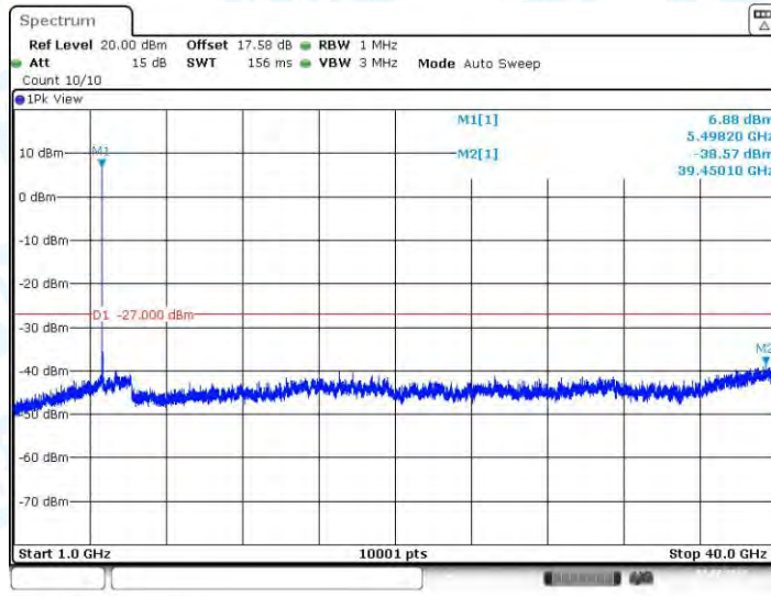
11N20-CDD_Ant3_5500_1000~40000
