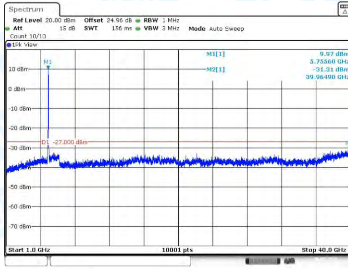
11N40-CDD_Ant2_5755_1000~40000
