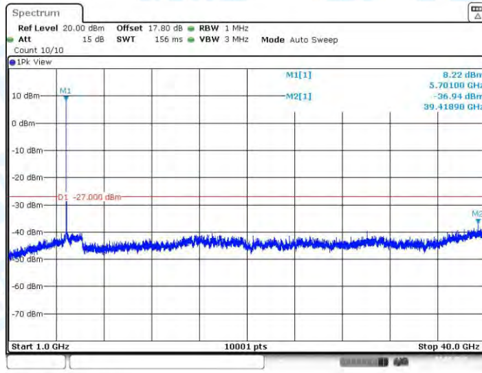
11N20-CDD_Ant4_5700_1000~40000
