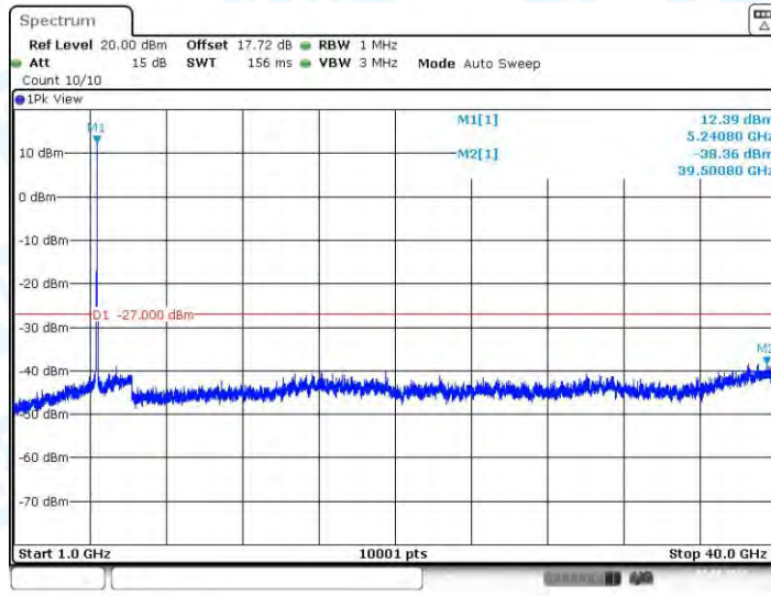
11N20-CDD_Ant4_5240_1000~40000
