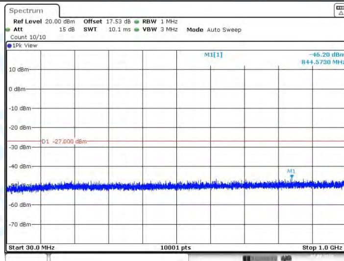
11N20-CDD_Ant4_5200_30~1000
