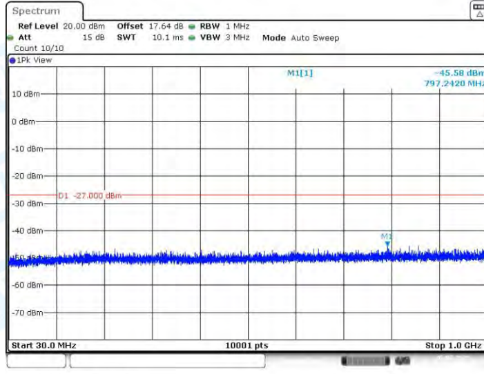
11A_Ant2_5580_30~1000
