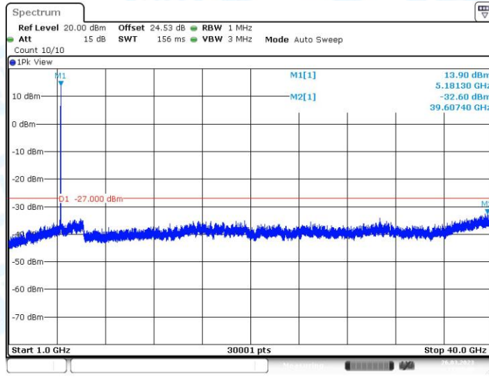
11AC20MIMO_Ant1_5180_1000~40000
