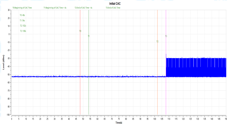
Radar Burst at the Beginning of the Channel Availability Check Time
