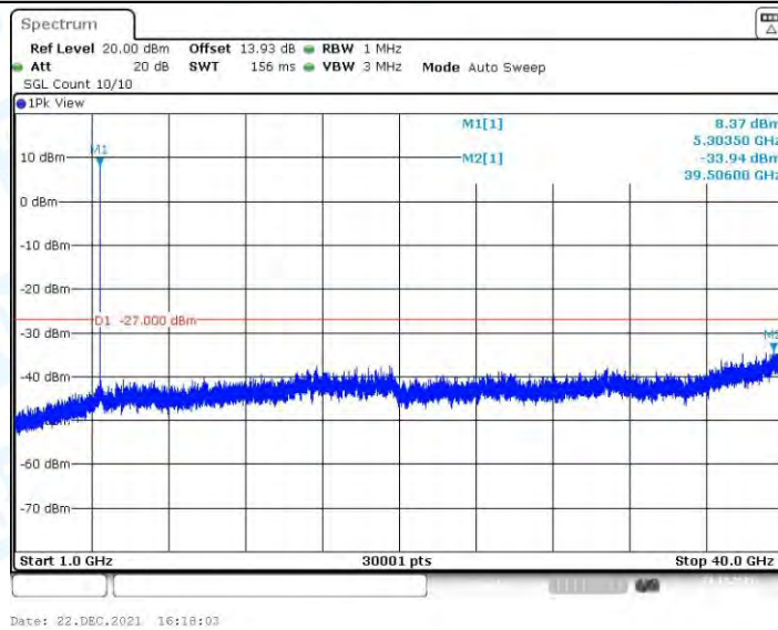
11A_Ant3_5300_1000~40000
