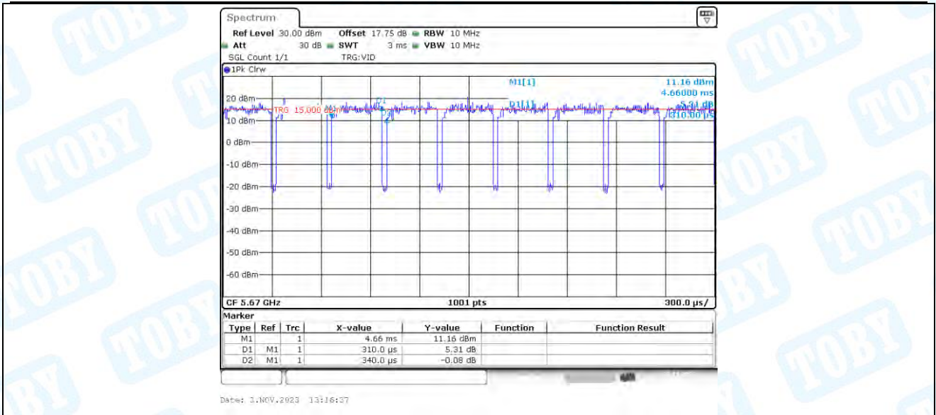
11AX40_Ant3_5670
