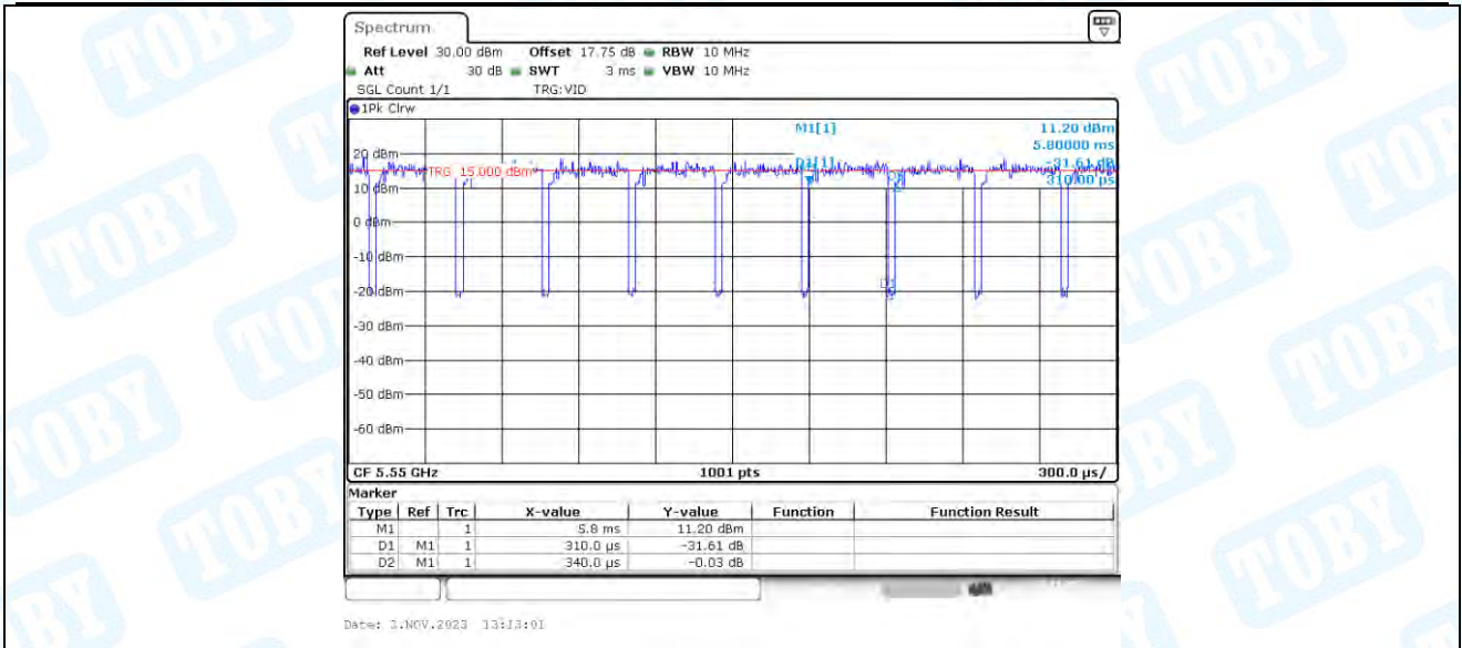
11AX40_Ant4_5550
