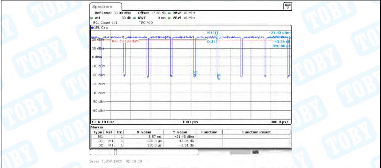
11AX20_Ant2_5180
