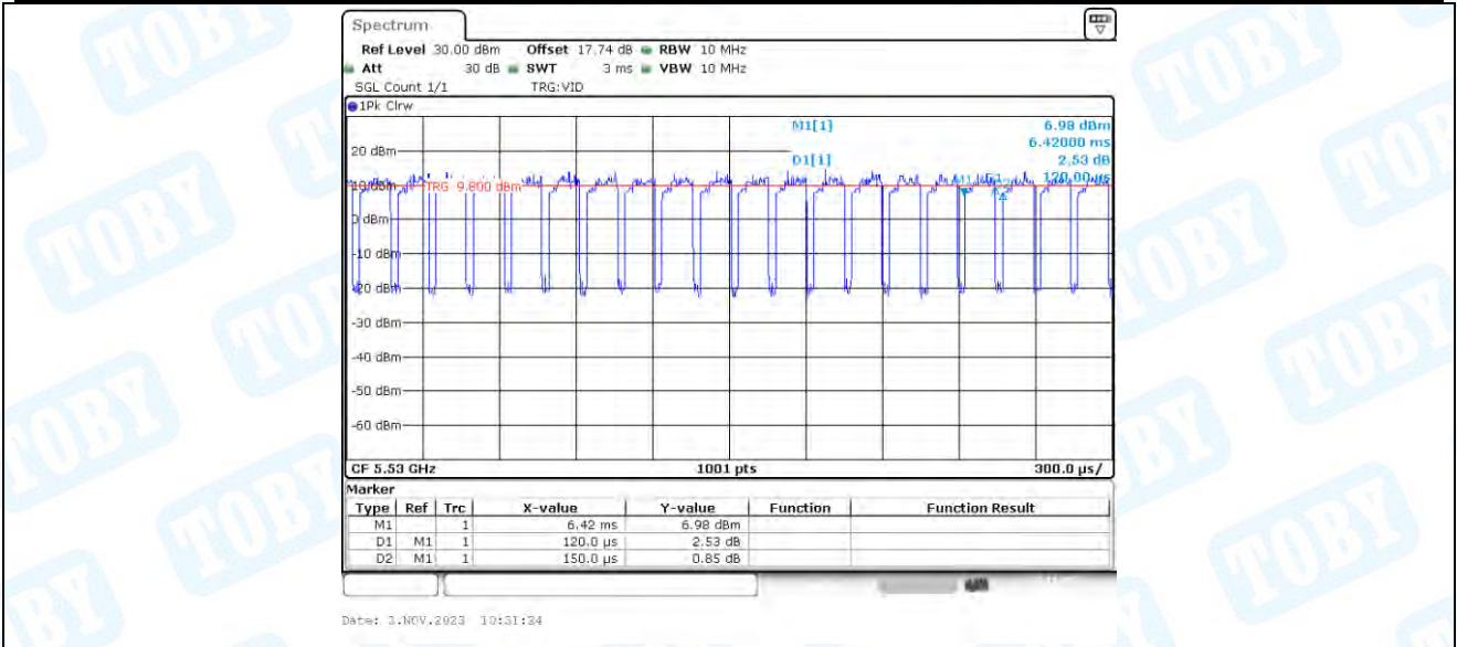
11AC80_Ant4_5530
