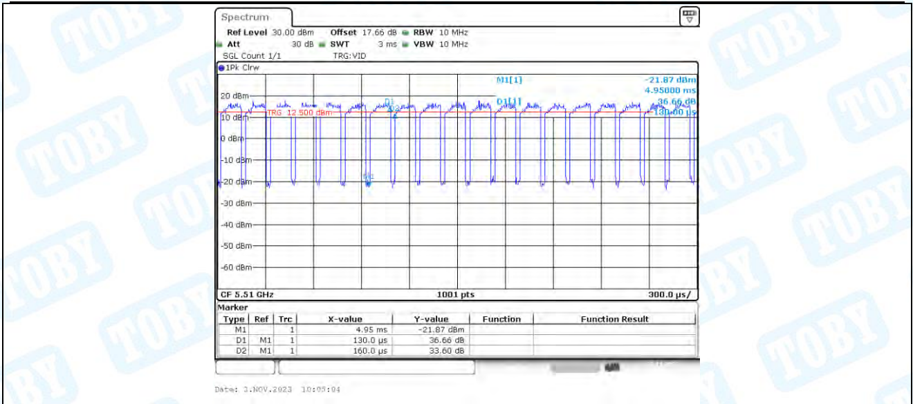
11AC40_Ant3_5510
