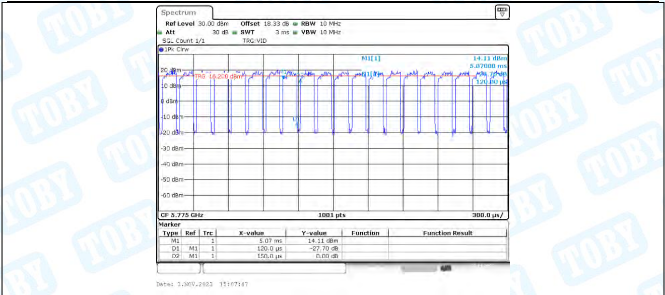
11AC80_Ant4_5775
