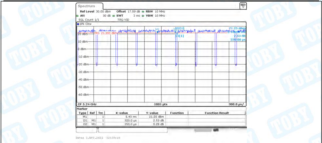
11AX20_Ant2_5240
