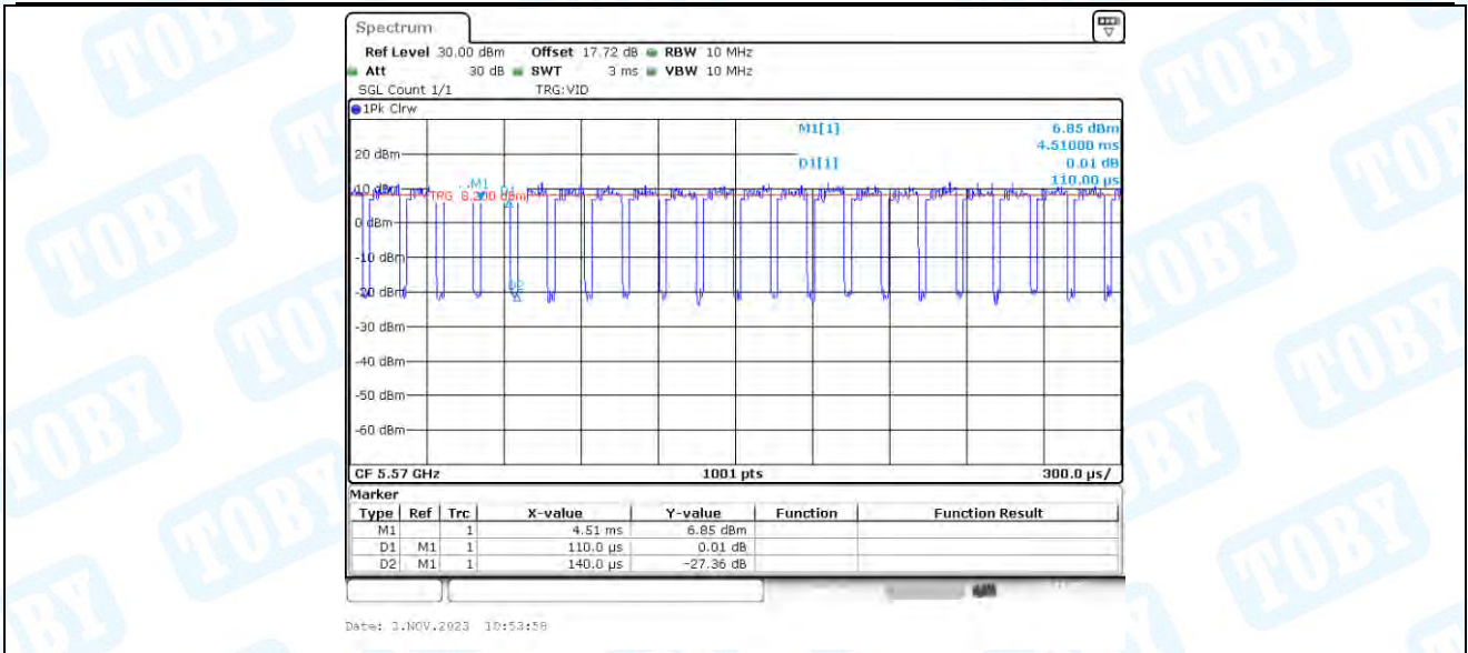
11AC160_Ant2_5570
