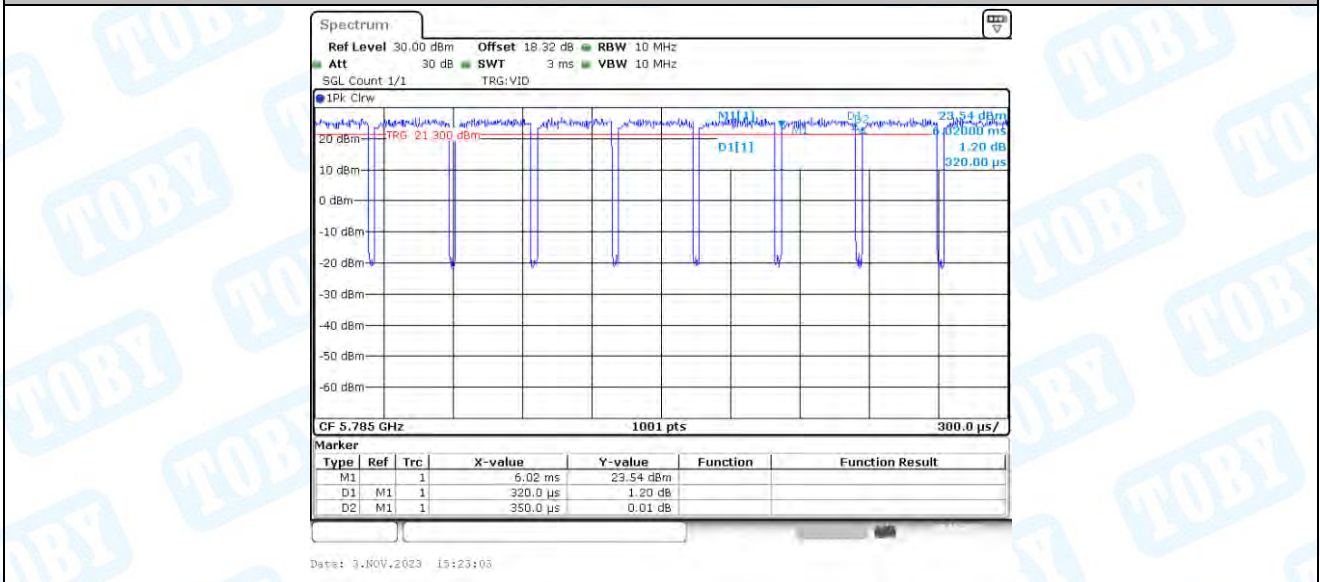
11AX20_Ant3_5785
