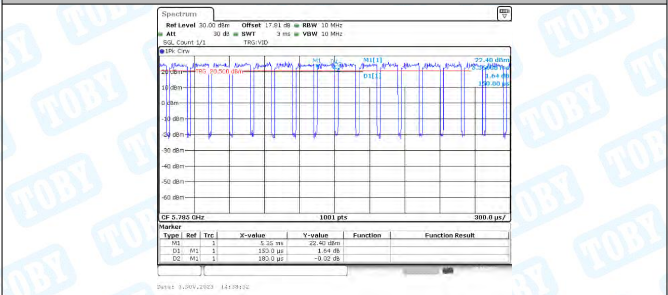
11AC20_Ant2_5785
