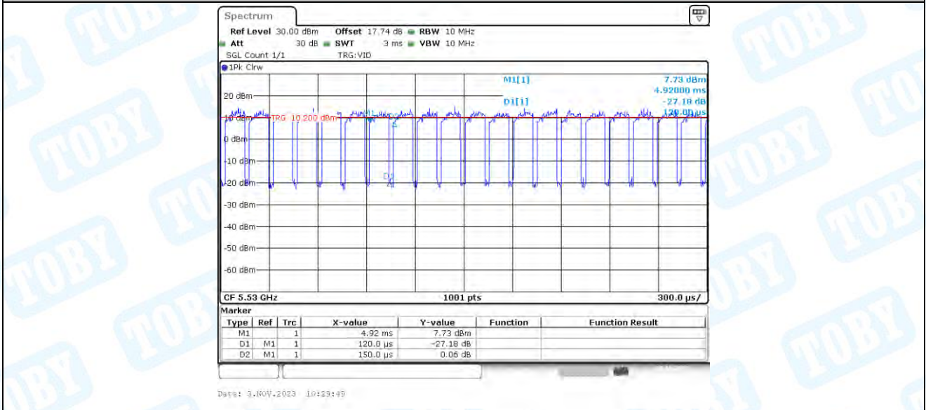
11AC80_Ant2_5530
