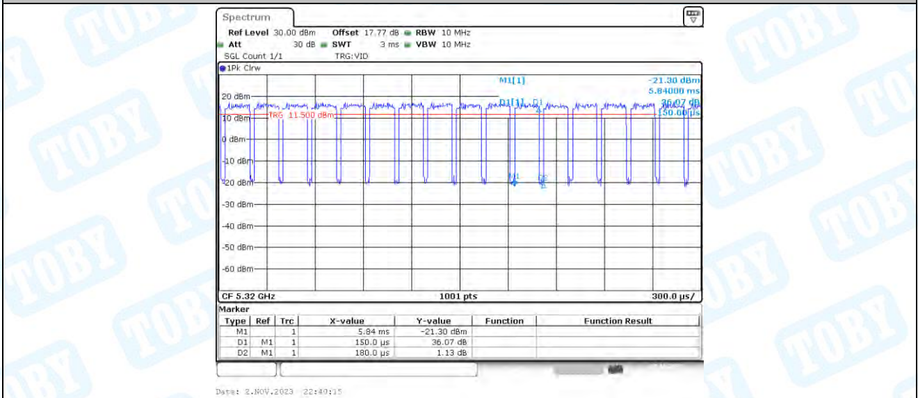
11AC20_Ant4_5320
