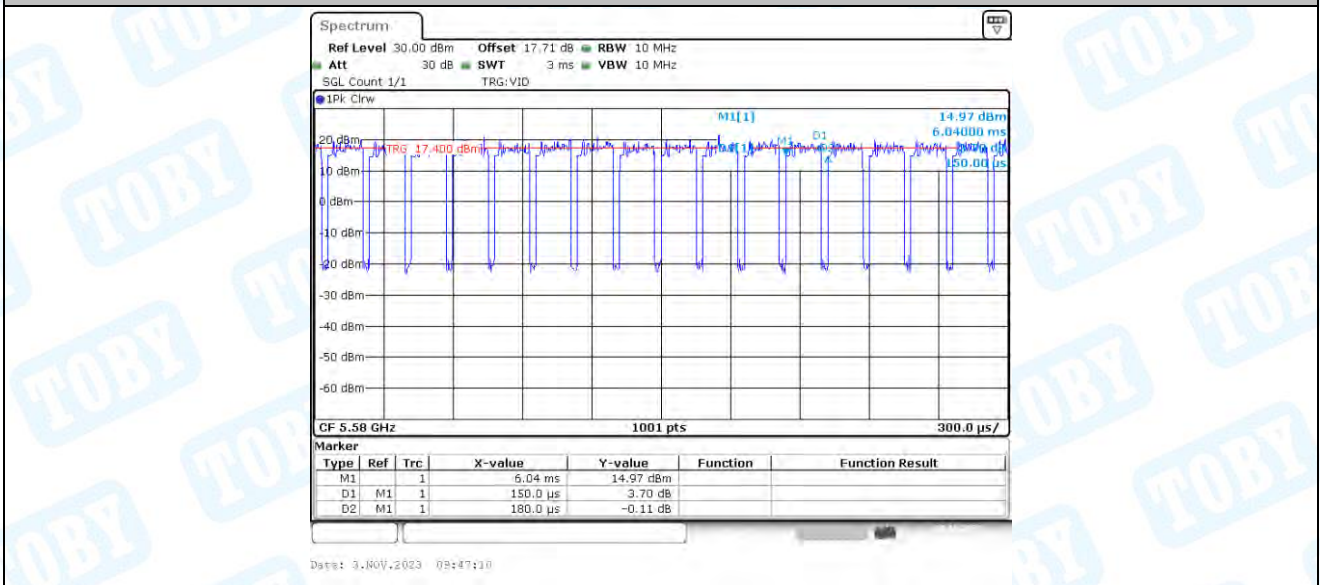
11AC20_Ant3_5580
