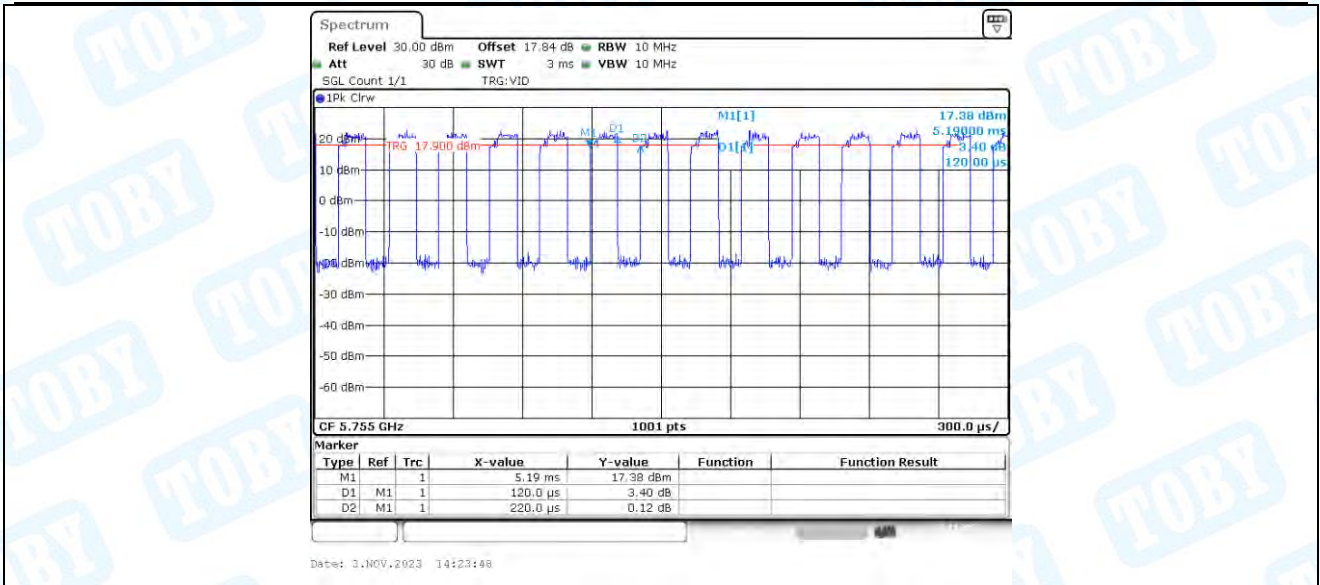
11N40_Ant4_5755
