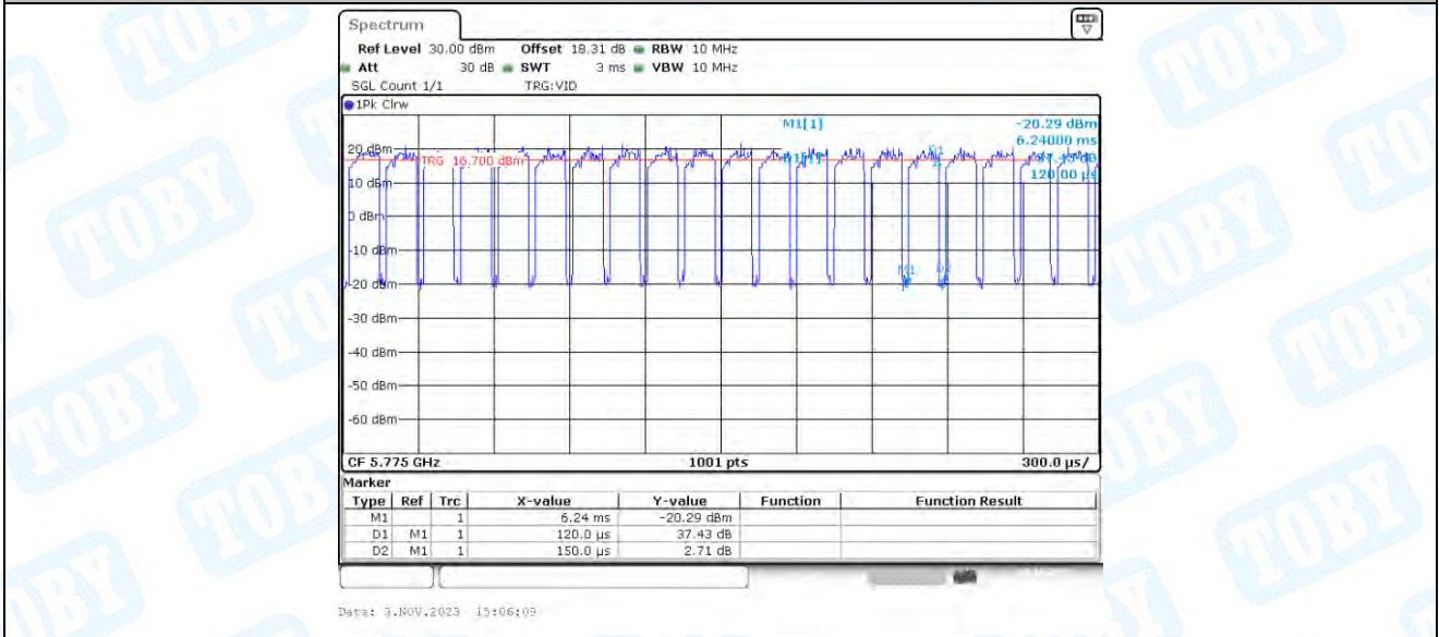
11AC80_Ant2_5775
