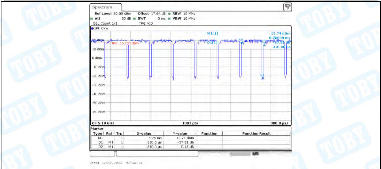
11AX40_Ant3_5190
