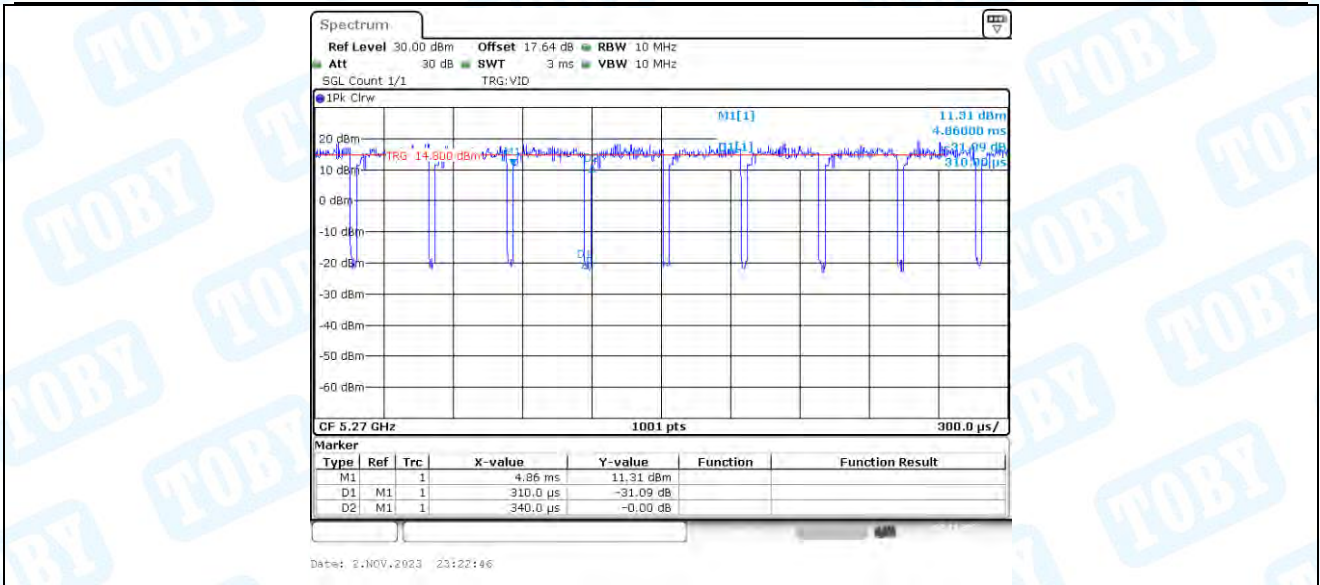
11AX40_Ant4_5270
