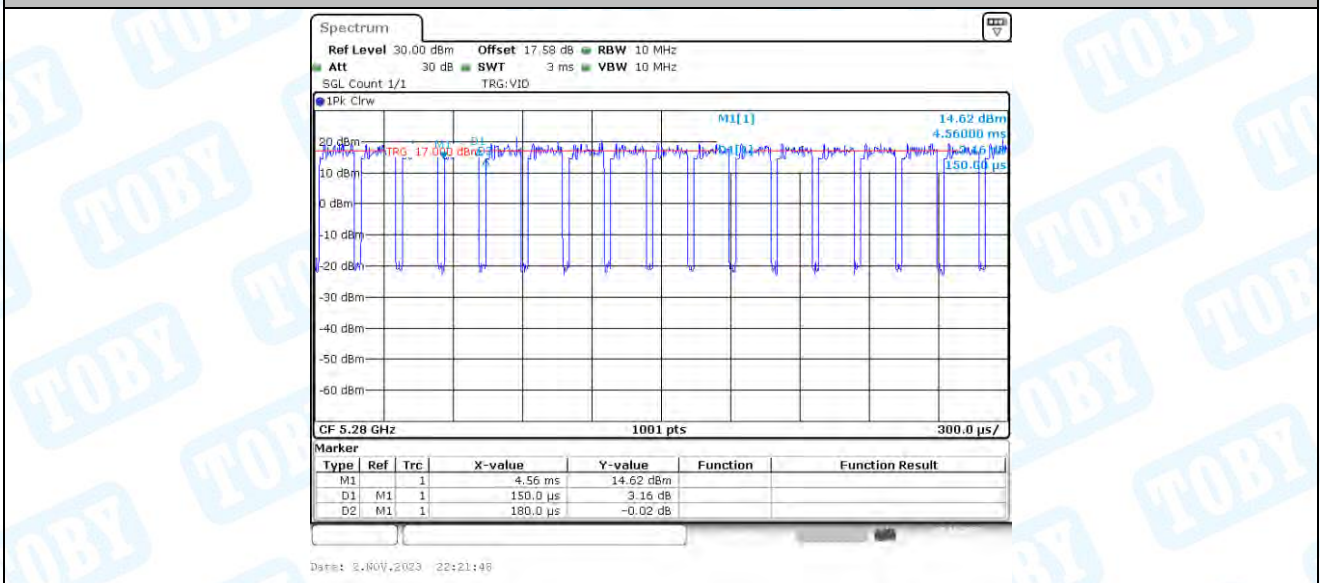
11AC20_Ant3_5280
