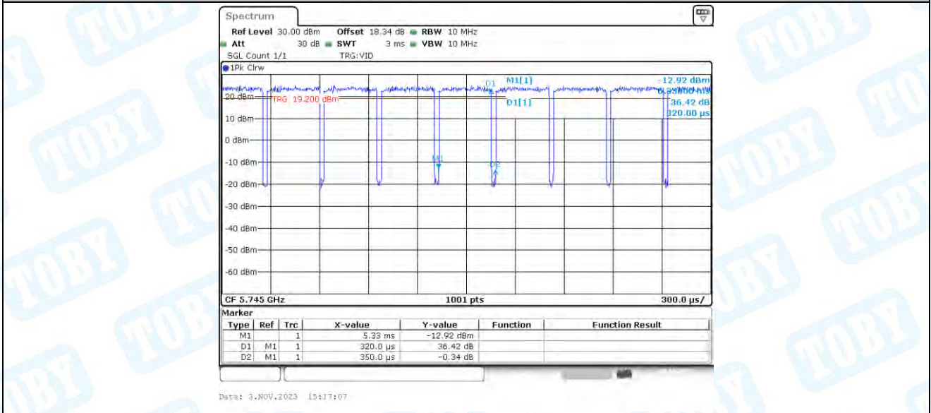
11AX20_Ant4_5745
