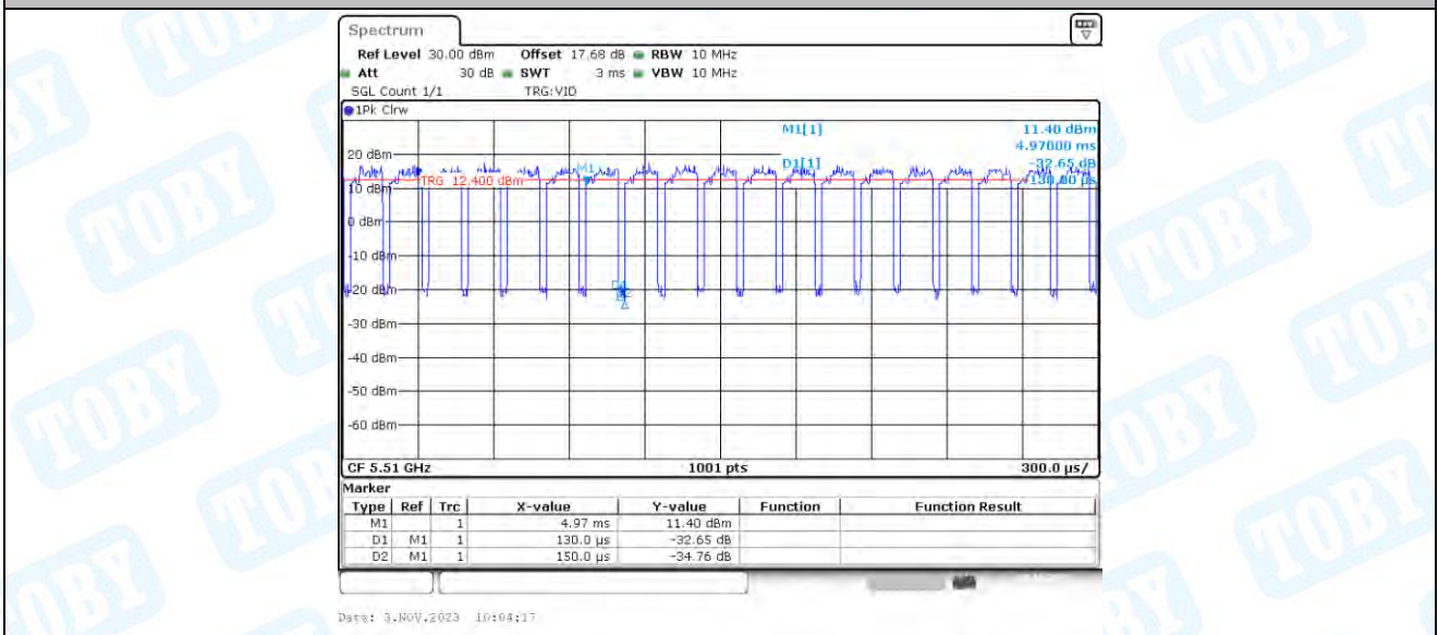
11AC40_Ant2_5510
