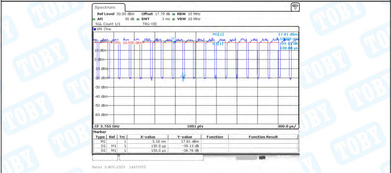
11AC40_Ant3_5755
