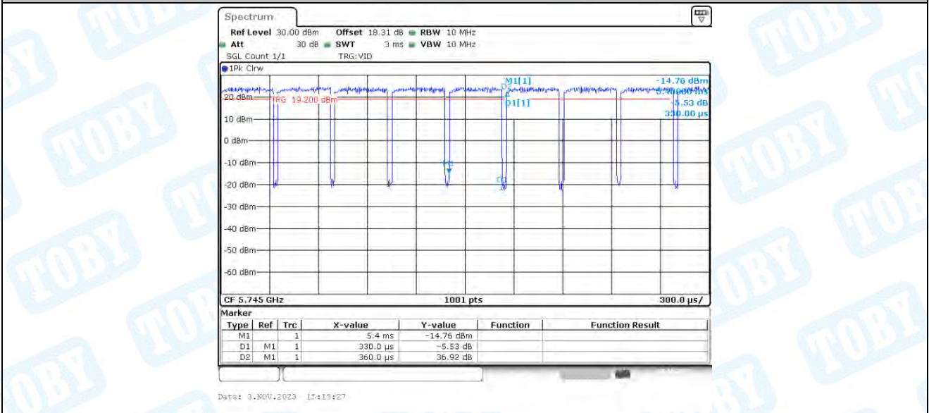
11AX20_Ant2_5745
