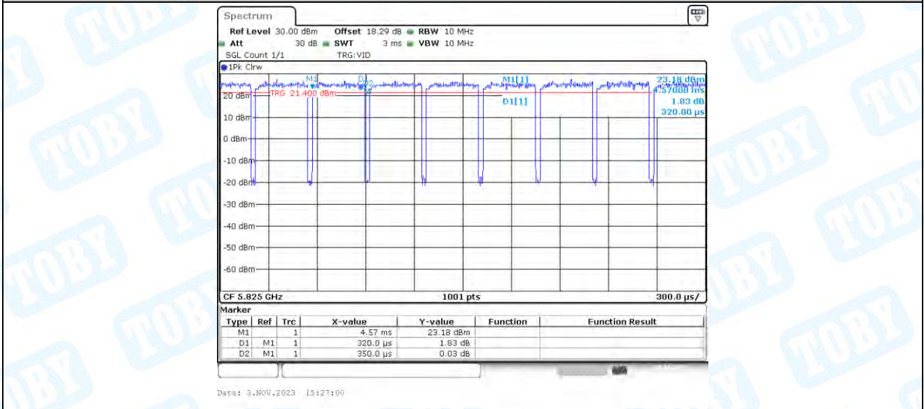
11AX20_Ant2_5825
