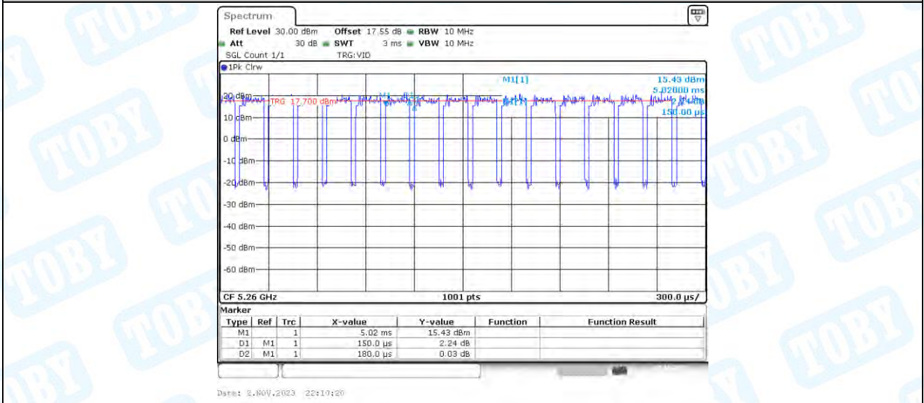
11AC20_Ant3_5260
