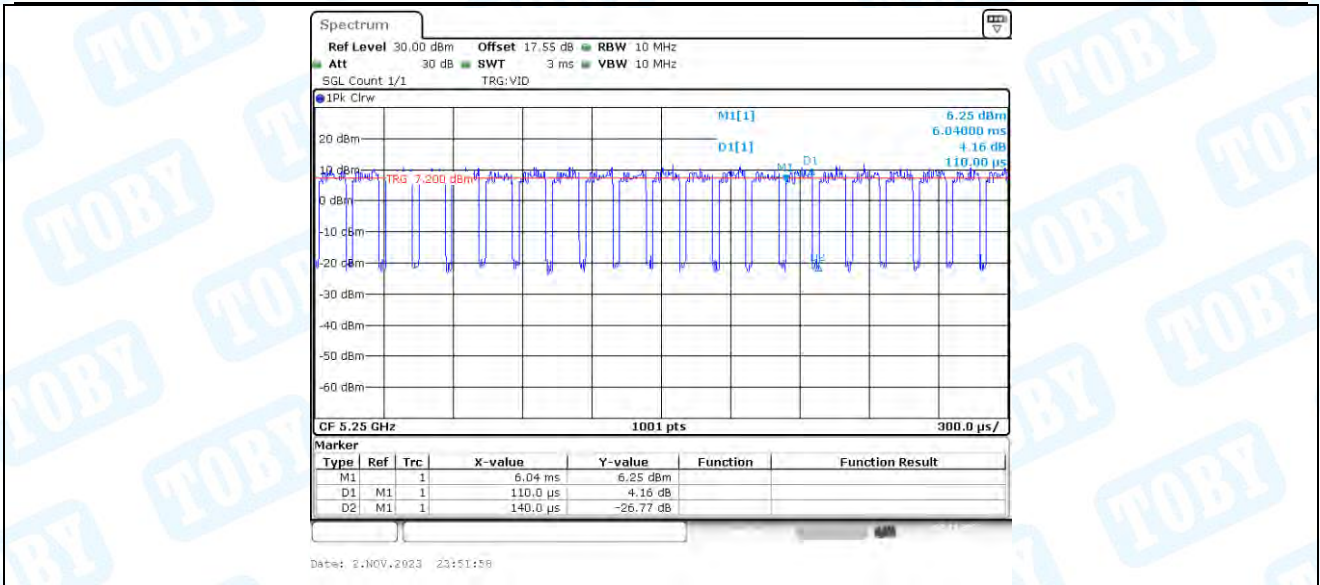
11AC160_Ant3_5250
