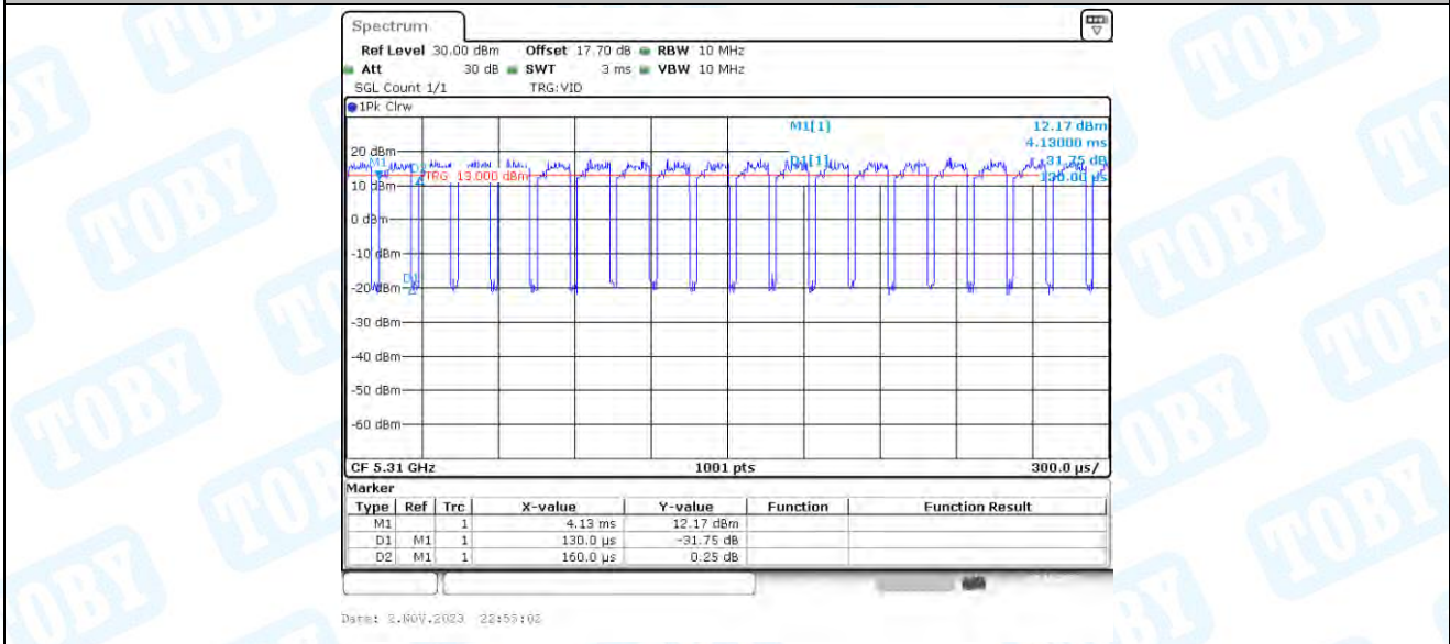
11AC40_Ant3_5310
