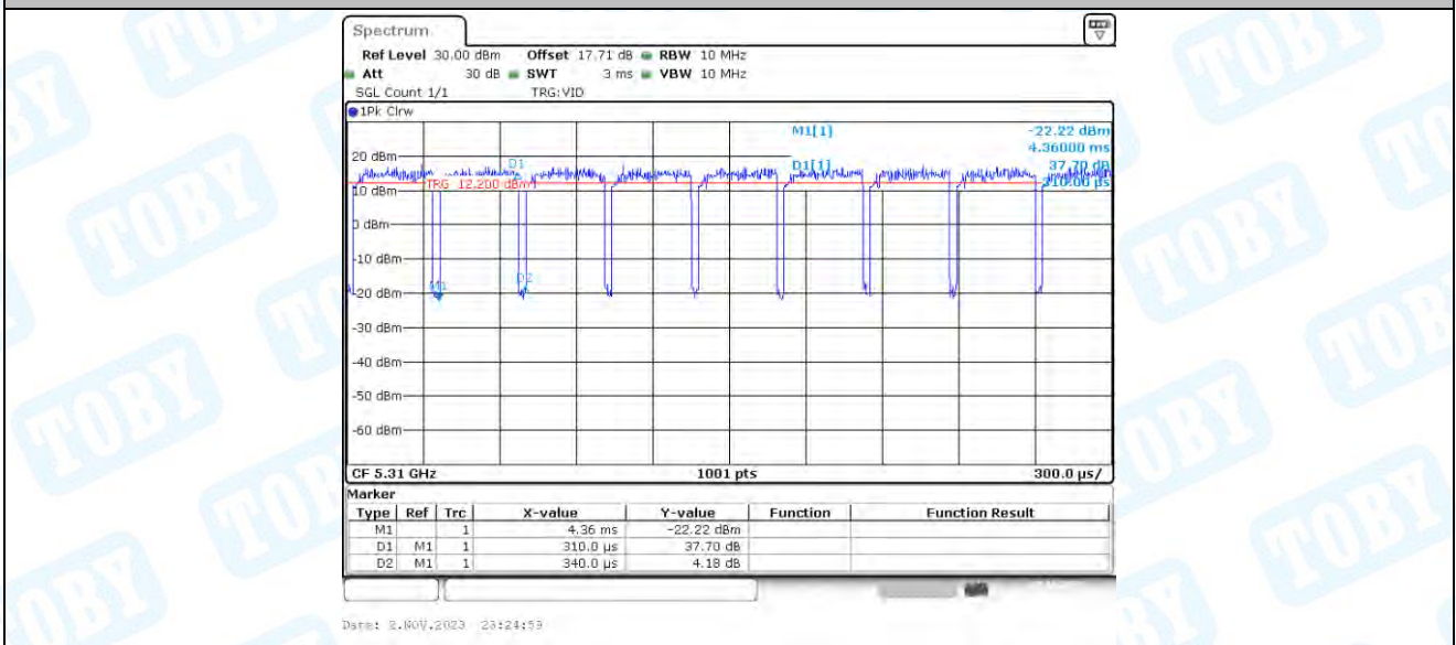
11AX40_Ant2_5310
