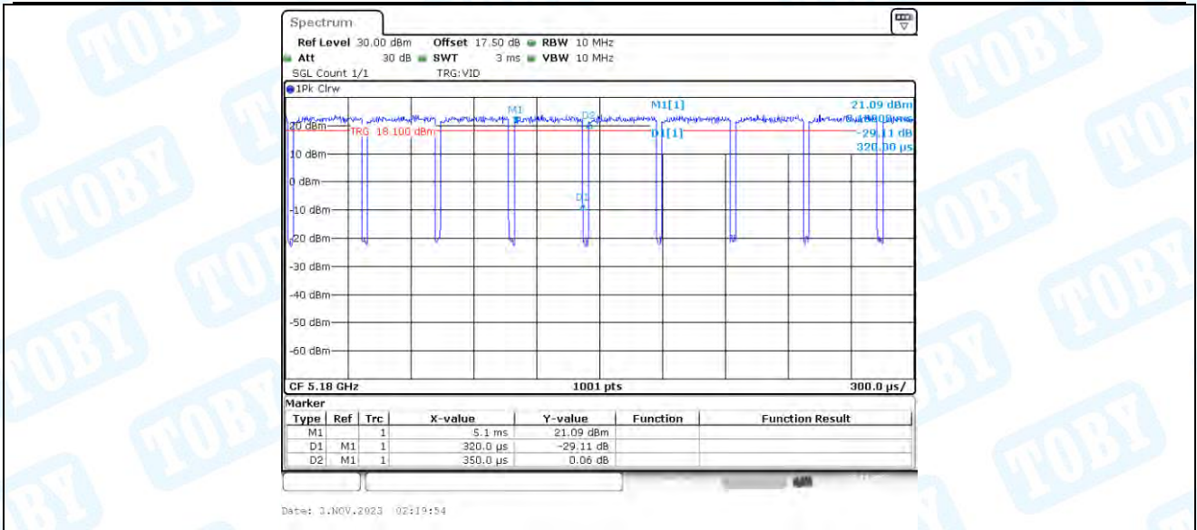
11AX20_Ant4_5180
