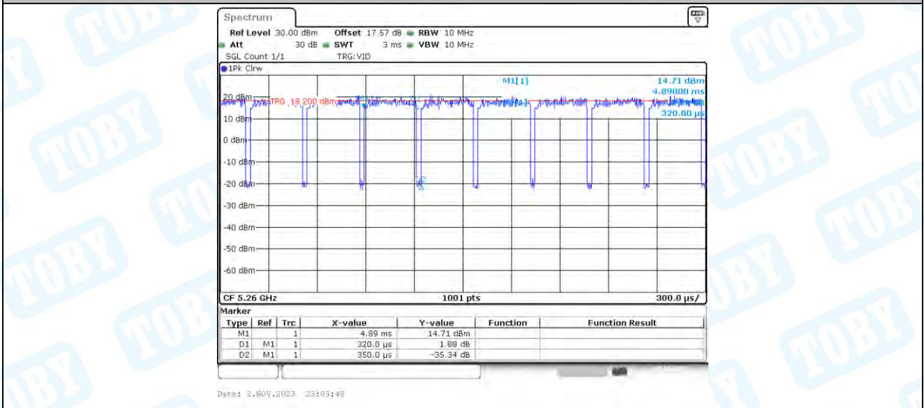
11AX20_Ant2_5260
