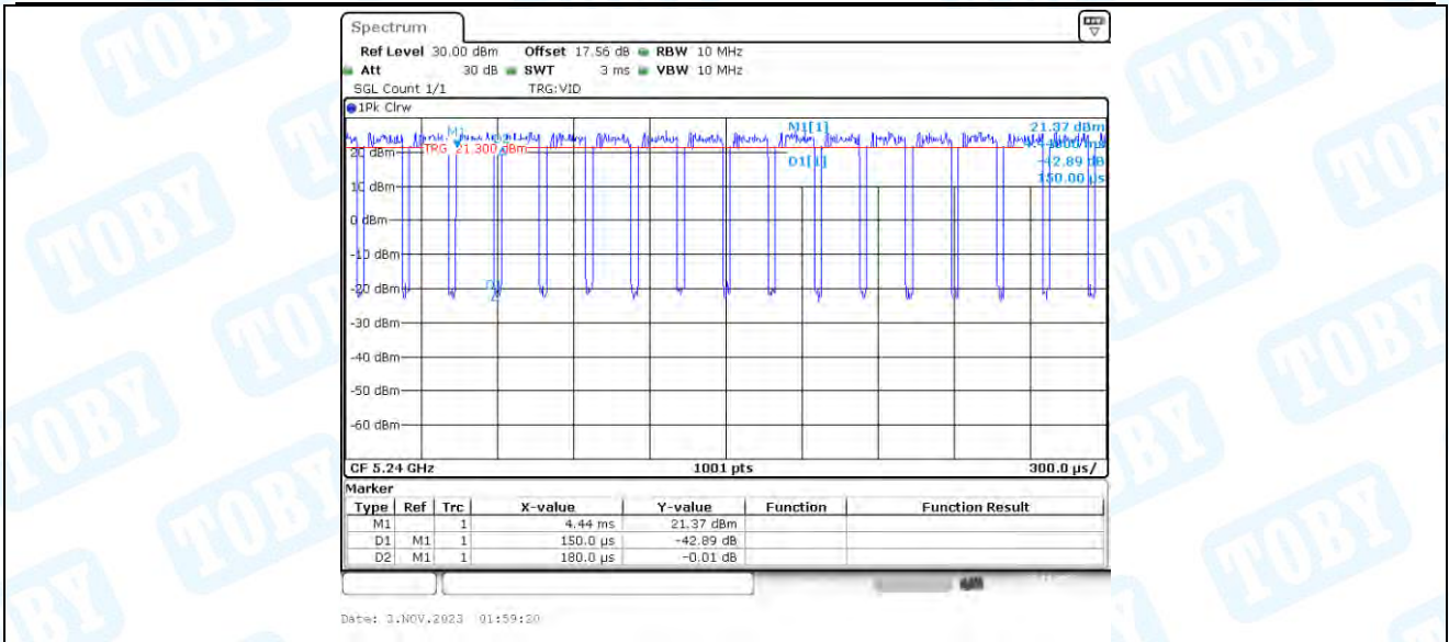
11AC20_Ant3_5240
