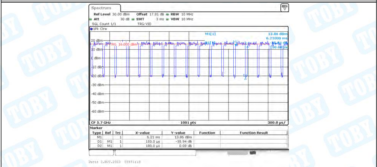
11AC20_Ant2_5700
