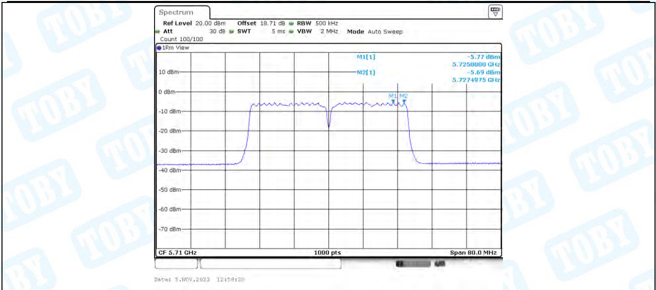
11AC40-BF_Ant4_5710_UNII-3
