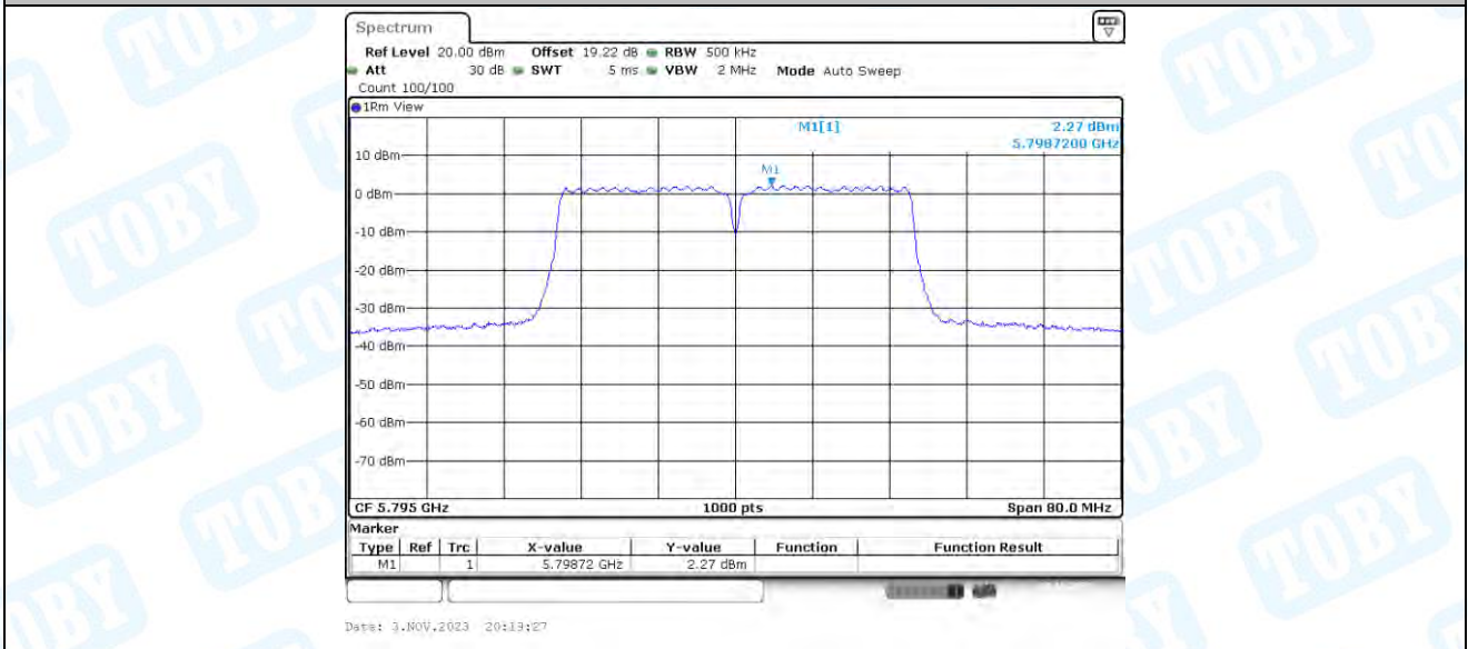
11AC40-BF_Ant3_5795
