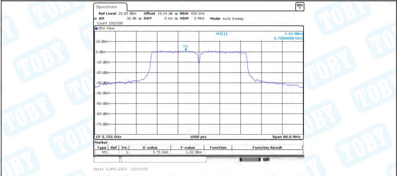
11AC40-BF_Ant4_5755
