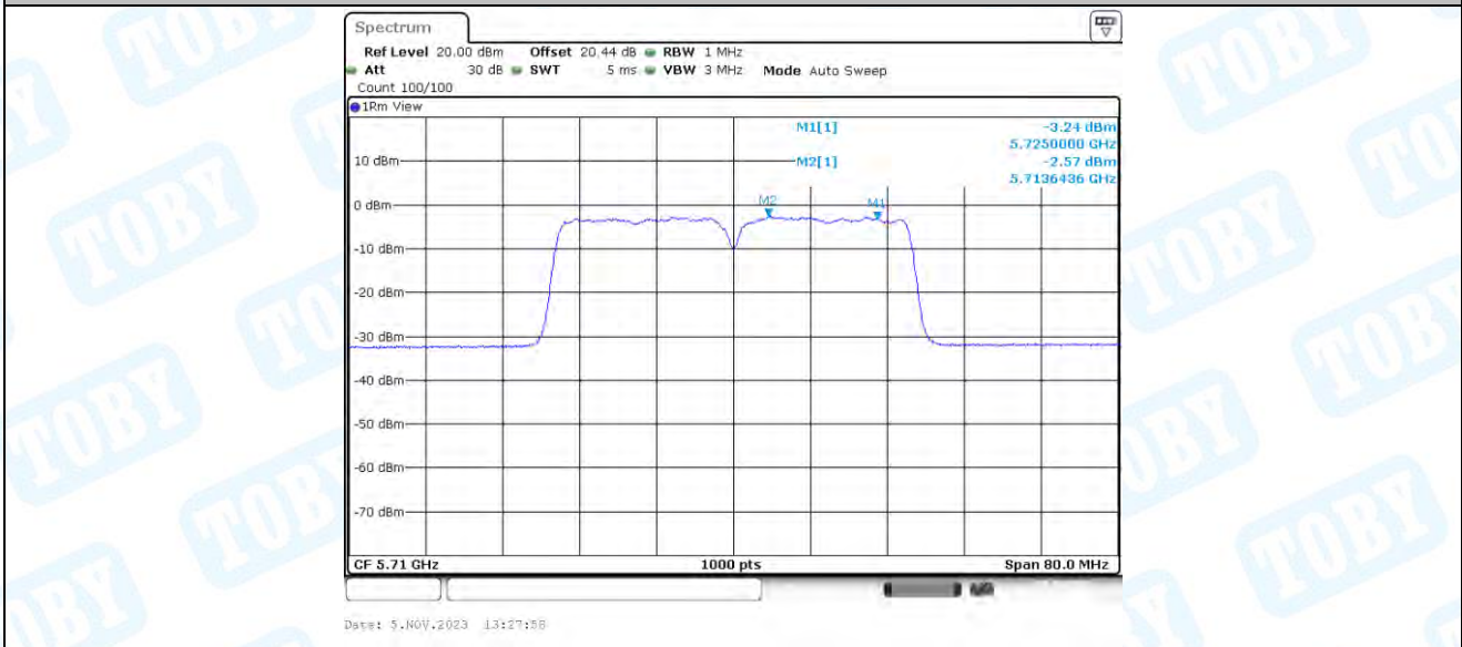
11N40-BF_Ant4_5710_UNII-2C
