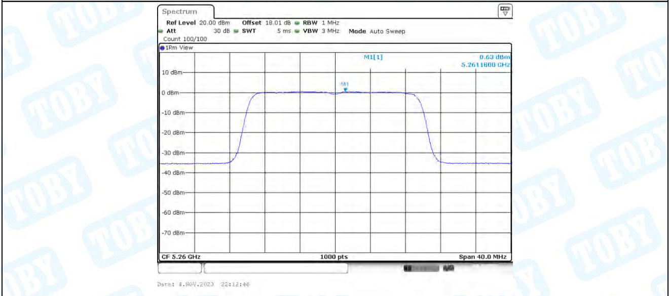
11AX20-BF_Ant4_5260
