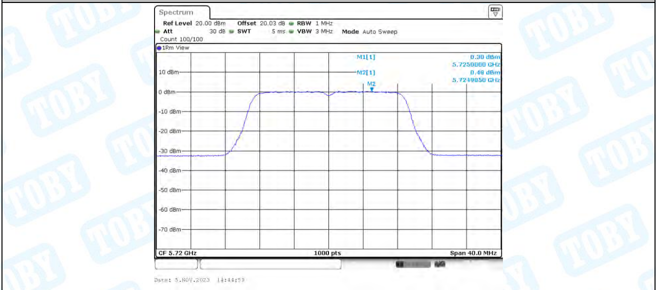
11N20-BF_Ant4_5720_UNII-2C
