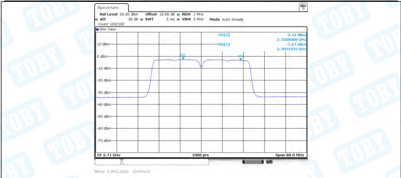
11AC40-BF_Ant2_5710_UNII-2C
