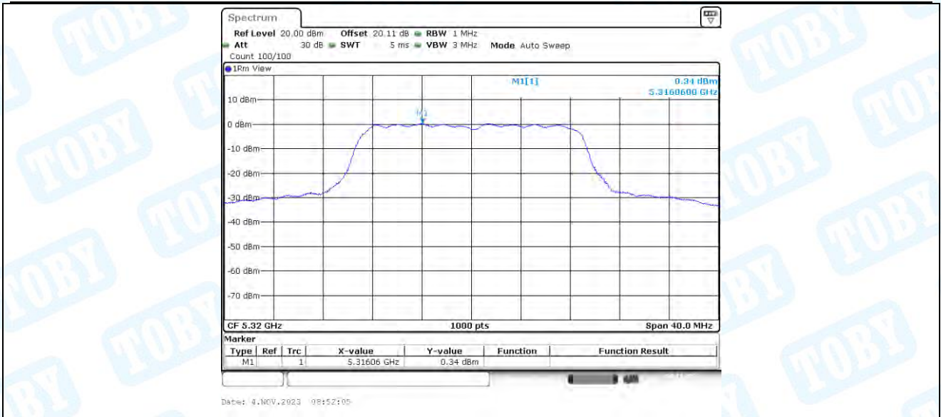
11N20-BF_Ant4_5320
