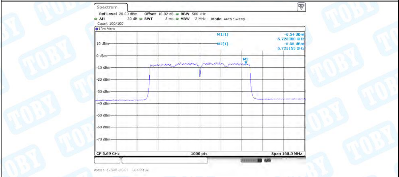
11AC80-BF_Ant4_5690_UNII-3
