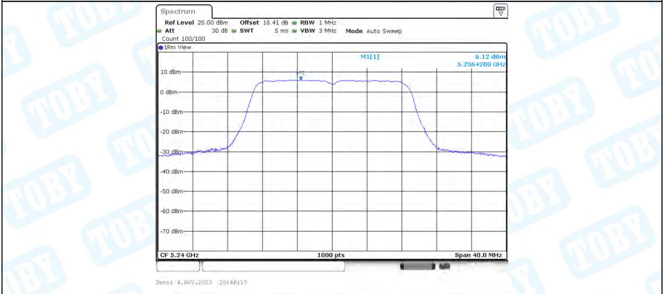
11AC20-BF_Ant4_5240
