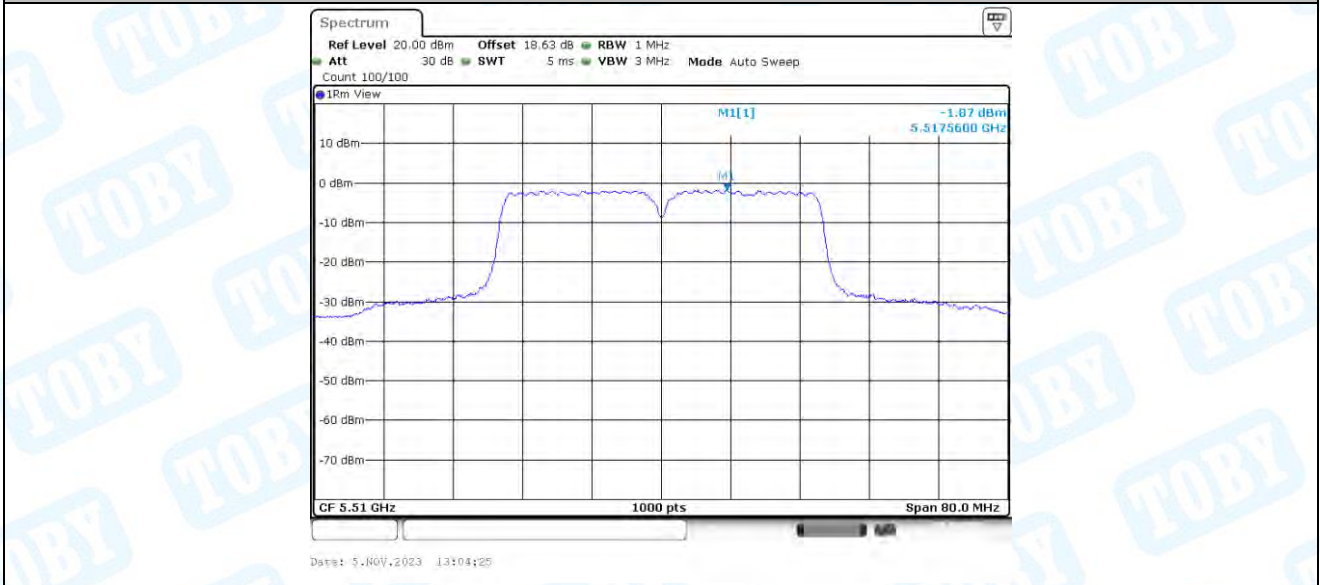
11AC40-BF_Ant3_5510
