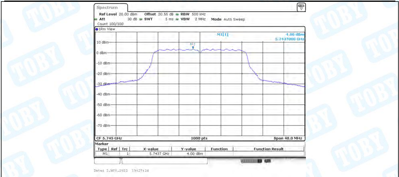
11N20-BF_Ant4_5745
