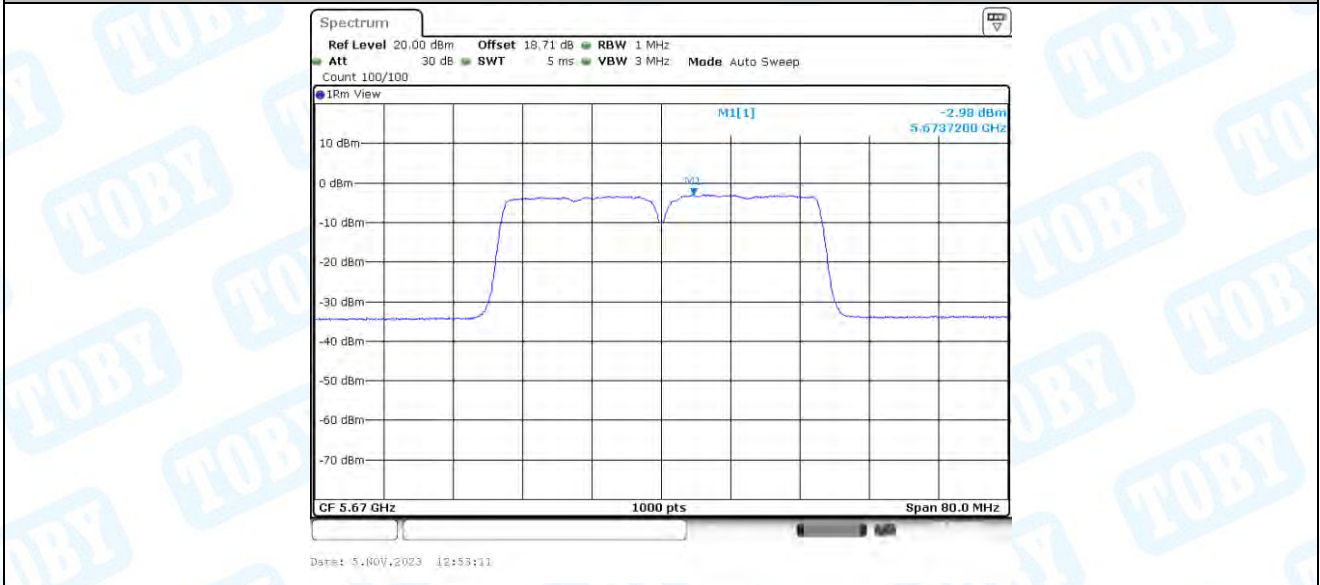
11AC40-BF_Ant4_5670
