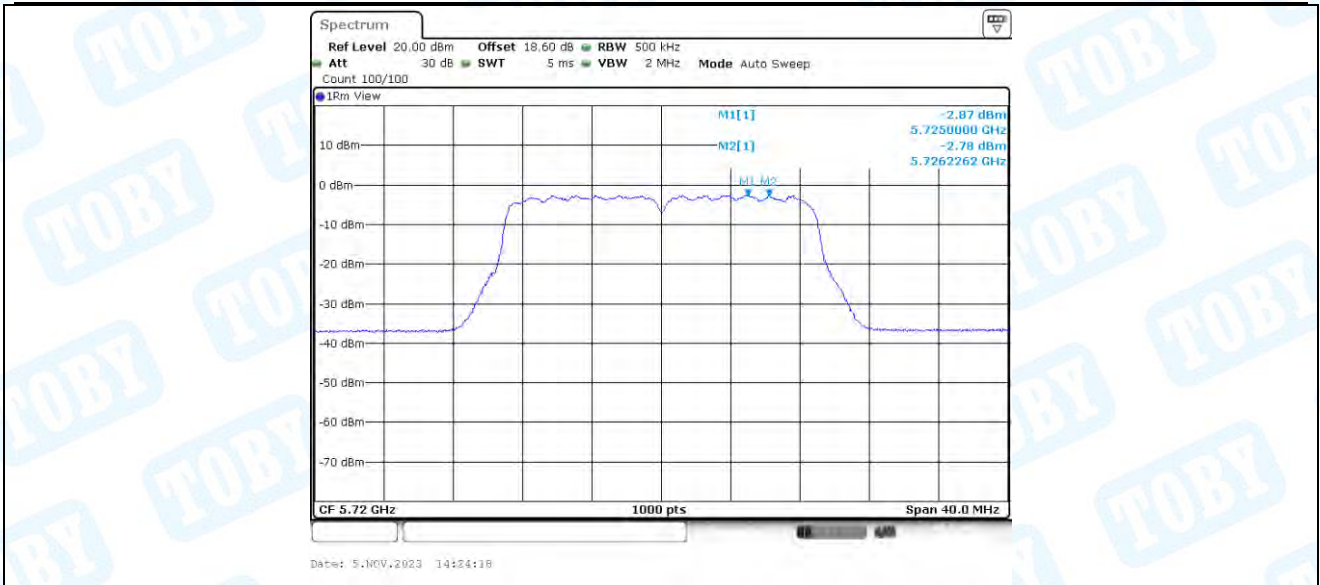
11AC20-BF_Ant4_5720_UNII-3
