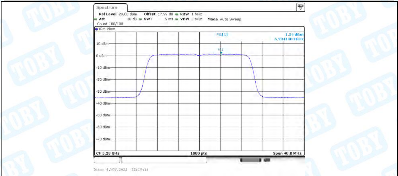
11AX20-BF_Ant2_5280
