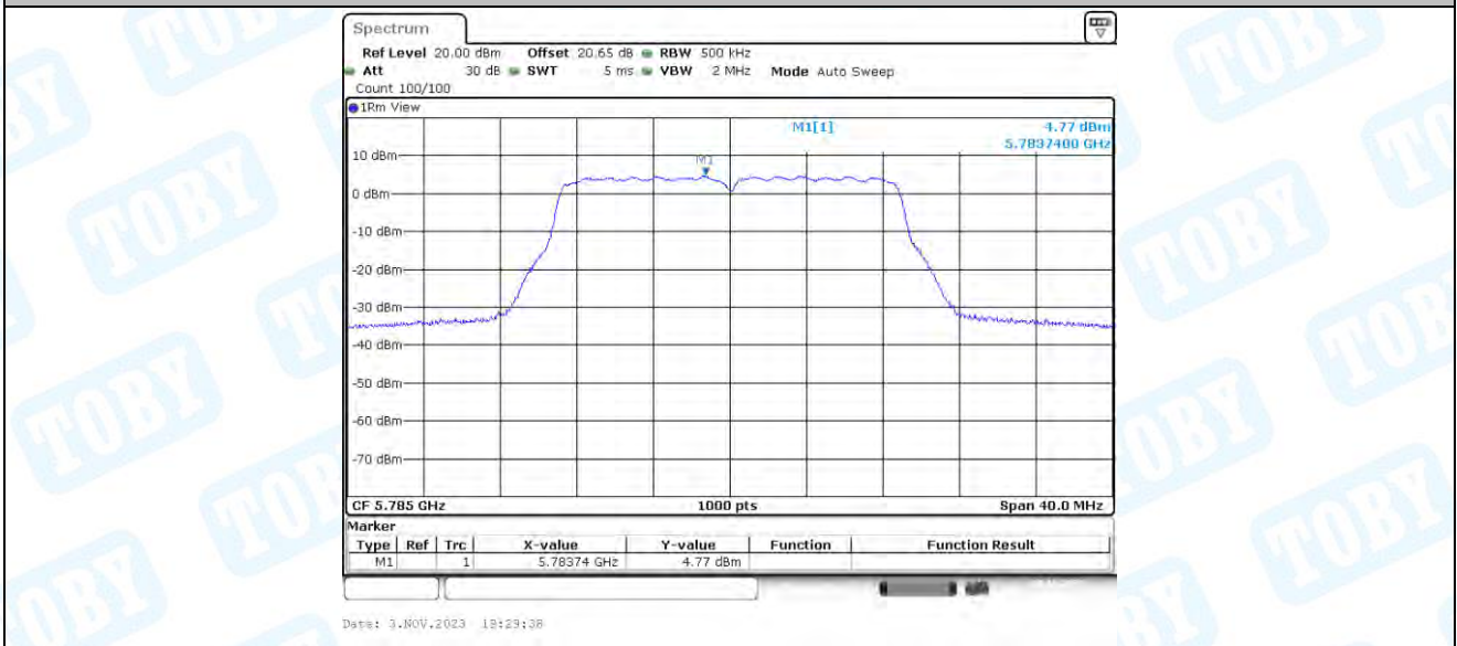
11N20-BF_Ant2_5785
