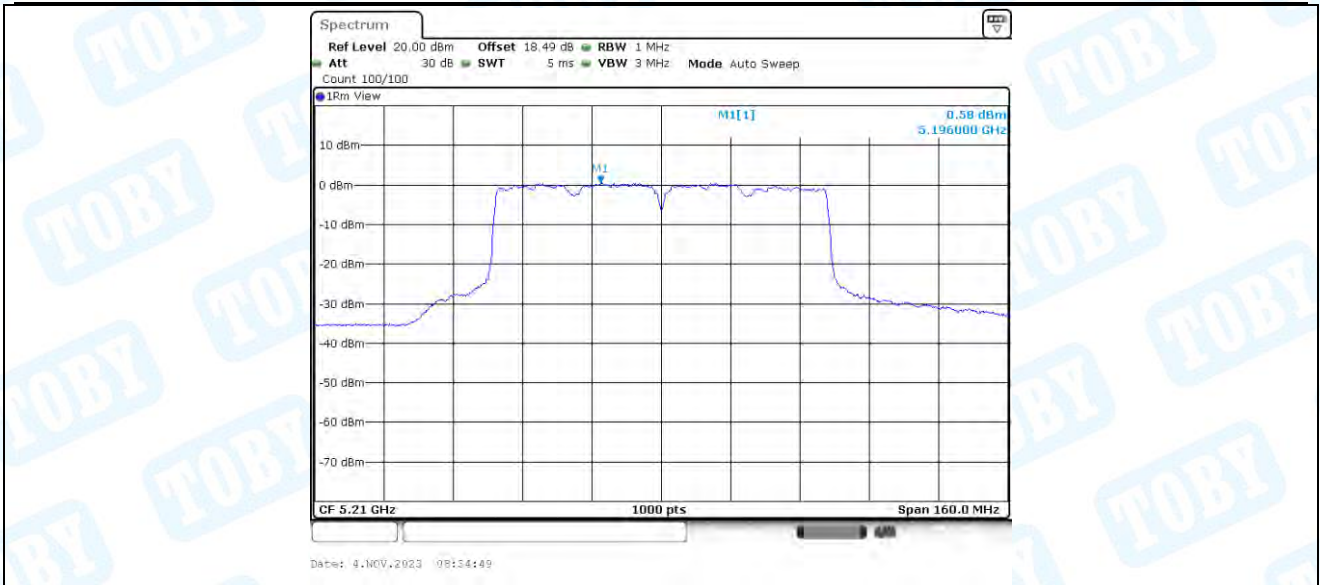
11AC80-BF_Ant4_5210
