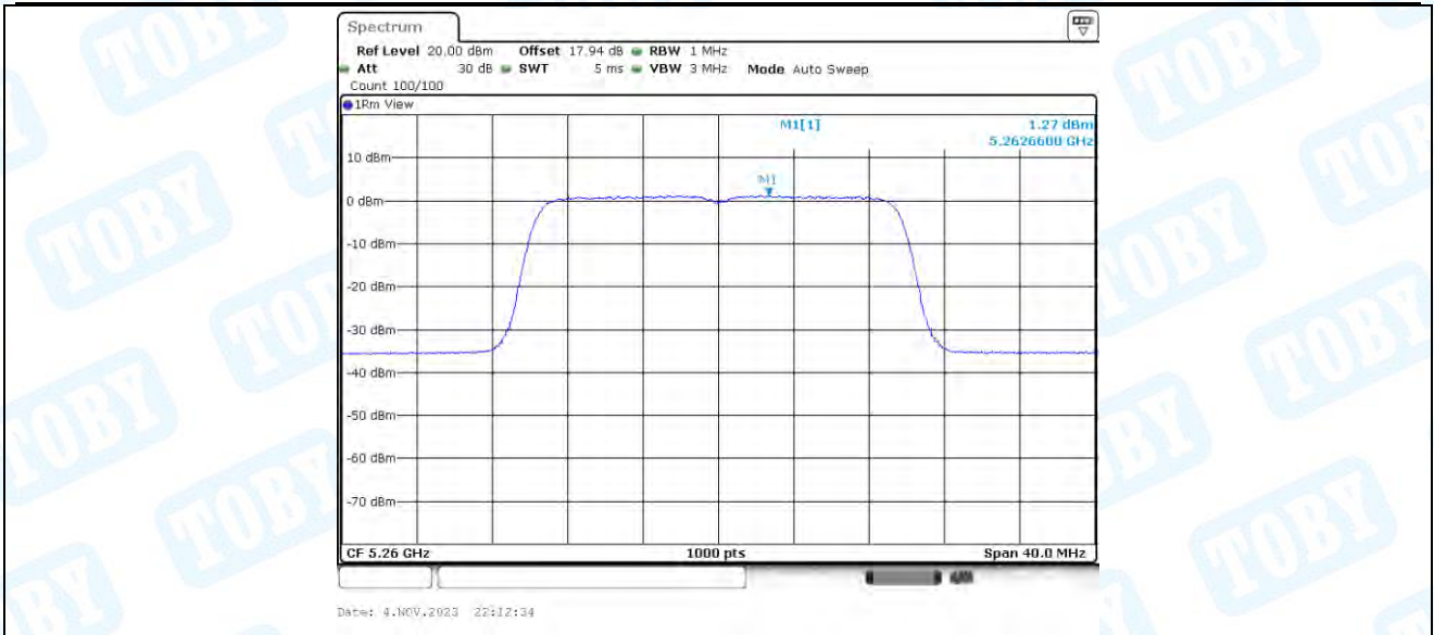
11AX20-BF_Ant3_5260
