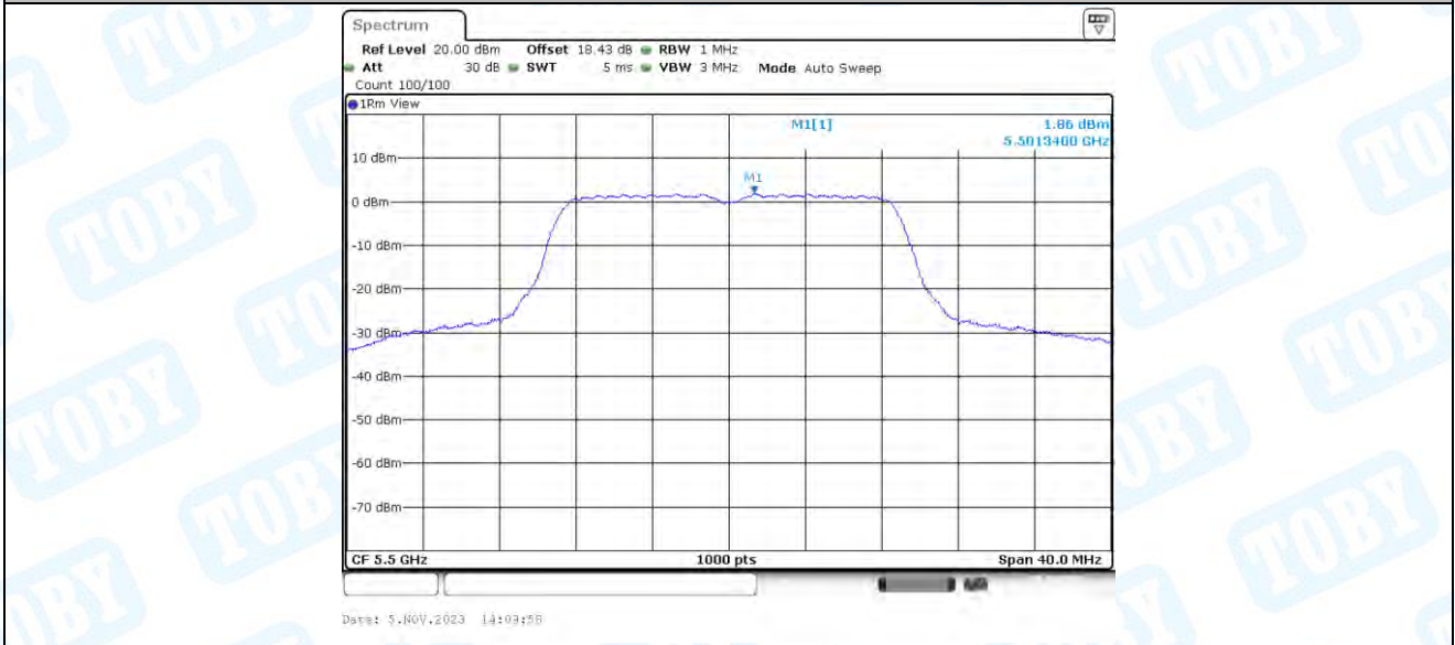
11AC20-BF_Ant3_5500
