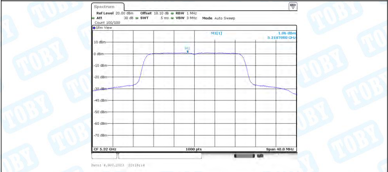
11AX20-BF_Ant2_5320
