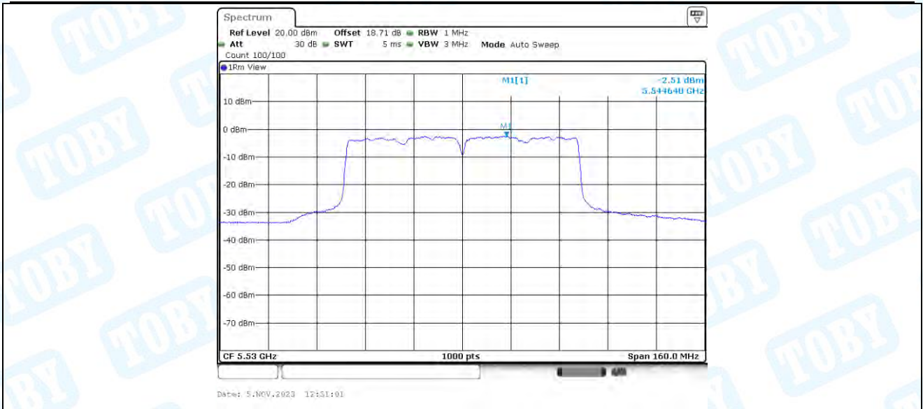
11AC80-BF_Ant2_5530
