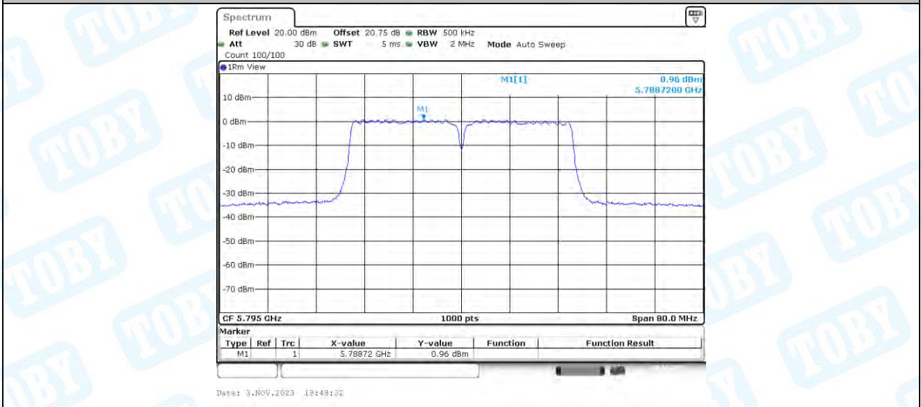
11N40-BF_Ant4_5795
