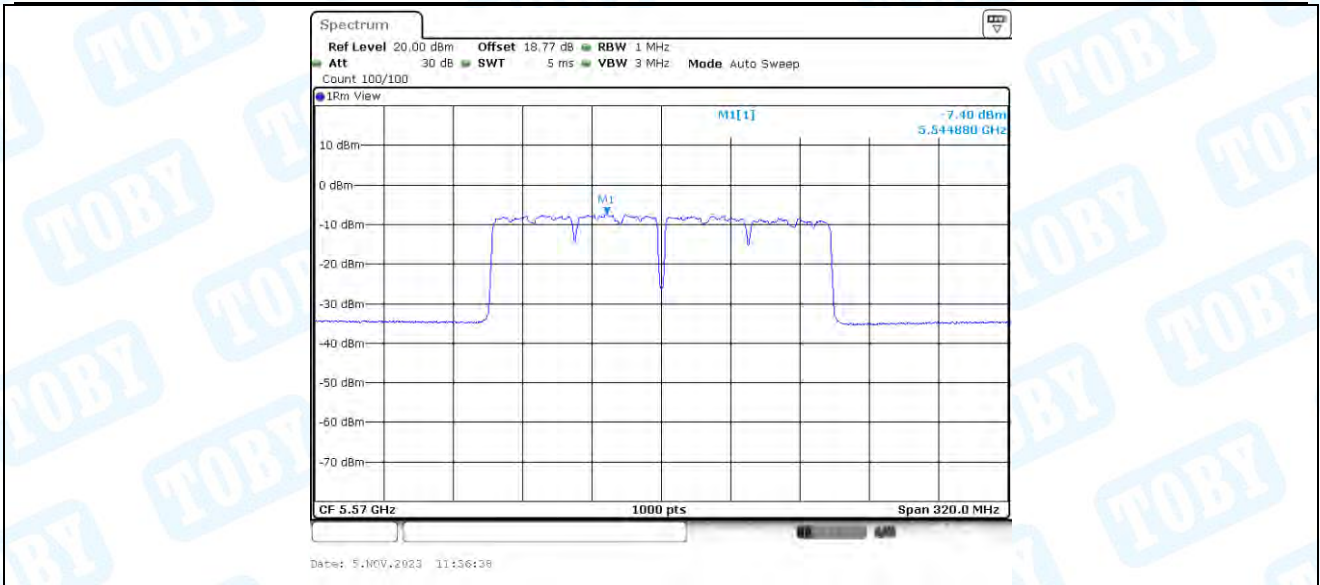
11AC160-BF_Ant4_5570
