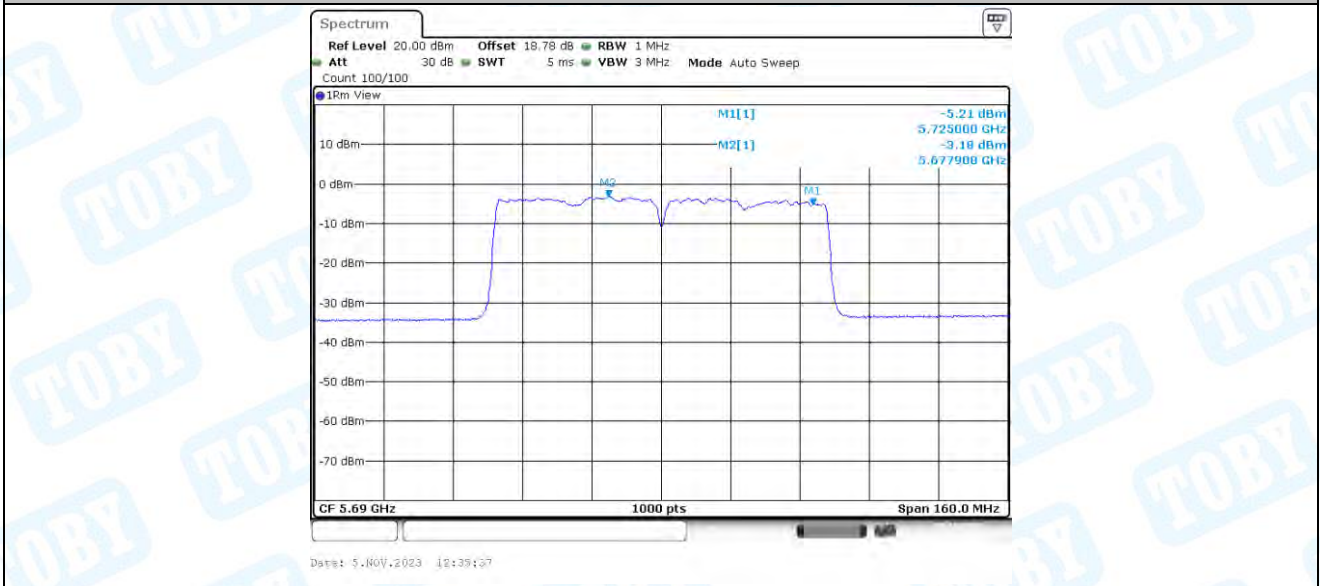
11AC80-BF_Ant2_5690_UNII-2C
