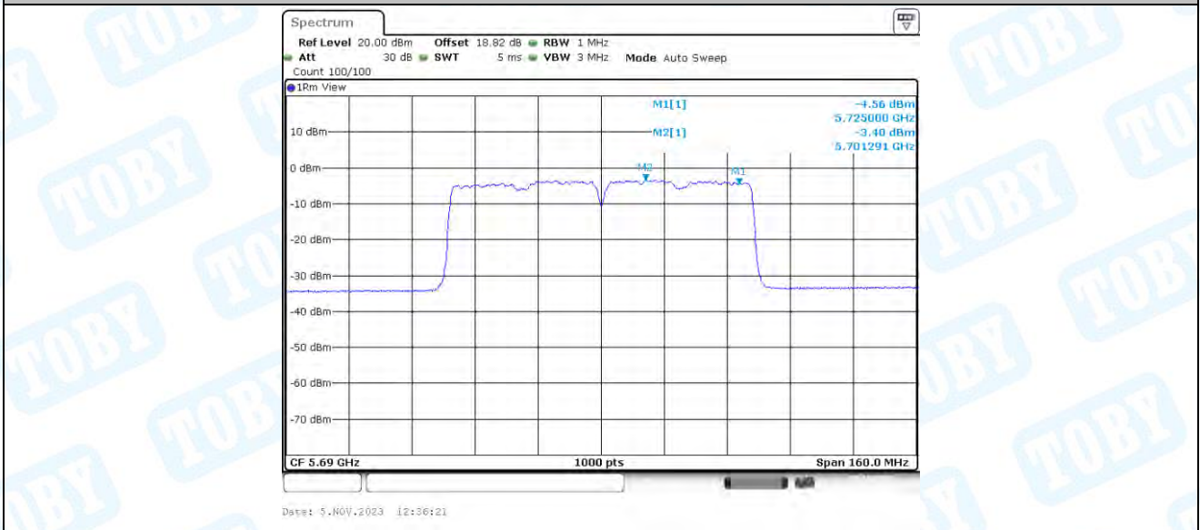
11AC80-BF_Ant4_5690_UNII-2C
