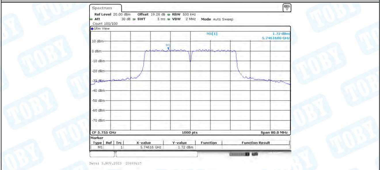
11AC40-BF_Ant2_5755
