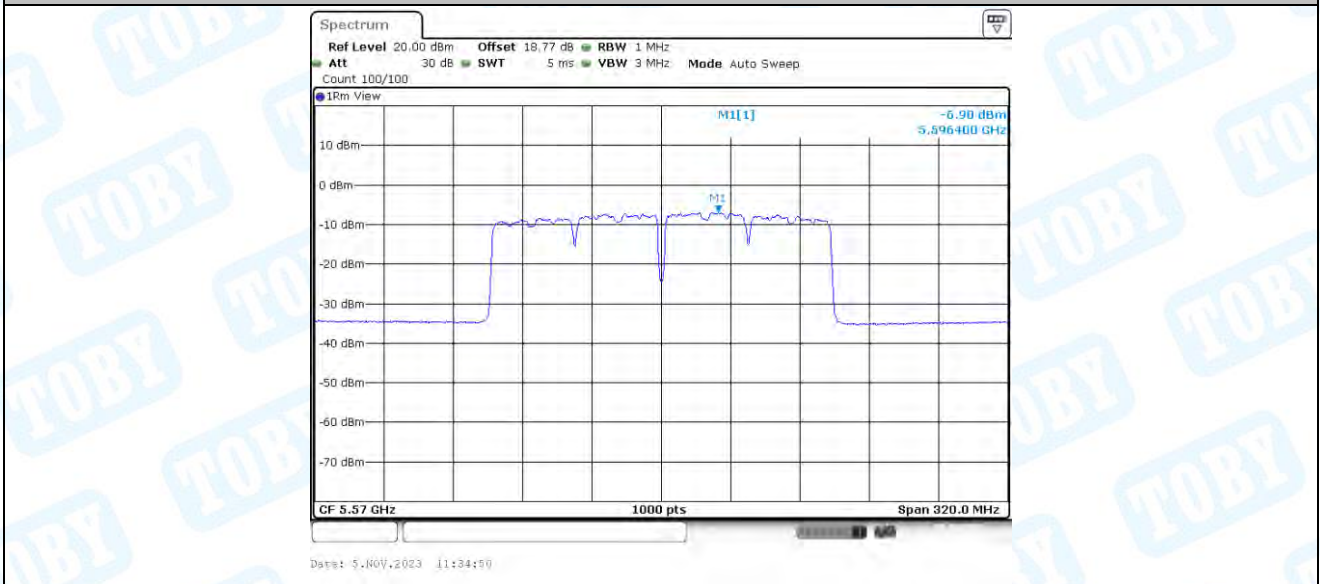
11AC160-BF_Ant2_5570
