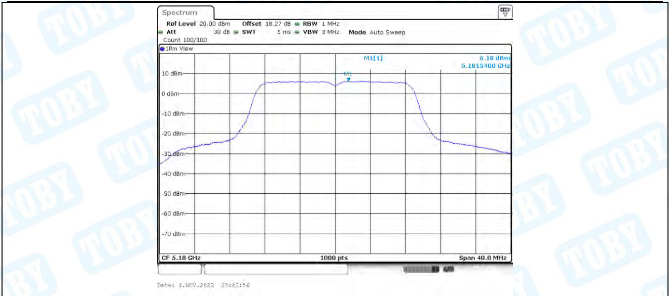
11AC20-BF_Ant2_5180
