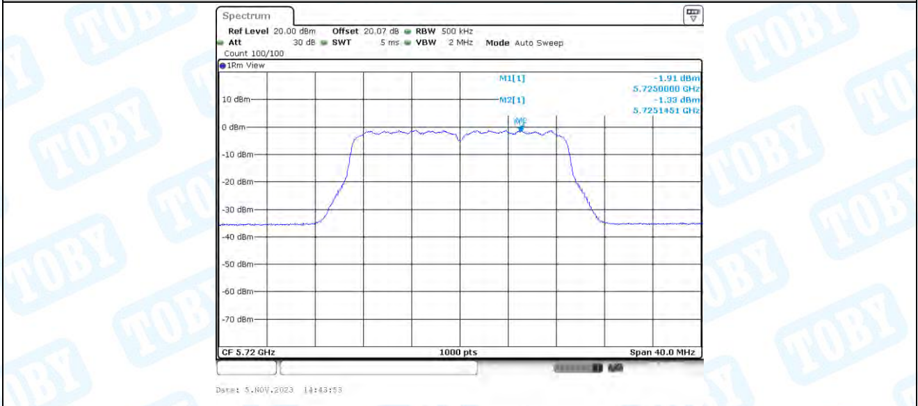
11N20-BF_Ant3_5720_UNII-3
