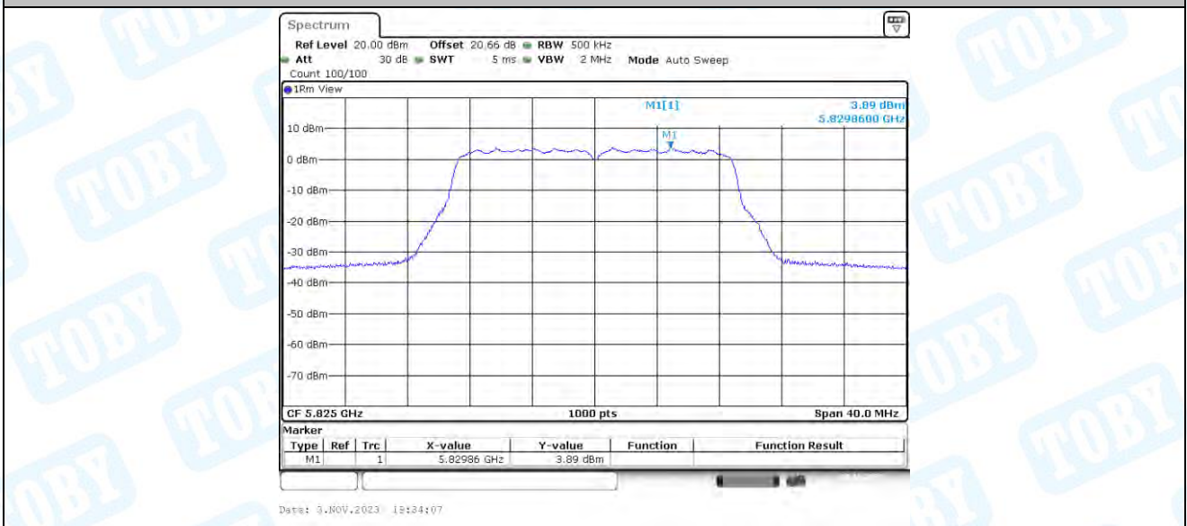
11N20-BF_Ant4_5825
