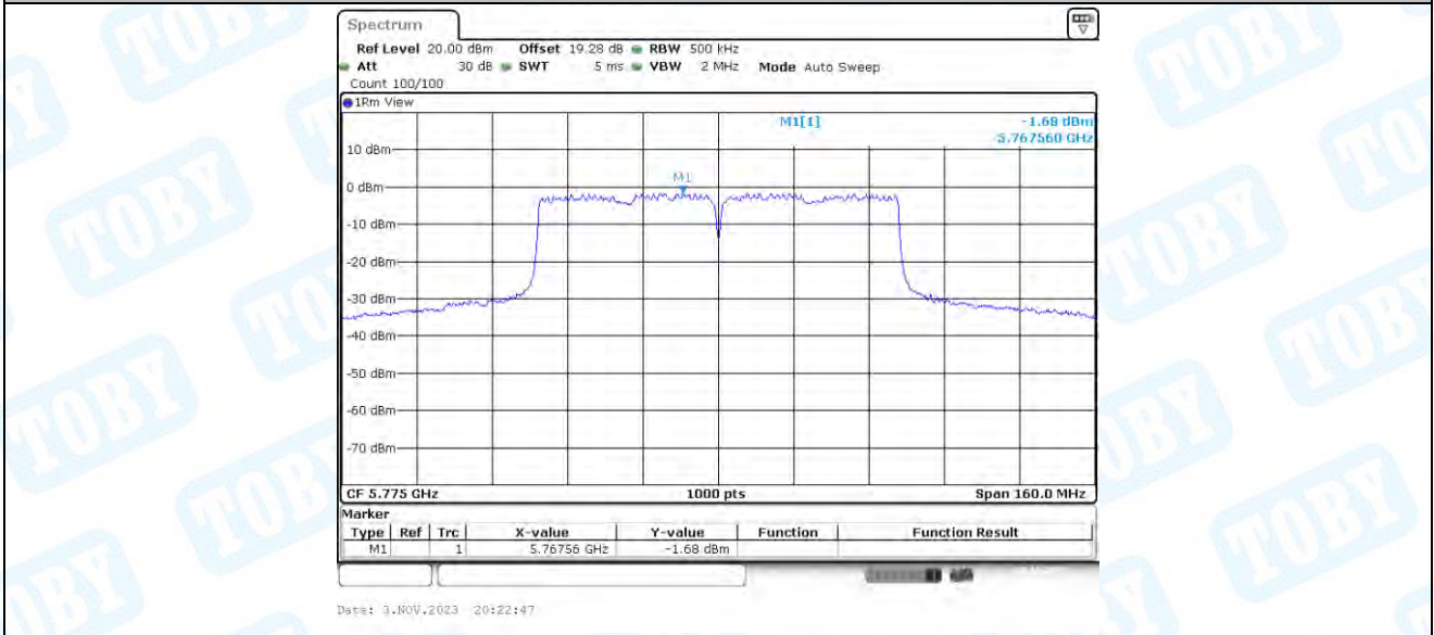
11AC80-BF_Ant2_5775
