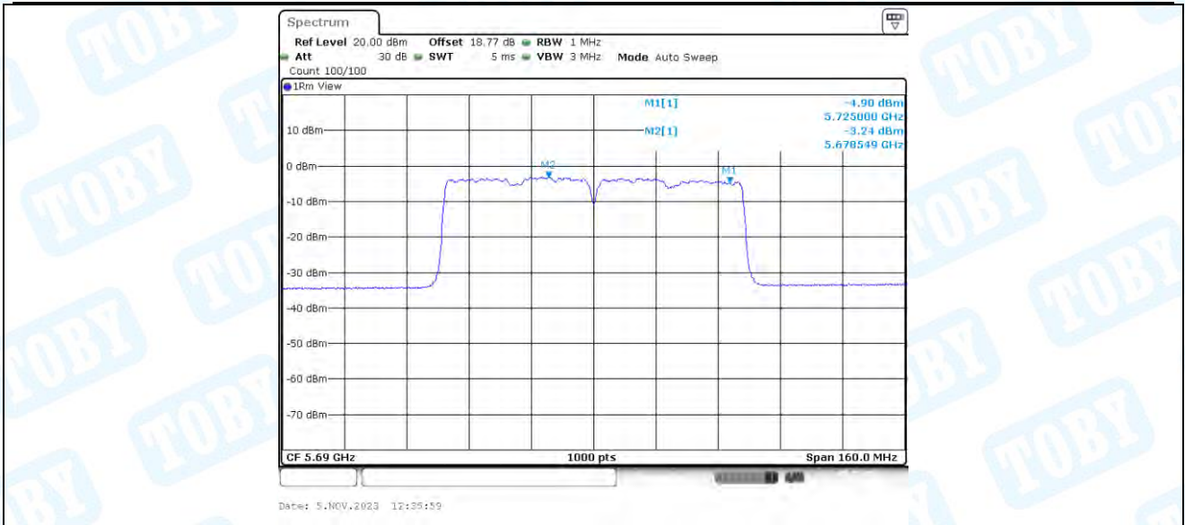
11AC80-BF_Ant3_5690_UNII-2C
