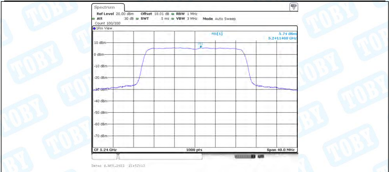
11AX20-BF_Ant4_5240
