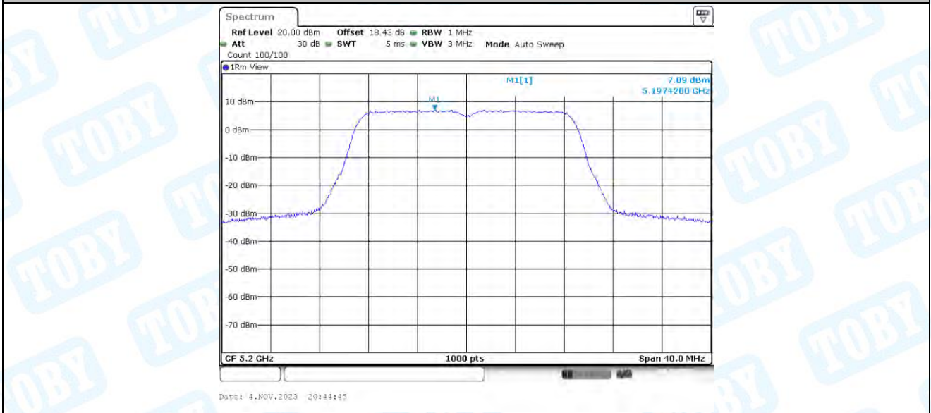
11AC20-BF_Ant3_5200
