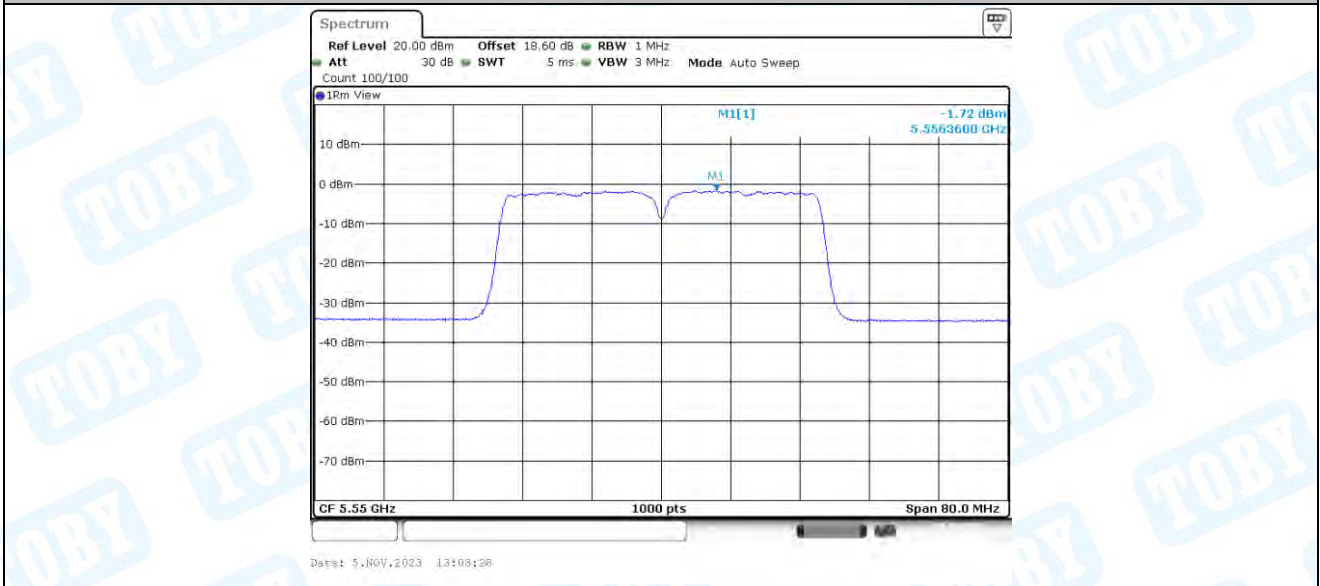
11AC40-BF_Ant3_5550
