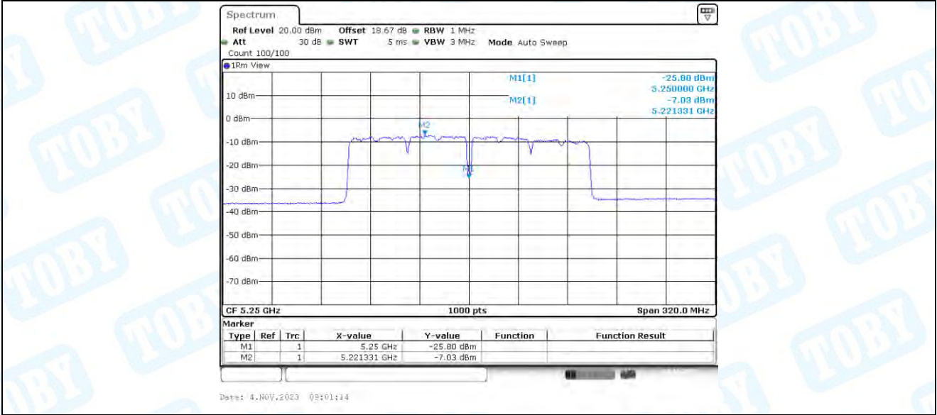
11AC160-BF_Ant4_5250_UNII-1
