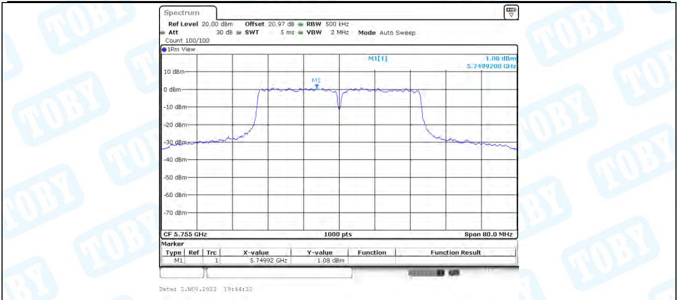
11N40-BF_Ant4_5755
