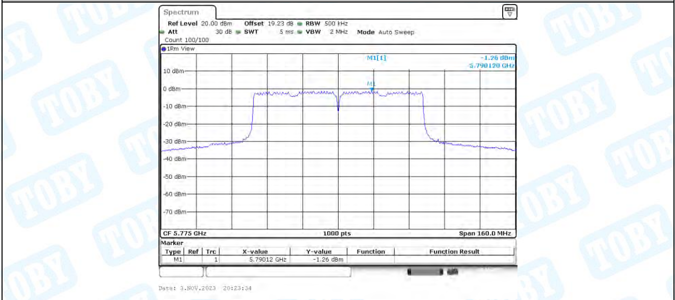
11AC80-BF_Ant3_5775
