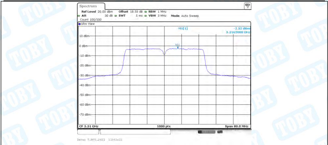
11AC40-BF_Ant2_5510
