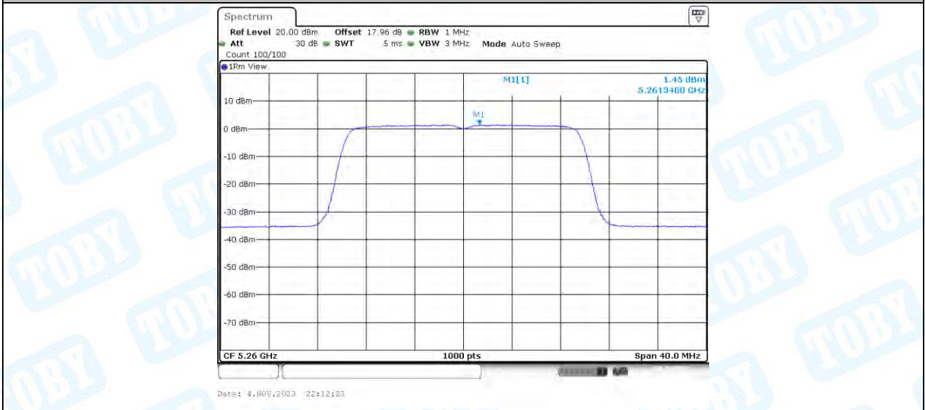
11AX20-BF_Ant2_5260
