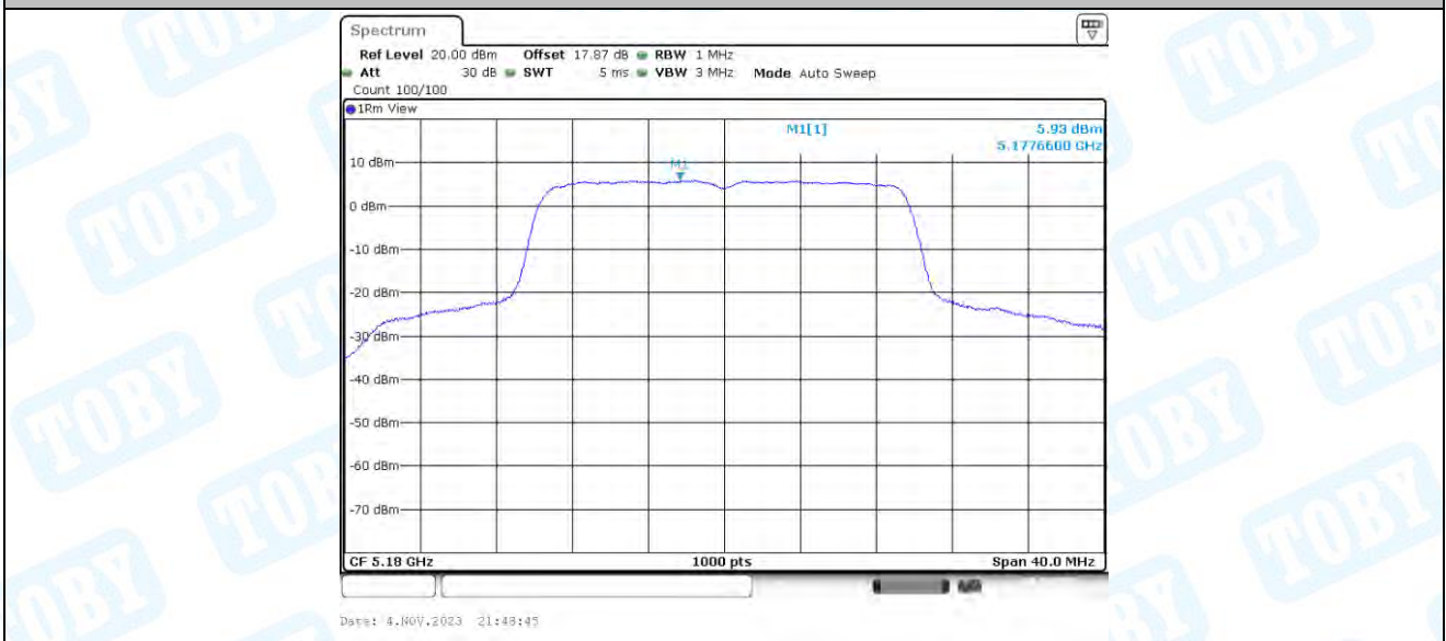
11AX20-BF_Ant2_5180
