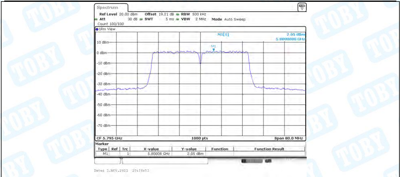
11AC40-BF_Ant2_5795
