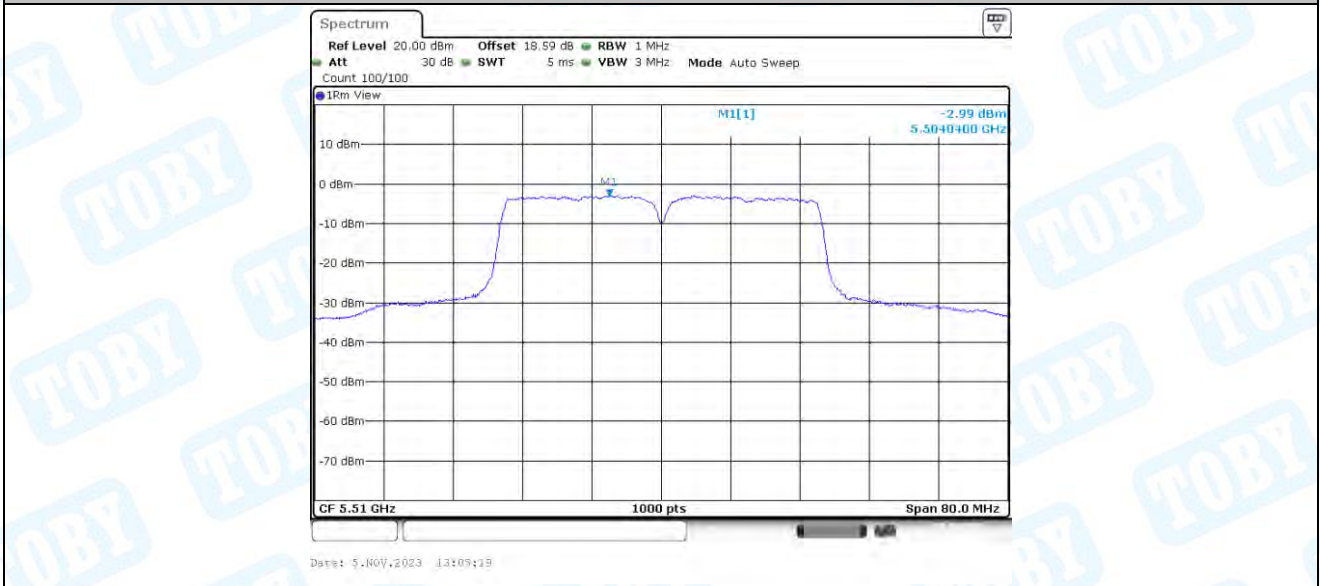
11AC40-BF_Ant4_5510
