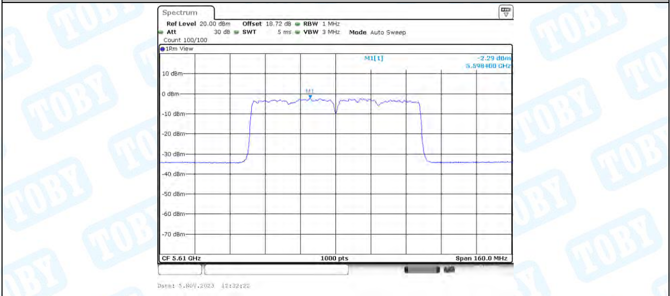
11AC80-BF_Ant2_5610
