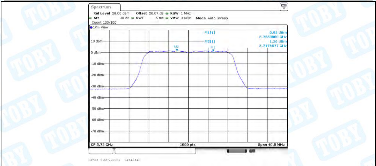
11N20-BF_Ant3_5720_UNII-2C
