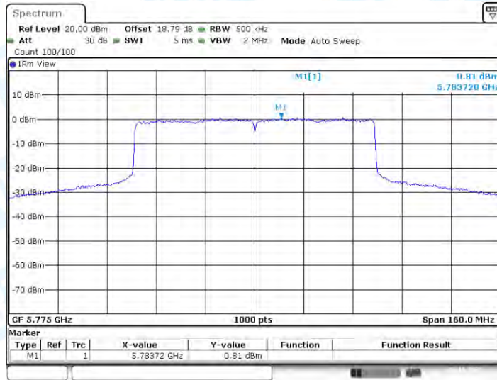
11AX80-CDD_Ant4_5775
