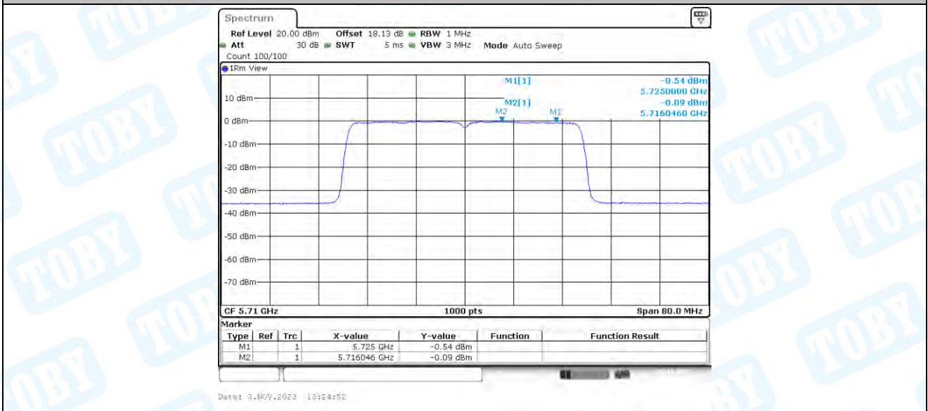
11AX40-CDD_Ant3_5710_UNII-2C
