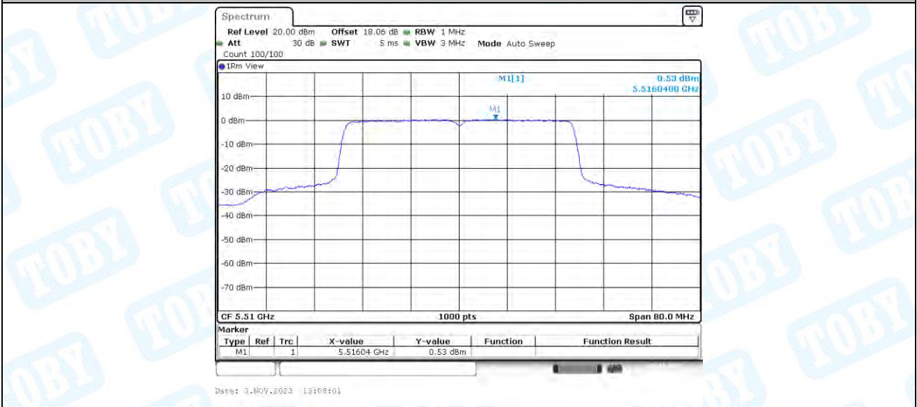
11AX40-CDD_Ant3_5510
