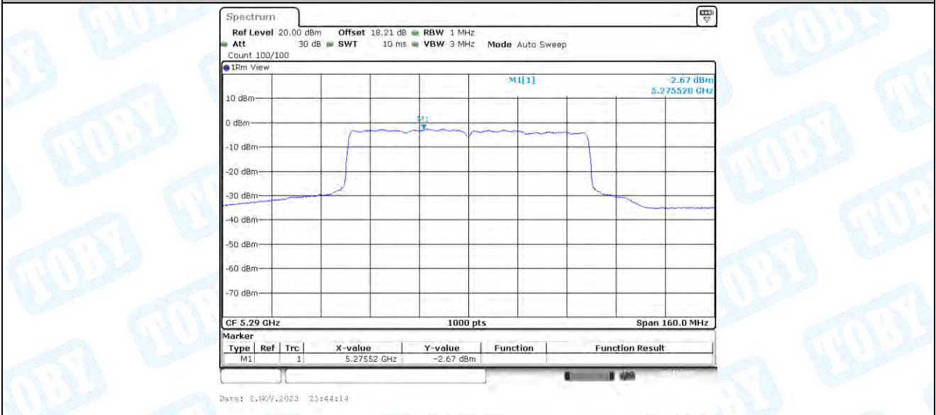
11AX80-CDD_Ant4_5290
