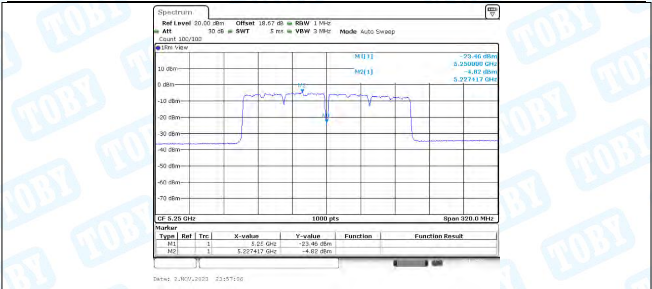
11AC160-CDD_Ant4_5250_UNII-1
