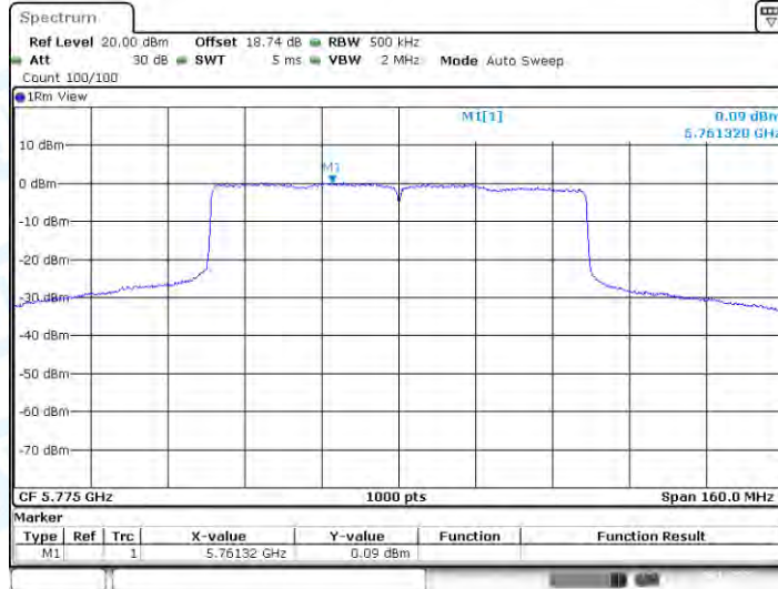
11AX80-CDD_Ant3_5775
