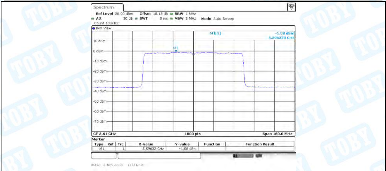
11AX80-CDD_Ant3_5610
