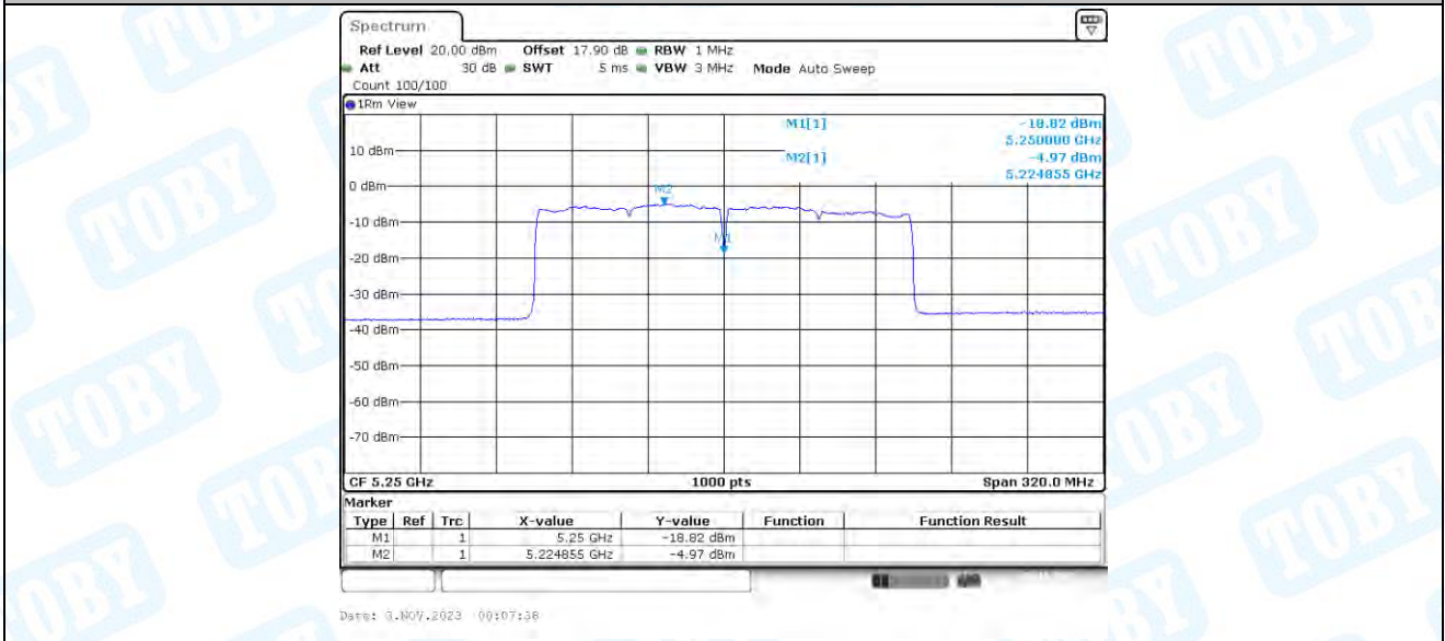
11AX160-CDD_Ant4_5250_UNII-1
