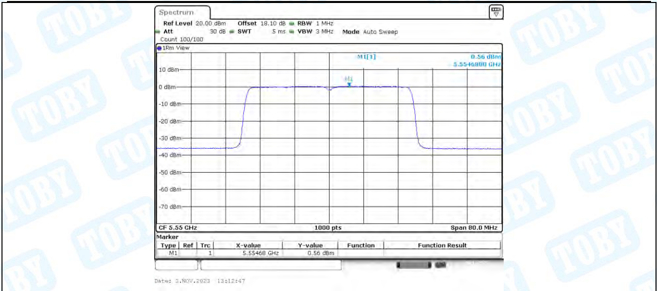
11AX40-CDD_Ant3_5550
