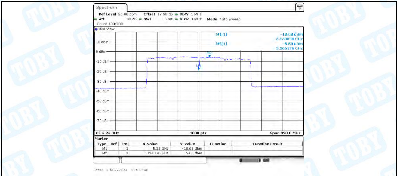
11AX160-CDD_Ant4_5250_UNII-2A
