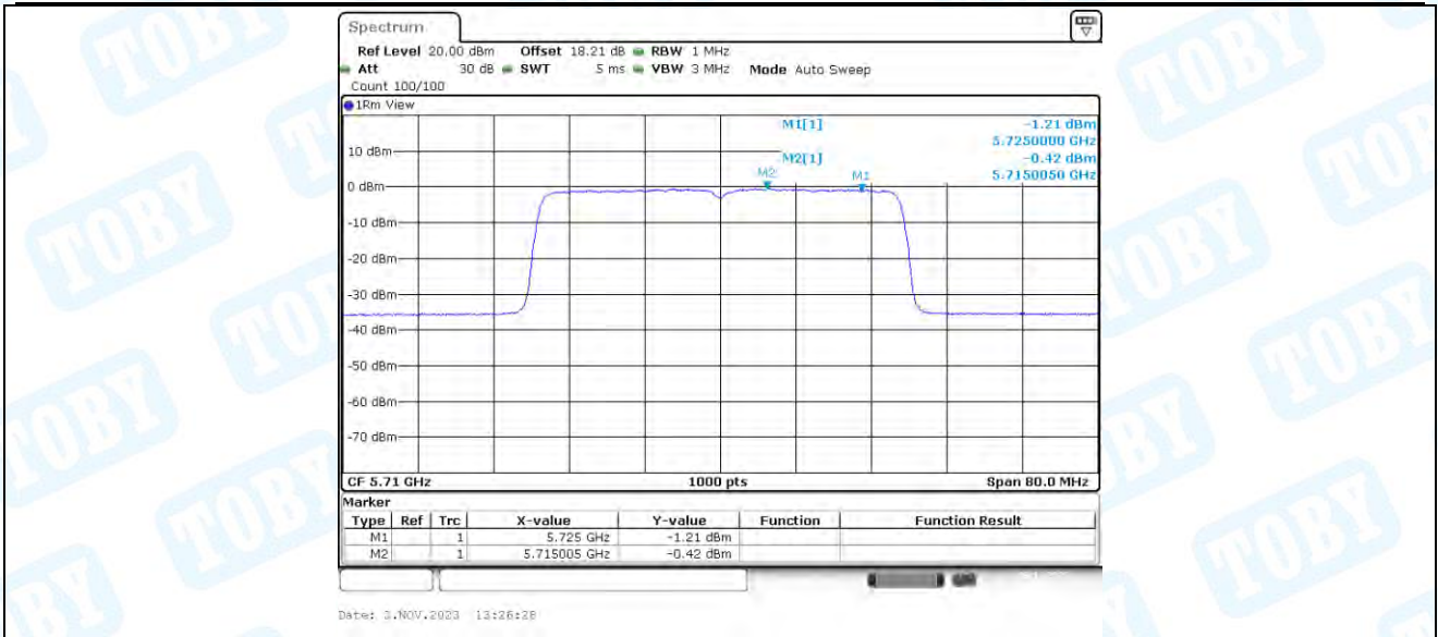
11AX40-CDD_Ant4_5710_UNII-2C
