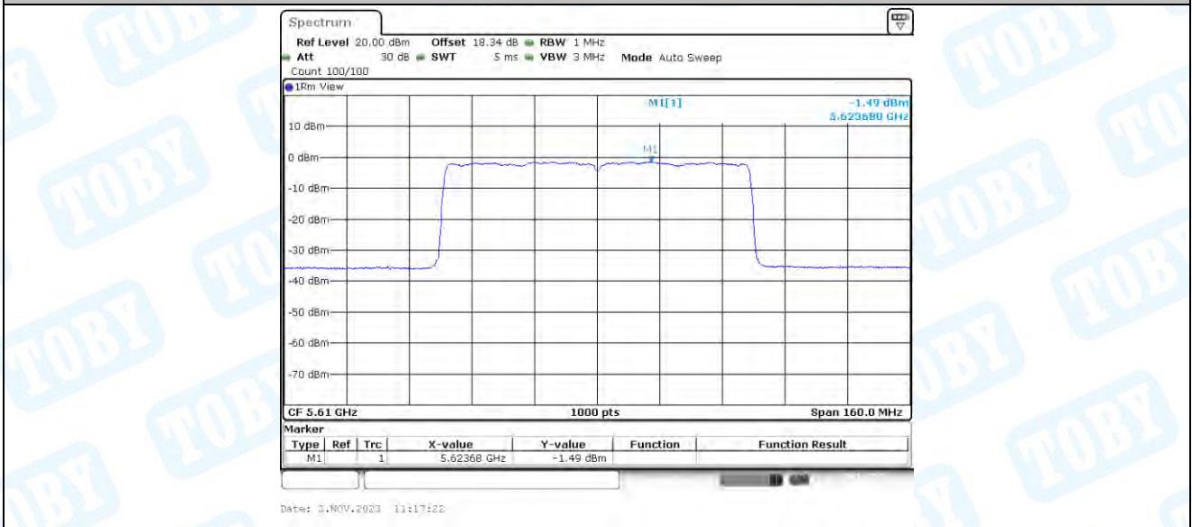
11AX80-CDD_Ant4_5610
