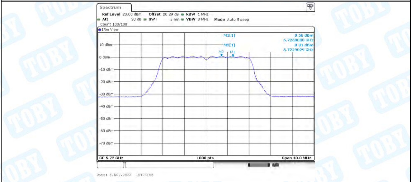
11A-BF_Ant4_5720_UNII-2C
