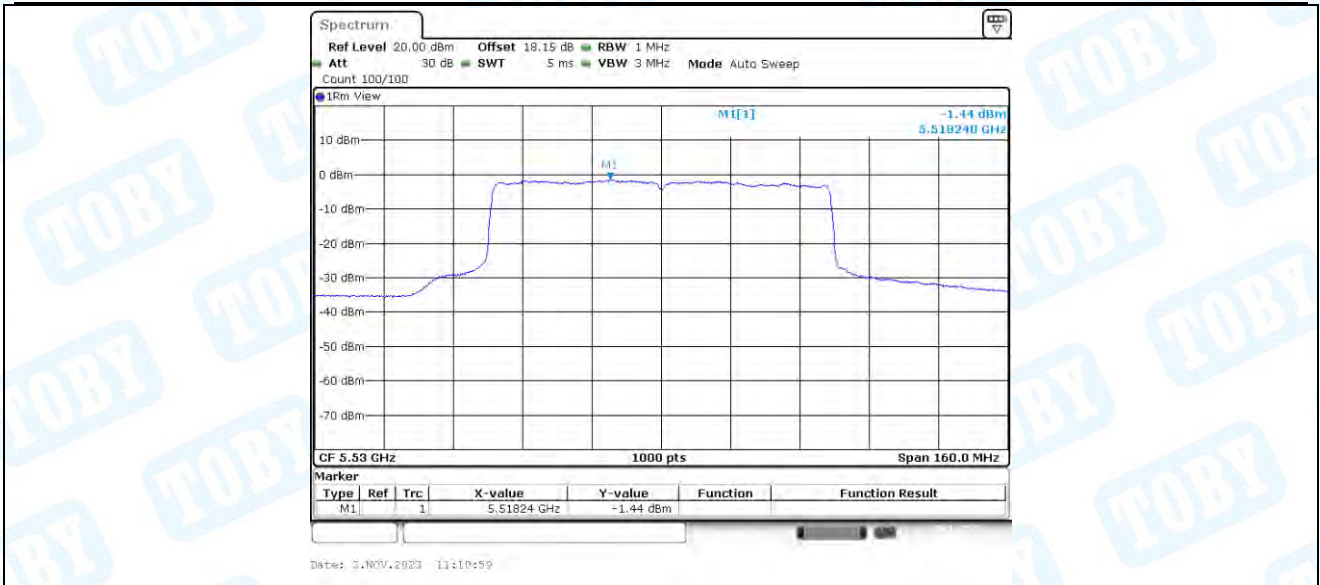
11AX80-CDD_Ant4_5530
