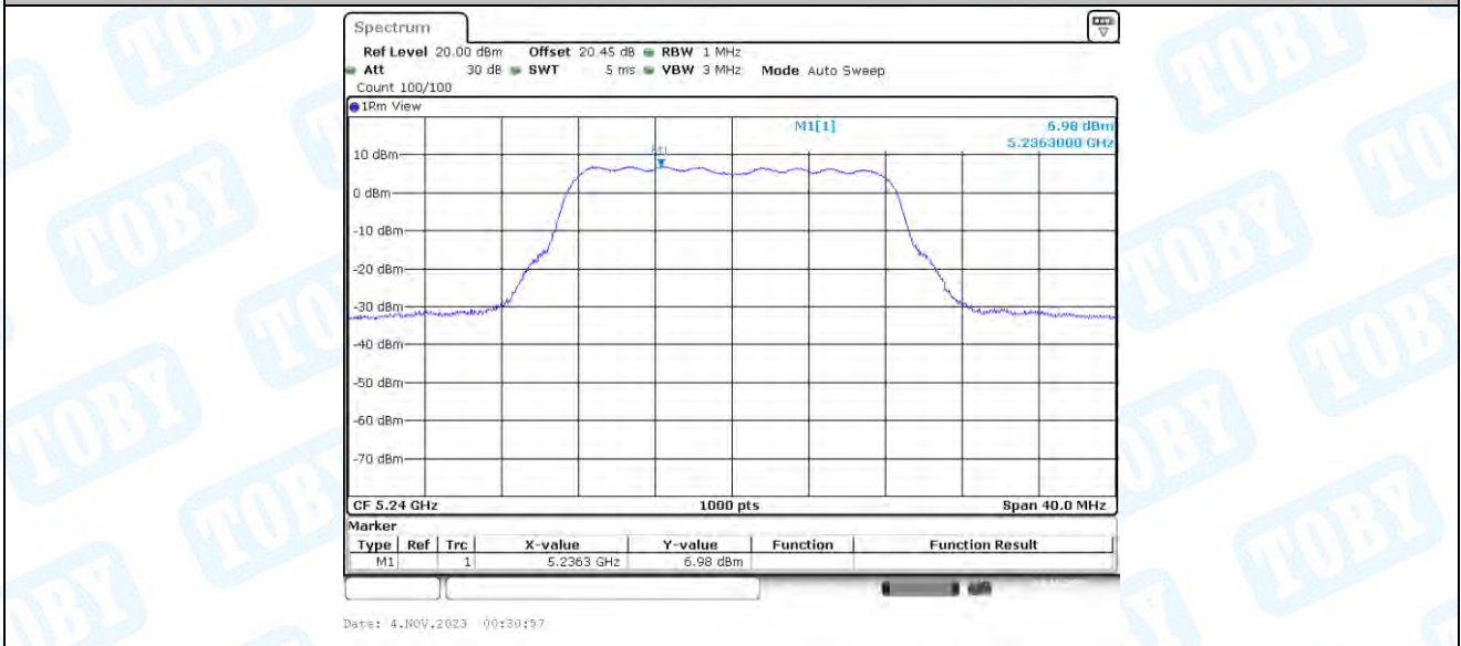
11A-BF_Ant4_5240
