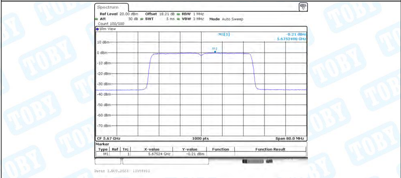
11AX40-CDD_Ant4_5670
