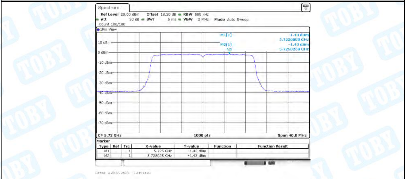
11AX20-CDD_Ant4_5720_UNII-3
