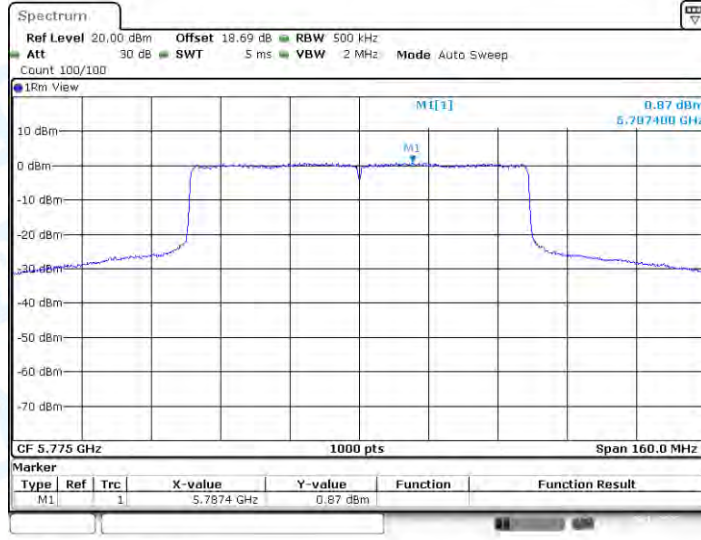
11AX80-CDD_Ant3_5775
