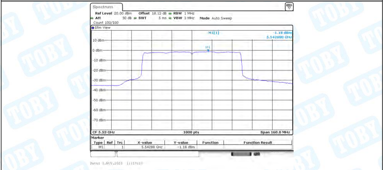
11AX80-CDD_Ant3_5530
