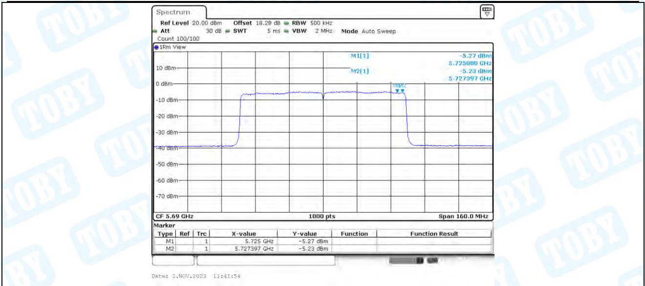
11AX80-CDD_Ant4_5690_UNII-3
