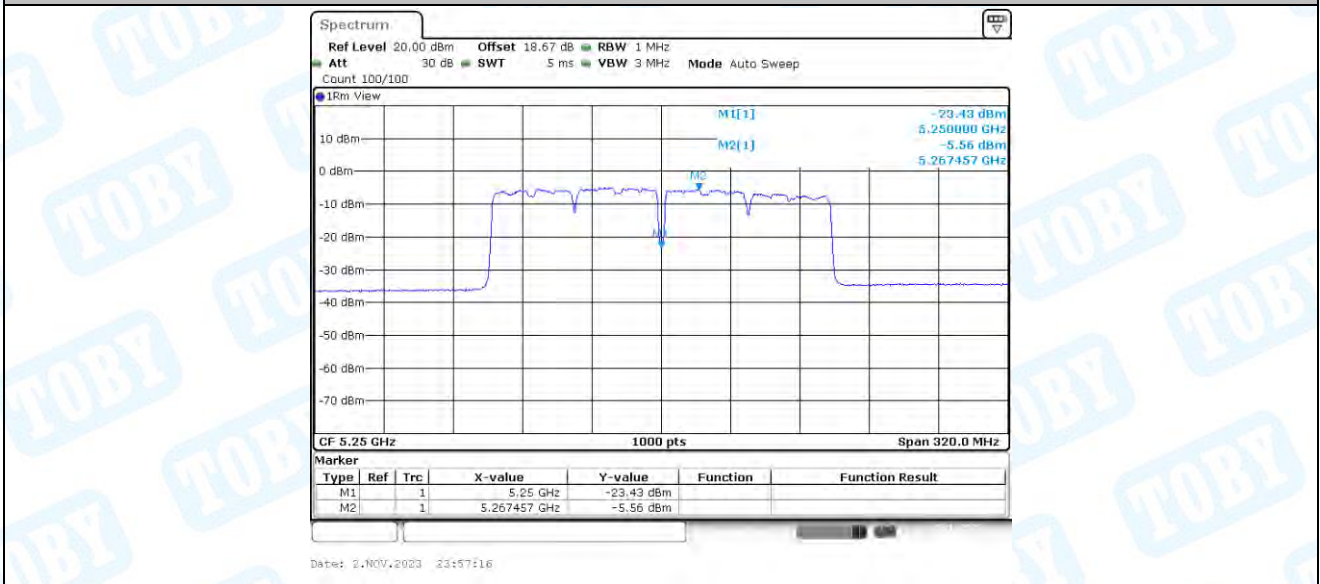
11AC160-CDD_Ant4_5250_UNII-2A
