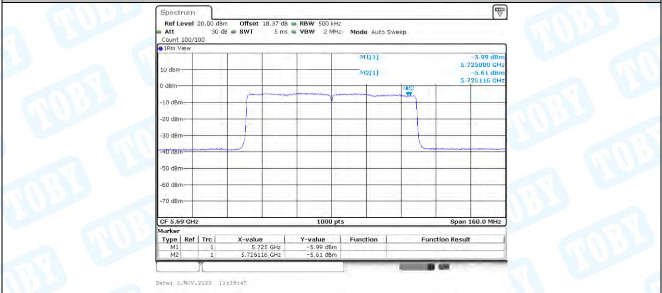
11AX80-CDD_Ant2_5690_UNII-3
