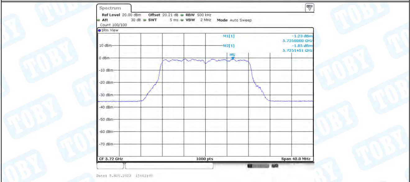
11A-BF_Ant3_5720_UNII-3
