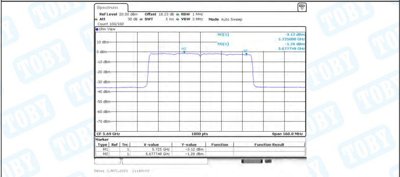
11AX80-CDD_Ant3_5690_UNII-2C
