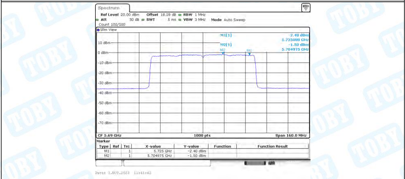
11AX80-CDD_Ant4_5690_UNII-2C
