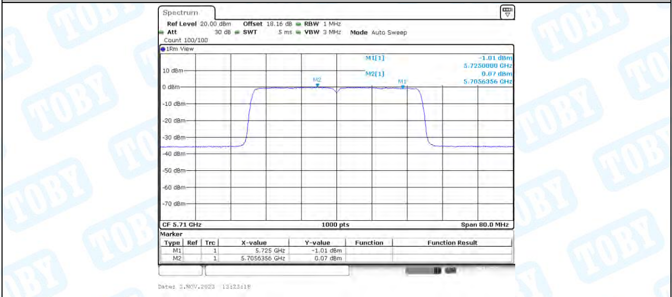
11AX40-CDD_Ant2_5710_UNII-2C
