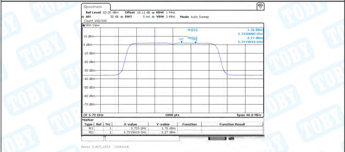
11AX20-CDD_Ant3_5720_UNII-2C
