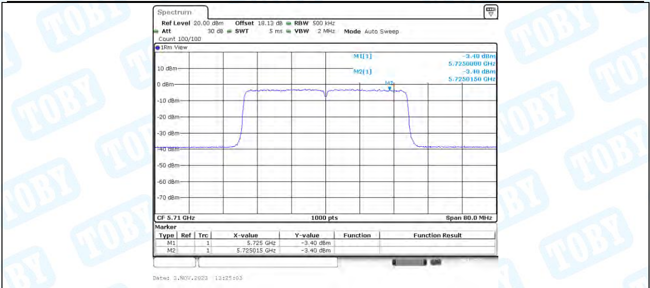
11AX40-CDD_Ant3_5710_UNII-3
