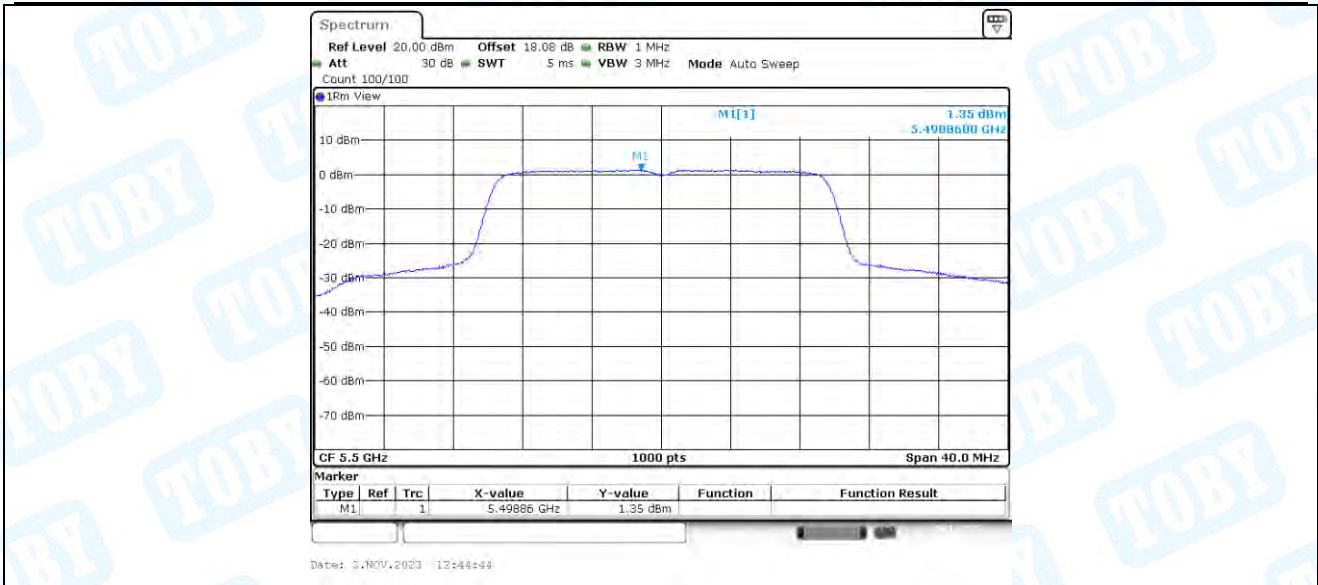
11AX20-CDD_Ant4_5500
