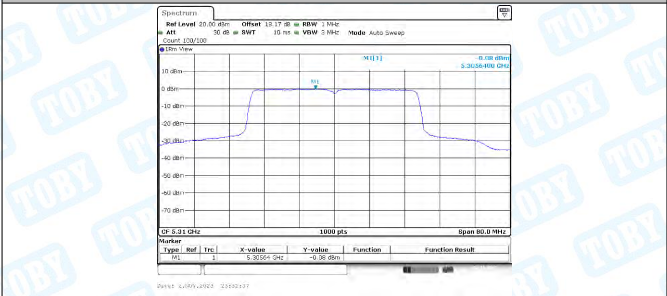
11AX40-CDD_Ant4_5310
