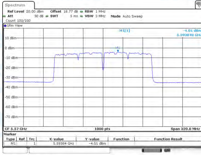
11AC160-CDD_Ant2_5570
