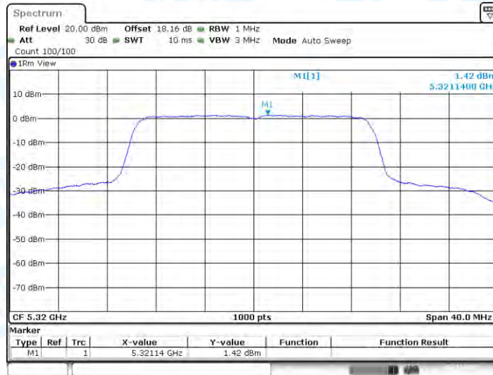
11AX20-CDD_Ant3_5320
