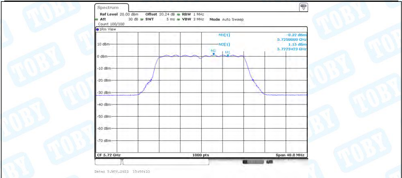
11A-BF_Ant2_5720_UNII-2C
