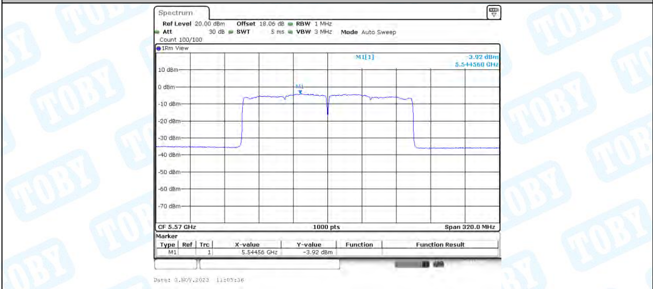
11AX160-CDD_Ant4_5570
