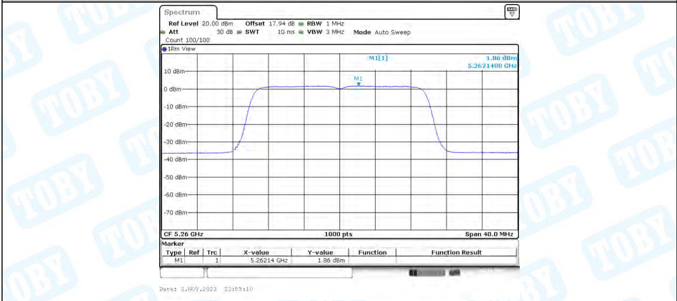
11AX20-CDD_Ant3_5260
