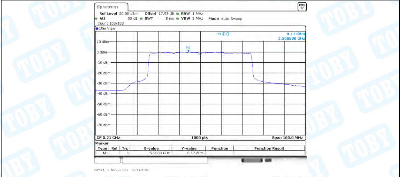
11AX80-CDD_Ant4_5210
