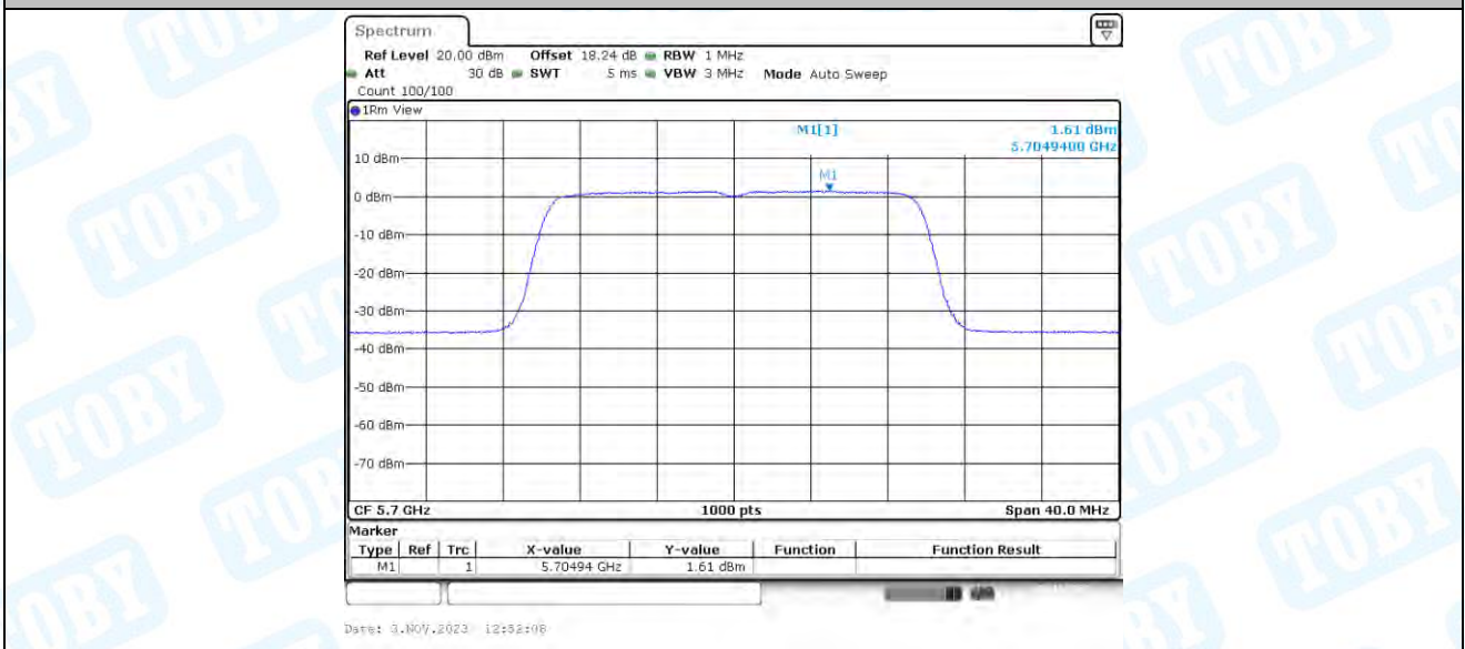
11AX20-CDD_Ant4_5700
