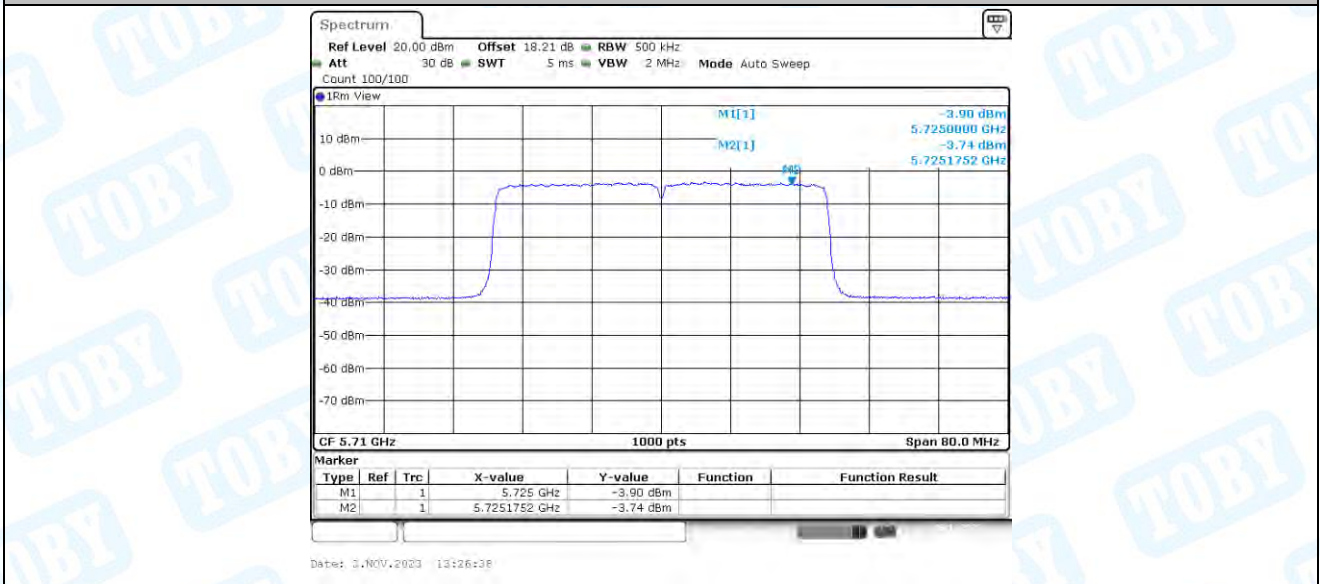
11AX40-CDD_Ant4_5710_UNII-3
