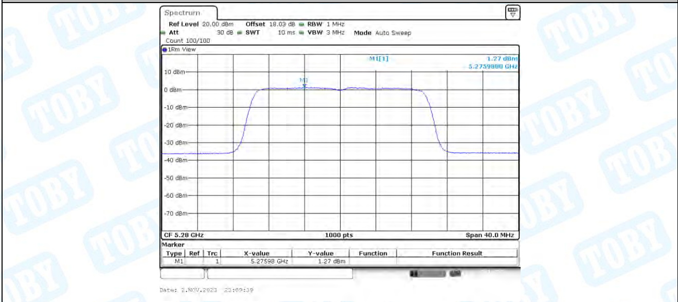
11AX20-CDD_Ant4_5280
