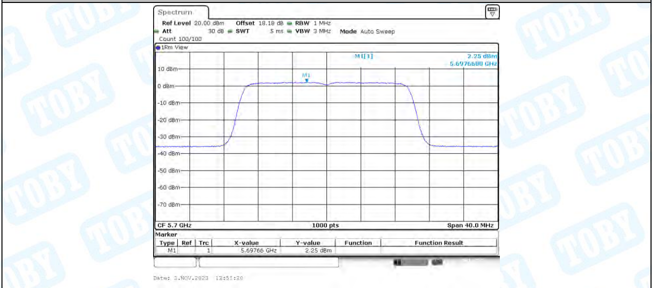
11AX20-CDD_Ant3_5700
