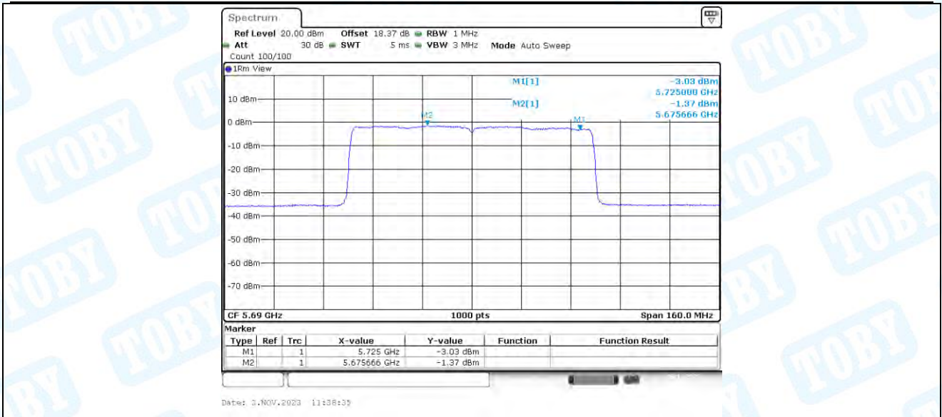
11AX80-CDD_Ant2_5690_UNII-2C
