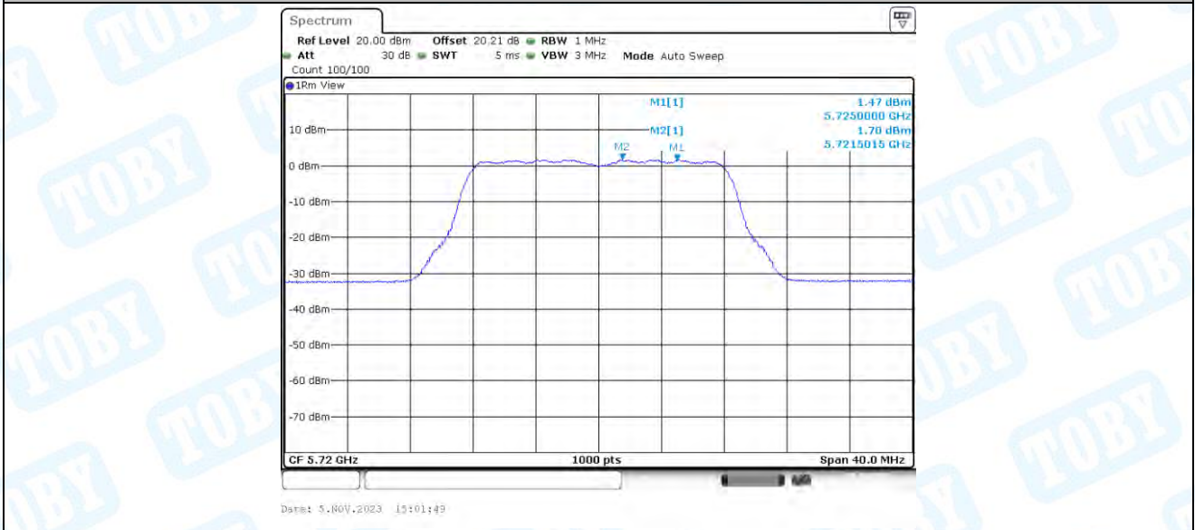
11A-BF_Ant3_5720_UNII-2C
