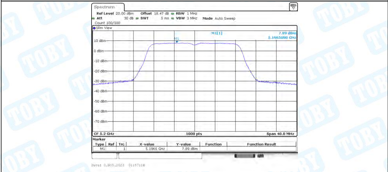
11AC20-CDD_Ant4_5200
