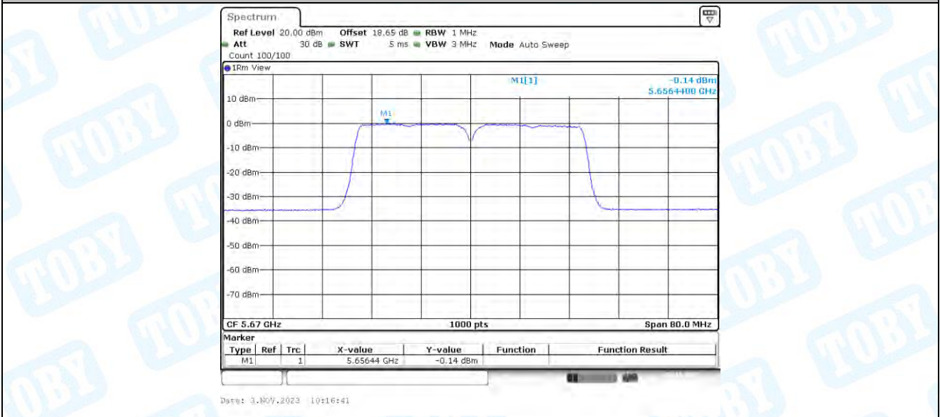
11AC40-CDD_Ant3_5670
