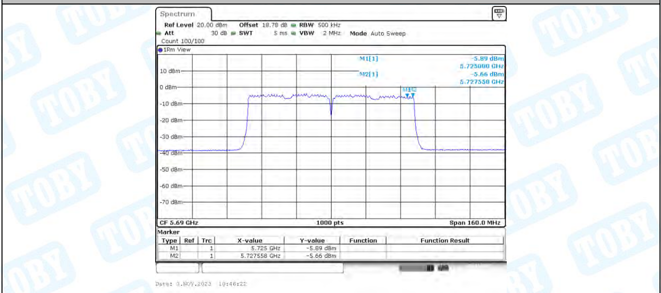
11AC80-CDD_Ant2_5690_UNII-3
