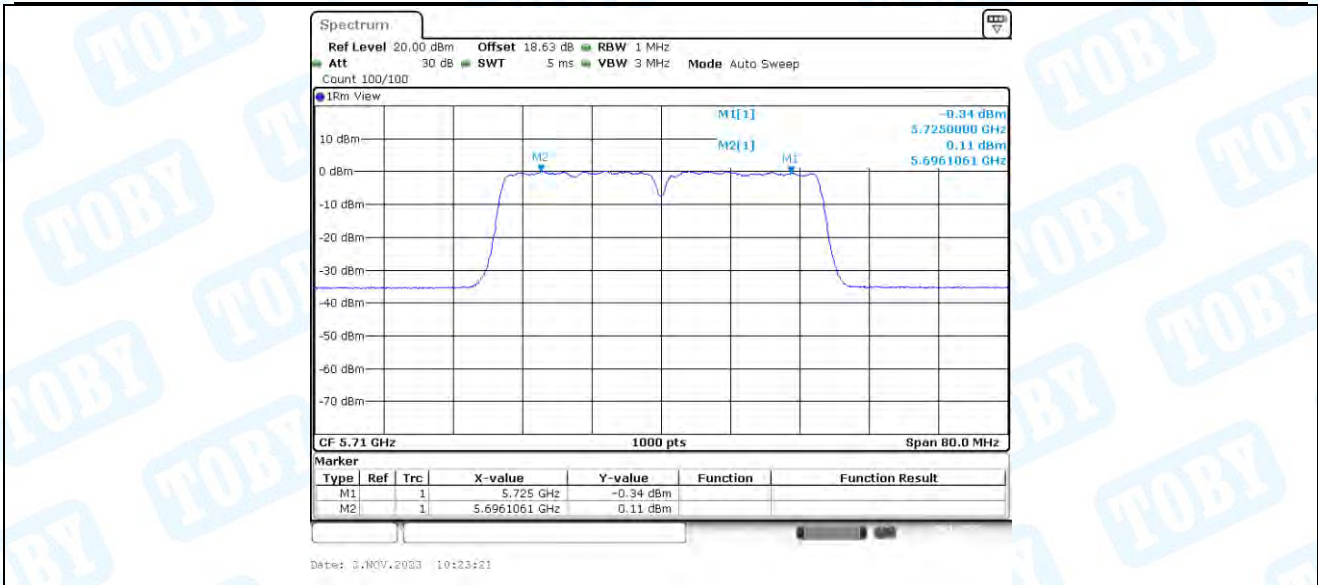
11AC40-CDD_Ant3_5710_UNII-2C
