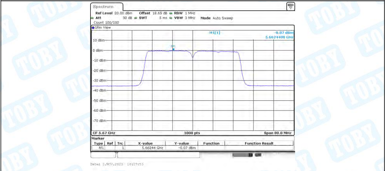
11AC40-CDD_Ant2_5670
