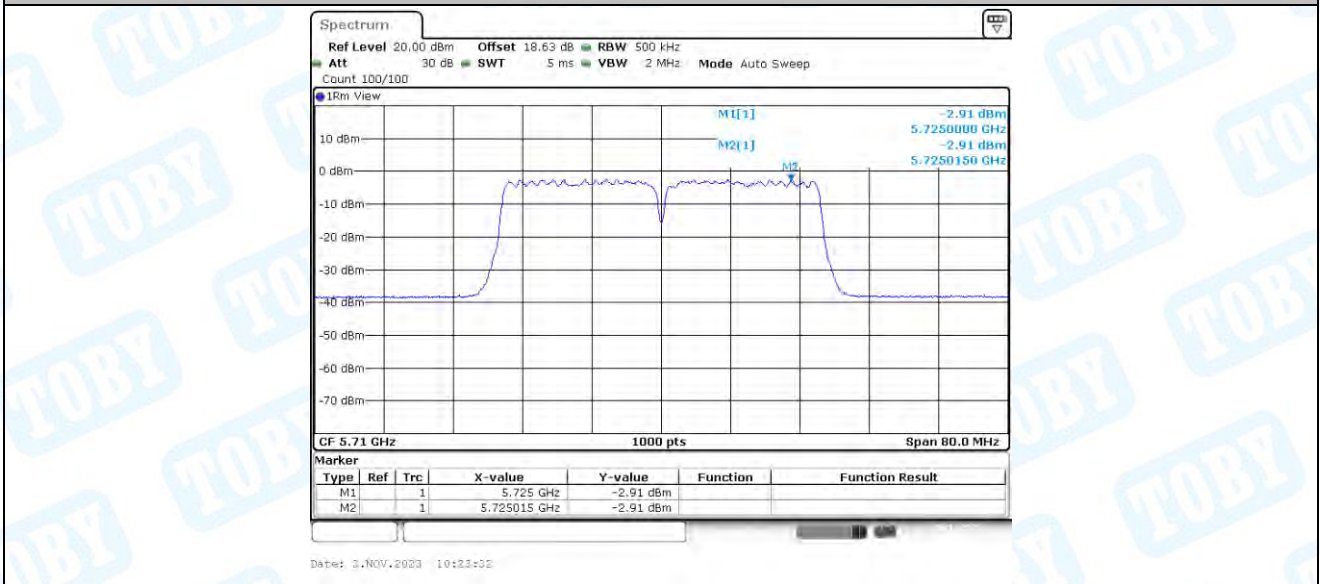
11AC40-CDD_Ant3_5710_UNII-3
