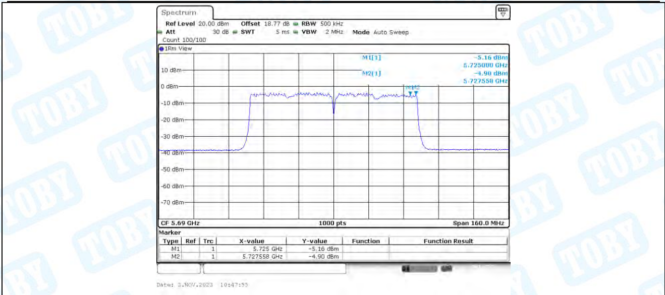
11AC80-CDD_Ant3_5690_UNII-3
