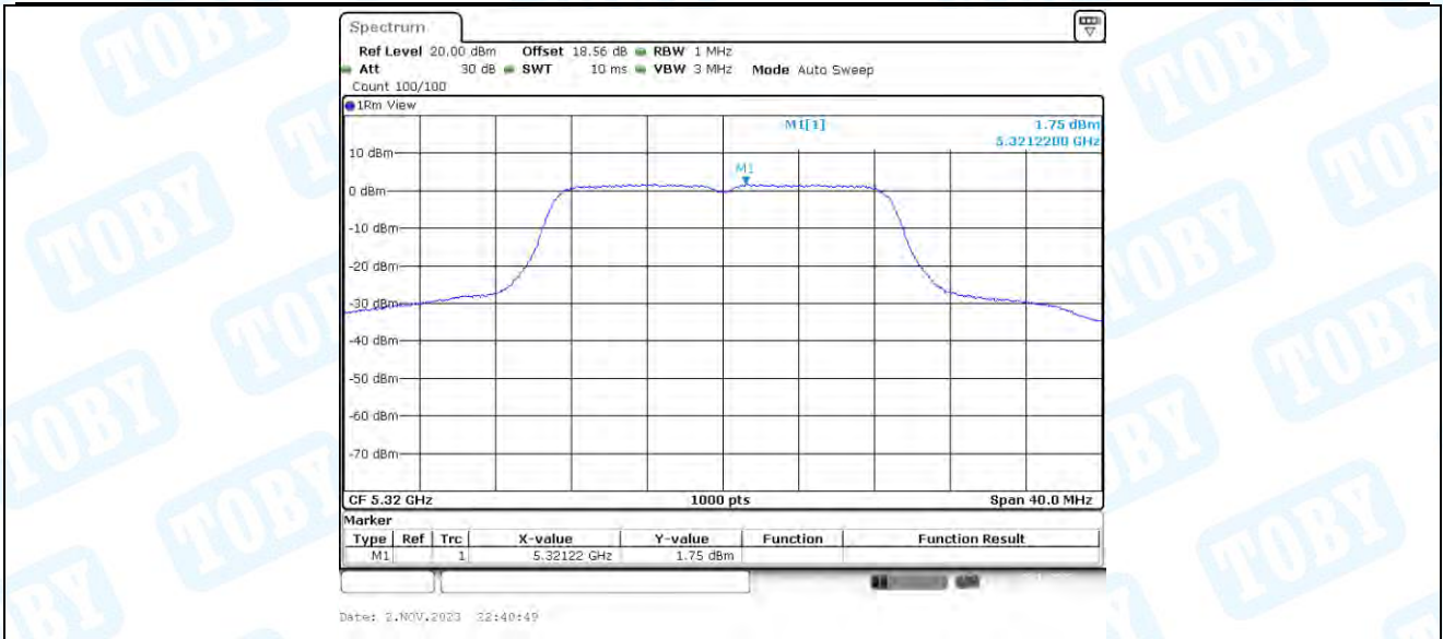
11AC20-CDD_Ant4_5320
