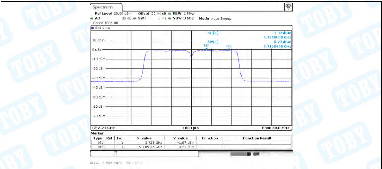
11N40-CDD_Ant4_5710_UNII-2C
