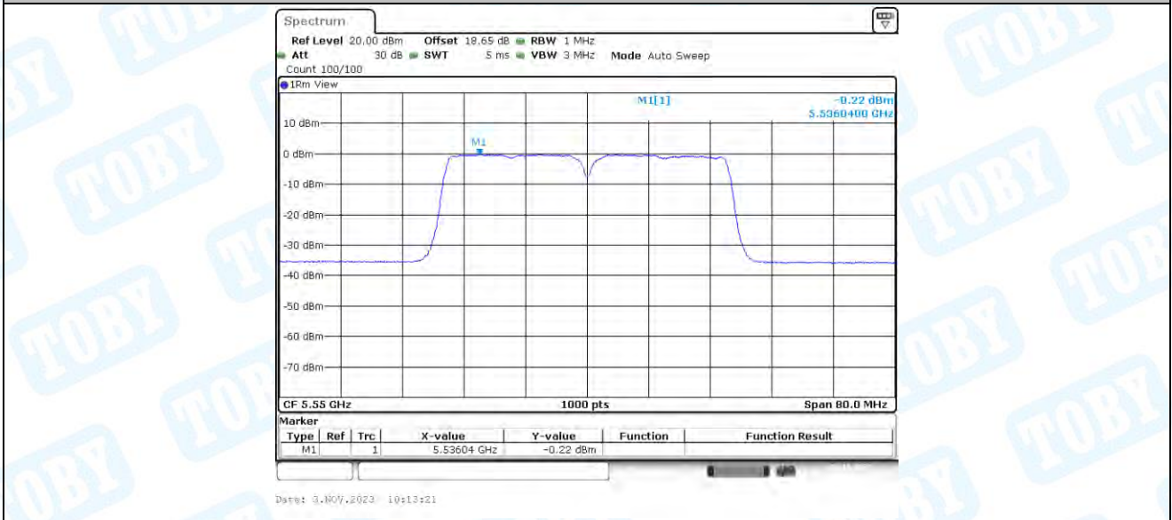
11AC40-CDD_Ant4_5550
