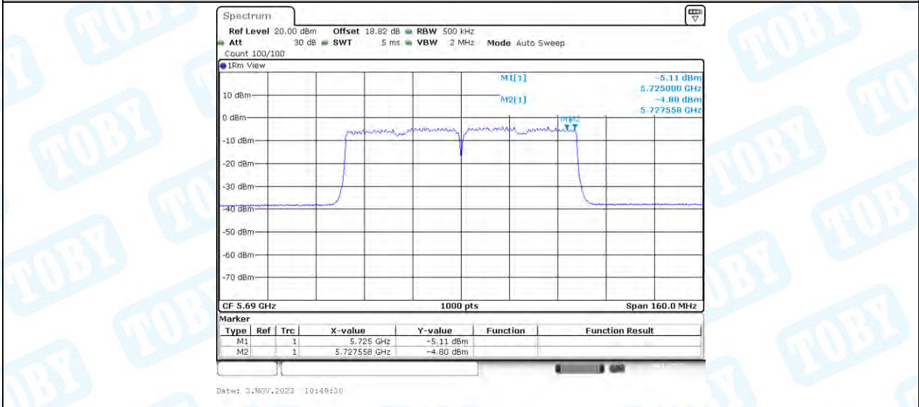
11AC80-CDD_Ant4_5690_UNII-3
