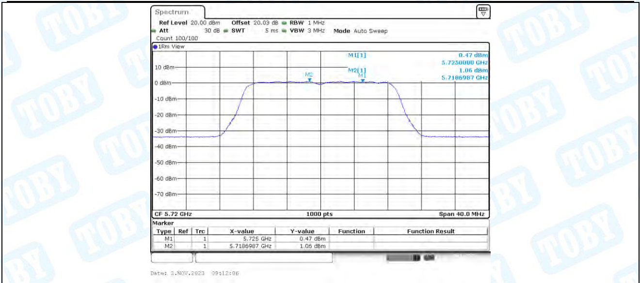
11N20-CDD_Ant4_5720_UNII-2C
