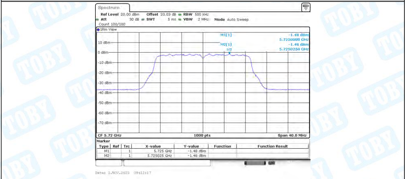
11N20-CDD_Ant4_5720_UNII-3
