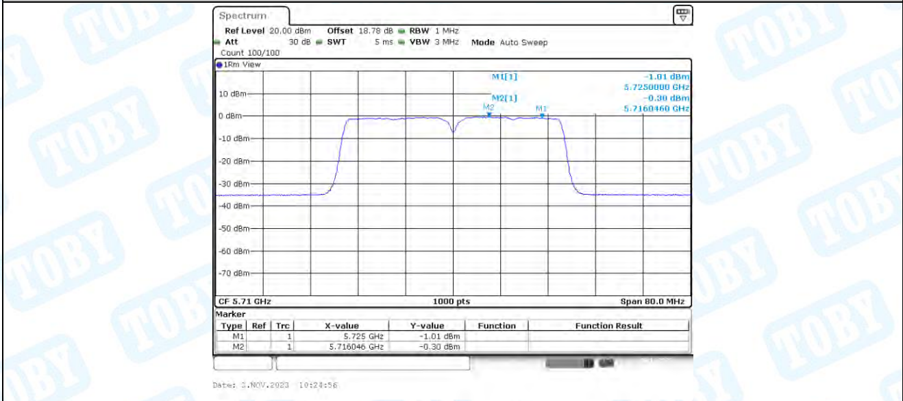
11AC40-CDD_Ant4_5710_UNII-2C
