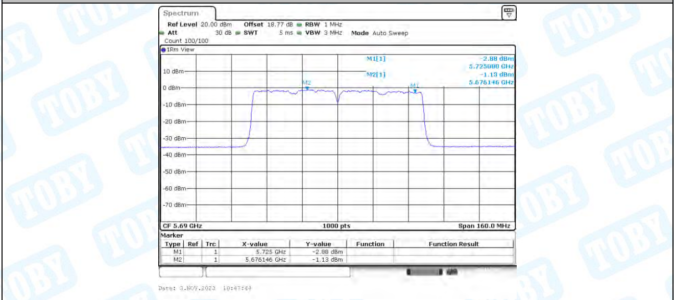
11AC80-CDD_Ant3_5690_UNII-2C
