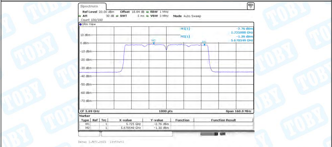
11AC80-CDD_Ant1_5690_UNII-3
