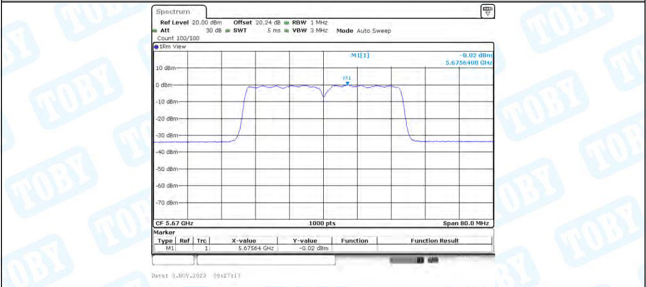
11N40-CDD_Ant4_5670
