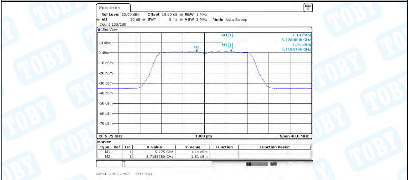
11AC20-CDD_Ant4_5720_UNII-2C
