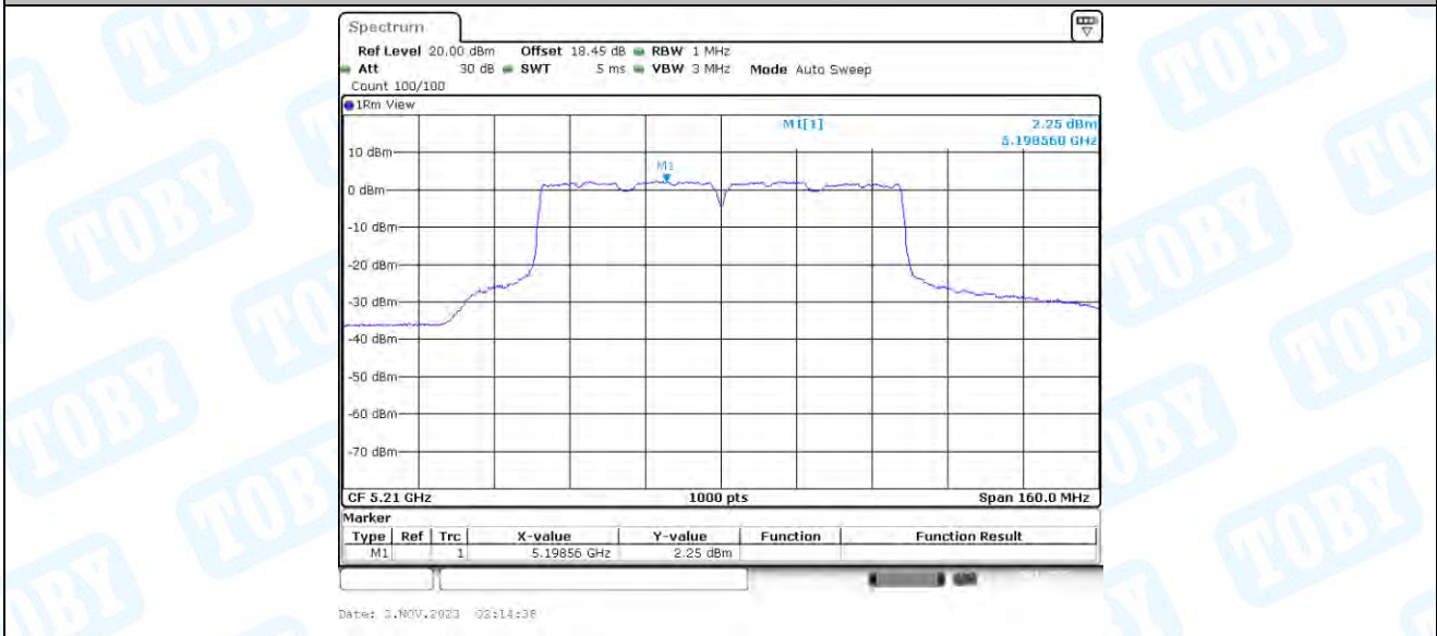
11AC80-CDD_Ant3_5210
