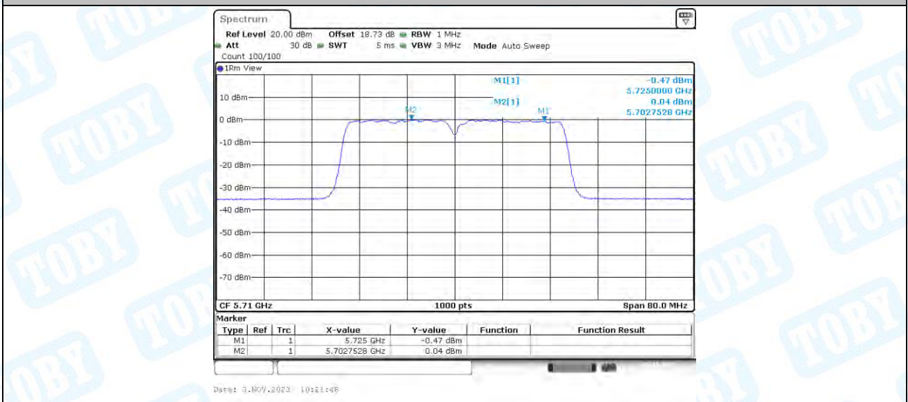
11AC40-CDD_Ant2_5710_UNII-2C
