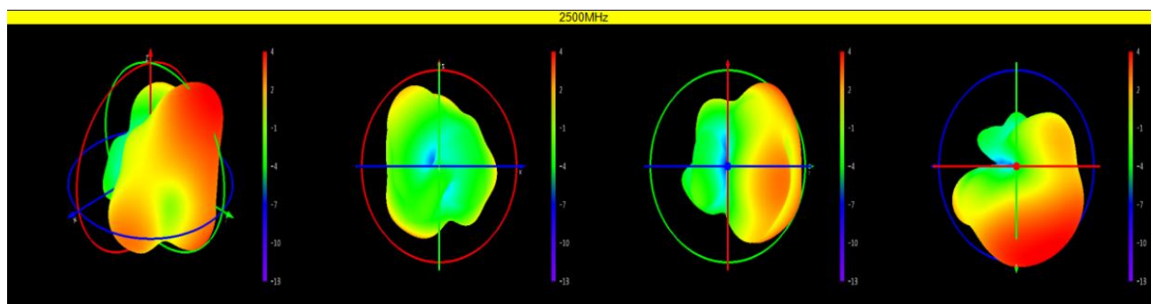
Phi=90 freq=2500MHz
