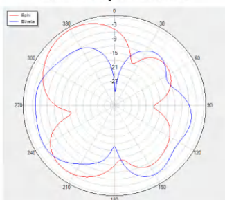
Phi=0 freq=2450MHz
