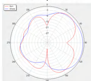
Phi=90 freq=2500MHz
