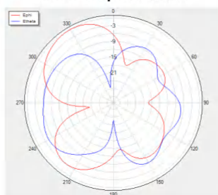
Phi=0 freq=2500MHz
