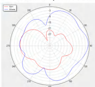
Theta=90 freq=2450MHz
