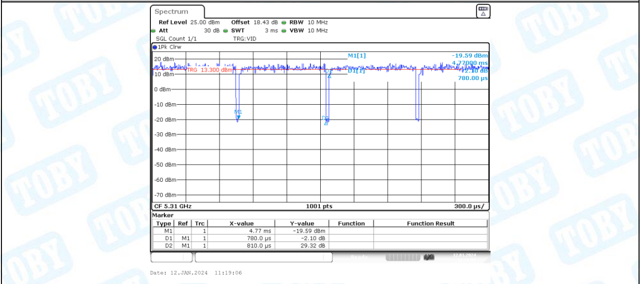
11AX40-CDD_Ant2_5310
