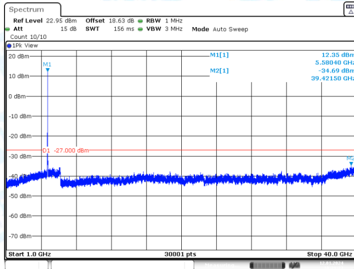
11AX20-CDD_Ant2_5580_1000~40000
