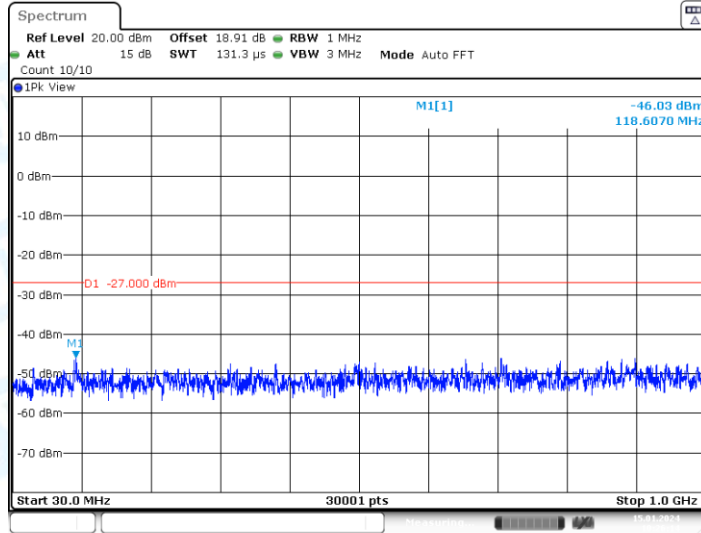
11AC80-CDD_Ant2_5690_30~1000
