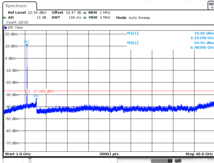
11AX20-CDD_Ant1_5260_1000~40000
