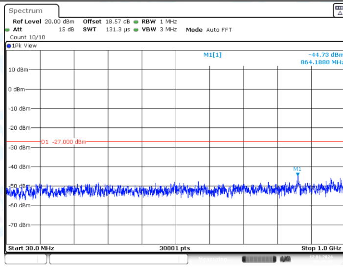
11AX20-CDD_Ant2_5240_30~1000
