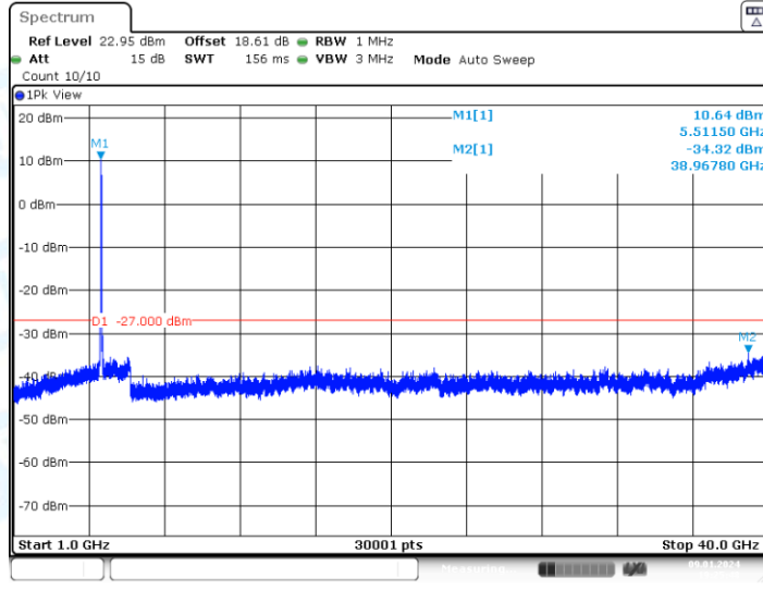
11AC40-CDD_Ant2_5510_1000~40000
