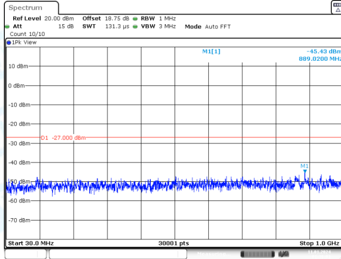
11AC40-CDD_Ant2_5755_30~1000
