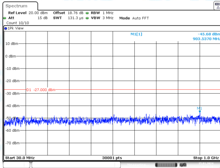
11AC80-CDD_Ant2_5775_30~1000
