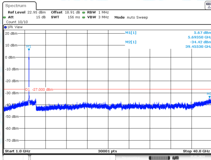
11AC80-CDD_Ant2_5690_1000~40000
