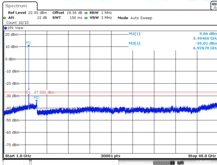
11AX20-CDD_Ant1_5500_1000~40000
