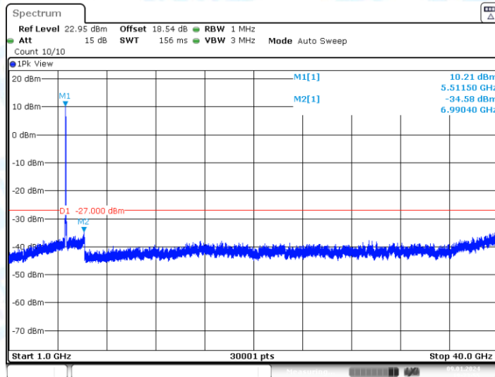
11AC40-CDD_Ant1_5510_1000~40000
