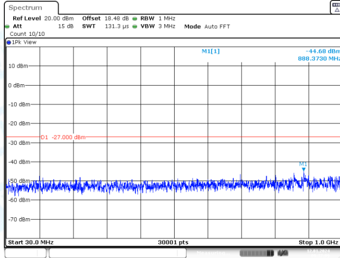
11AX20-CDD_Ant2_5200_30~1000
