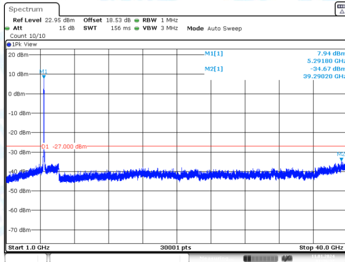
11AC80-CDD_Ant2_5290_1000~40000
