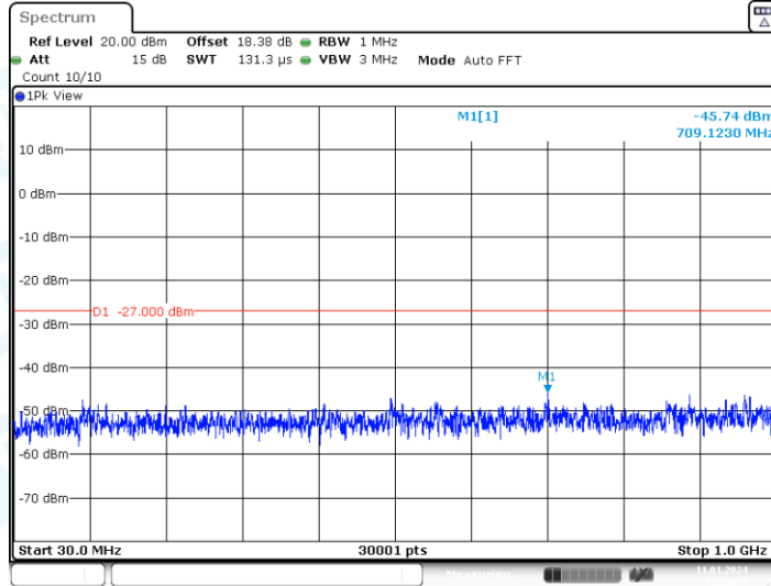
11AC80-CDD_Ant1_5210_30~1000
