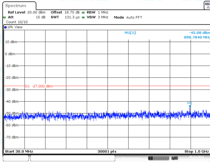
11AC20-CDD_Ant2_5745_30~1000
