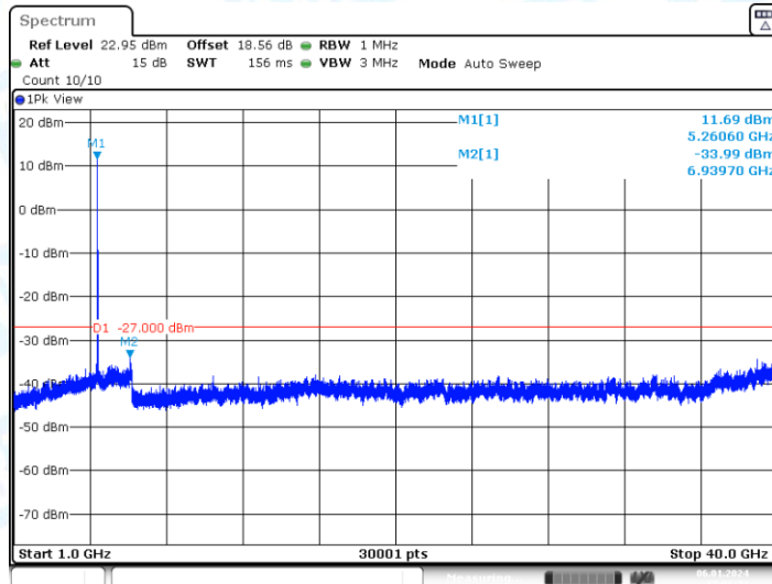
11AC20-CDD_Ant2_5260_1000~40000
