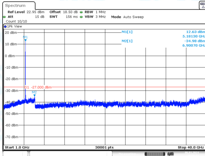
11AC20-CDD_Ant2_5180_1000~40000
