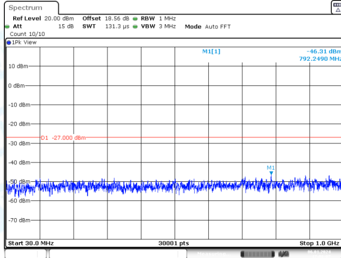
11AC20-CDD_Ant2_5260_30~1000
