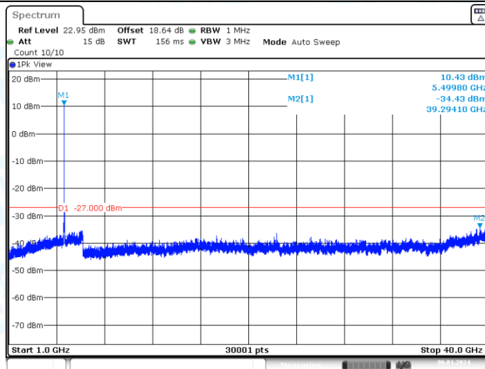
11AC20-CDD_Ant2_5500_1000~40000
