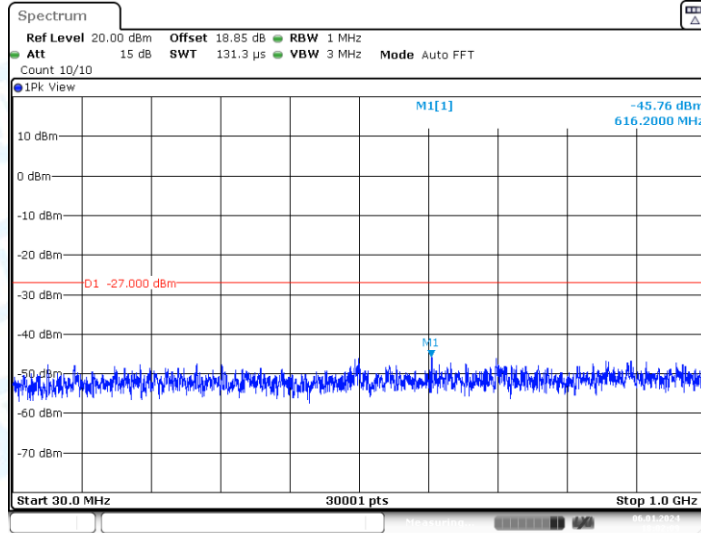
11AC20-CDD_Ant2_5825_30~1000
