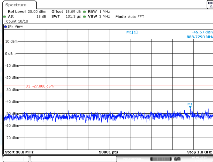
11AC20-CDD_Ant1_5785_30~1000
