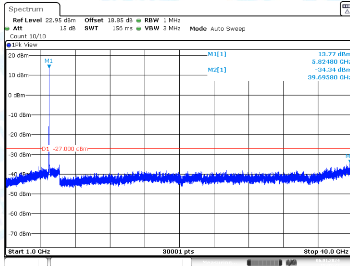
11AC20-CDD_Ant2_5825_1000~40000
