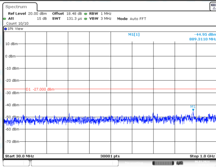
11AC40-CDD_Ant2_5190_30~1000
