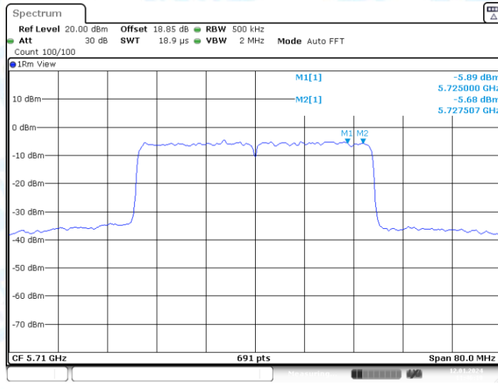
11AX40-CDD_Ant2_5710_UNII-3
