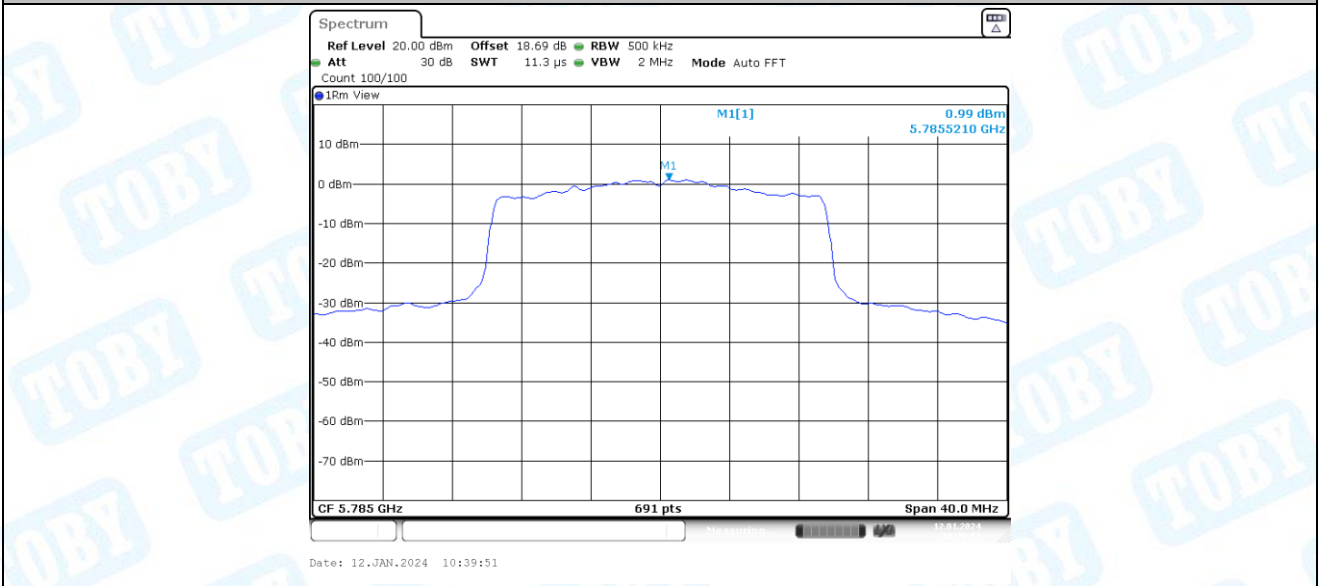
11AX20-CDD_Ant2_5785
