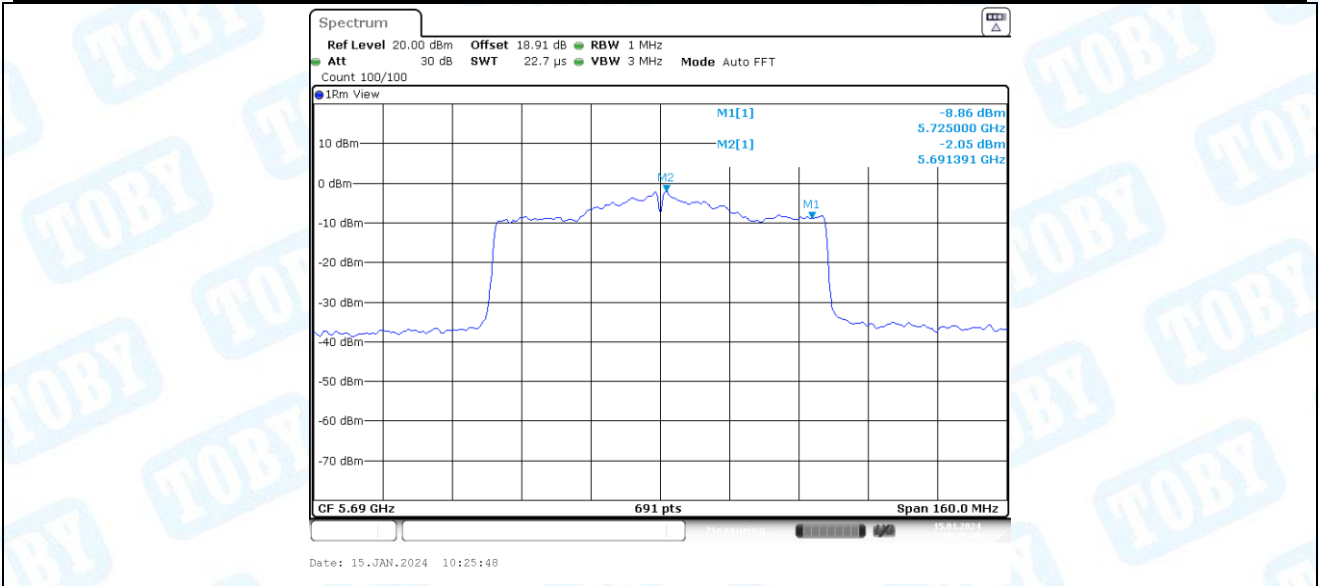
11AC80-CDD_Ant1_5690_UNII-3
