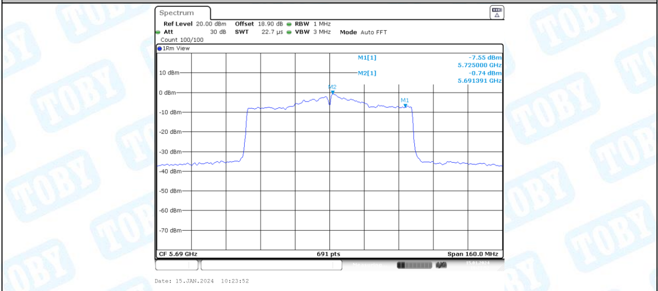
11AC80-CDD_Ant2_5690_UNII-2C
