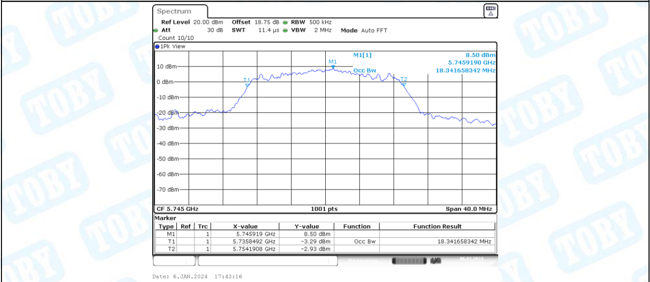
11AC20-CDD_Ant2_5745
