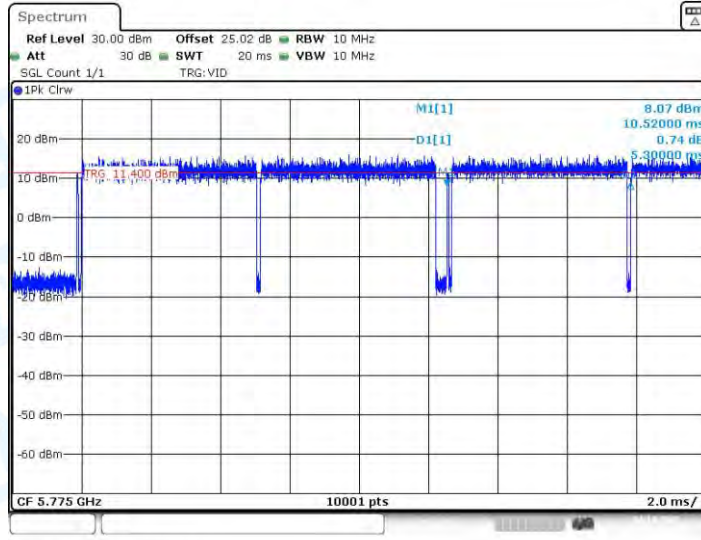
11AC80-BF_Ant2_5775
