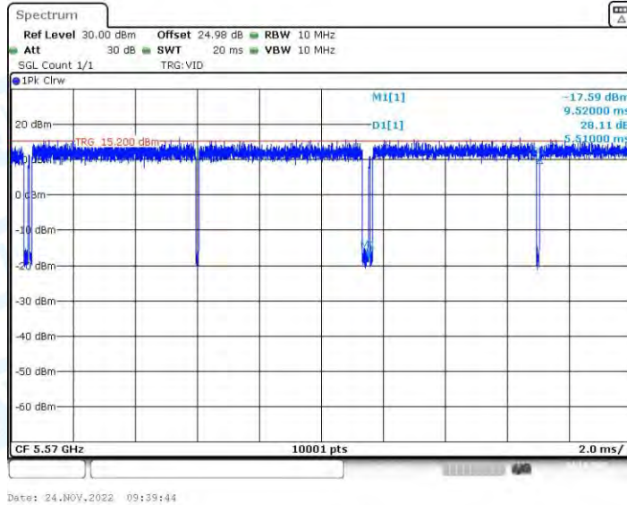
11AC160-BF_Ant2_5570
