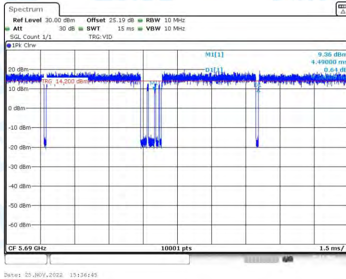
11AX80-BF_Ant2_5690
