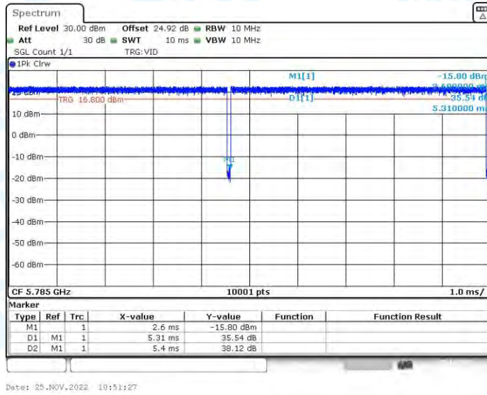
11AX20-BF_Ant2_5785
