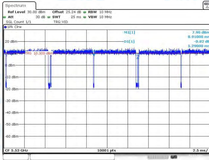
11AC80-BF_Ant2_5530
