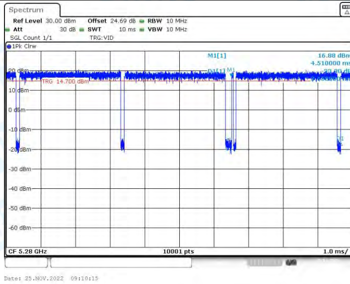
11AX20-BF_Ant2_5280
