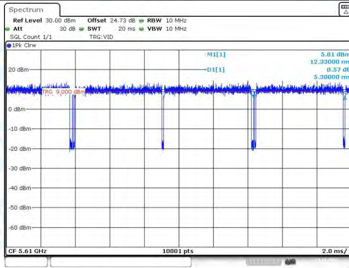
11AC80-BF_Ant1_5610
