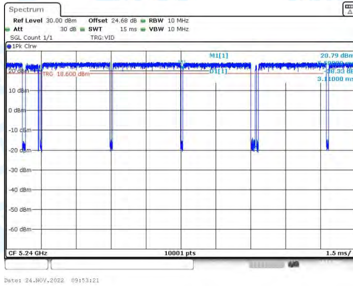
11AX20-BF_Ant2_5240
