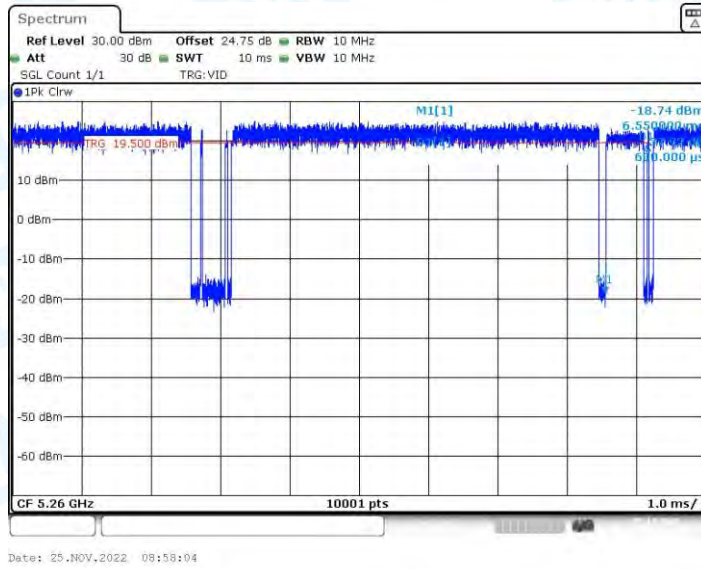
11AX20-BF_Ant2_5260
