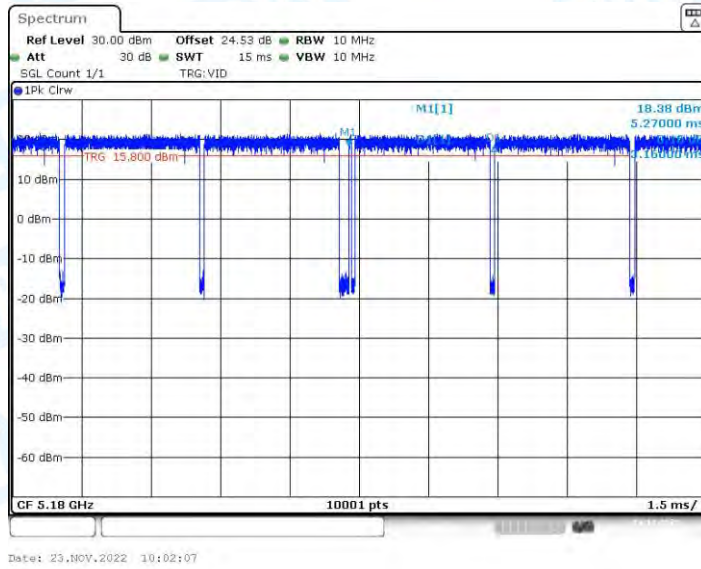
11AX20-BF_Ant2_5180
