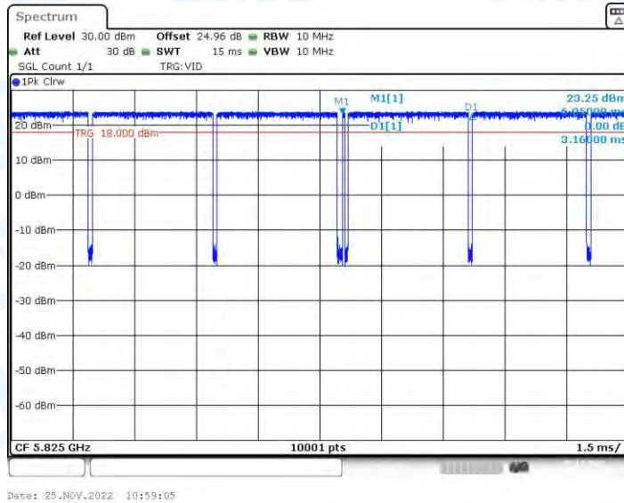
11AX20-BF_Ant2_5825
