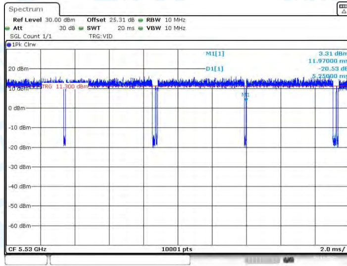
11AC80-BF_Ant2_5530
