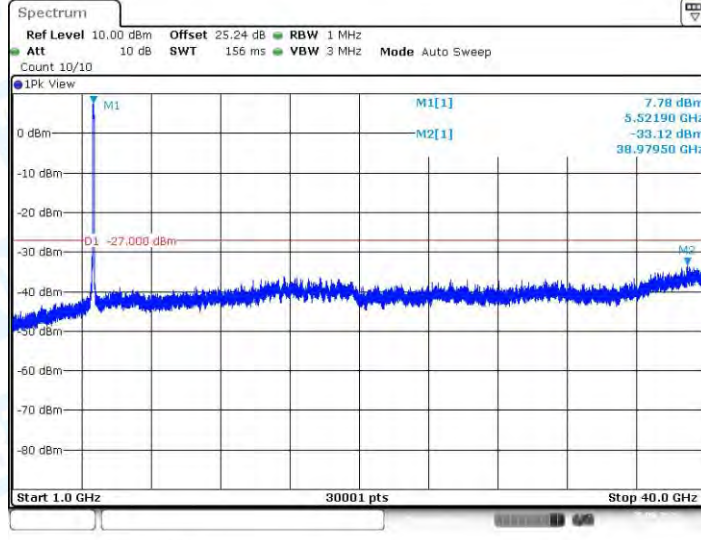
11AC80-SDM_Ant1_5530_1000~40000
