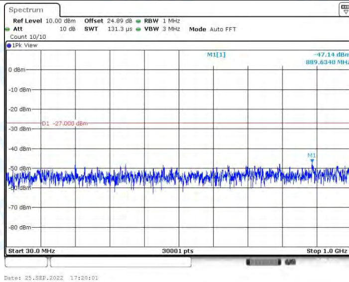
11AC80-SDM_Ant2_5290_1000~40000
