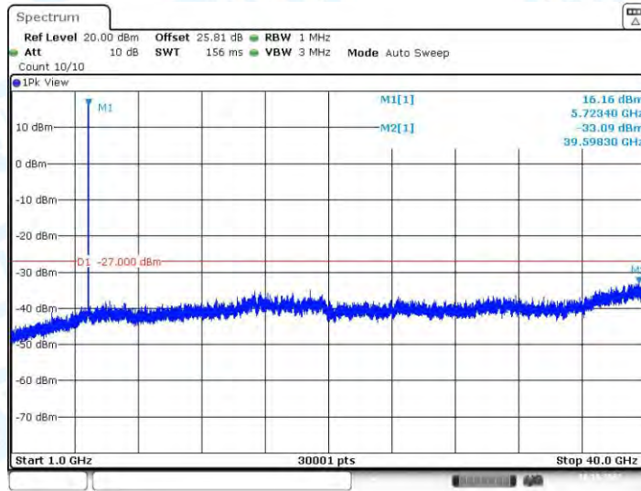
11N20-SDM_Ant2_5720_1000~40000
