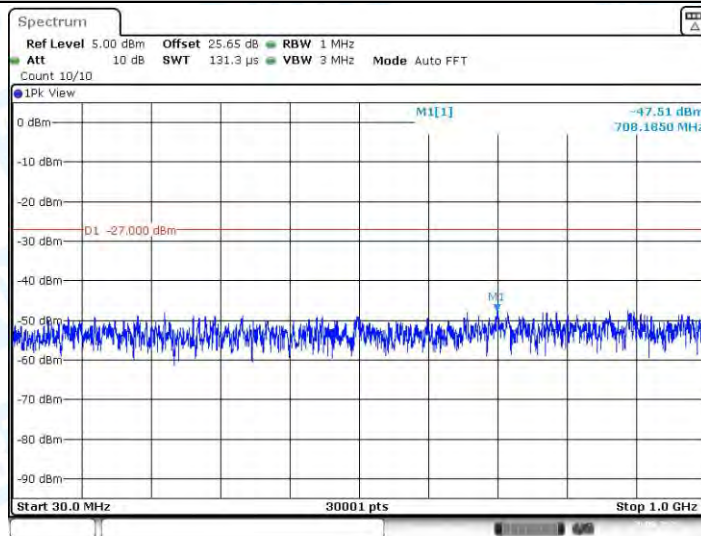
11N20-SDM_Ant1_5745_30~1000
