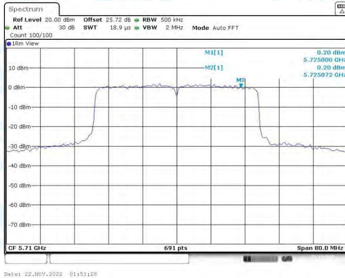
11AX40-CDD_Ant2_5710_UNII-3
