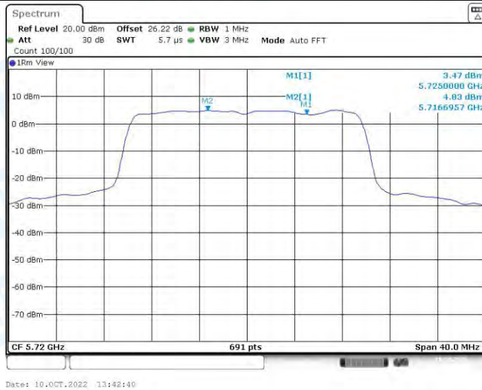
11AX20-SDM_Ant2_5720_UNII-2C
