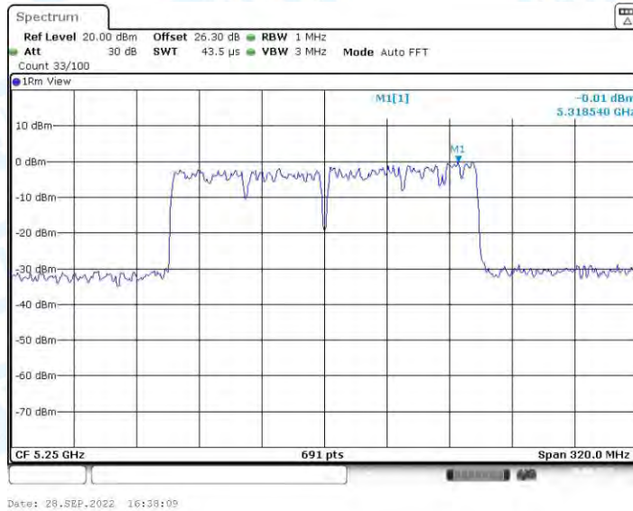
11AC160-SDM_Ant2_5250
