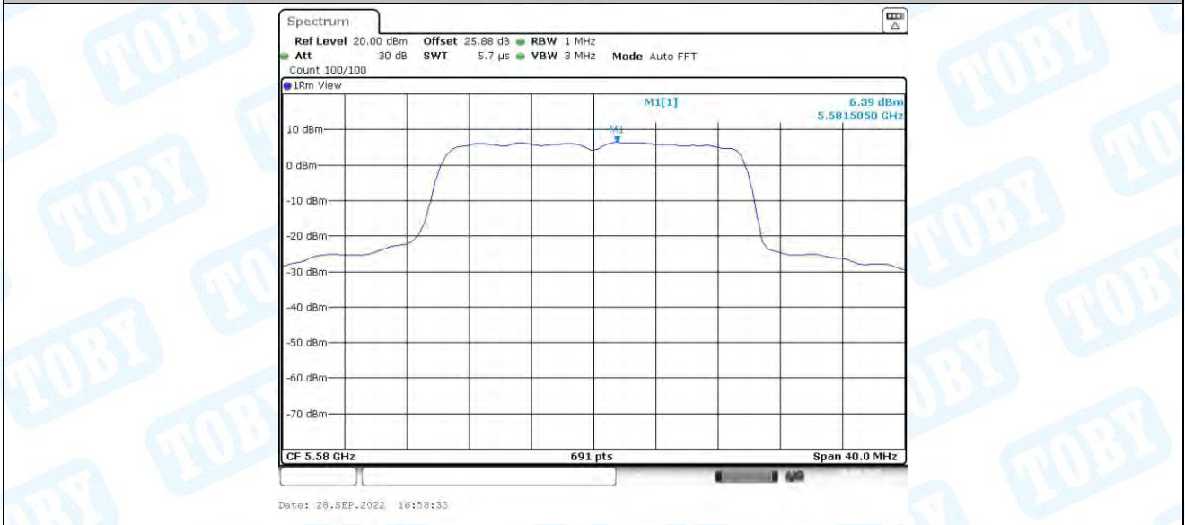
11AX20-SDM_Ant2_5580
