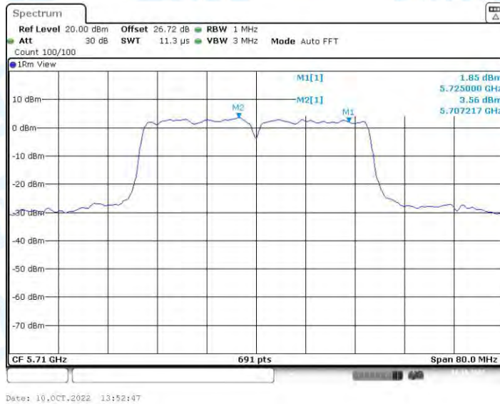
11AC40-SDM_Ant2_5710_UNII-2C
