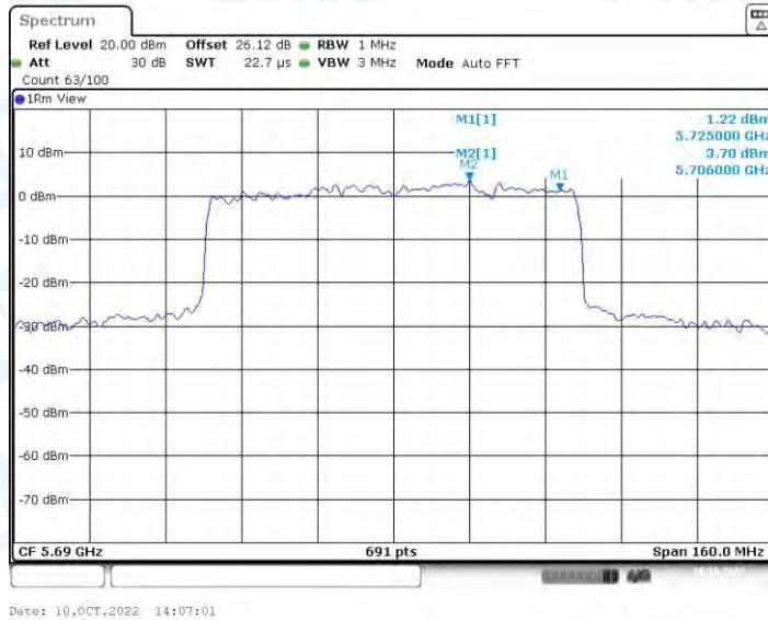
11AX80-SDM_Ant2_5690_UNII-2C
