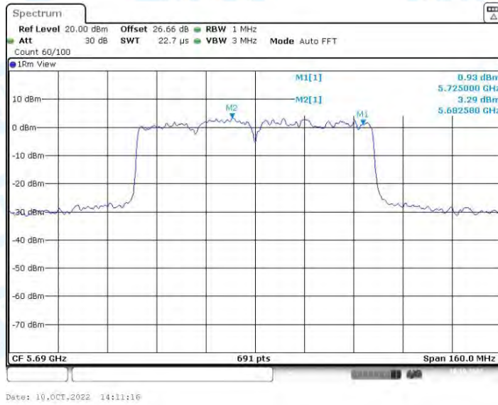
11AC80-SDM_Ant2_5690_UNII-2C
