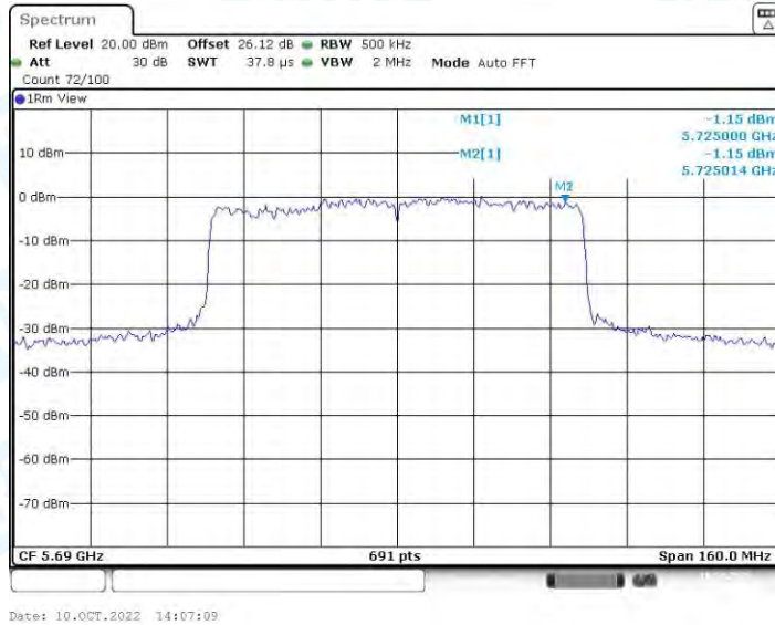
11AX80-SDM_Ant2_5690_UNII-3
