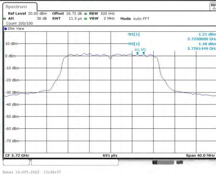
11AC20-SDM_Ant2_5720_UNII-3
