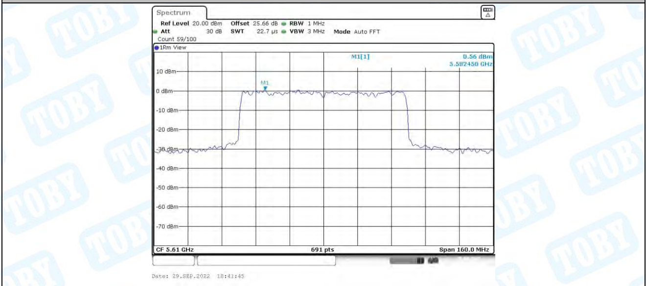
11AX80-SDM_Ant2_5610
