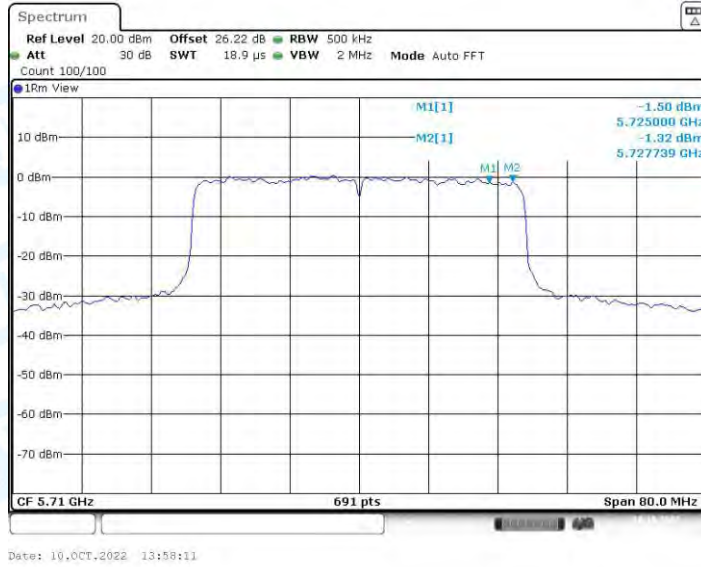
11AX40-SDM_Ant2_5710_UNII-3
