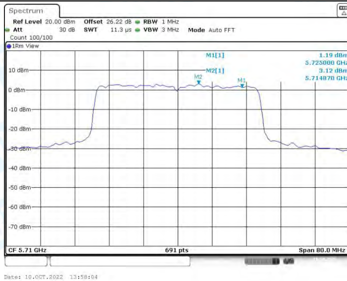
11AX40-SDM_Ant2_5710_UNII-2C
