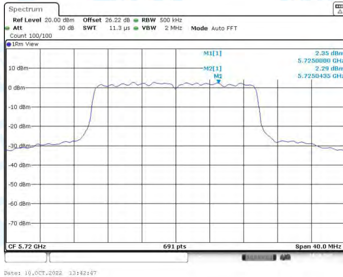
11AX20-SDM_Ant2_5720_UNII-3
