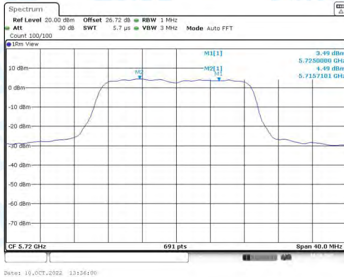
11AC20-SDM_Ant2_5720_UNII-2C
