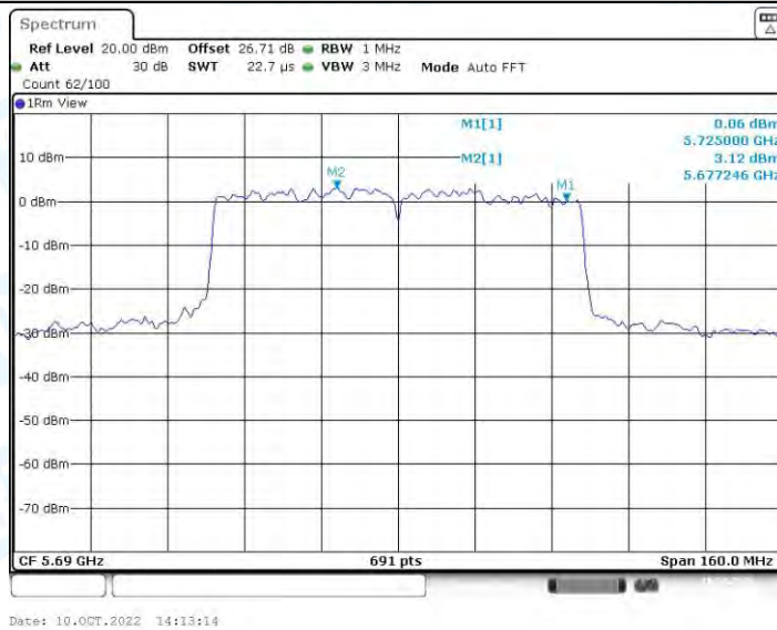
11AC80-SDM_Ant1_5690_UNII-3
