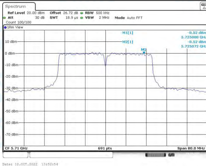
11AC40-SDM_Ant2_5710_UNII-3
