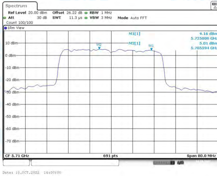
11AX40-SDM_Ant1_5710_UNII-3
