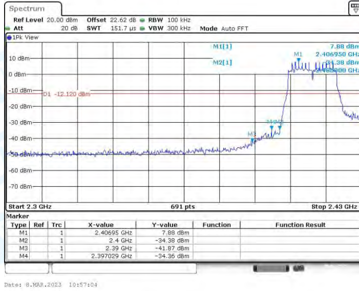
VHT20-SDM_Ant2_Low_2412
