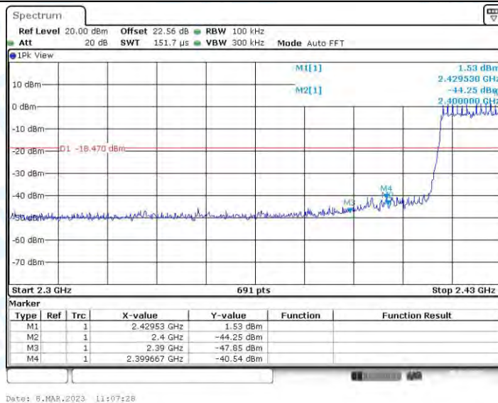
VHT40-SDM_Ant2_Low_2422
