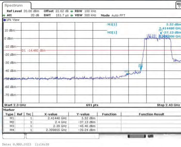
11AX20-SDM_Ant2_Low_2412
