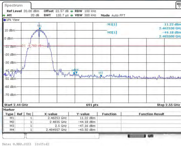
11G-SISO_Ant1_Low_2412
