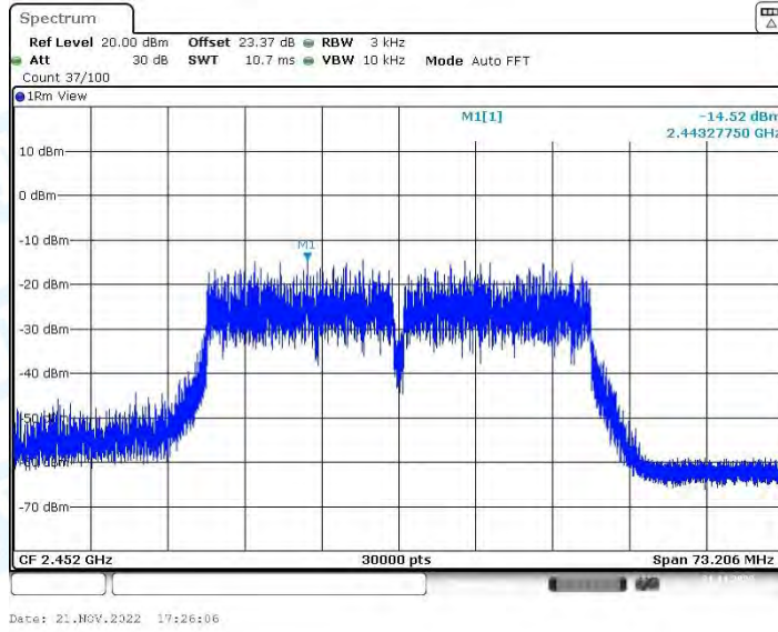
VHT40-CDD_Ant2_2452
