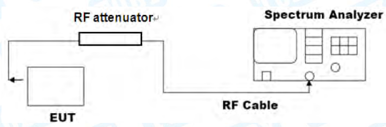
Above 1GHz Test Setup Conducted measurement
