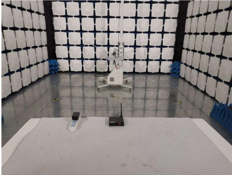
Blow 1GHz for radiated emission test setup
