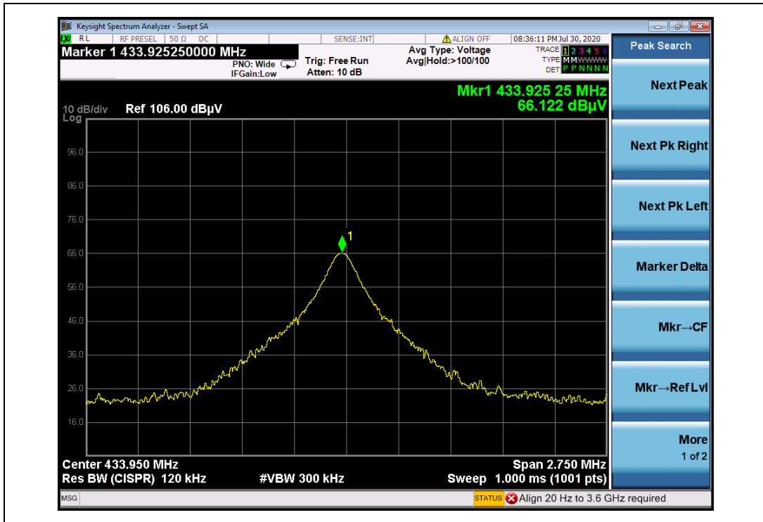
(433.92MHz, Antenna Horizontal)
