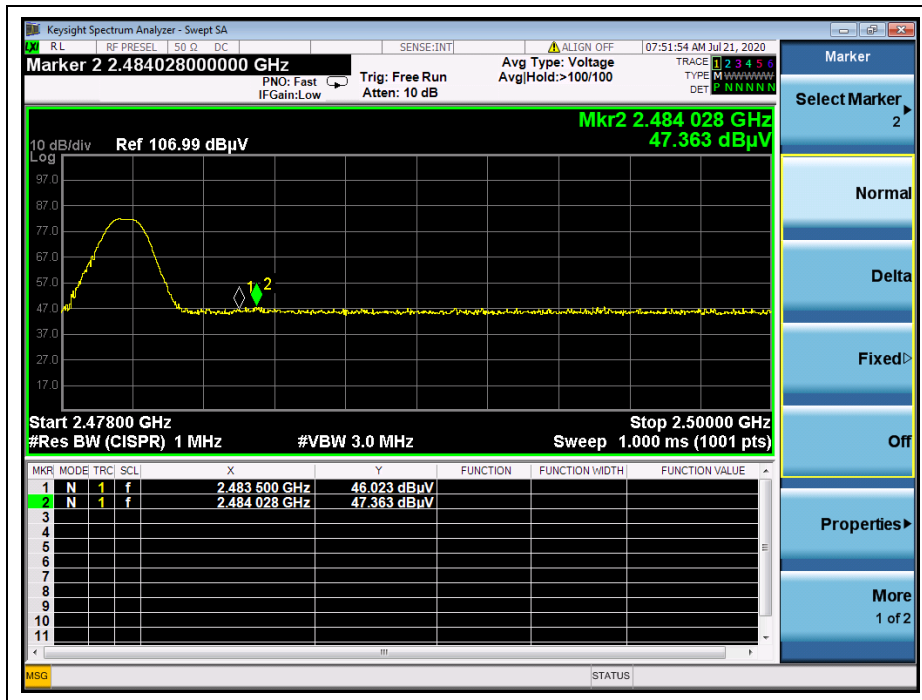
(PEAK,Channel = 78,GFSK)
