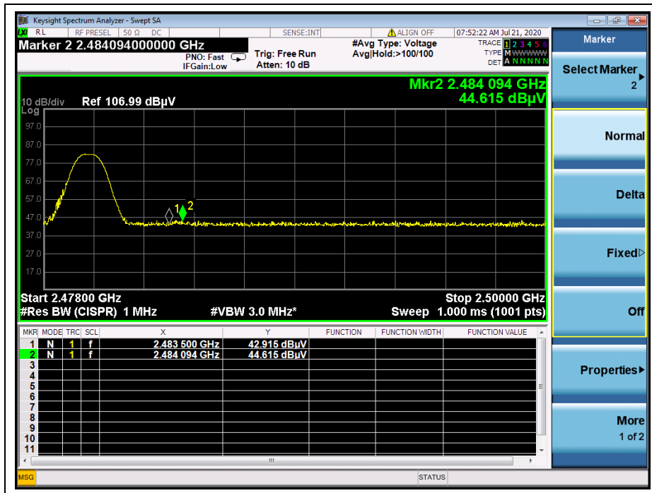
(AVERAGE,Channel = 78, GFSK)
