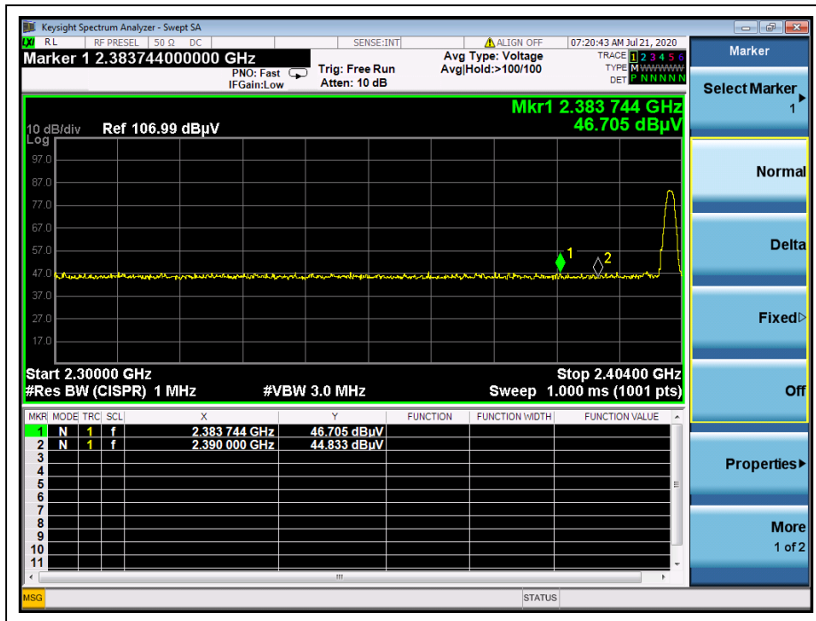
(PEAK,Channel = 0, GFSK)
