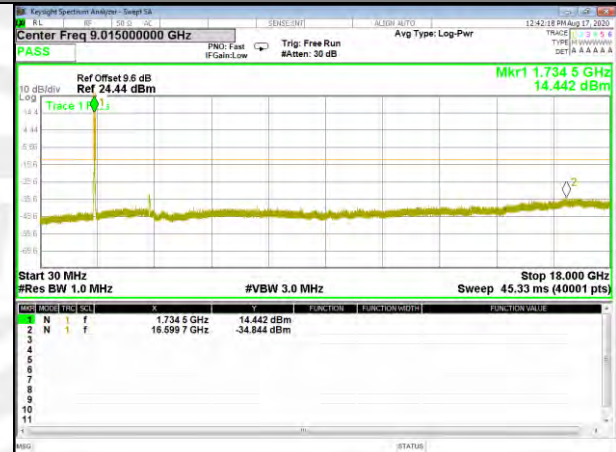
Band4_20M_16QAM_High
