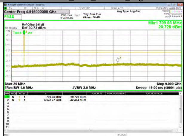
Band12_10M_16QAM_High
