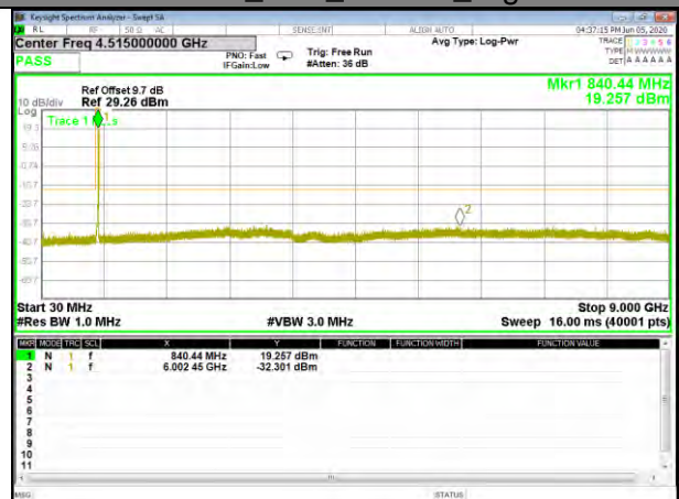
Band5_10M_16QAM_High
