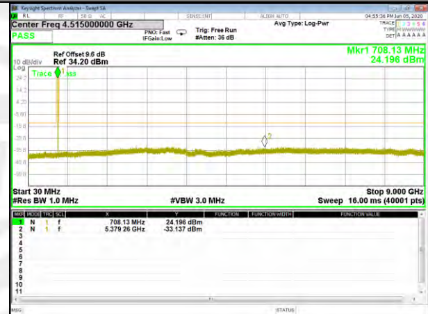
Band12_1.4M_16QAM_High
