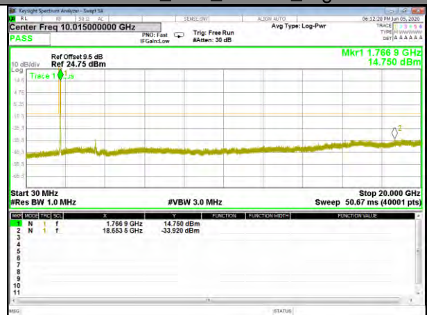
Band66_15M_16QAM_High
