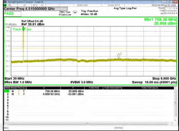
Band12_10M_16QAM_Middle
