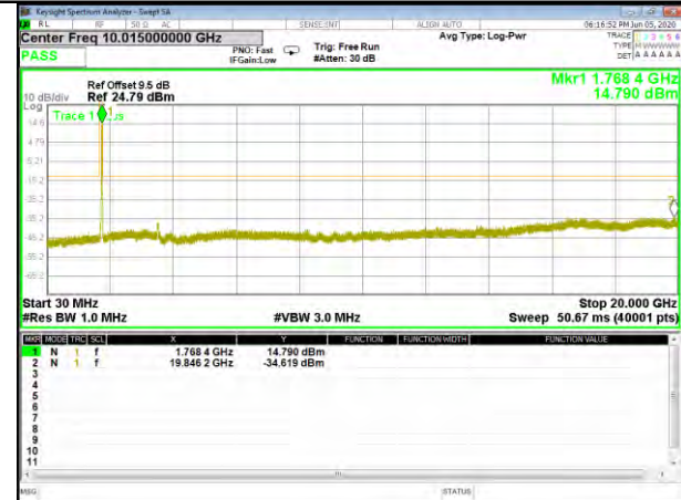
Band66_20M_QPSK_High
