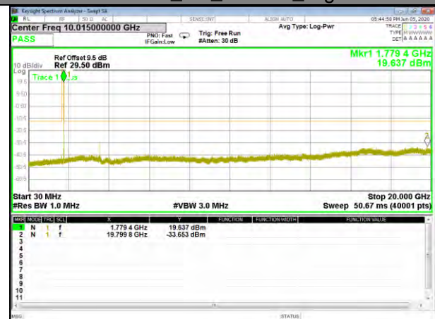
Band66_3M_16QAM_High
