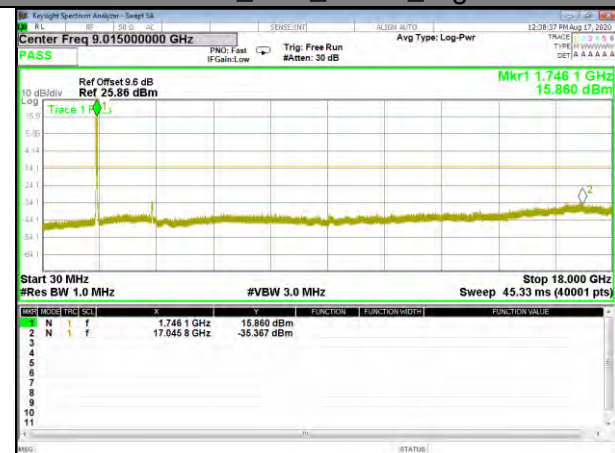
Band4_20M_QPSK_High
