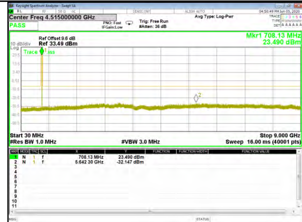
Band12_1.4M_QPSK_High
