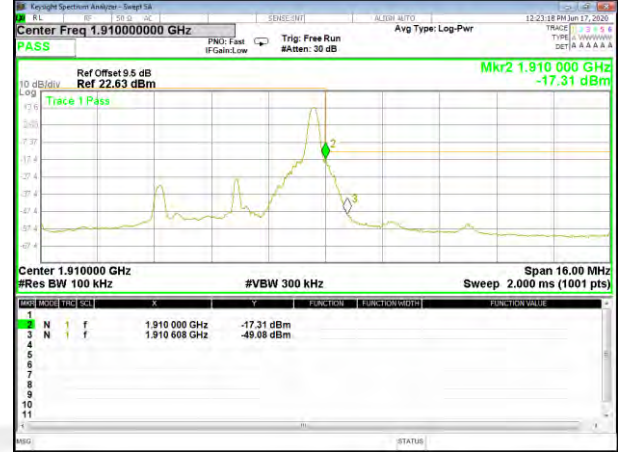
Band2_5M_QPSK_High_Full-RB
