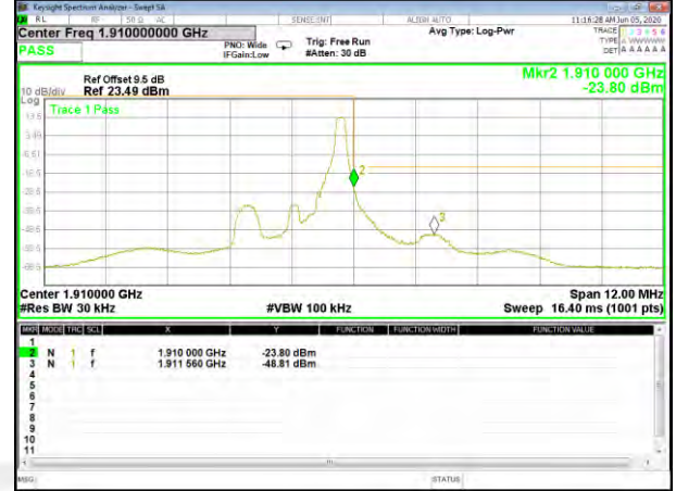
Band2_1.4M_16QAM_High_Full-RB
