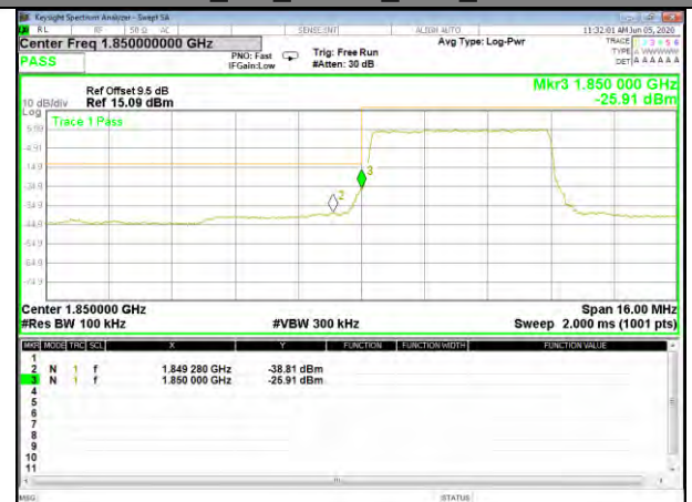
Band2_5M_QPSK_Low_Full-RB
