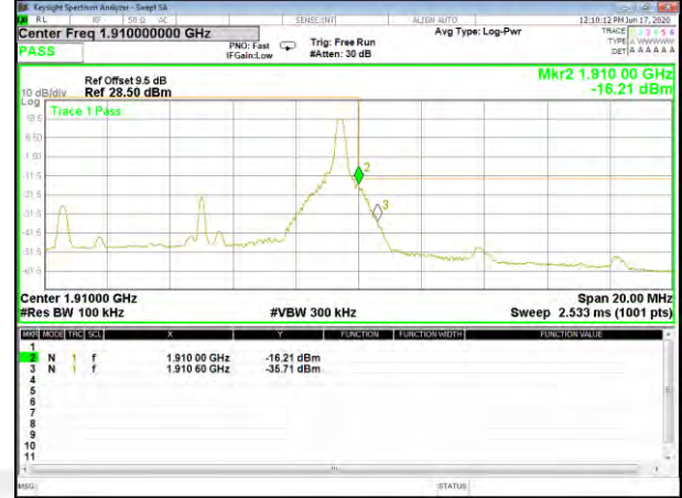
Band2_10M_16QAM_High_Full-RB
