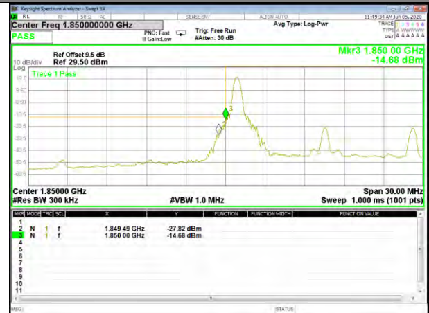
Band2_15M_QPSK_Low_1-RB
