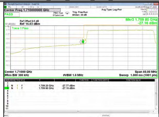
Band4_20M_QPSK_Low_Full-RB
