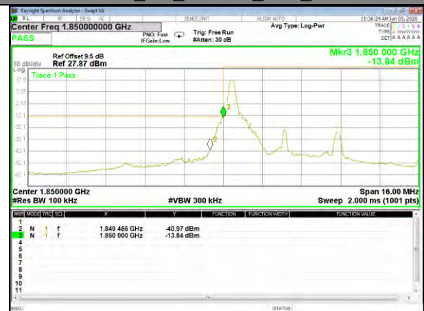
Band2_5M_16QAM_Low_1-RB
