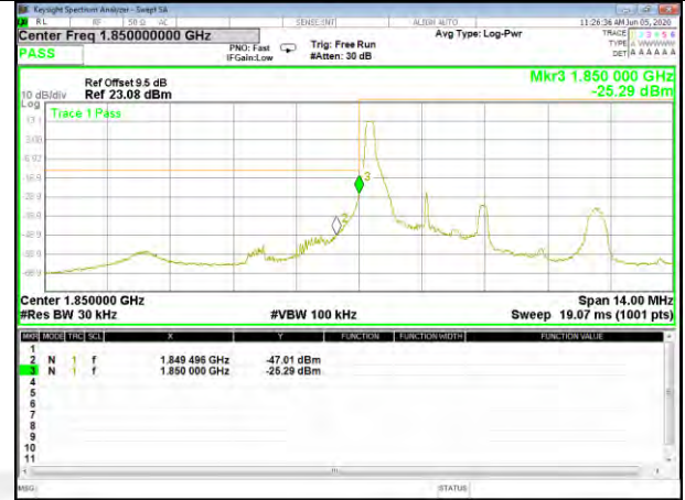
Band2_3M_16QAM_Low_Full-RB
