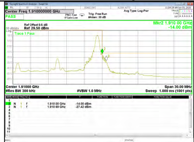
Band2_15M_16QAM_High_1-RB
