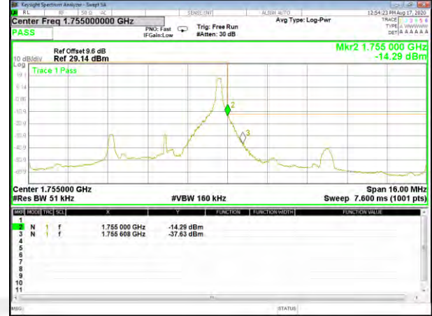
Band4_5M_QPSK_High_Full-RB
