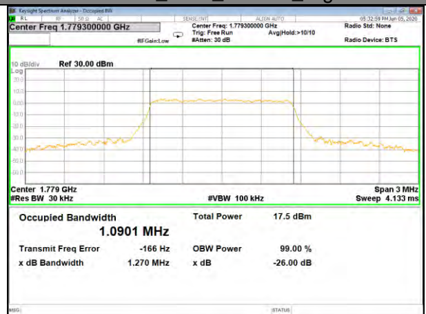
Band66_1.4M_16QAM_High
