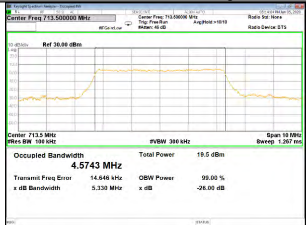
Band12_5M_16QAM_High
