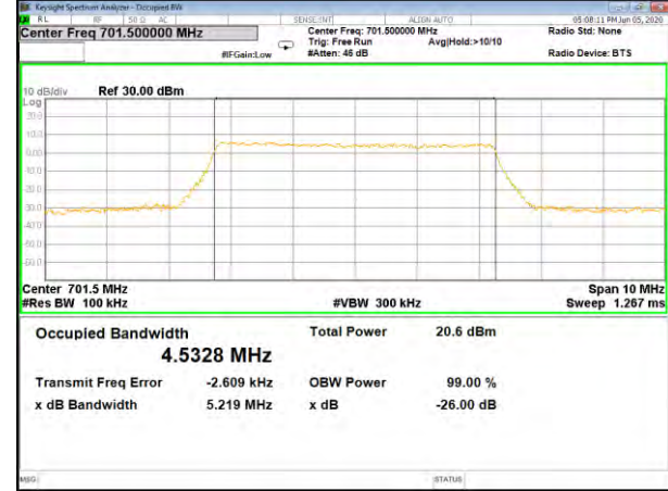
Band12_5M_QPSK_Middle
