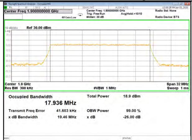
Band2_20M_16QAM_High
