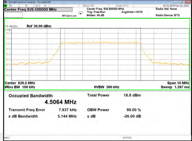
Band5_5M_16QAM_Middle
