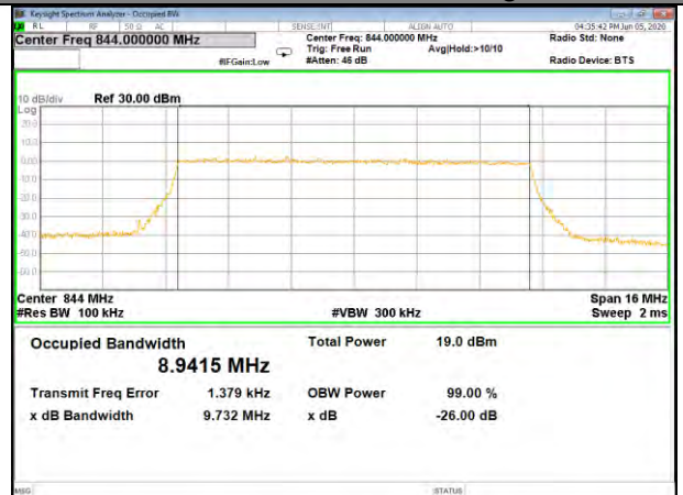
Band5_10M_16QAM_High
