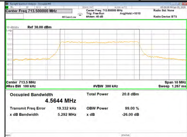
Band12_5M_QPSK_High
