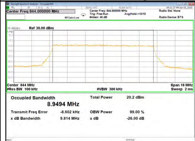
Band5_10M_QPSK_High
