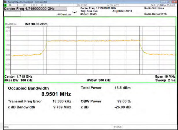
Band66_10M_16QAM_Middle
