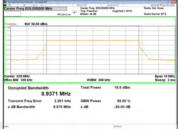
Band5_10M_16QAM_Middle
