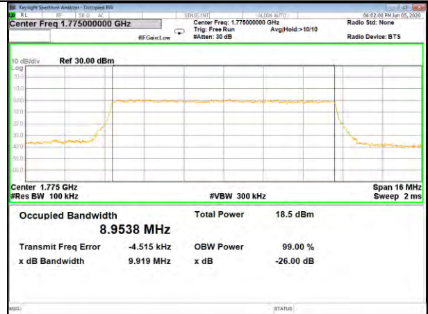
Band66_10M_16QAM_High
