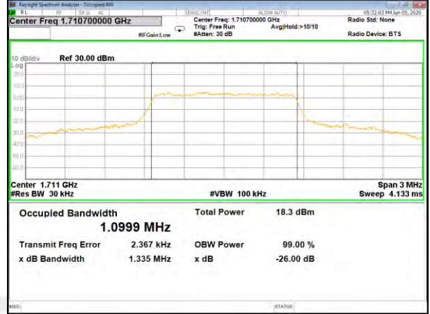
Band66_1.4M_16QAM_Middle
