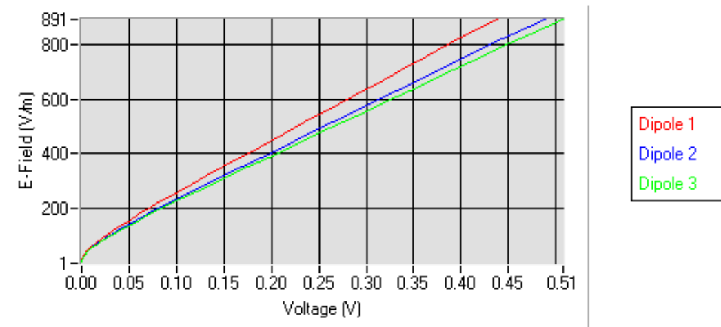
Calibration curves
