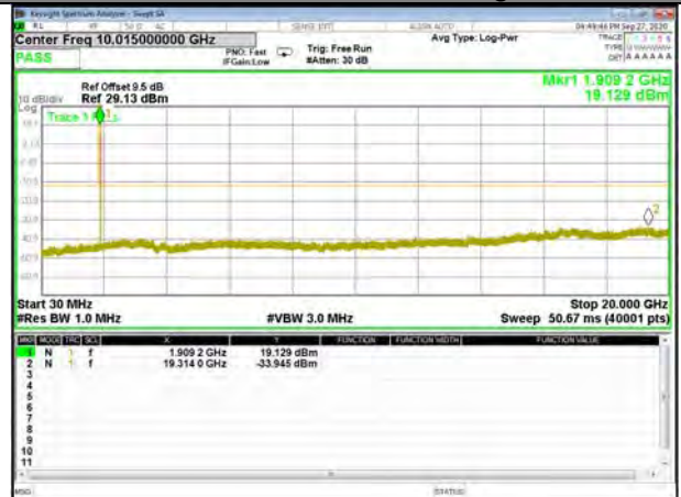
Band2_3M_16QAM_High
