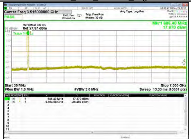
Band71_15M_16QAM_High
