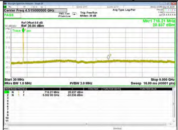
Band12_5M_16QAM_High
