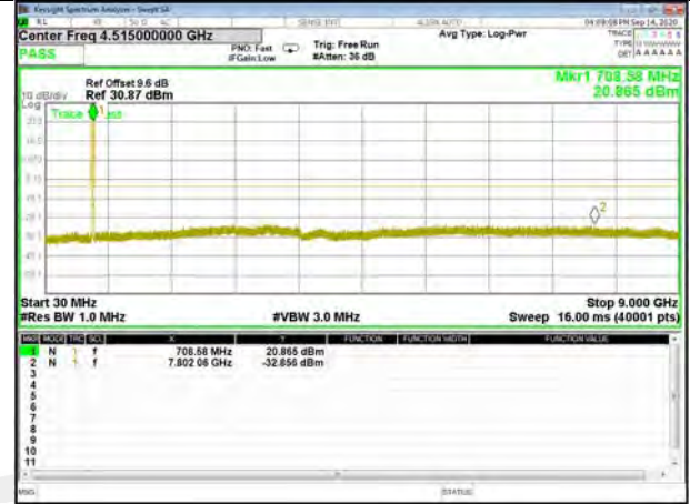
Band12_10M_16QAM_Middle
