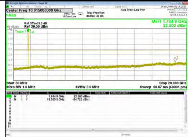
Band66_1.4M_QPSK_High
