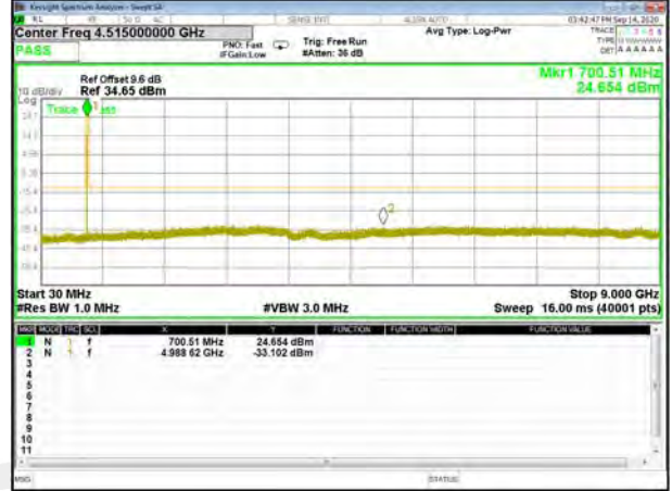
Band12_1.4M_16QAM_Middle
