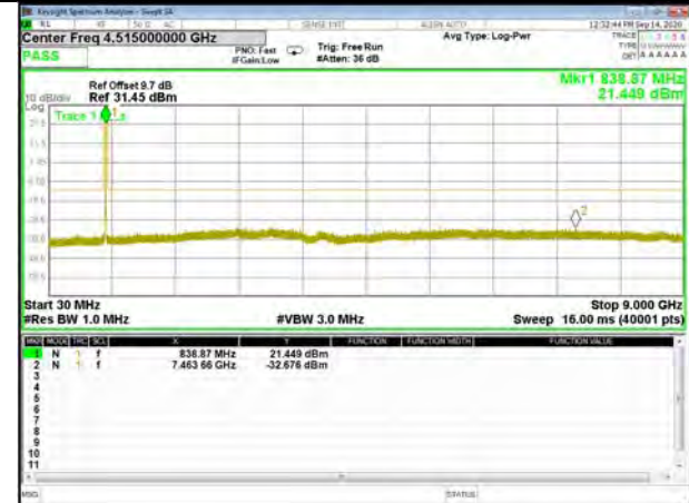
Band5_5M_QPSK_High
