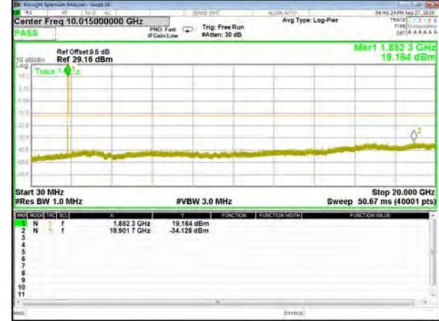
Band2_3M_QPSK_Middle
