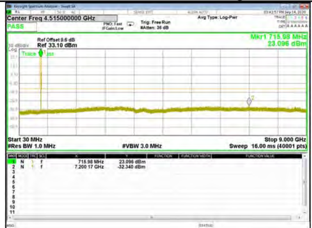
Band12_1.4M_16QAM_High
