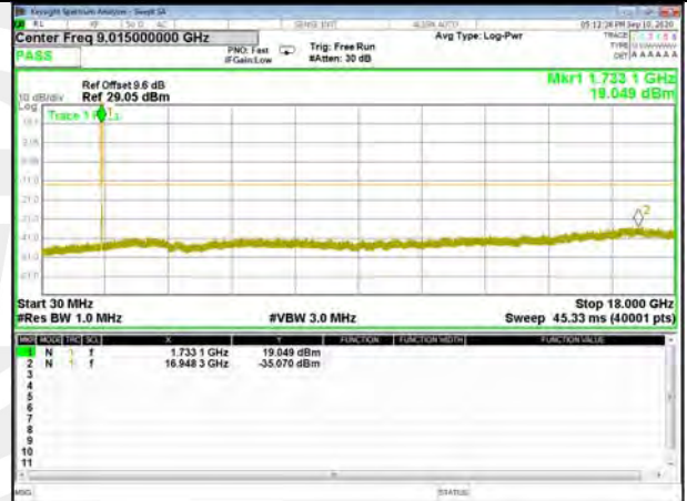
Band4_5M_16QAM_High
