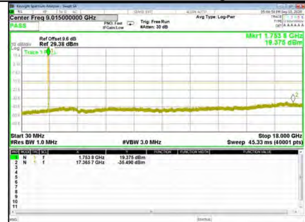
Band4_5M_QPSK_High
