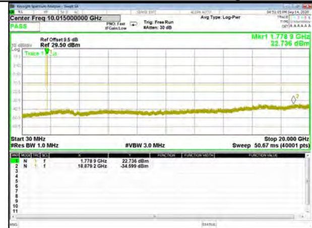
Band66_1.4M_QPSK_High
