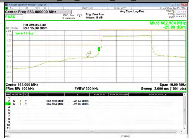
Band71_5M_16QAM_Low_Full-RB
