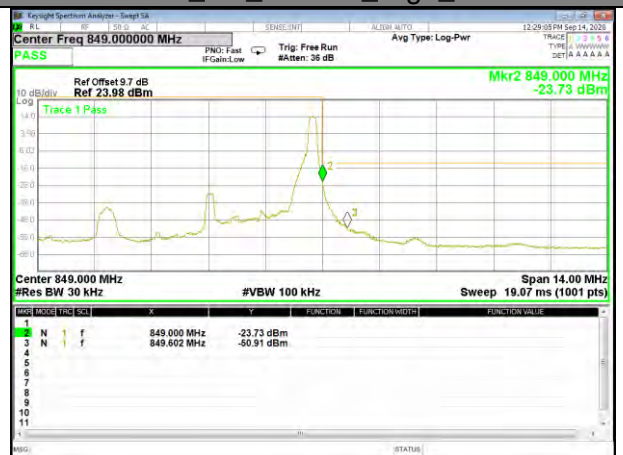
Band5_3M_16QAM_High_1-RB
