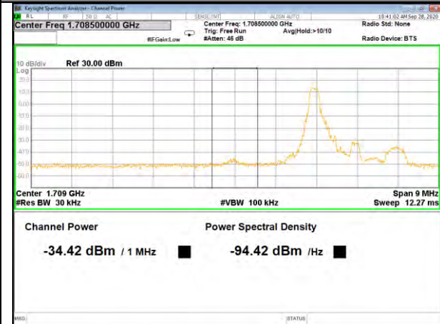
Band66_1.4M_16QAM_Low_Full-RB
