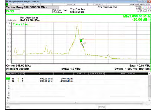
Band71_20M_16QAM_High_1-RB
