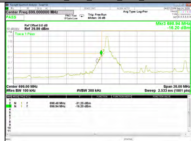
Band12_10M_QPSK_Low_1-RB
