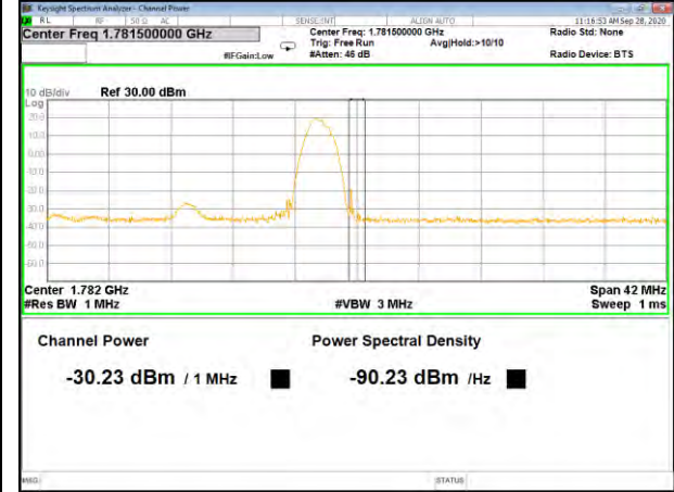
Band66_20M_16QAM_High_Full-RB
