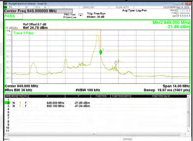
Band5_3M_QPSK_High_Full-RB
