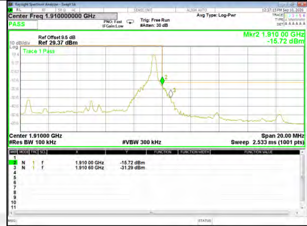
Band2_10M_16QAM_High_Full-RB
