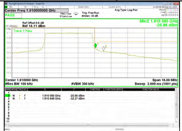
Band2_5M_16QAM_High_Full-RB
