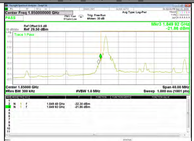
Band2_20M_16QAM_Low_1-RB
