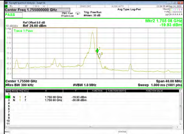
Band4_20M_16QAM_High_Full-RB
