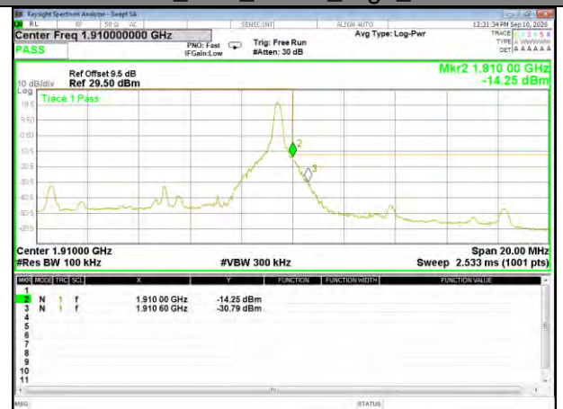
Band2_10M_QPSK_High_1-RB
