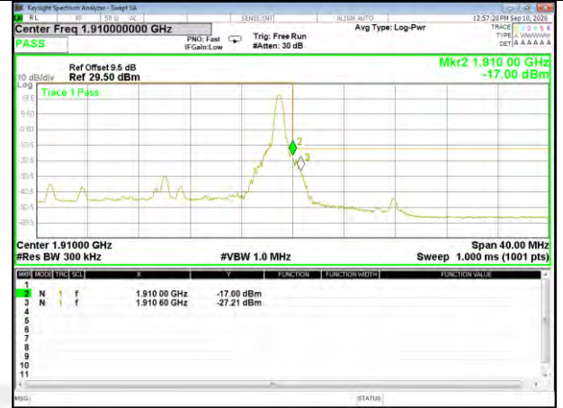
Band2_20M_QPSK_High_Full-RB
