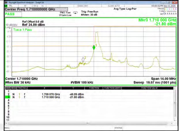
Band4_3M_16QAM_Low_Full-RB
