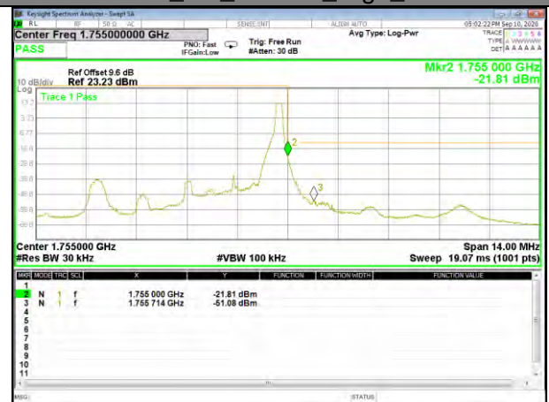
Band4_3M_16QAM_High_1-RB
