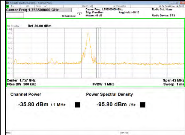
Band4_20M_16QAM_High_Full-RB
