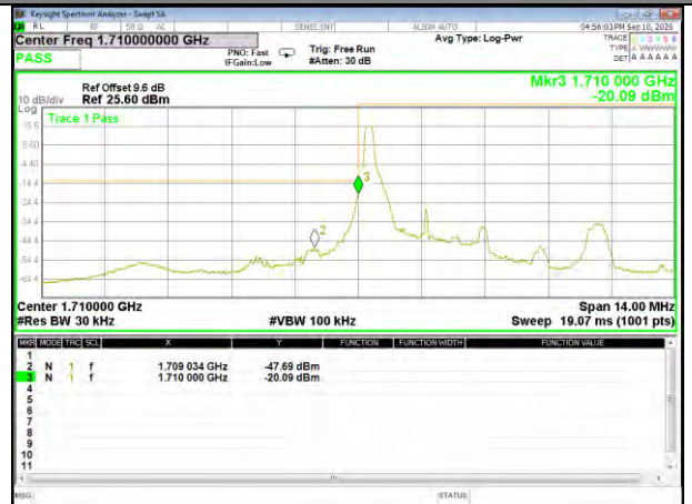
Band4_3M_QPSK_Low_1-RB
