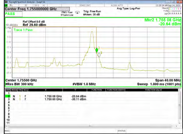
Band4_20M_QPSK_High_Full-RB
