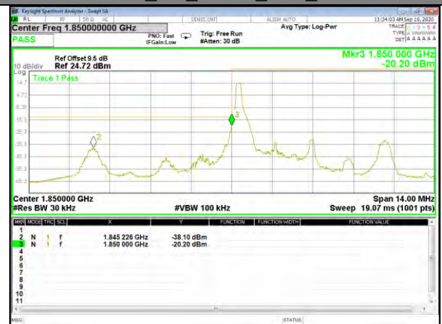
Band2_3M_QPSK_Low_1-RB
