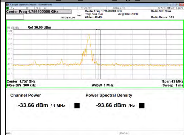
Band4_15M_16QAM_High_1-RB
