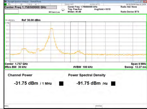
Band4_1.4M_16QAM_High_Full-RB
