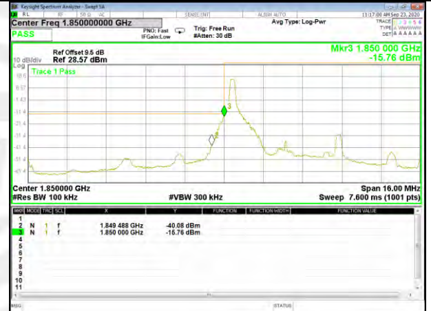
Band2_5M_QPSK_Low_Full-RB
