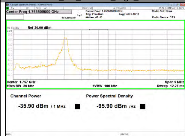
Band4_3M_16QAM_High_1-RB
