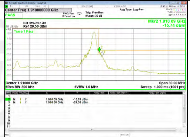
Band2_15M_QPSK_High_Full-RB
