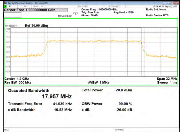
Band2_20M_16QAM_High
