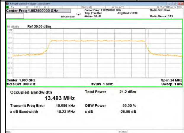
Band2_15M_QPSK_High
