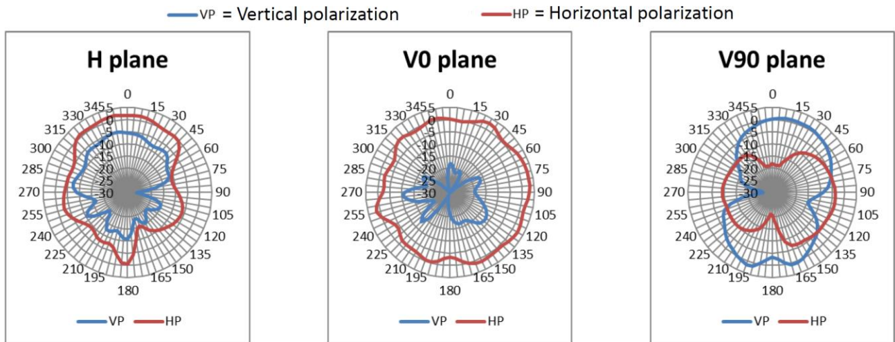
Figure 7 Niche Antenna 2.4 GHz Operation
