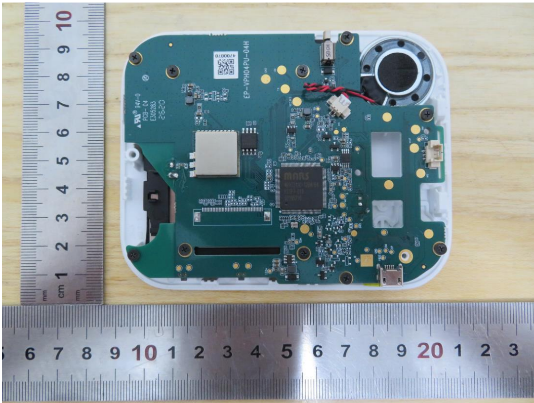
Internal View of EUT-4(VPH 04 PU)
