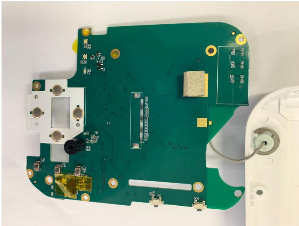
Internal View of EUT-9(VPH 02 PU)
