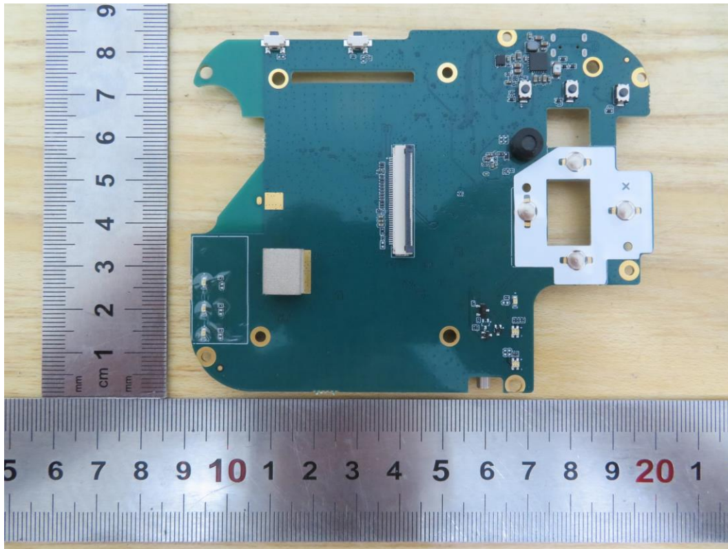
Internal View of EUT-6(VPH 04 PU)
