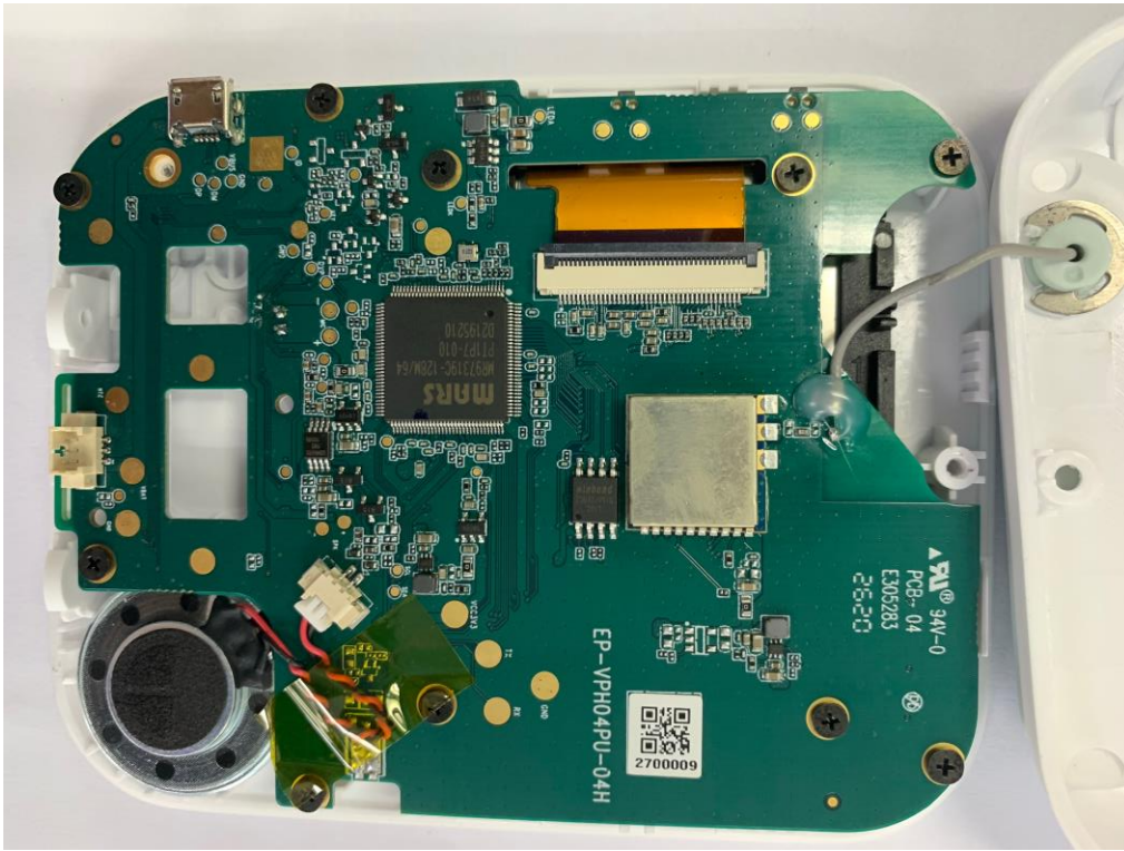
Internal View of EUT-8(VPH 02 PU)
