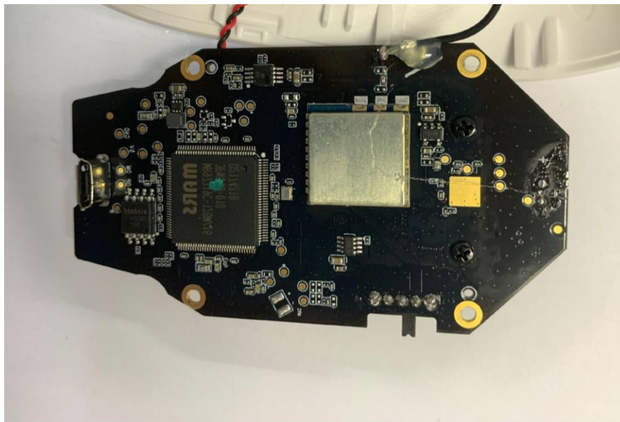
Internal View of EUT-6(VPH 01 BU)
