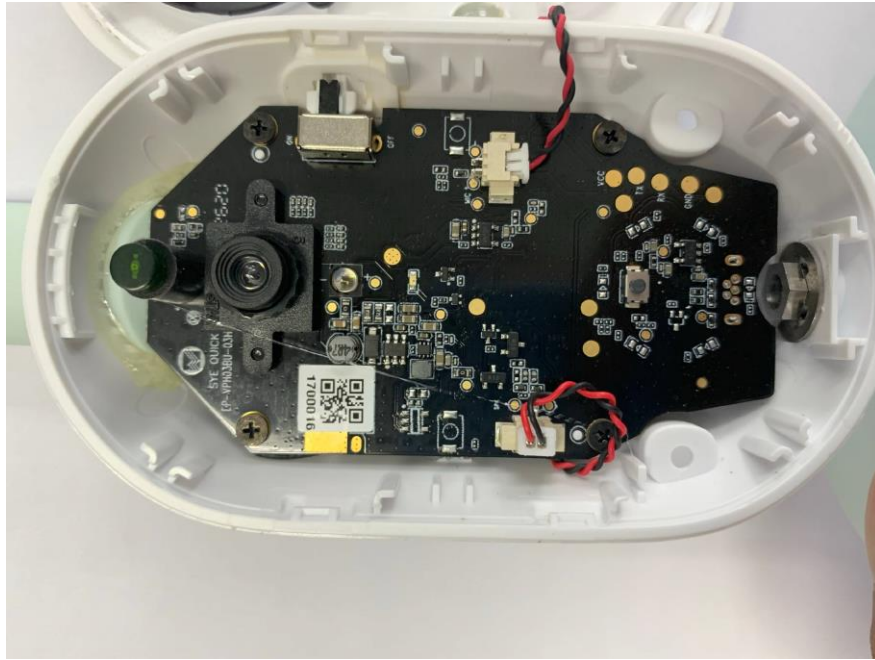
Internal View of EUT-6(VPH 01 BU)
