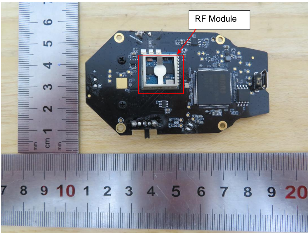
Internal View of EUT-4(VPH 03 BU)
